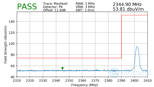
Plot 7-38. Radiated Restricted Lower Band Edge Measurement (Peak)
