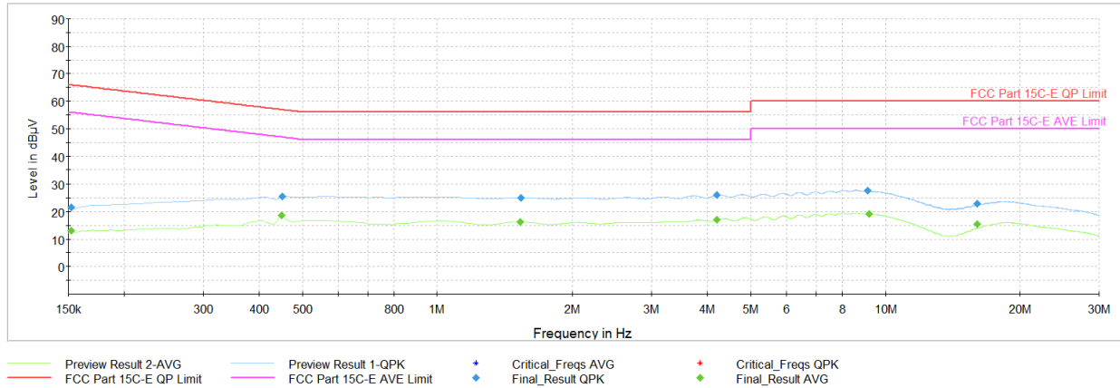
Plot 7-44. AC Line-Conducted Test Plot (L1, GFSK – Ch.39, with AC/DC Adapter)
