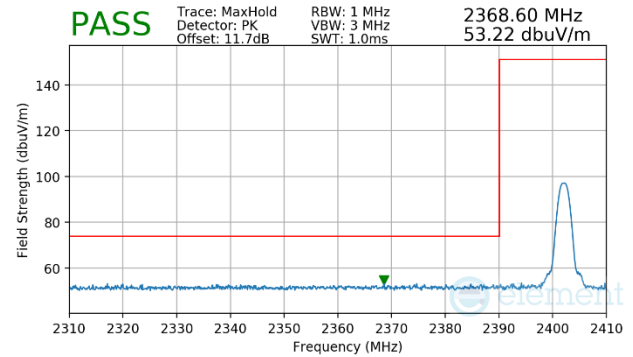
Plot 7-36. Radiated Restricted Lower Band Edge Measurement (Peak)
