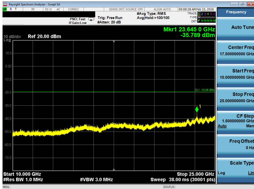
Plot 7-32. Conducted Spurious Plot (Bluetooth (LE), 1Mbps – Ch. 39)
