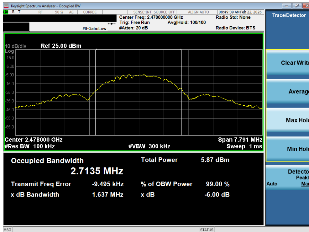
Plot 7-12.6dB BW Plot (Bluetooth (LE), 2Mbps – Ch. 36)
