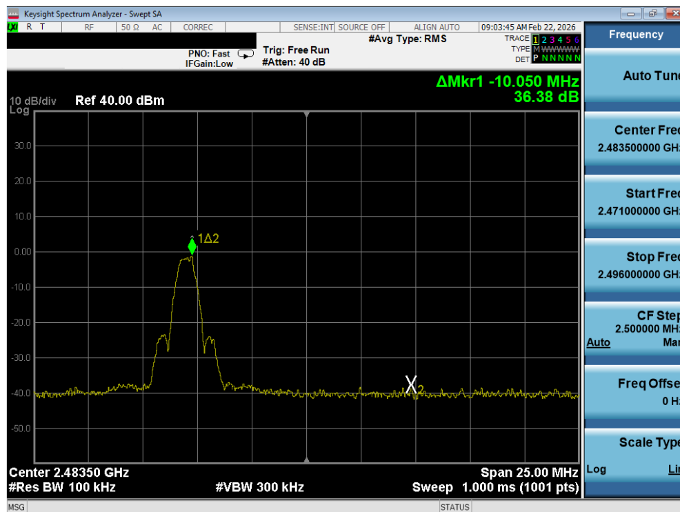
Plot 7-22. Band Edge Plot (Bluetooth (LE), 1Mbps – Ch. 36)
