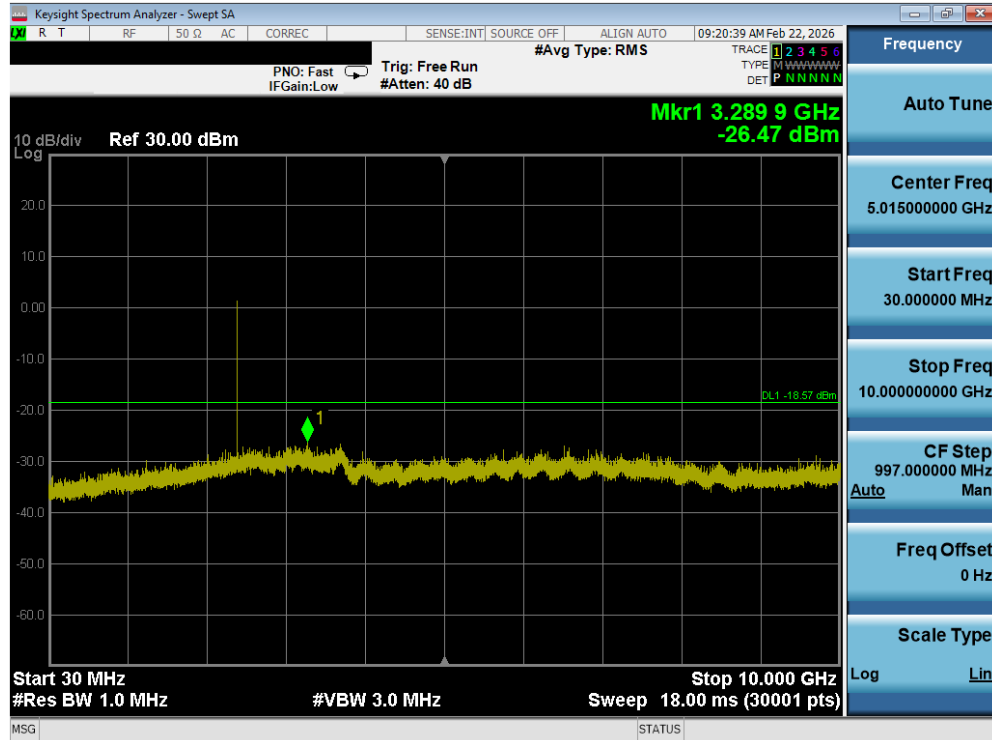
Plot 7-27. Conducted Spurious Plot (Bluetooth (LE), 1Mbps – Ch. 37)
