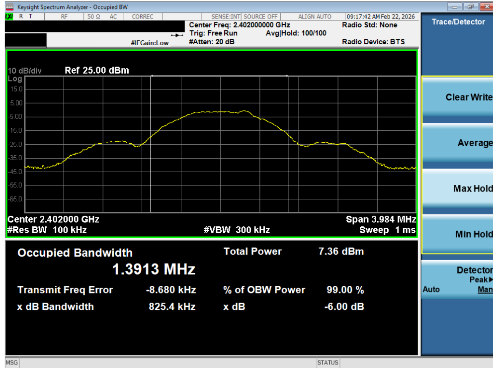
Plot 7-7.6dB BW Plot (Bluetooth (LE), 1Mbps – Ch. 37)
