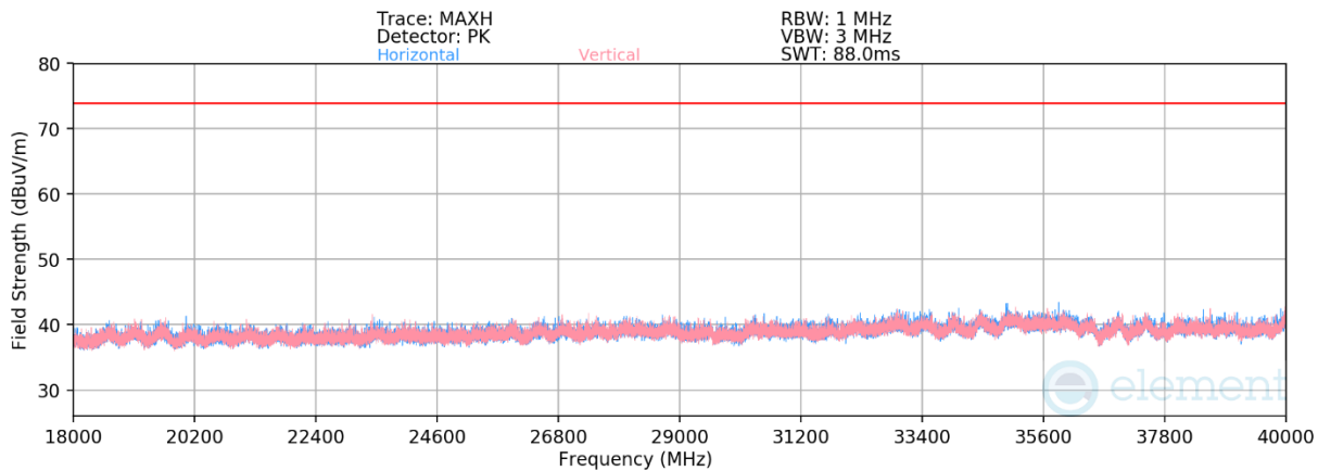
Plot 7-41. Radiated Spurious Emissions Above 18 GHz (1Mbps – Ch. 17)
