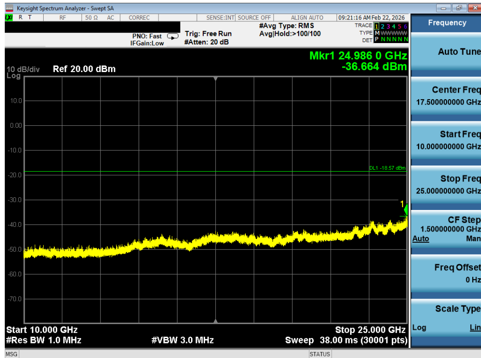
Plot 7-28. Conducted Spurious Plot (Bluetooth (LE), 1Mbps – Ch. 37)
