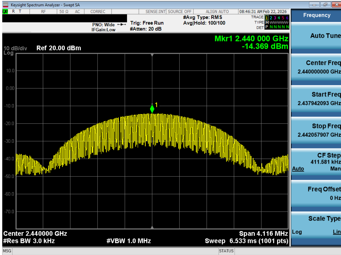
Plot 7-17. Power Spectral Density Plot (Bluetooth (LE), 2Mbps – Ch. 17)
