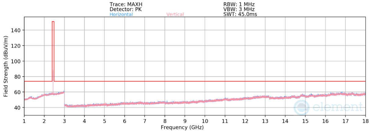
Plot 7-40. Radiated Spurious Emissions 1-18 GHz (1Mbps – Ch. 17)
