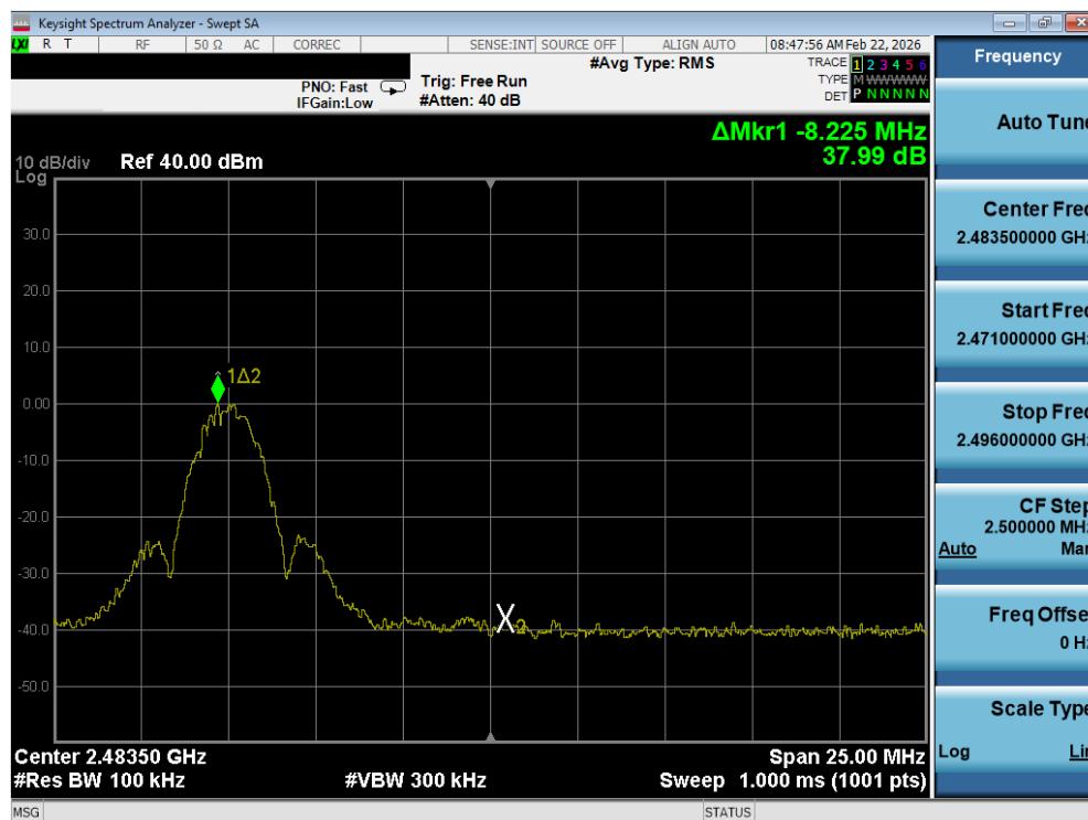
Plot 7-25. Band Edge Plot (Bluetooth (LE), 2Mbps – Ch. 35)
