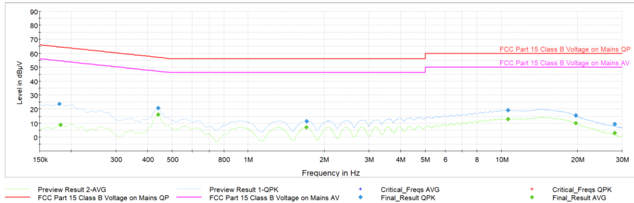
Plot 7-51. AC Line Conducted Plot with Bluetooth LE (N, 1Mbps – Ch.17, with AC/DC Adapter)
