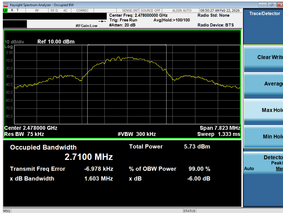
Plot 7-6. 99% OBW Plot (Bluetooth (LE), 2Mbps – Ch. 36)
