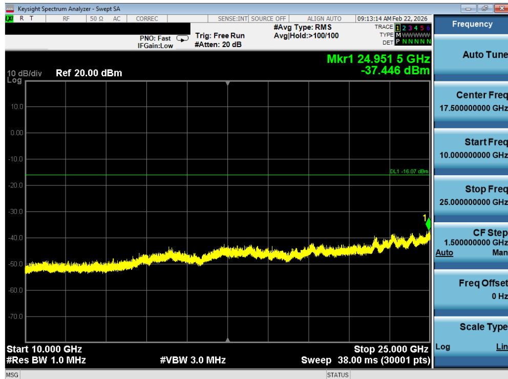
Plot 7-30. Conducted Spurious Plot (Bluetooth (LE), 1Mbps – Ch. 17)
