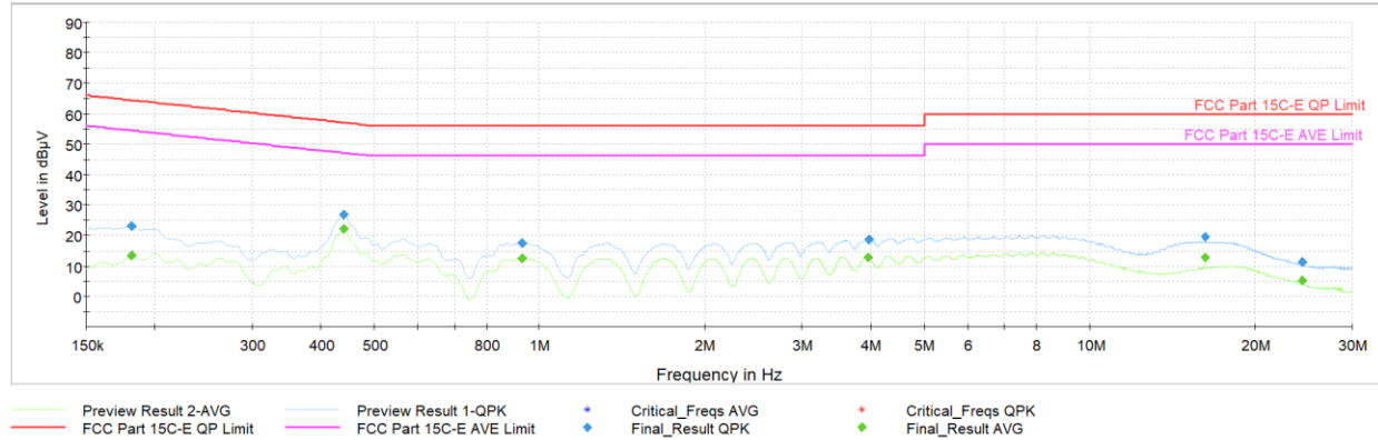
Plot 7-50. AC Line Conducted Plot with Bluetooth LE (L1, 1Mbps – Ch.17 with AC/DC Adapter)
