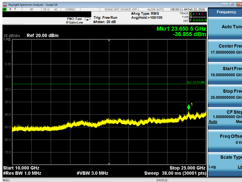
Plot 7-34. Conducted Spurious Plot (Bluetooth (LE), 2Mbps – Ch. 0)
