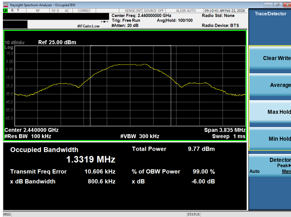
Plot 7-8. 6dB BW Plot (Bluetooth (LE), 1Mbps – Ch. 17)
