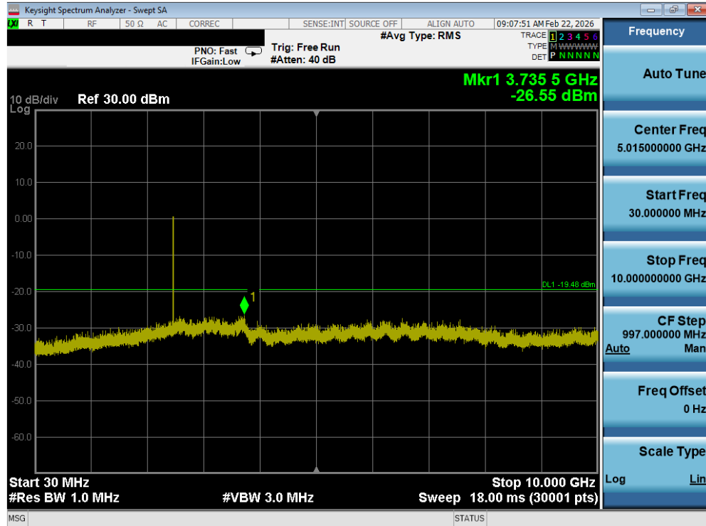
Plot 7-31. Conducted Spurious Plot (Bluetooth (LE), 1Mbps – Ch. 39)
