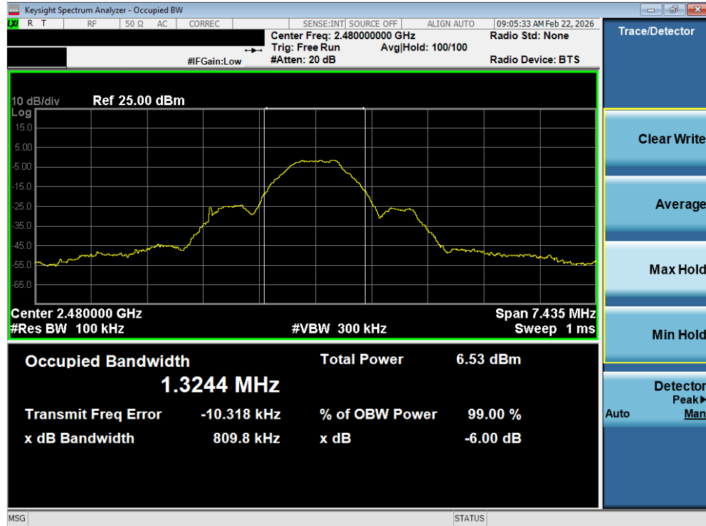
Plot 7-9. 6dB BW Plot (Bluetooth (LE), 1Mbps – Ch. 39)
