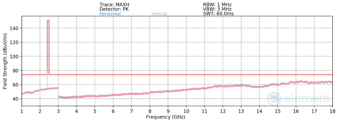
Plot 7-39. Radiated Spurious Emissions 1-18 GHz (1Mbps – Ch. 0)
