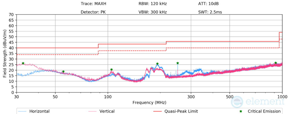
Plot 7-49. Radiated Spurious Emissions Below 1 GHz (1Mbps – Ch.17, Pol. H & V, with AC/DC Adapter)
