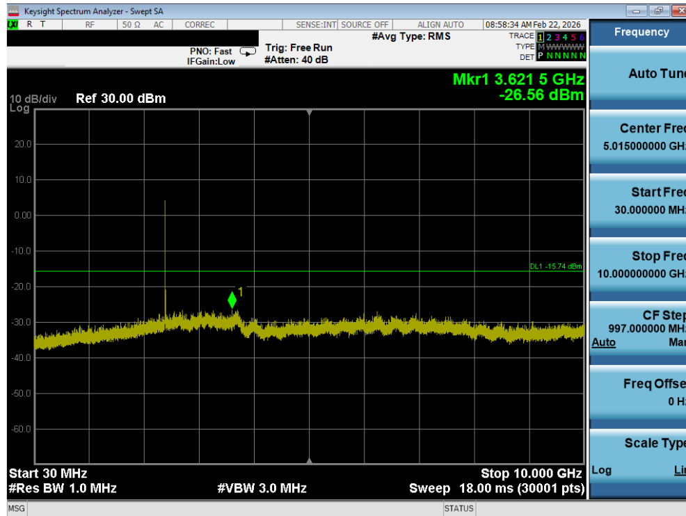
Plot 7-33. Conducted Spurious Plot (Bluetooth (LE), 2Mbps – Ch. 0)
