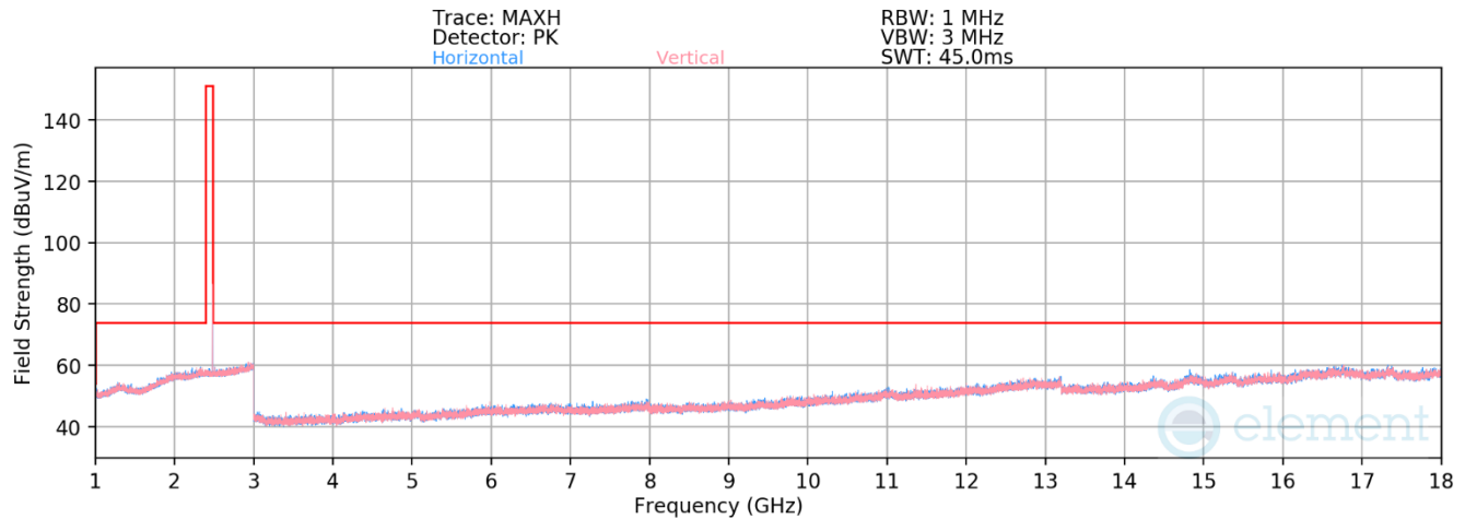
Plot 7-42. Radiated Spurious Emissions 1-18 GHz (1Mbps – Ch. 39)
