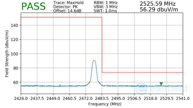
Plot 7-48. Radiated Restricted Upper Band Edge Measurement (Peak)
