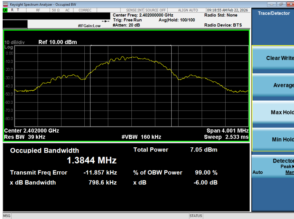
Plot 7-1. 99% OBW Plot (Bluetooth (LE), 1Mbps – Ch. 37)
