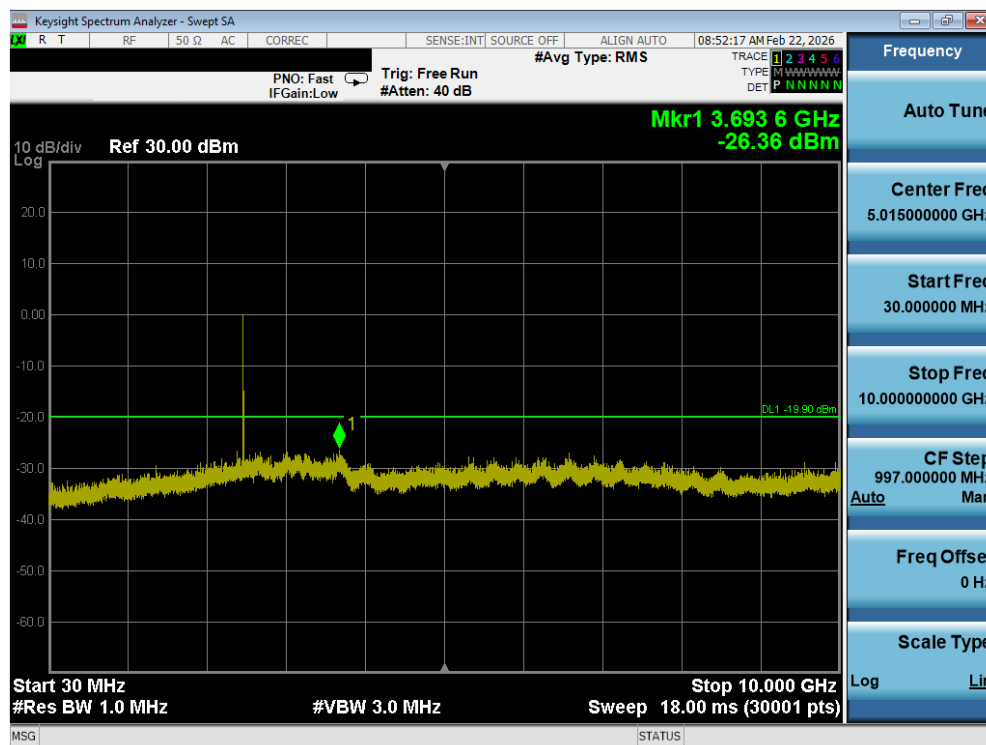
Plot 7-37. Conducted Spurious Plot (Bluetooth (LE), 2Mbps – Ch. 36)
