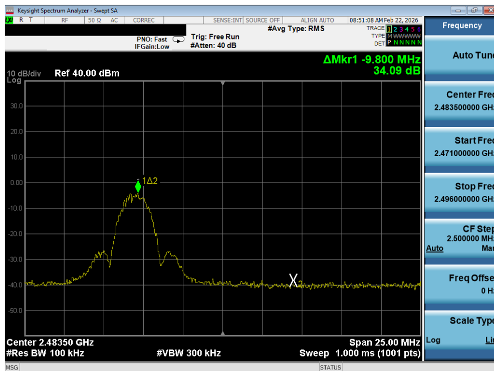
Plot 7-26. Band Edge Plot (Bluetooth (LE), 2Mbps – Ch. 36)
