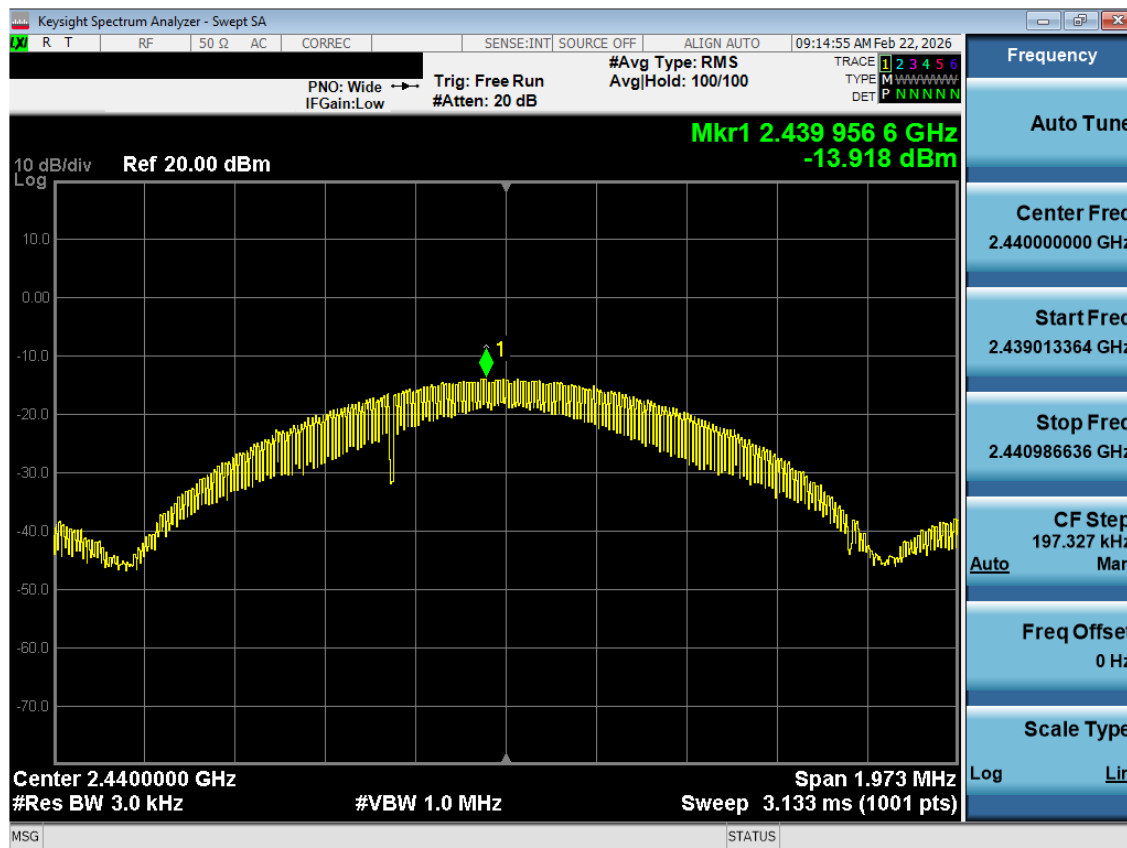
Plot 7-14. Power Spectral Density Plot (Bluetooth (LE), 1Mbps – Ch. 17)
