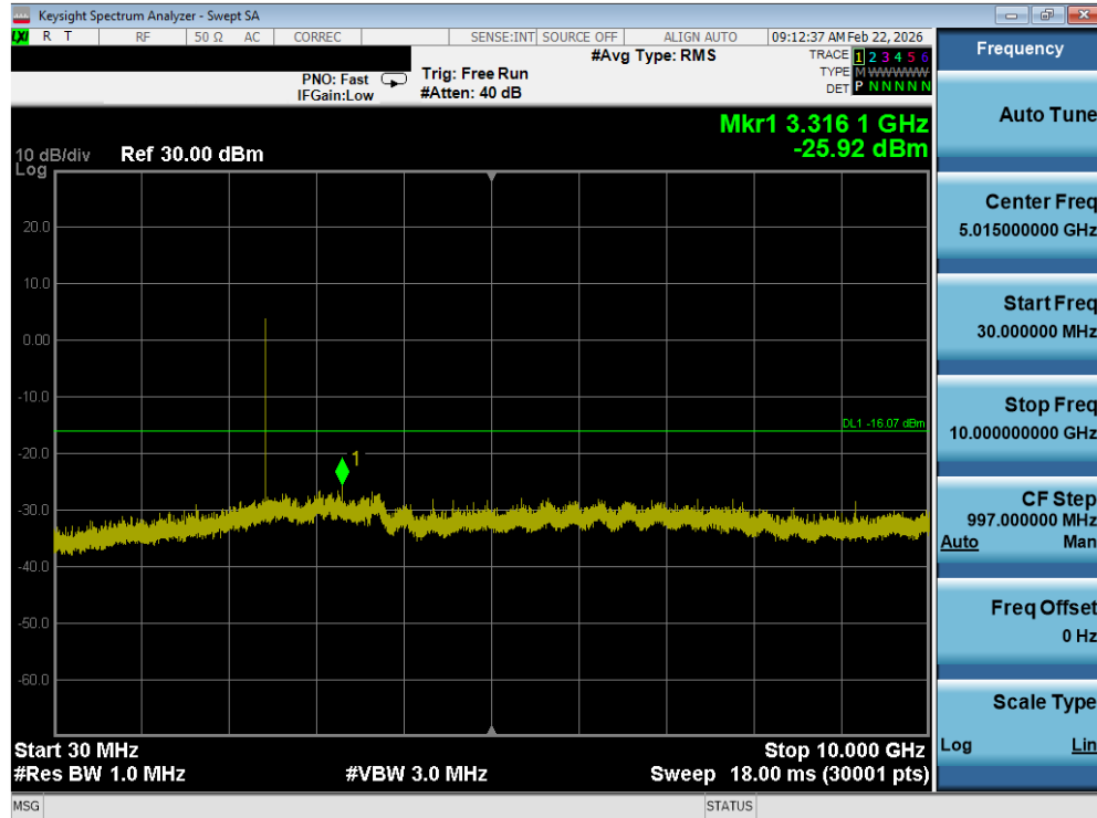
Plot 7-29. Conducted Spurious Plot (Bluetooth (LE), 1Mbps – Ch. 17)
