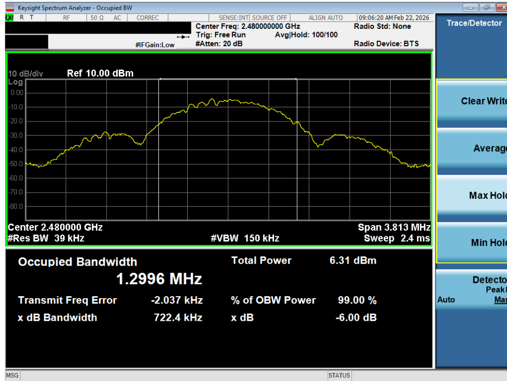
Plot 7-3. 99% OBW Plot (Bluetooth (LE), 1Mbps – Ch. 39)
