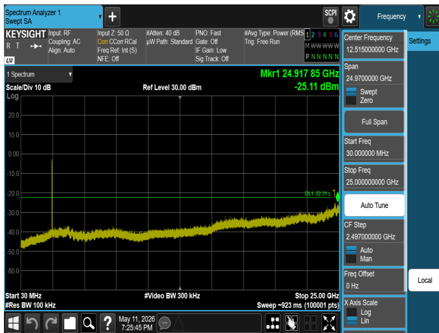
Plot 7-41. Conducted Spurious Plot (802.11g – Ch. 11)
