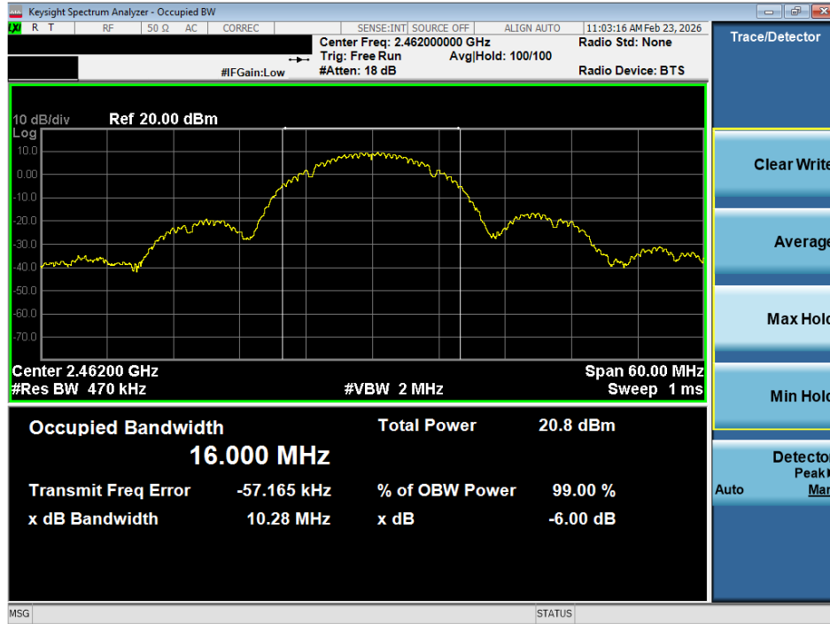
Plot 7-1 99% OBW (20MHz BW 802.11b - Ch.11)
