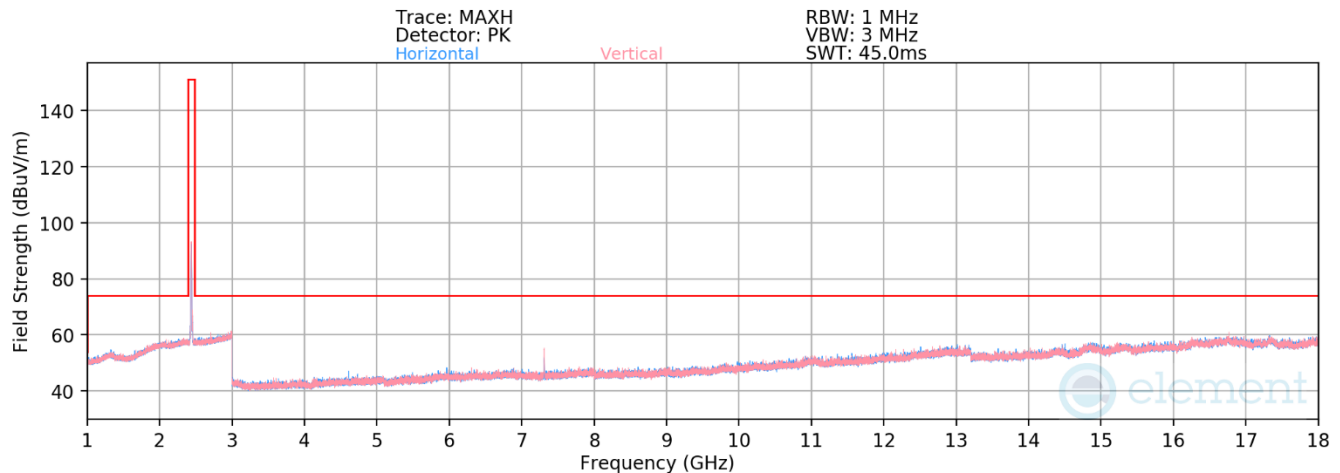
Plot 7-46. Radiated Spurious Emissions above 1GHz (802.11b – Ch. 6)
