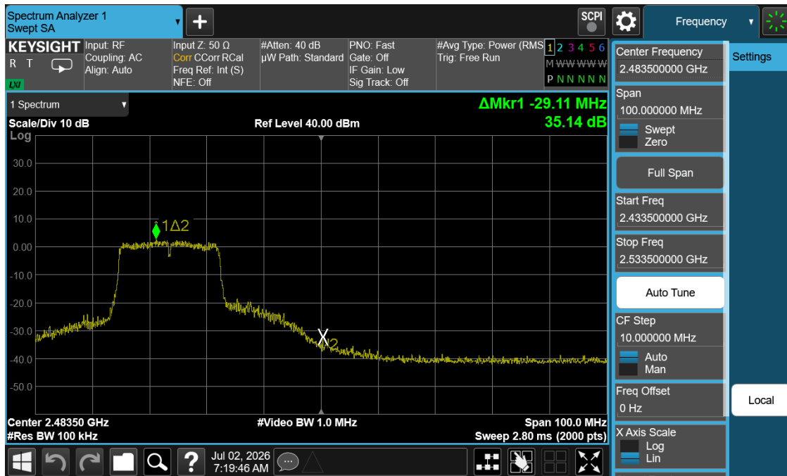
Plot 7-32. Band Edge Plot (802.11n (2.4GHz) – Ch. 10)
