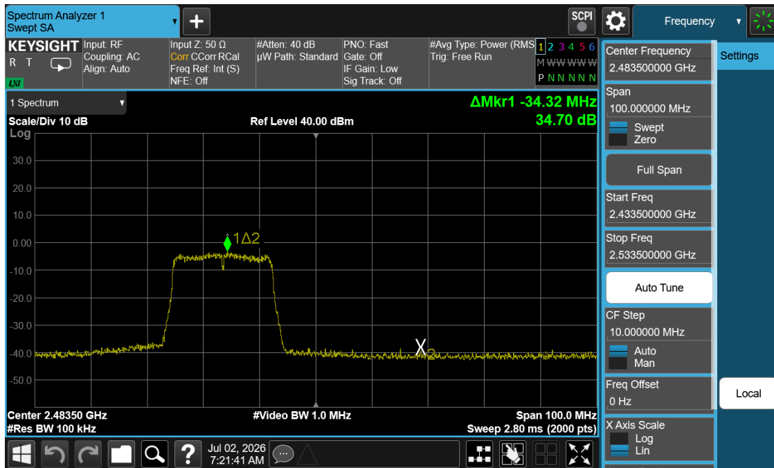
Plot 7-34. Band Edge Plot (802.11n (2.4GHz) – Ch. 12)
