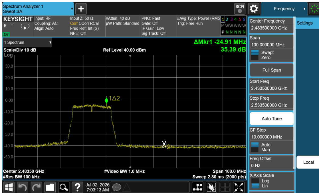
Plot 7-26. Band Edge Plot (802.11g – Ch. 12)
