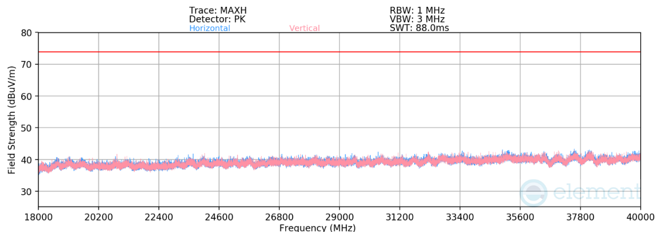
Plot 7-48. Radiated Spurious Emissions above 18GHz (802.11b – Ch.11)
