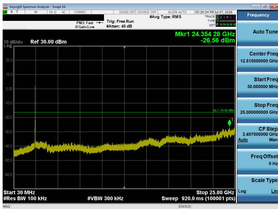
Plot 7-43. Conducted Spurious Plot (802.11n – Ch. 6)
