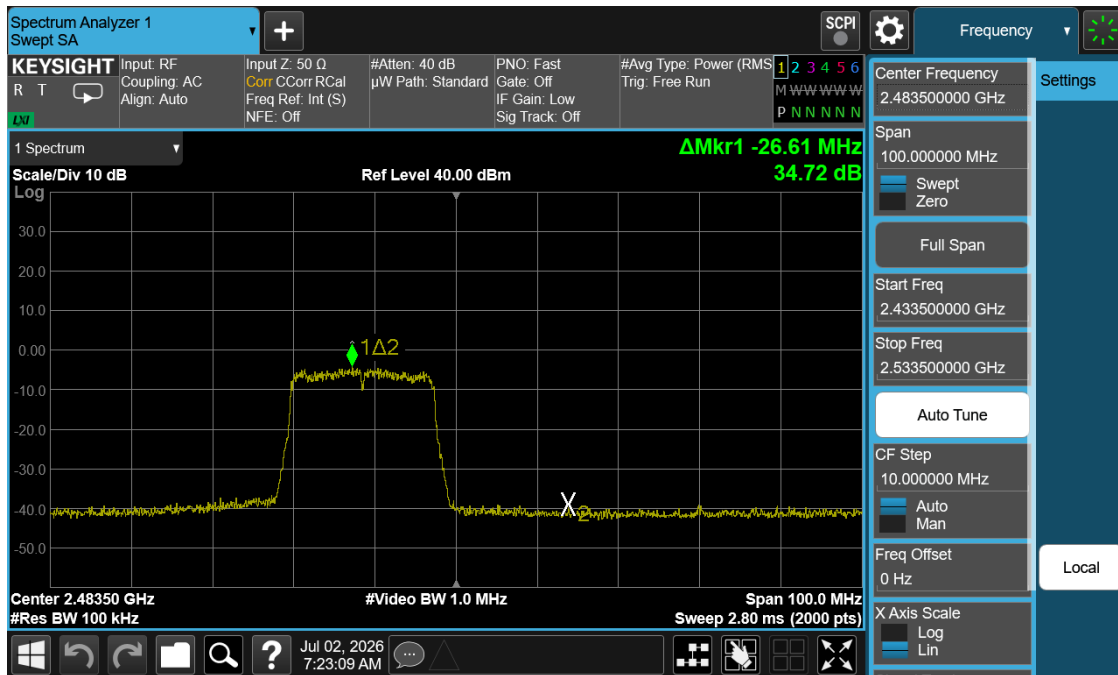
Plot 7-35. Band Edge Plot (802.11n (2.4GHz) – Ch. 13)
