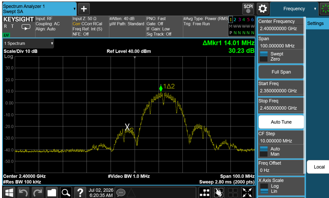
Plot 7-10. Band Edge Plot (802.11b – Ch. 1)
