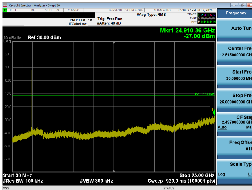
Plot 7-36. Conducted Spurious Plot (802.11b – Ch. 1)
