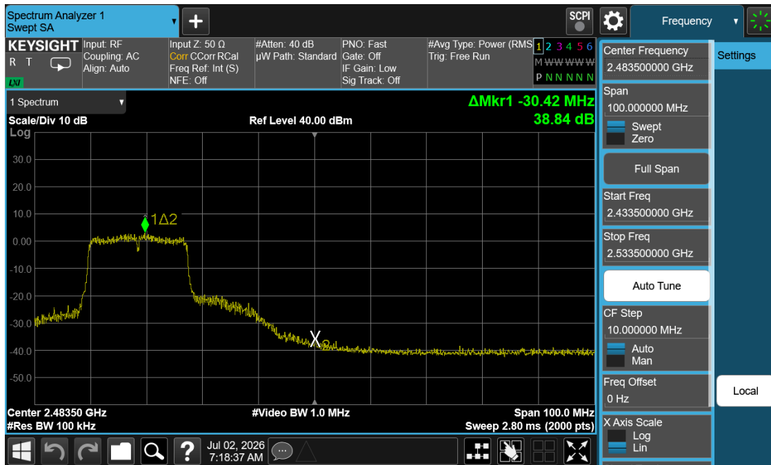
Plot 7-31. Band Edge Plot (802.11n (2.4GHz) – Ch. 9)
