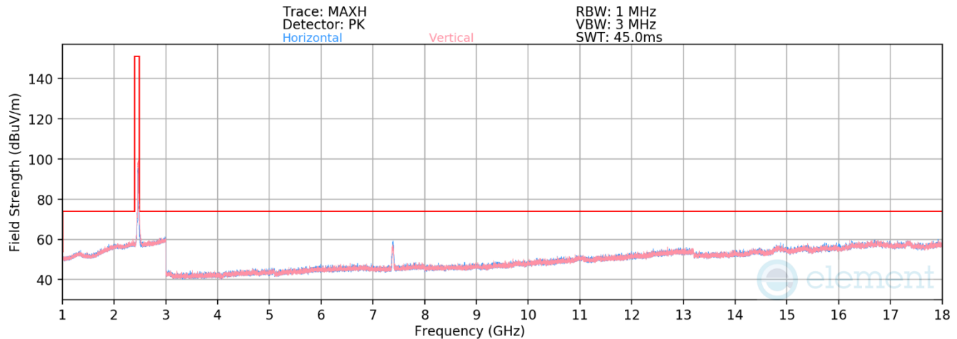
Plot 7-51. Radiated Spurious Emissions above 1GHz (802.11g – Ch. 11)
