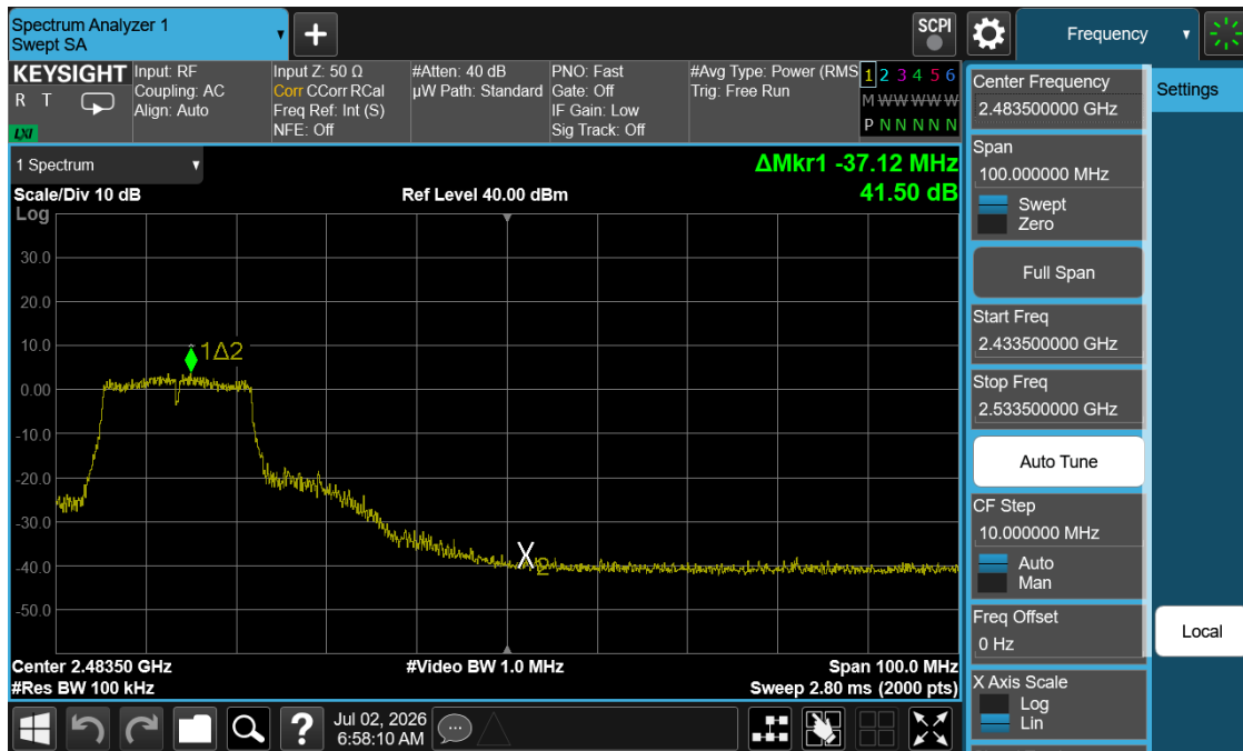
Plot 7-22. Band Edge Plot (802.11g – Ch. 8)
