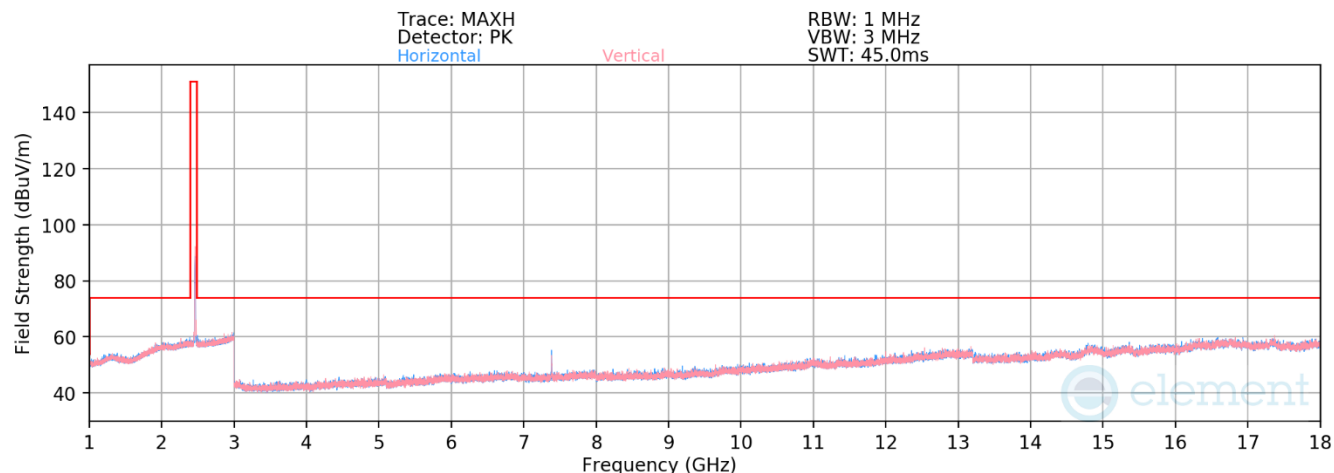
Plot 7-47. Radiated Spurious Emissions above 1GHz (802.11b – Ch. 11)
