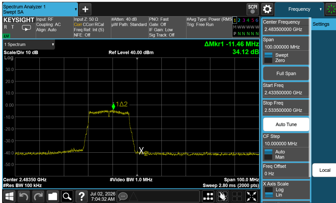
Plot 7-27. Band Edge Plot (802.11g – Ch. 13)
