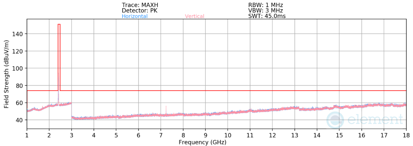
Plot 7-45. Radiated Spurious Emissions above 1GHz (802.11b – Ch. 1)
