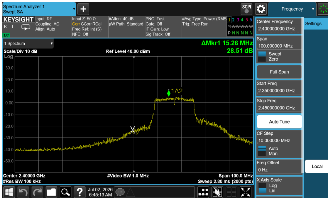
Plot 7-19. Band Edge Plot (802.11g – Ch. 2)
