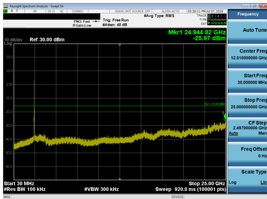
Plot 7-40. Conducted Spurious Plot (802.11g – Ch. 6)
