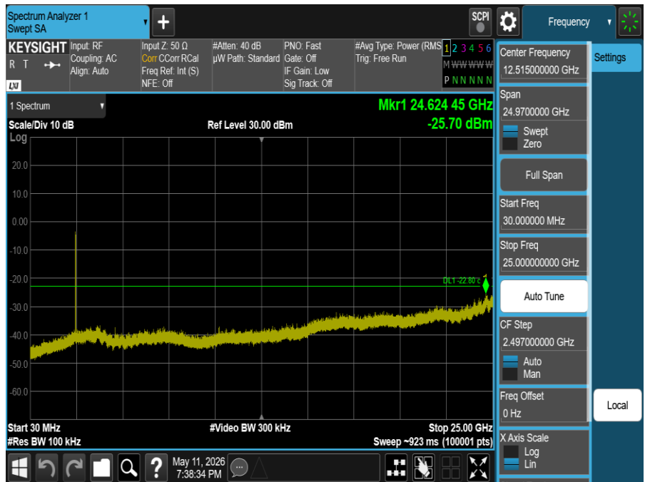
Plot 7-44. Conducted Spurious Plot (802.11n – Ch. 11)
