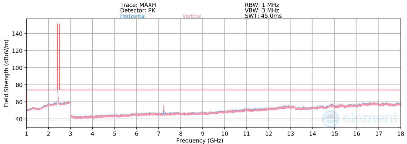
Plot 7-49. Radiated Spurious Emissions above 1GHz (802.11g – Ch. 1)
