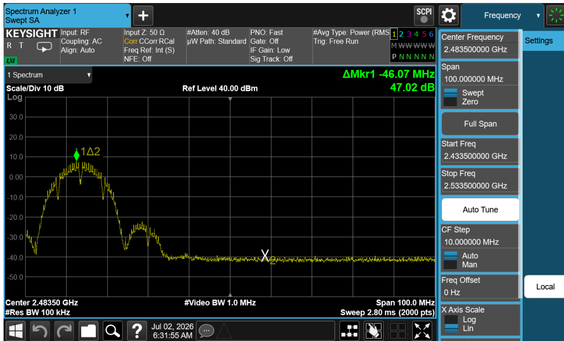
Plot 7-12. Band Edge Plot (802.11b – Ch. 8)
