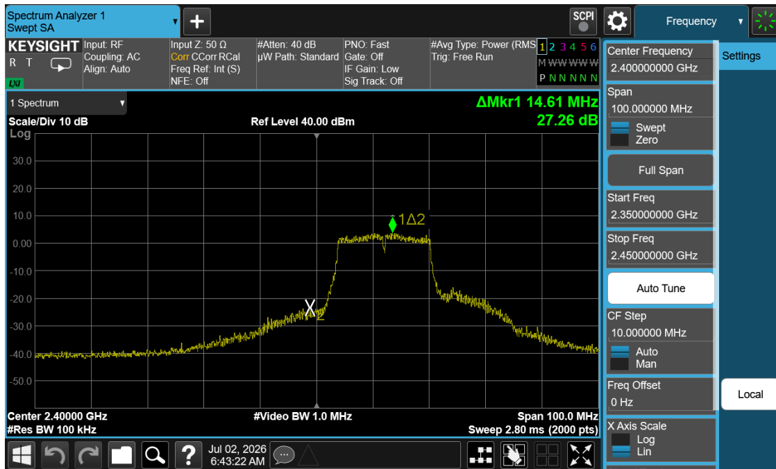
Plot 7-18. Band Edge Plot (802.11g – Ch. 1)
