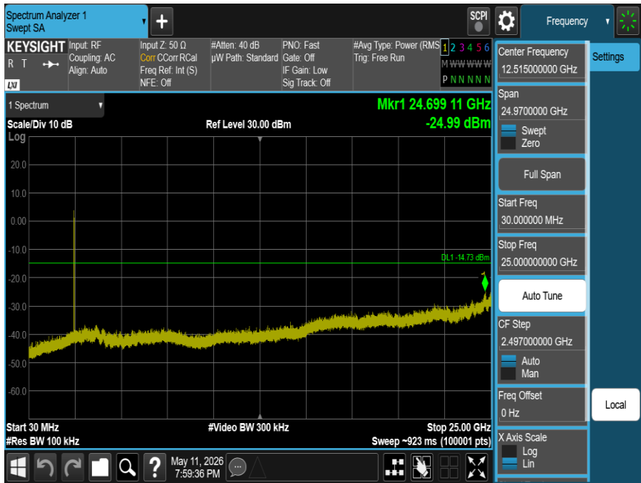
Plot 7-38. Conducted Spurious Plot (802.11b – Ch. 11)
