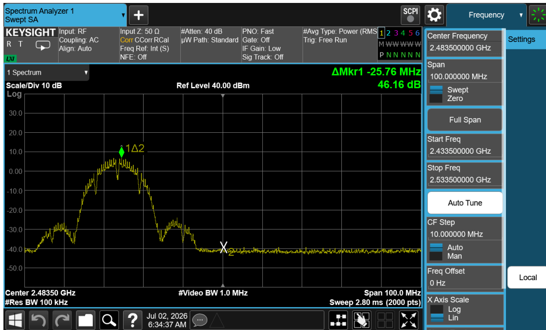
Plot 7-14. Band Edge Plot (802.11b – Ch. 10)
