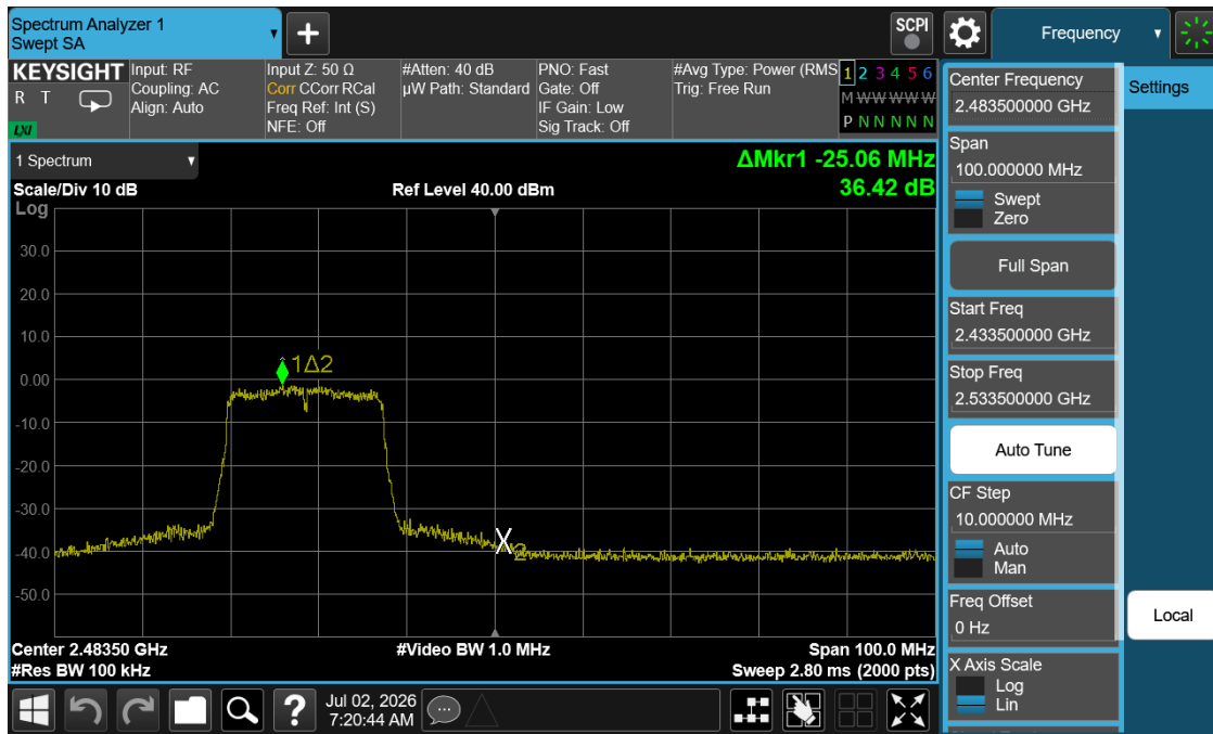
Plot 7-33. Band Edge Plot (802.11n (2.4GHz) – Ch. 11)
