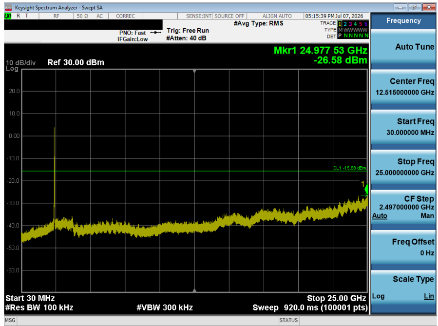
Plot 7-39. Conducted Spurious Plot (802.11g – Ch. 1)
