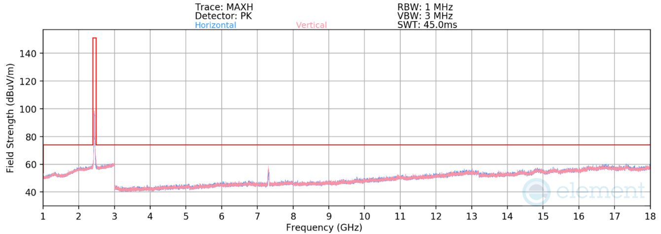
Plot 7-50. Radiated Spurious Emissions above 1GHz (802.11g – Ch. 6)
