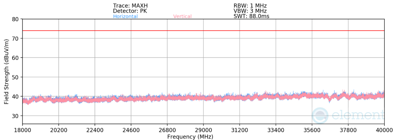
Plot 7-52. Radiated Spurious Emissions above 18GHz (802.11g – Ch.11)
