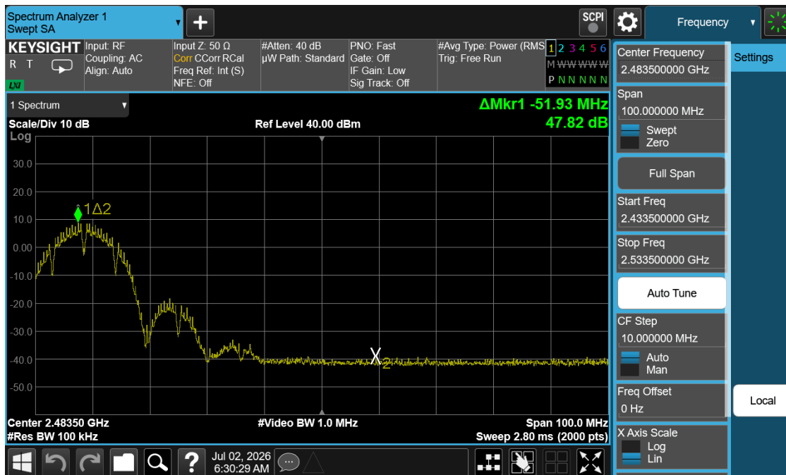
Plot 7-11. Band Edge Plot (802.11b – Ch. 7)
