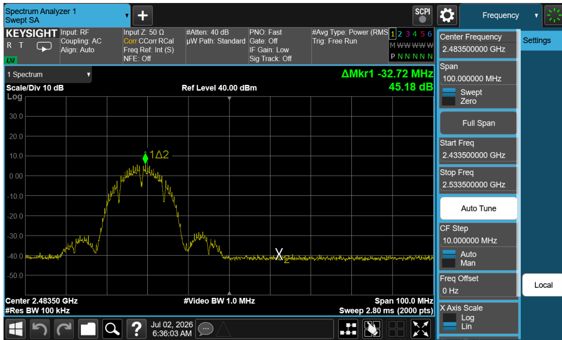
Plot 7-15. Band Edge Plot (802.11b – Ch. 11)
