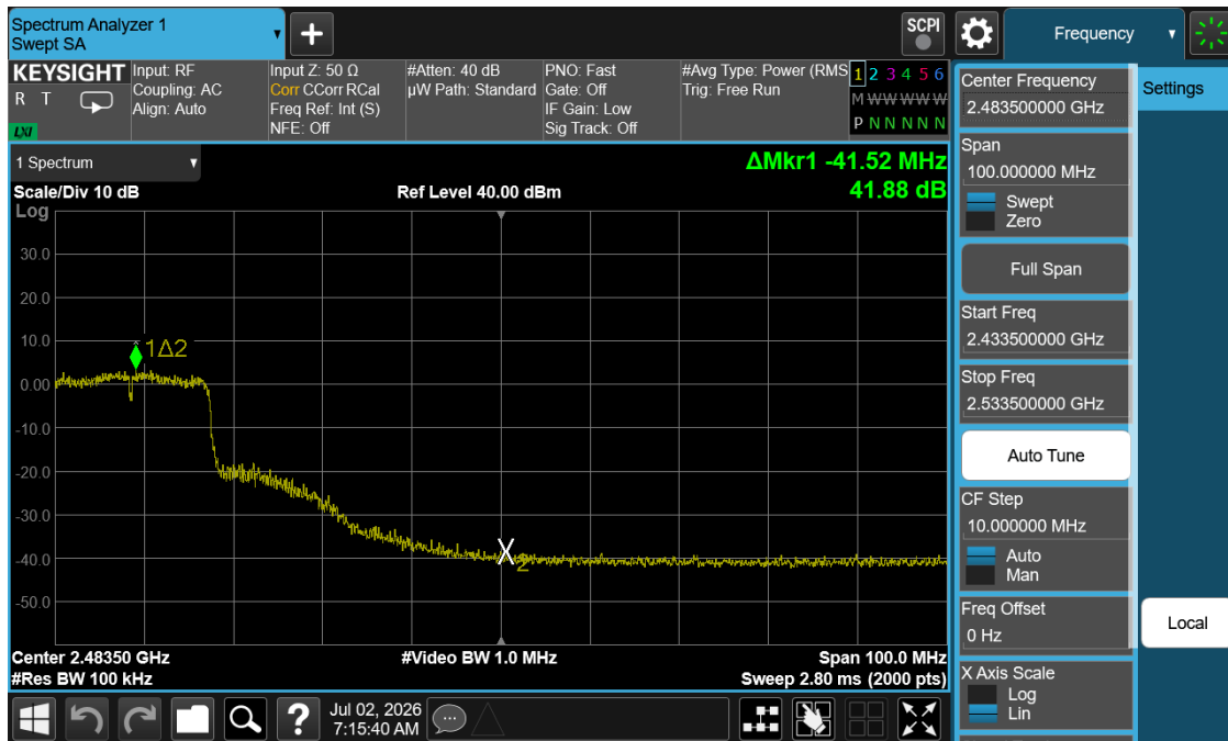
Plot 7-29. Band Edge Plot (802.11n (2.4GHz) – Ch. 7)
