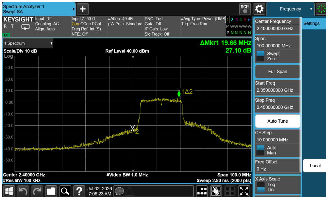
Plot 7-28. Band Edge Plot (802.11n (2.4GHz) – Ch. 1)
