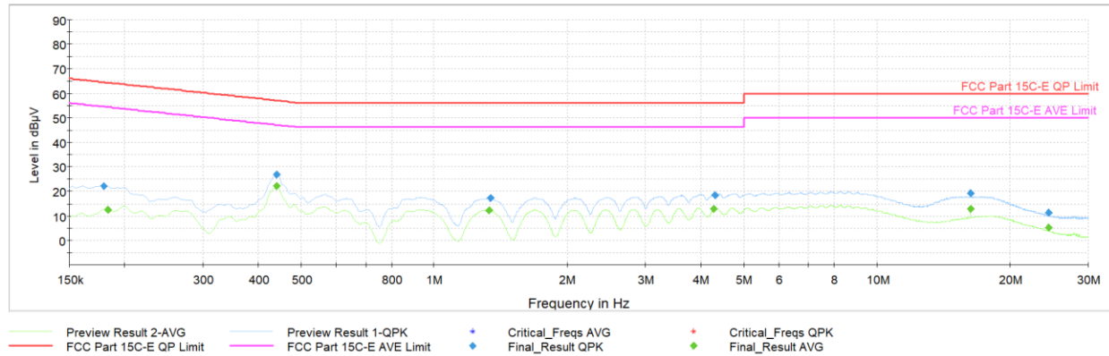
Plot 7-33. AC Line Conducted Plot with Bluetooth ANT+ (L1, ANT+ - Ch.79 with AC/DC Adapter)
