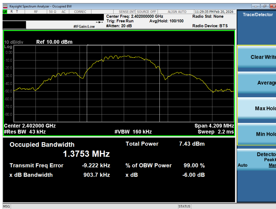
Plot 7-1. 99% OBW Plot (ANT+ – Ch. 1)
