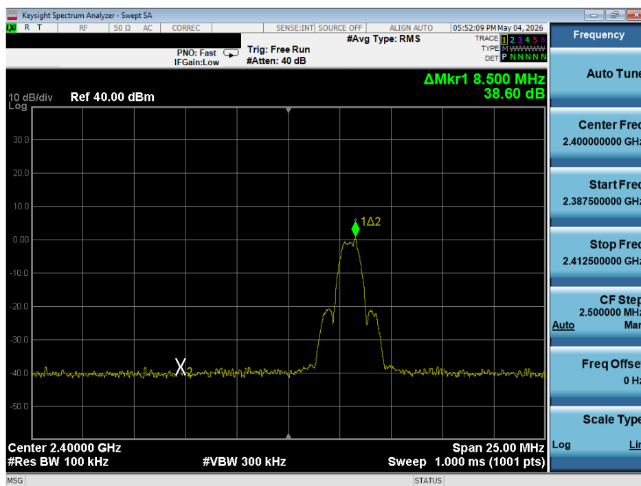
Plot 7-16. Band Edge Plot (ANT+ – Ch. 2)
