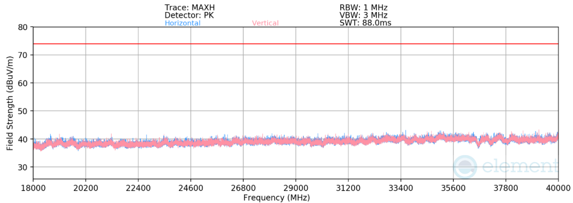
Plot 7-27. Radiated Spurious Emissions Above 18GHz (ANT+ – Ch. 79)
