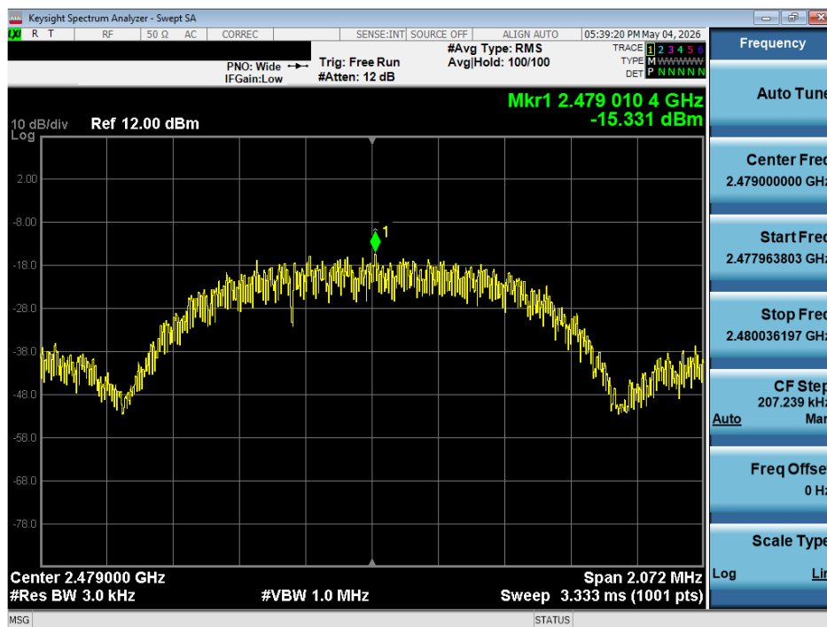
Plot 7-13. Power Spectral Density Plot (ANT+ – Ch. 78)
