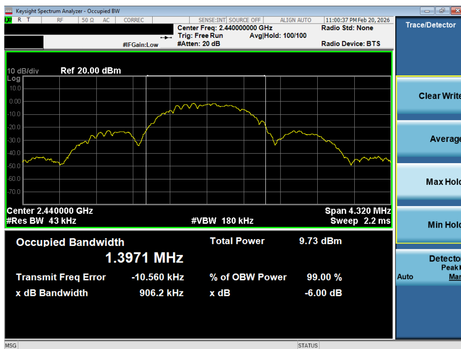
Plot 7-2. 99% OBW Plot (ANT+ – Ch. 39)
