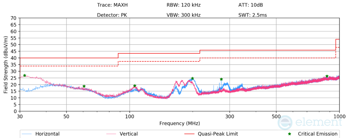
Plot 7-32. Radiated Spurious Emissions Below 1GHz (ANT+ – Ch.79 with AC/DC Adapter)
