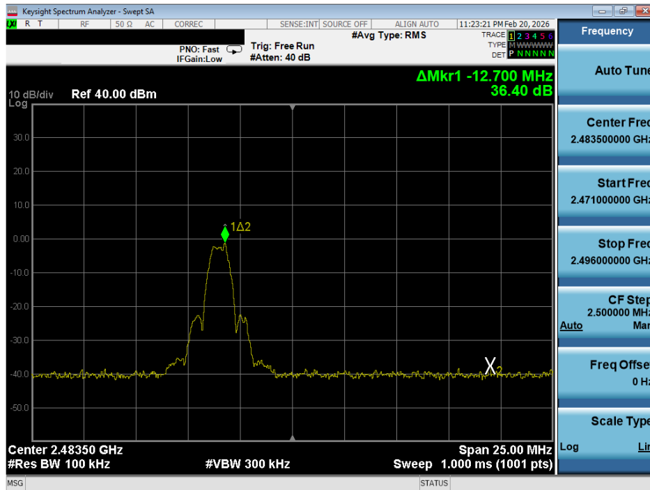
Plot 7-20. Band Edge Plot (ANT+ – Ch. 79)
