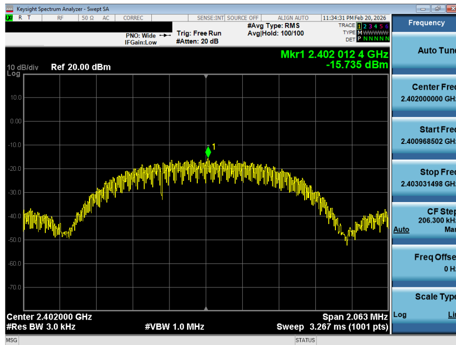
Plot 7-8. Power Spectral Density Plot (ANT+ – Ch. 1)
