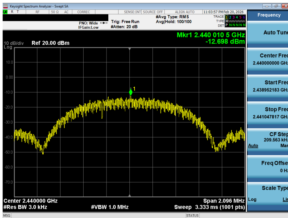
Plot 7-11. Power Spectral Density Plot (ANT+ – Ch. 39)
