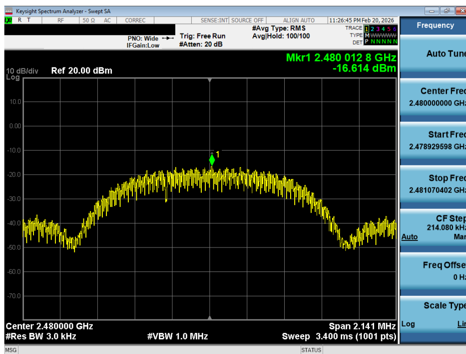
Plot 7-14. Power Spectral Density Plot (ANT+ – Ch. 79)
