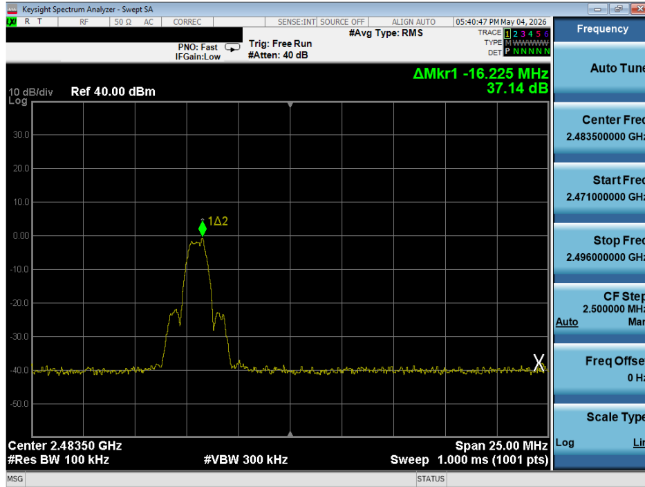
Plot 7-19. Band Edge Plot (ANT+ – Ch. 78)
