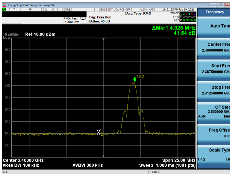
Plot 7-17. Band Edge Plot (ANT+ – Ch. 3)
