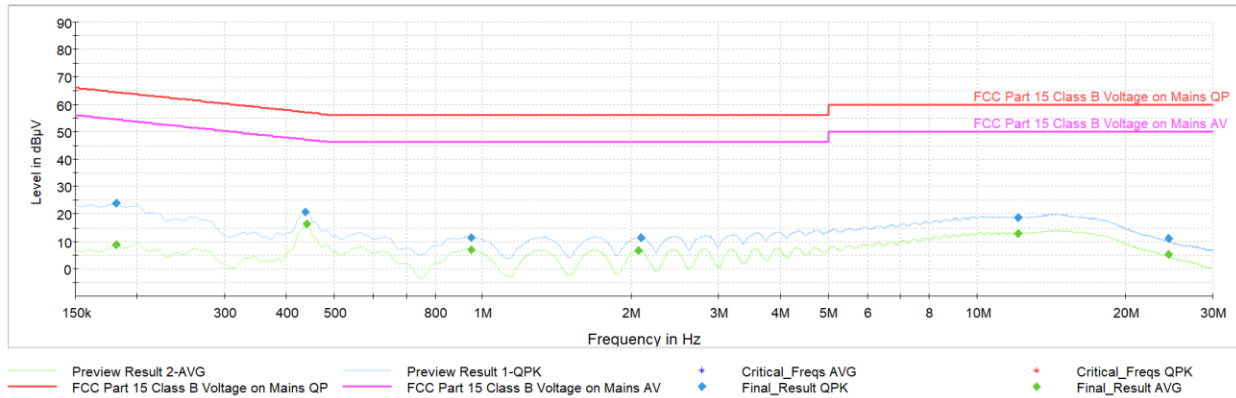
Plot 7-34. AC Line Conducted Plot with Bluetooth ANT+ (N, ANT+ - Ch.79 with AC/DC Adapter)
