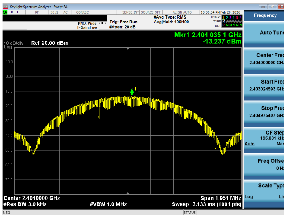
Plot 7-10. Power Spectral Density Plot (ANT+ – Ch. 3)
