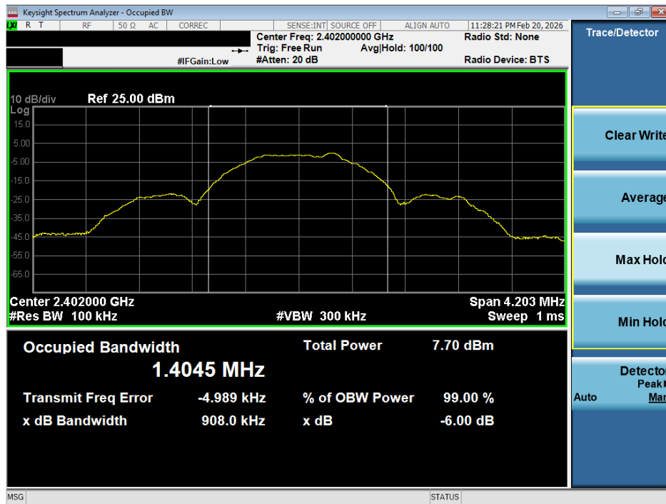
Plot 7-4. 6dB BW Plot (ANT+ – Ch. 1)
