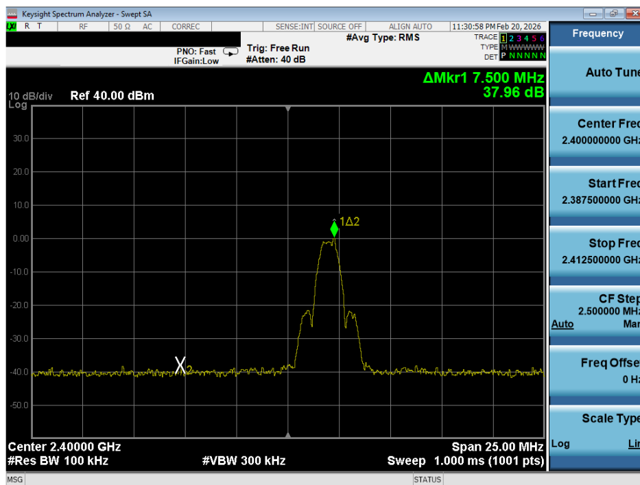
Plot 7-15. Band Edge Plot (ANT+ – Ch. 1)
