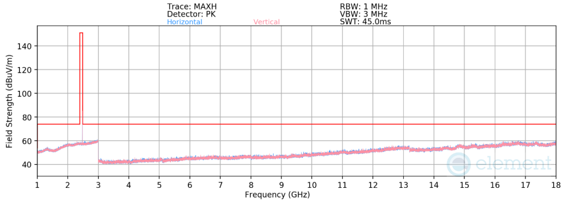
Plot 7-26. Radiated Spurious Emissions 1-18GHz (ANT+ – Ch. 79)
