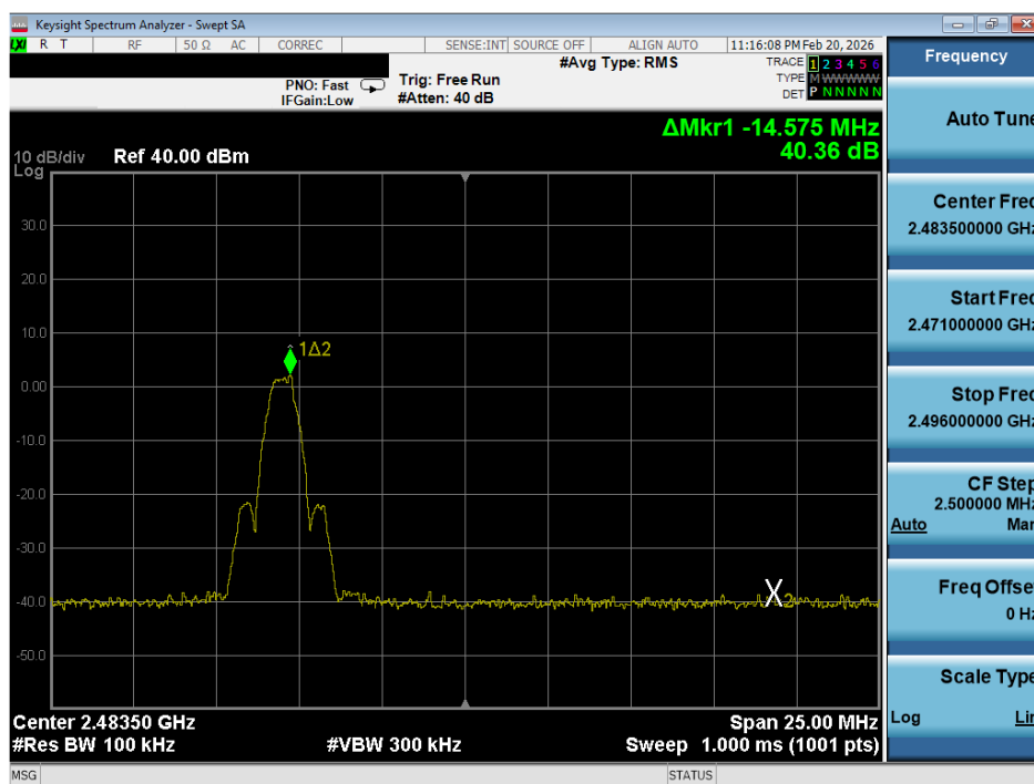
Plot 7-18. Band Edge Plot (ANT+ – Ch. 77)
