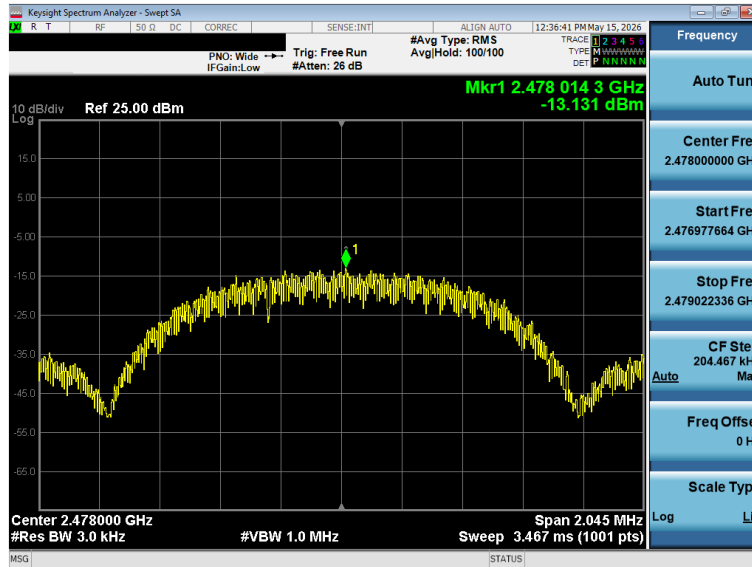
Plot 9-3. Power Spectral Density Plot (Spot-check)
