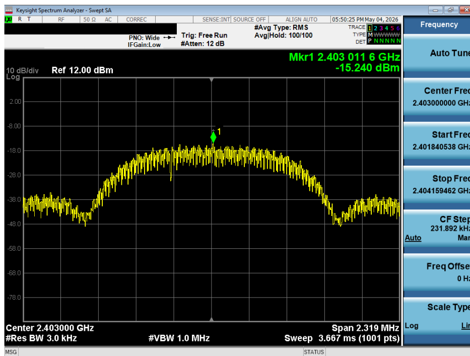
Plot 7-9. Power Spectral Density Plot (ANT+ – Ch. 2)
