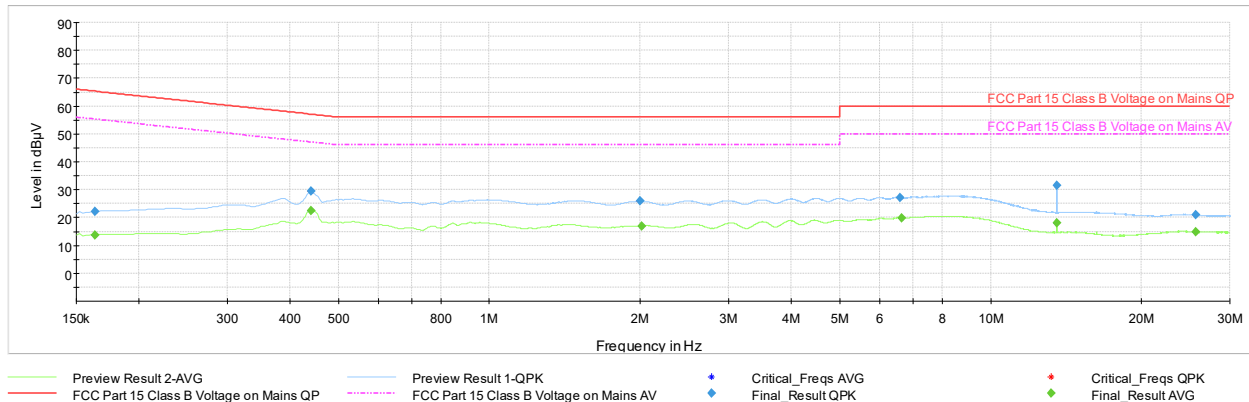
Plot 7-6. AC Line-Conducted Plot (N, with AC/DC Adapter)
