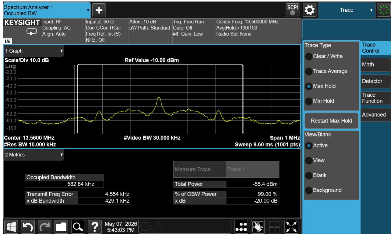
Plot 7-1. 99% Bandwidth Plot
