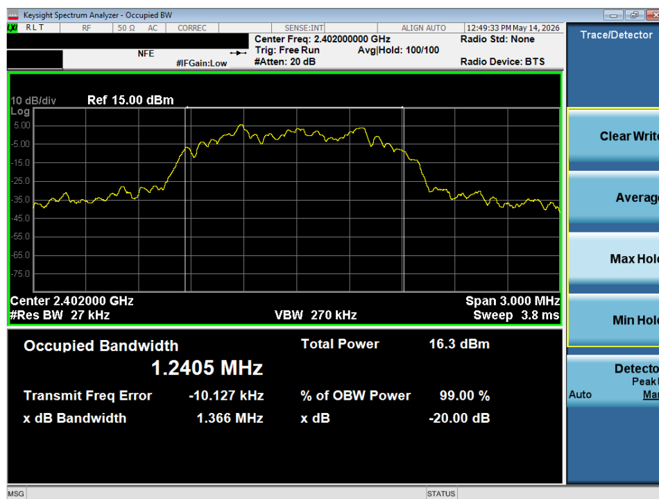
Plot 9-1. 20dB Bandwidth Plot (Spot-check)
