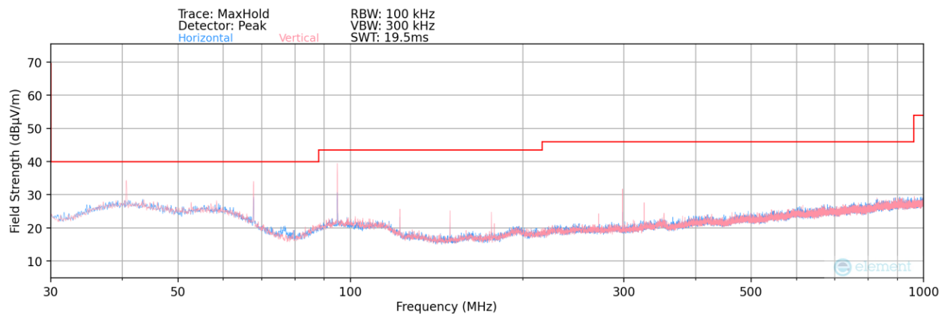
Plot 7-4. Radiated Spurious Plot 30MHz – 1GHz
