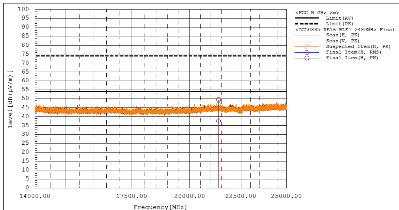
Figure RE16.1: Spectral data (BLE, 1 Mbps, 2480 MHz)
