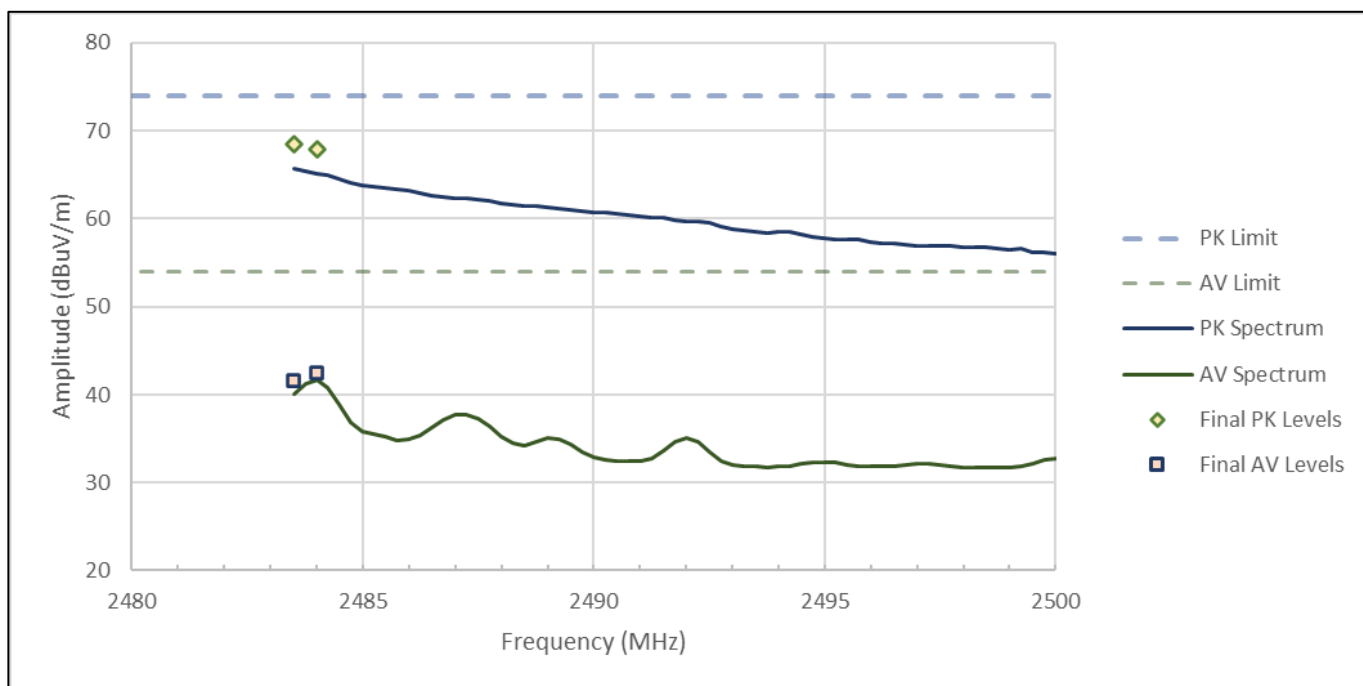
Figure RE03.3: FCC restricted band spectral data from 2483.5 to 2500 MHz (BLE, 1 Mbps, 2476 MHz)
