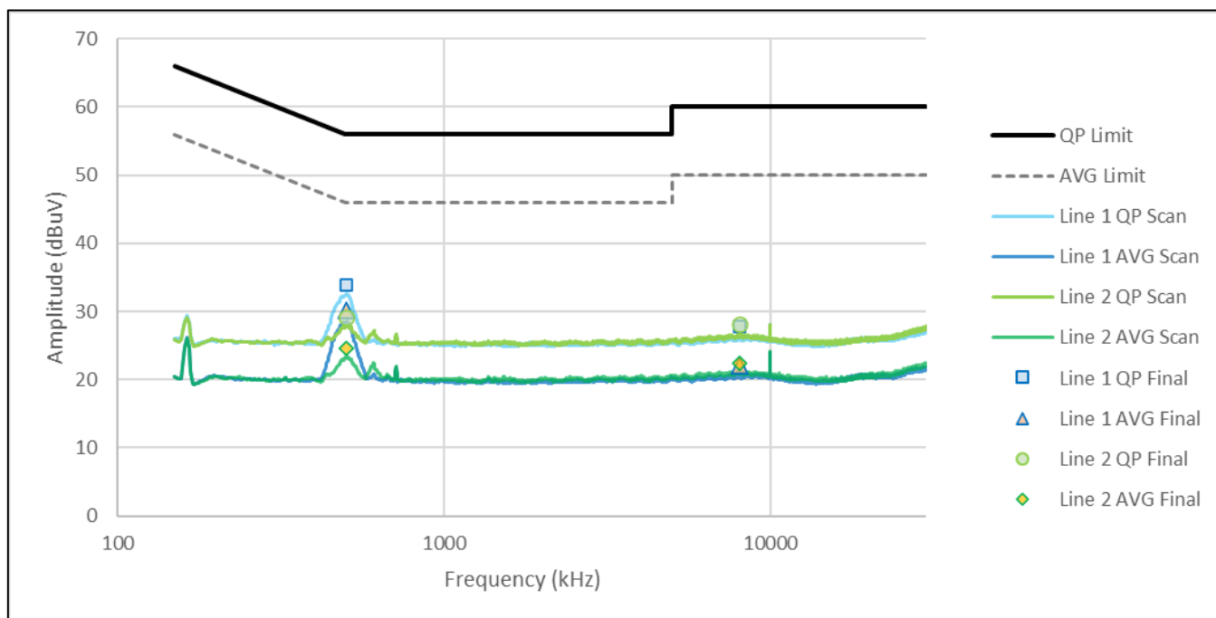
Figure CE03.1: Spectral data (ANT, 2440 MHz)
