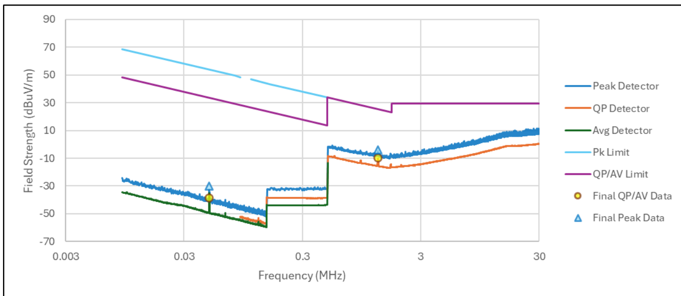
Figure RE22.1: Spectral data (BLE, 1 Mbps, 2480 MHz)
