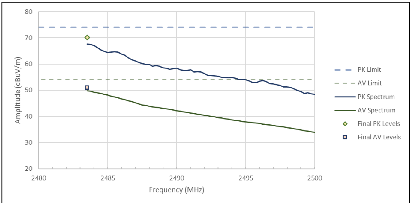
Figure RE01.6: FCC restricted band spectral data from 2483.5 to 2500 MHz (IEEE 802.11n, 1 Mbps, Ch11)
