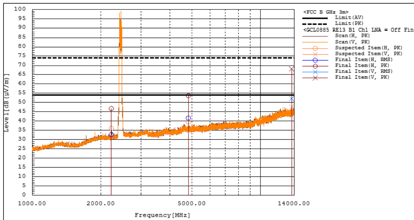
Figure RE13.1: Spectral data (IEEE 802.11b, 1 Mbps, Ch 1)
