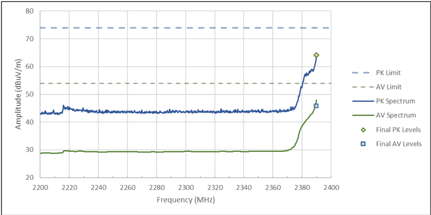
Figure RE01.2: FCC restricted band spectral data from 2200 to 2390 MHz (IEEE 802.11g, 18 Mbps, Ch1)
