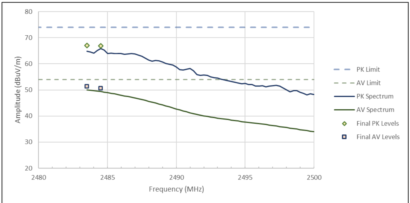
Figure RE01.8: FCC restricted band spectral data from 2483.5 to 2500 MHz (IEEE 802.11g, 24 Mbps, Ch12)
