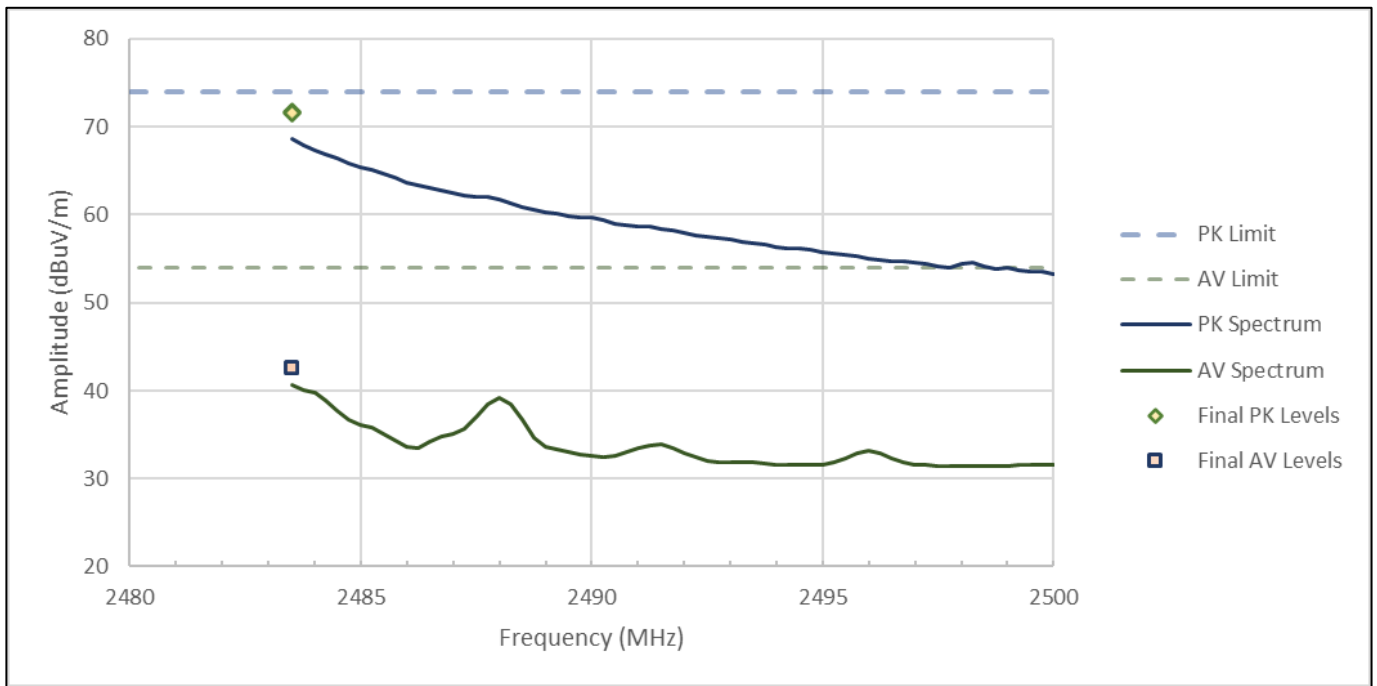
Figure RE03.4: FCC restricted band spectral data from 2483.5 to 2500 MHz (BLE, 1 Mbps, 2480 MHz)
