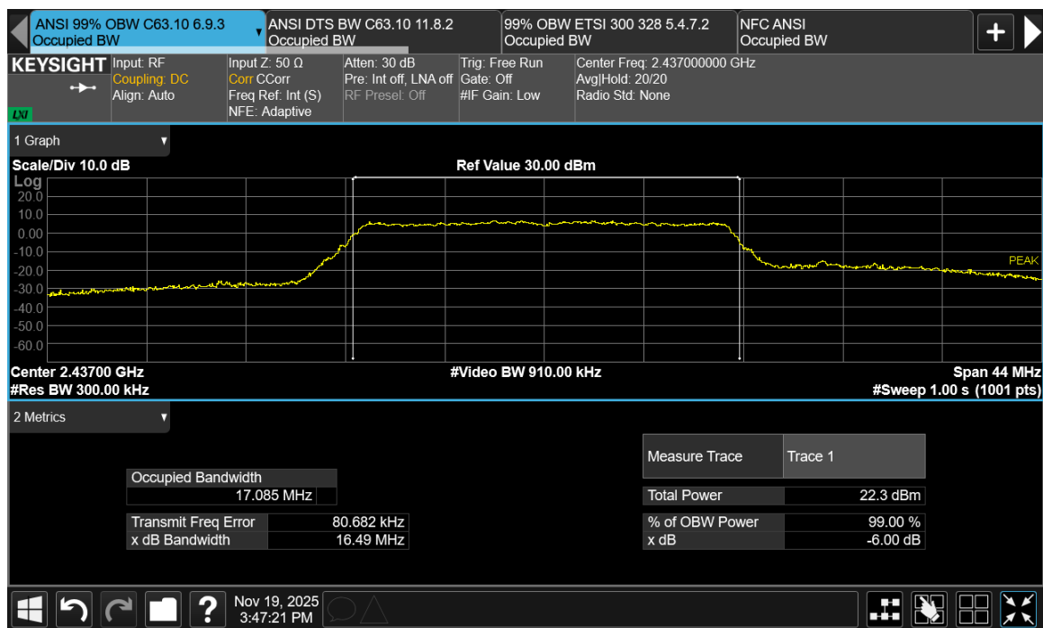
Figure TR15.5: Occupied bandwidth data for 802.11g 6 Mbps at channel 6
