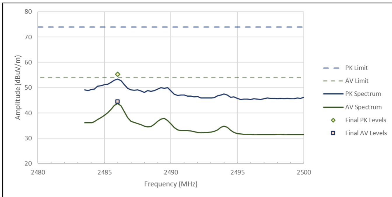
Figure RE04.3: FCC restricted band spectral data from 2483.5 to 2500 MHz (ANT, 2478 MHz)
