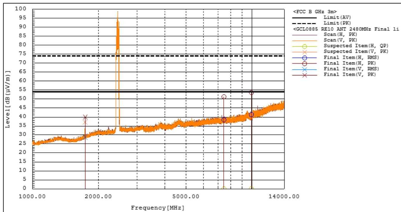
Figure RE10.3: Spectral data (ANT, 2480MHz)
