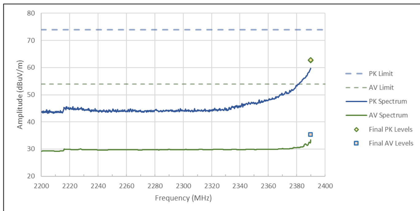
Figure RE03.1: FCC restricted band spectral data from 2200 to 2390 MHz (BLE, 1 Mbps, 2402 MHz)
