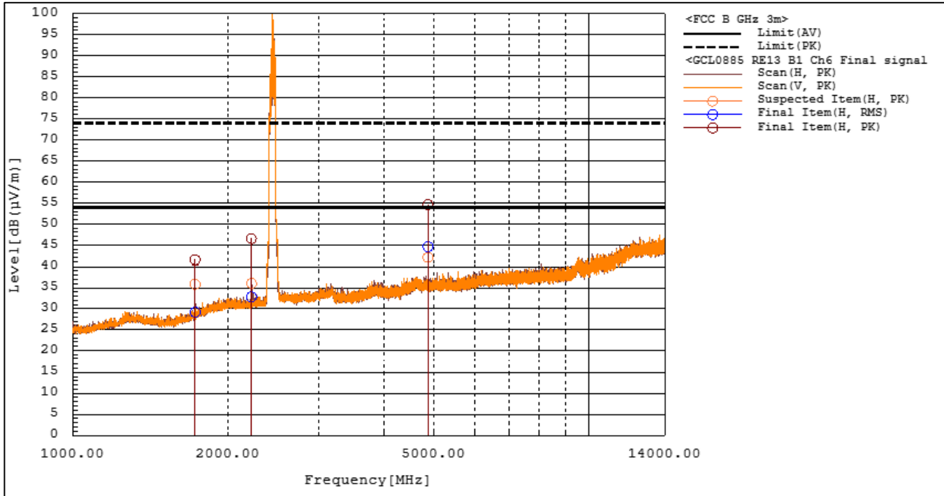
Figure RE13.2: Spectral data (IEEE 802.11b, 1 Mbps, Ch 6)
