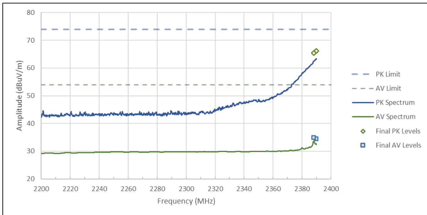
Figure RE03.2: FCC restricted band spectral data from 2200 to 2390 MHz (BLE, 1 Mbps, 2404 MHz)
