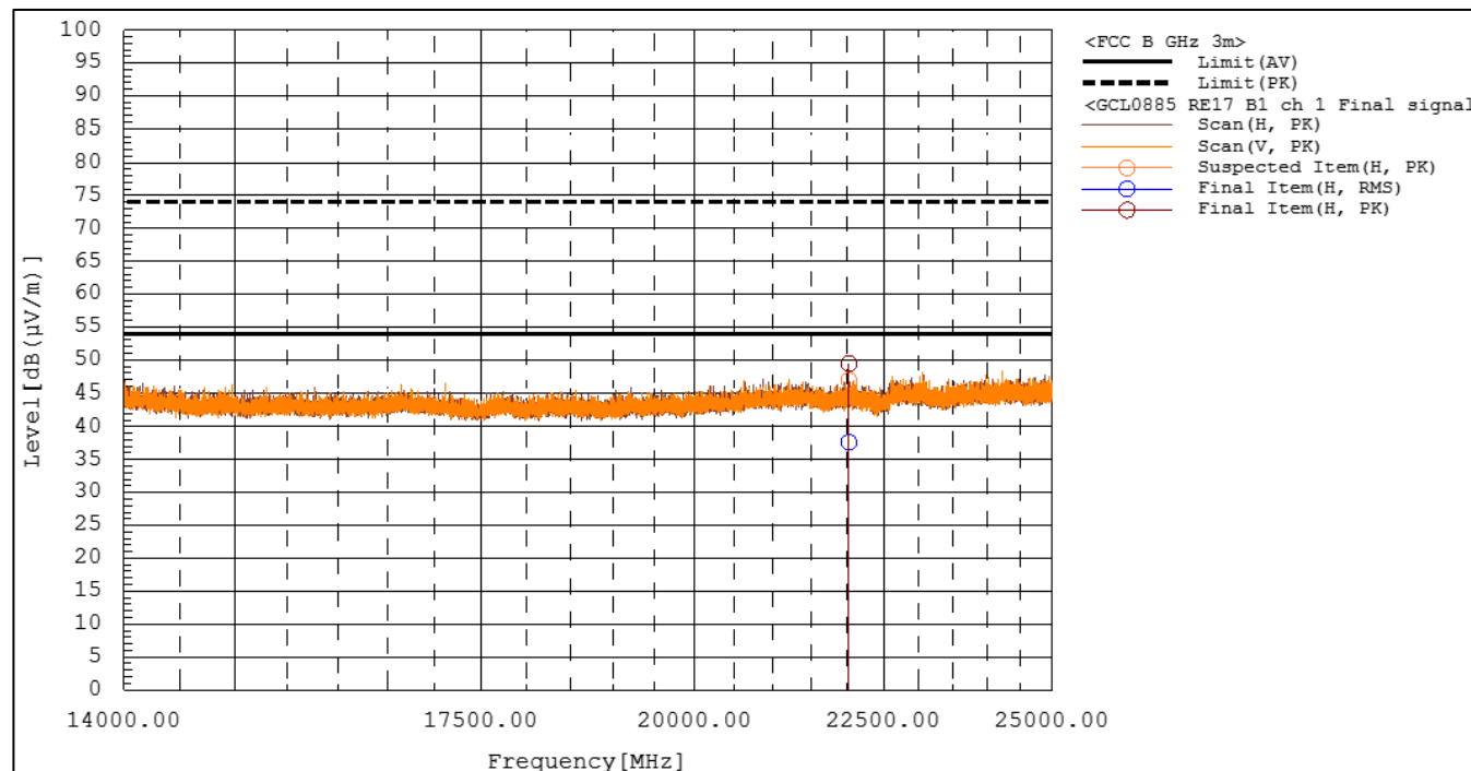
Figure RE17.1: Spectral data (IEEE 802.11b, 1 Mbps, Ch 1)
