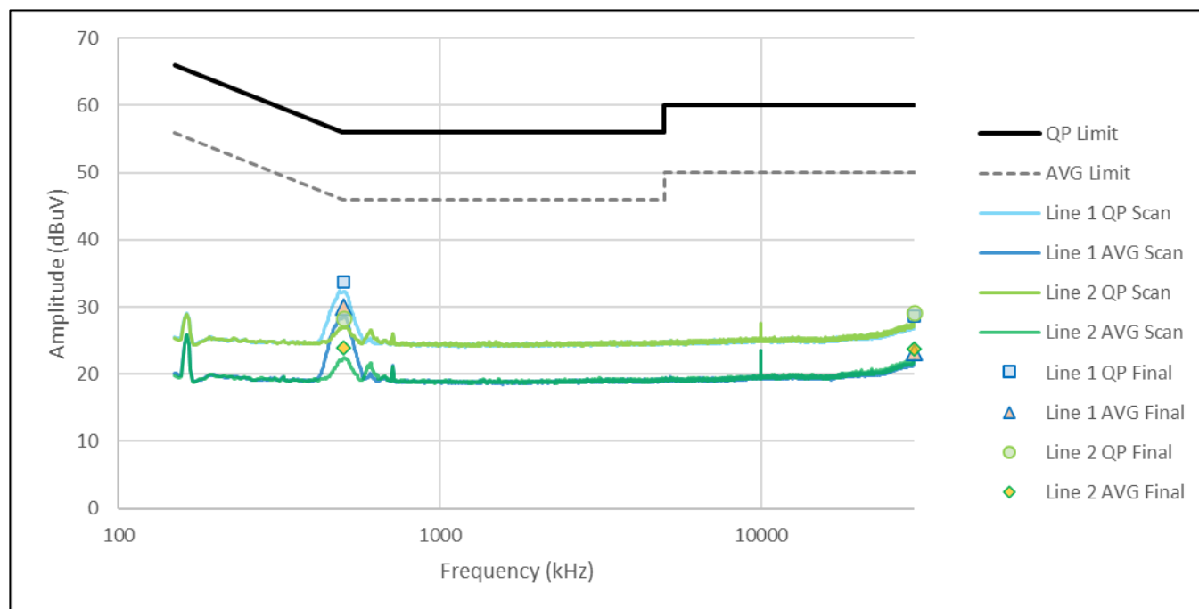
Figure CE04.1: Spectral data (IEEE 802.11b, 5.5 Mbps, Ch 6)
