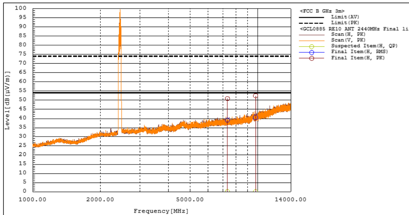
Figure RE10.2: Spectral data (ANT, 2440MHz)
