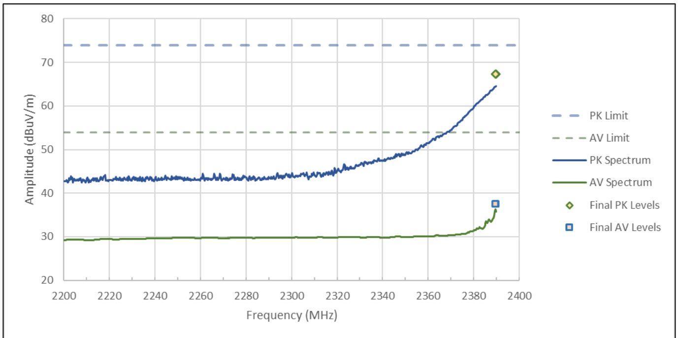
Figure RE03.5: FCC restricted band spectral data from 2200 to 2390 MHz (BLE, 2 Mbps, 2404 MHz)
