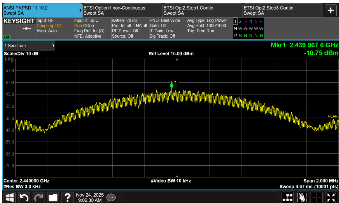
Figure TR30.3: Test data for ANT at 2440 MHz
