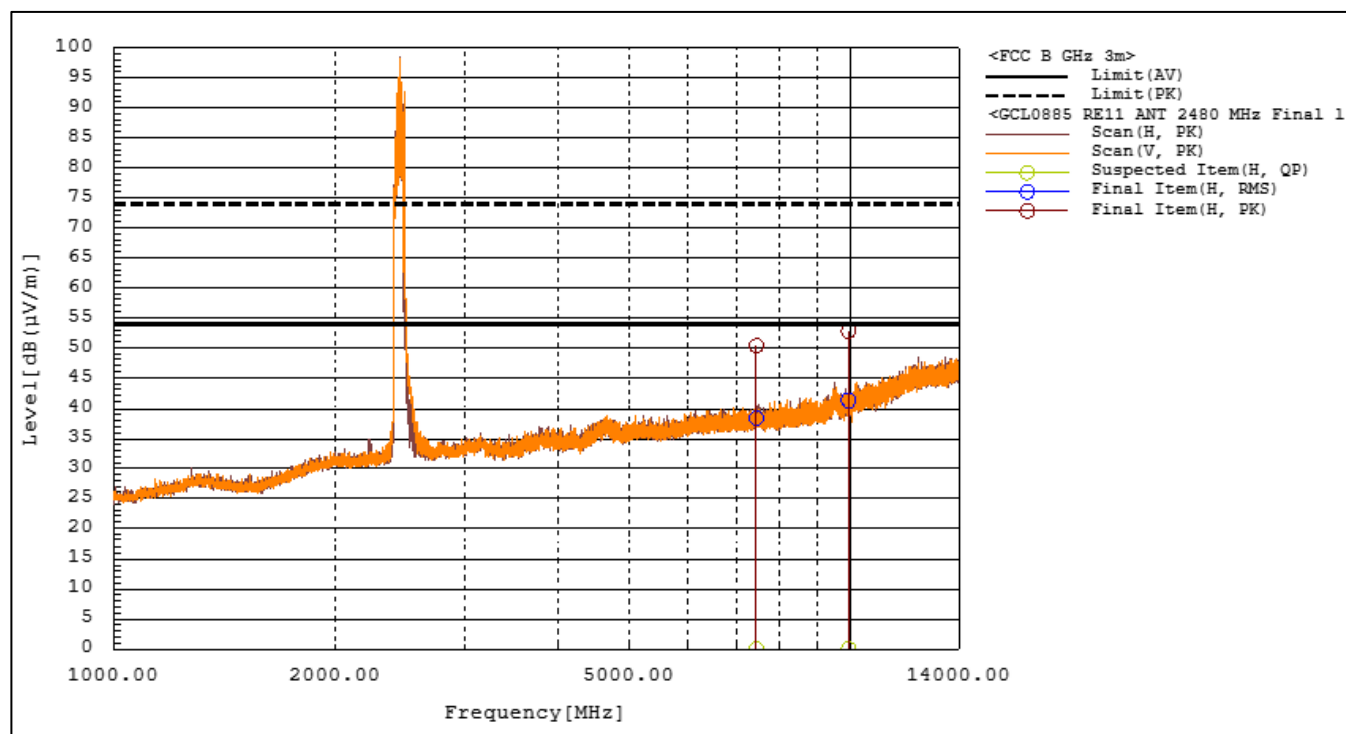
Figure RE11.3: Spectral data (2480 MHz)
