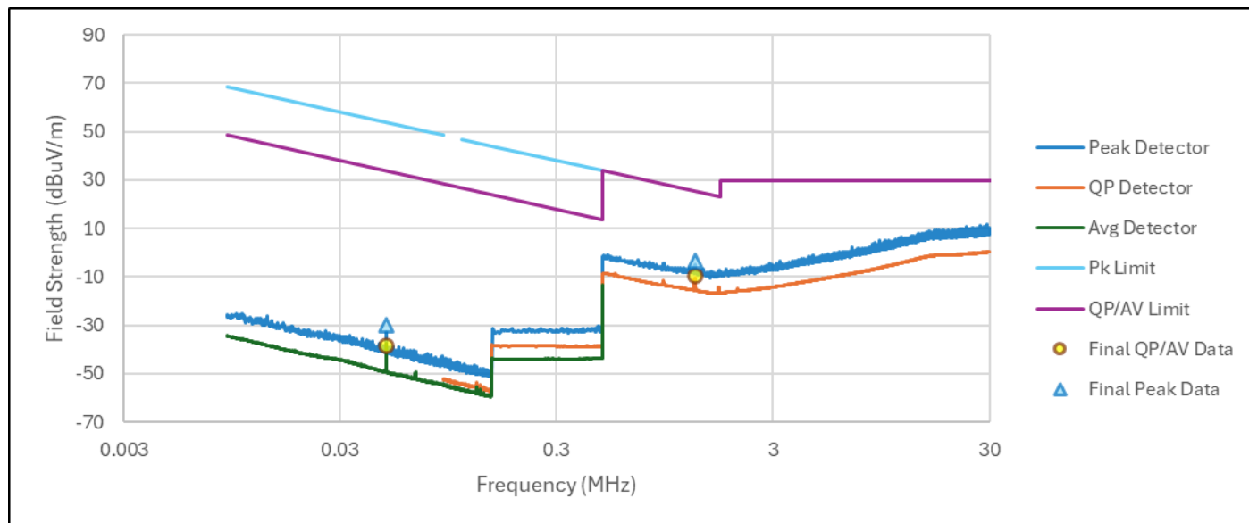
Figure RE21.1: Spectral data
