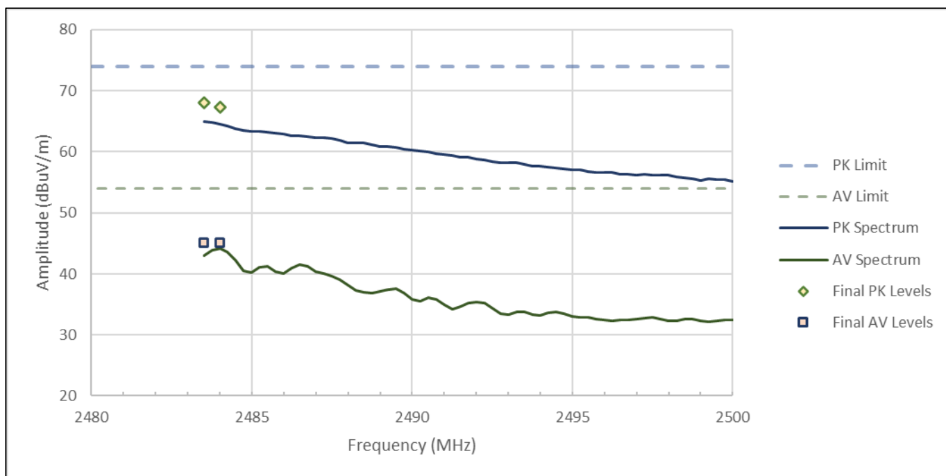
Figure RE03.6: FCC restricted band spectral data from 2483.5 to 2500 MHz (BLE, 2 Mbps, 2476 MHz)
