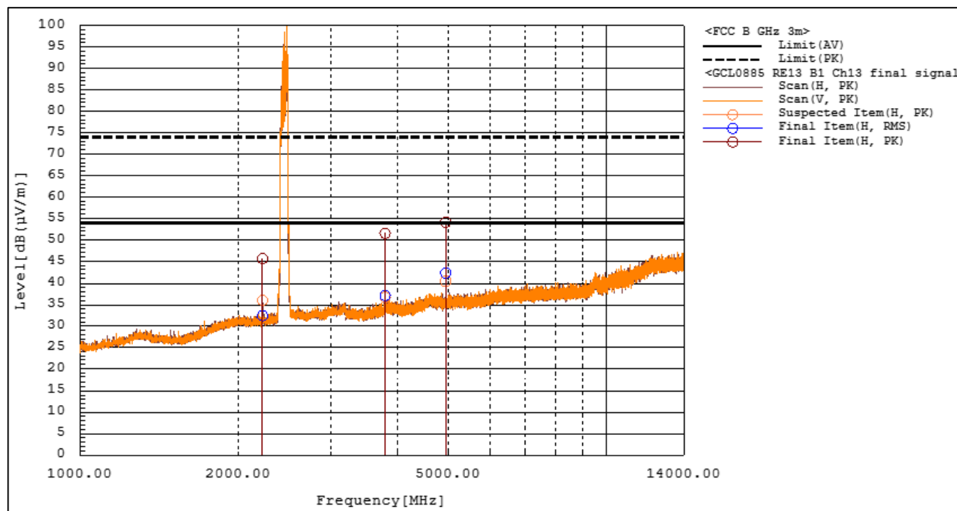
Figure RE13.4: Spectral data (IEEE 802.11b, 1 Mbps, Ch 13)
