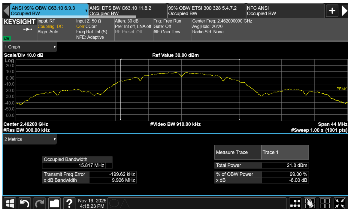
Figure TR15.4: Occupied bandwidth data for 802.11b 2 Mbps at channel 11
