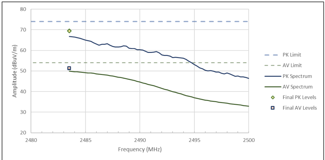
Figure RE01.10: FCC restricted band spectral data from 2483.5 to 2500 MHz (IEEE 802.11n, 4 Mbps, Ch13)
