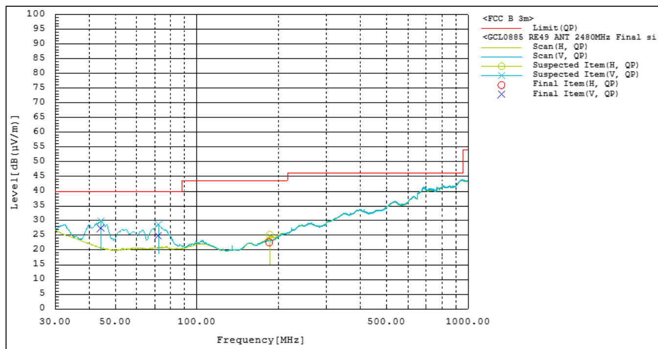
Figure RE49.1: Spectral data (ANT, 2480 MHz)
