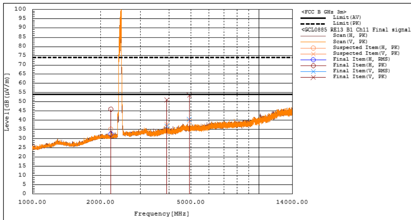
Figure RE13.3: Spectral data (IEEE 802.11b, 1 Mbps, Ch 11)
