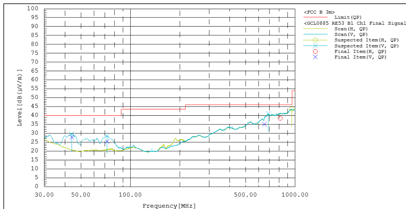
Figure RE53.1: Spectral data (IEEE 802.11b, 1 Mbps, Ch 1)
