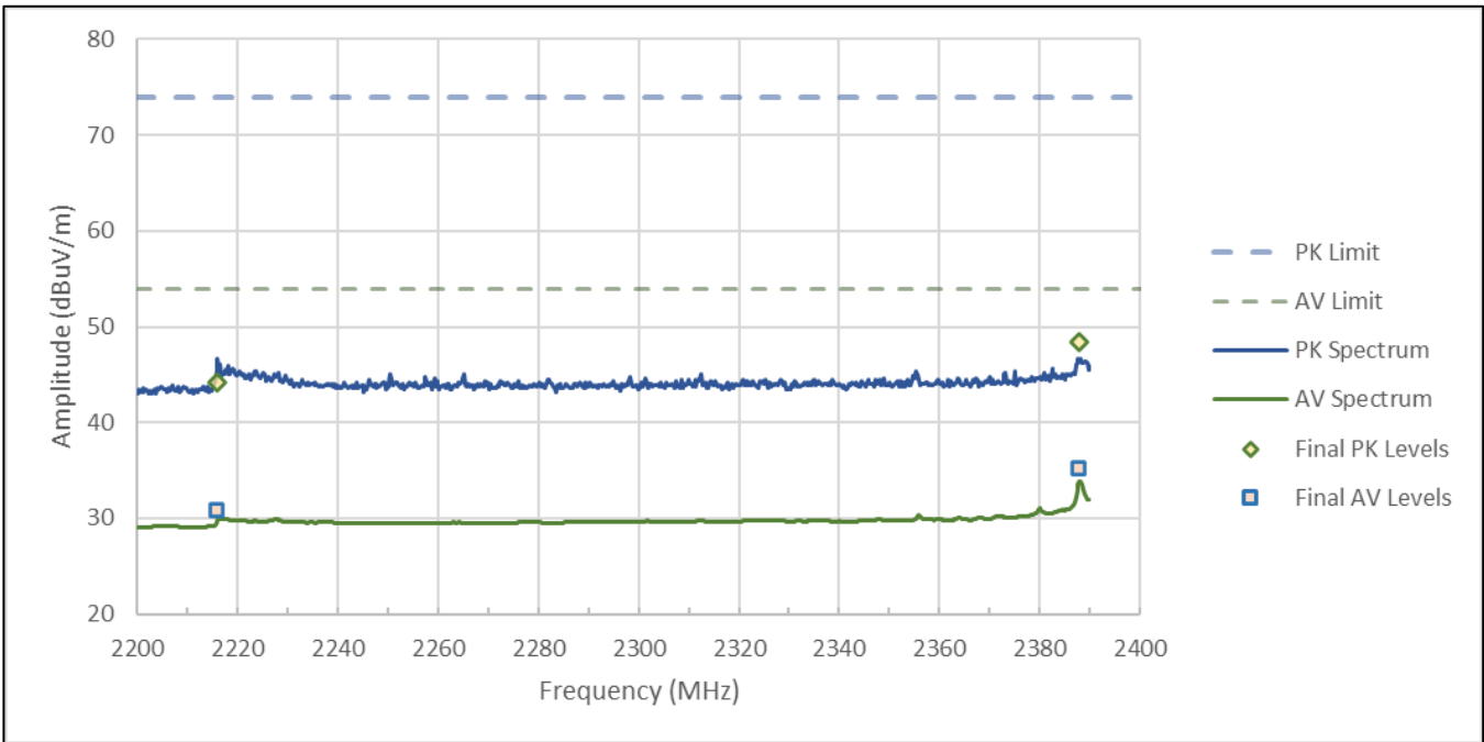
Figure RE04.2: FCC restricted band spectral data from 2200 to 2390 MHz (ANT, 2404 MHz)
