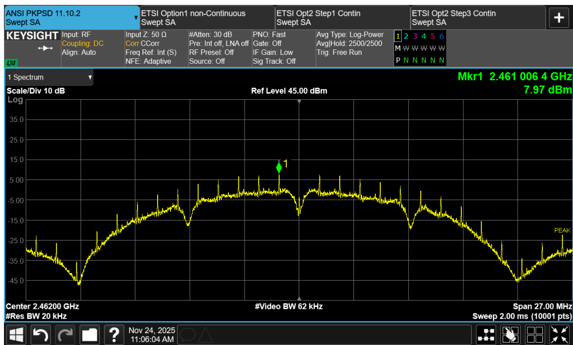
Figure TR30.4: Test data for IEEE 802.11b 1 Mbps at channel 11
