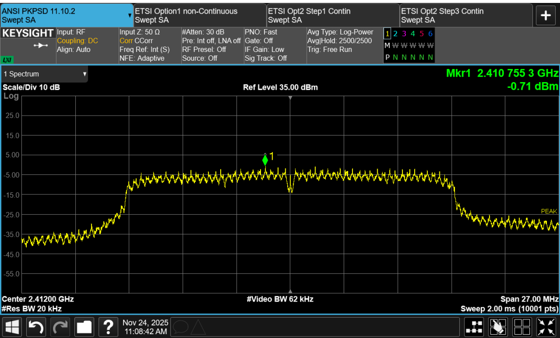
Figure TR30.5: Test data for IEEE 802.11g 9 Mbps at channel 1
