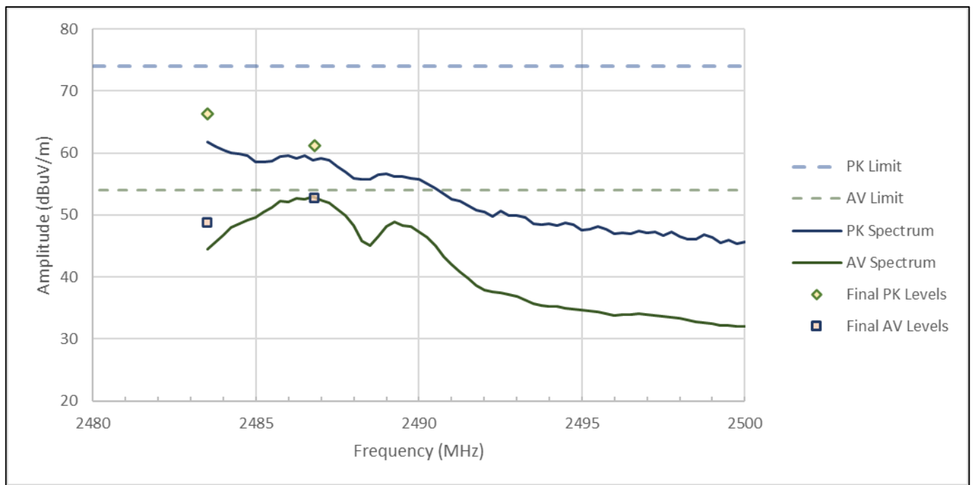
Figure RE01.9: FCC restricted band spectral data from 2483.5 to 2500 MHz (IEEE 802.11b, 1 Mbps, Ch13)
