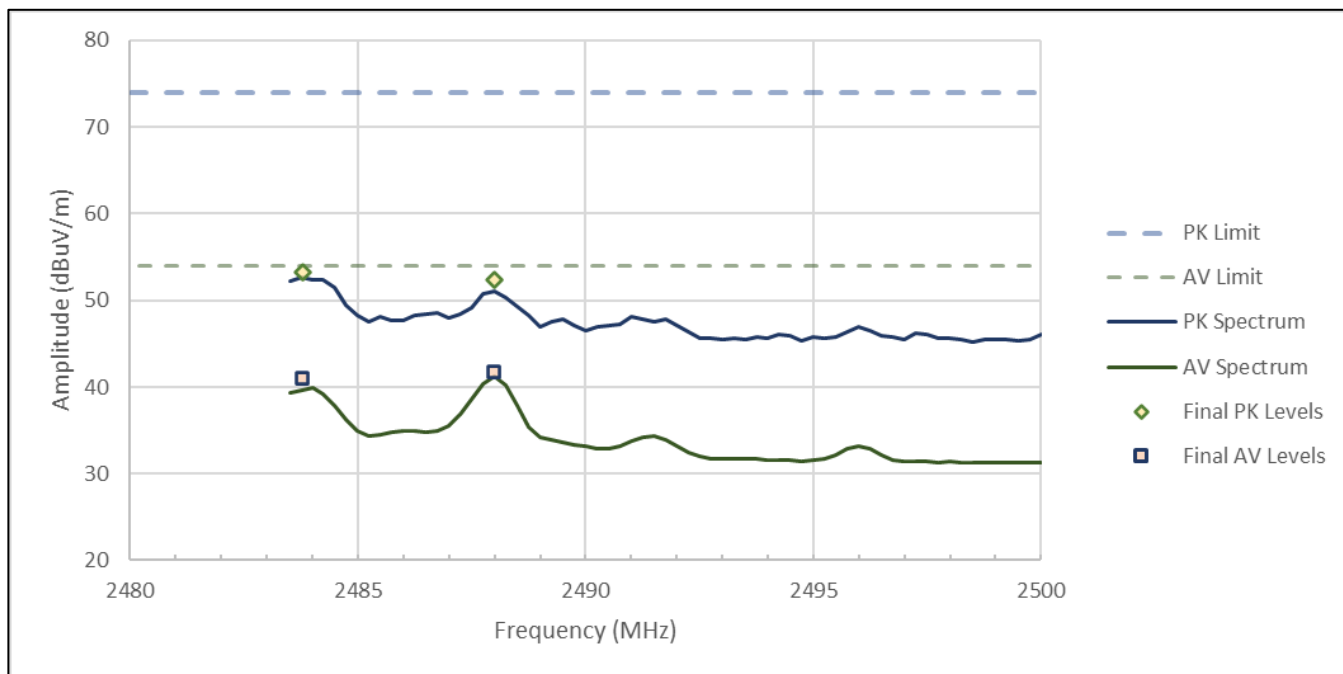
Figure RE04.4: FCC restricted band spectral data from 2483.5 to 2500 MHz (ANT, 2480 MHz)
