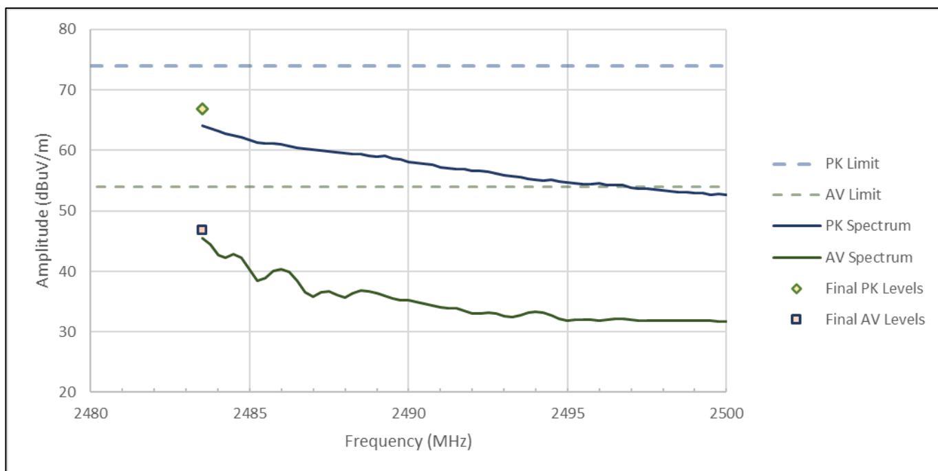
Figure RE03.7: FCC restricted band spectral data from 2483.5 to 2500 MHz (BLE, 2 Mbps, 2478 MHz)
