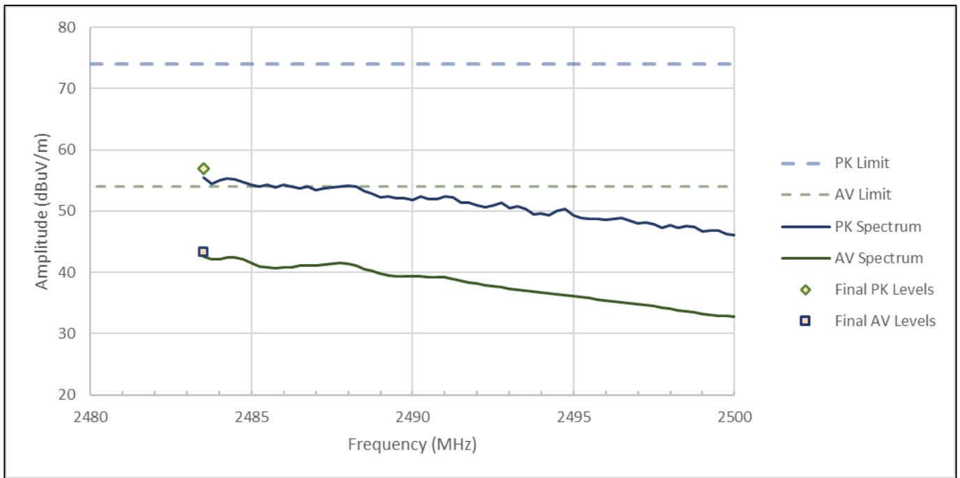
Figure RE01.5: FCC restricted band spectral data from 2483.5 to 2500 MHz (IEEE 802.11b, 1 Mbps, Ch11)
