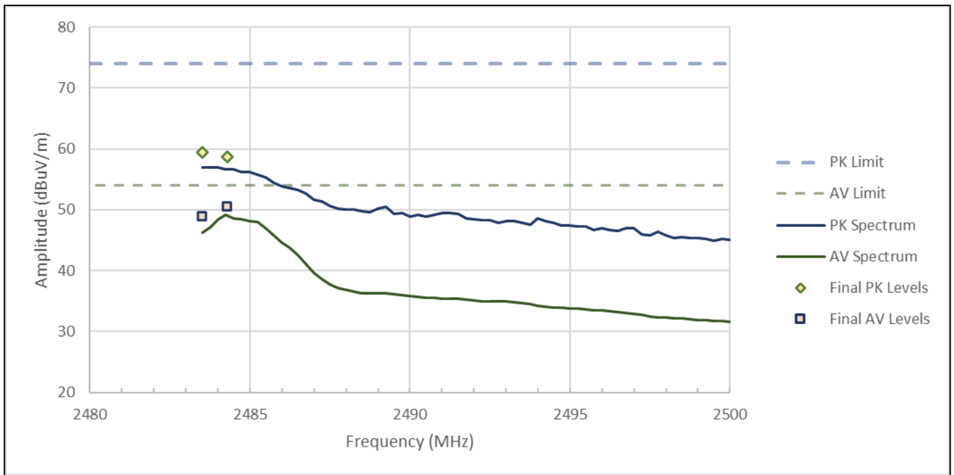
Figure RE01.7: FCC restricted band spectral data from 2483.5 to 2500 MHz (IEEE 802.11b, 1 Mbps, Ch12)
