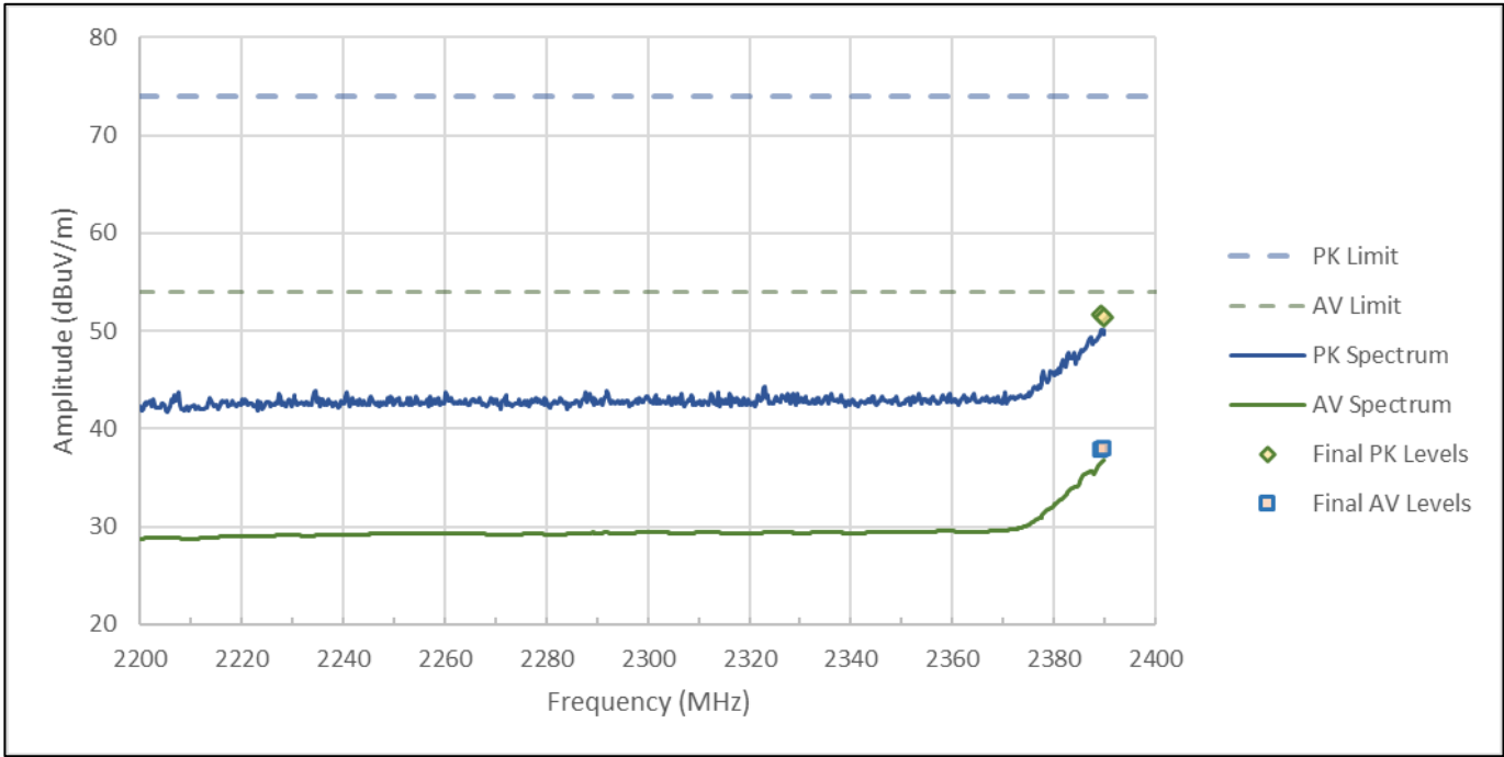
Figure RE01.1: FCC restricted band spectral data from 2200 to 2390 MHz (IEEE 802.11b, 1 Mbps, Ch1)
