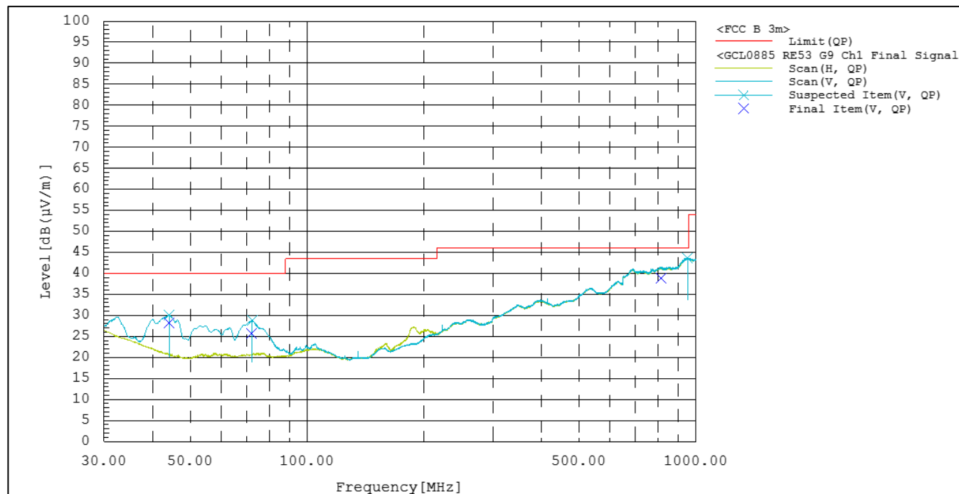
Figure RE53.2: Spectral data (IEEE 802.11g, 9 Mbps, Ch 1)
