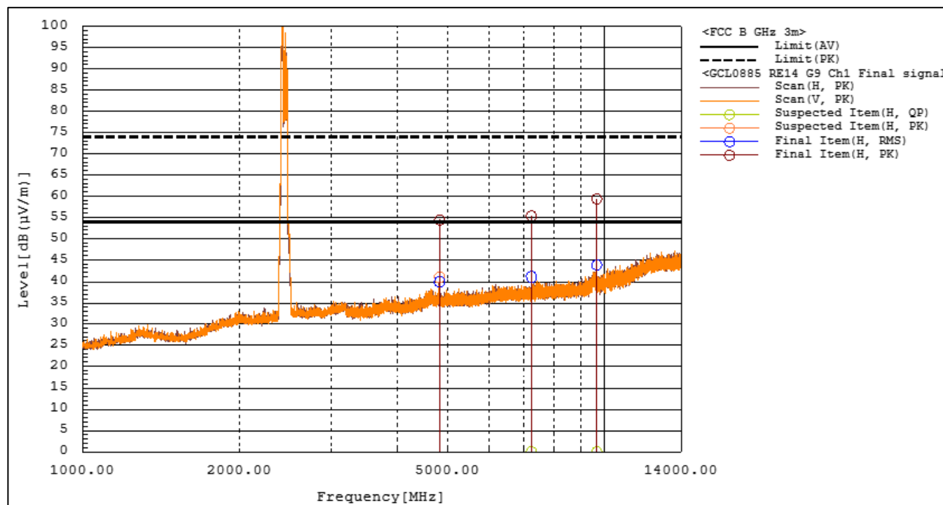
Figure RE13.5: Spectral data (IEEE 802.11g, 9 Mbps, Ch 1)
