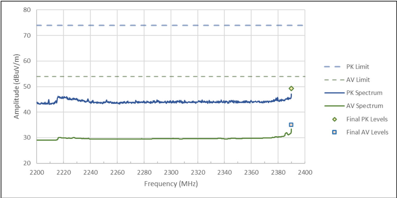
Figure RE04.1: FCC restricted band spectral data from 2200 to 2390 MHz (ANT, 2402 MHz)
