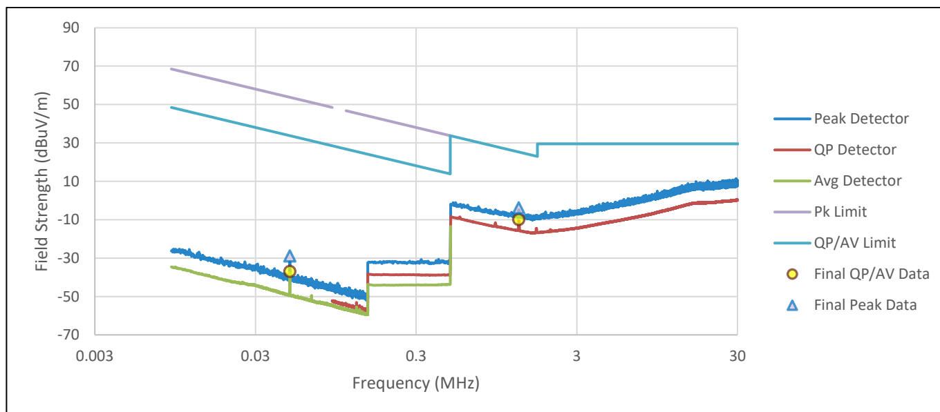
Figure RE24.1: Spectral data (IEEE 802.11b, 1 Mbps, Ch1)
