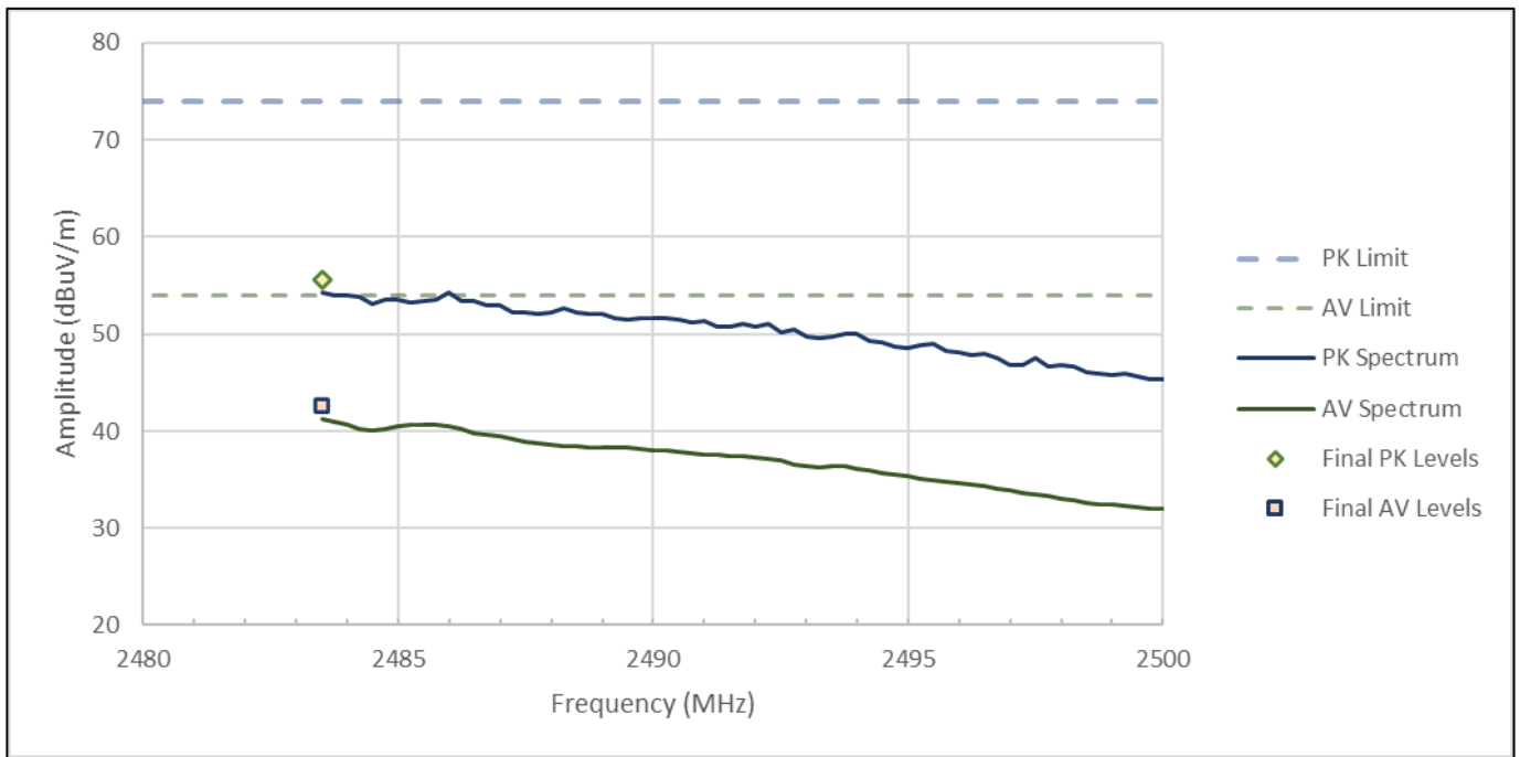
Figure RE01.3: FCC restricted band spectral data from 2483.5 to 2500 MHz (IEEE 802.11b, 1 Mbps, Ch10)
