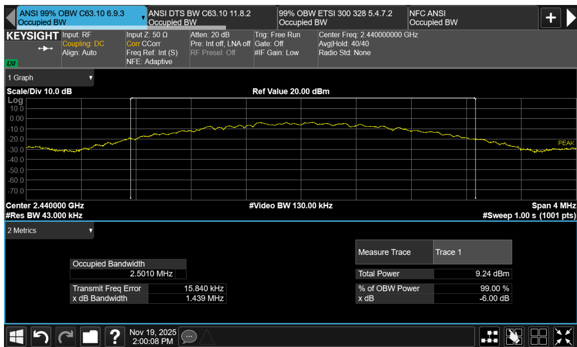
Figure TR15.3: Occupied bandwidth data for BLE 2 Mbps at mid channel (2440 MHz)
