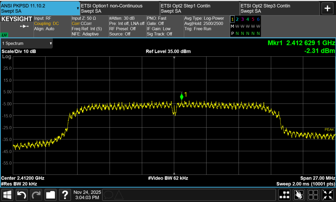
Figure TR30.6: Test data for IEEE 802.11n 1 MCS0 at channel 1
