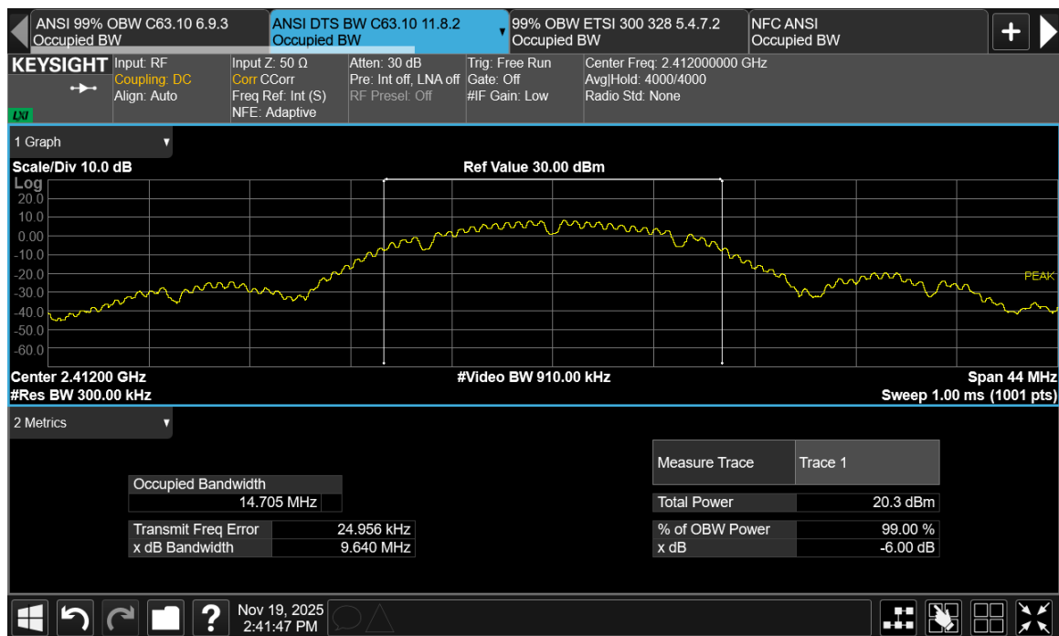
Figure TR11.4: Bandwidth data for 802.11b 1 Mbps at channel 1
