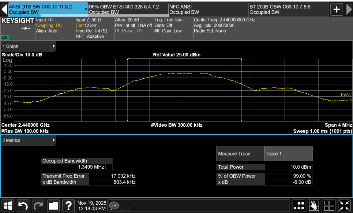
Figure TR11.2: Bandwidth data for ANT at mid channel (2440 MHz)
