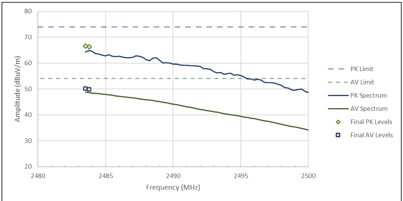
Figure RE01.4: FCC restricted band spectral data from 2483.5 to 2500 MHz (IEEE 802.11n, 3 Mbps, Ch10)
