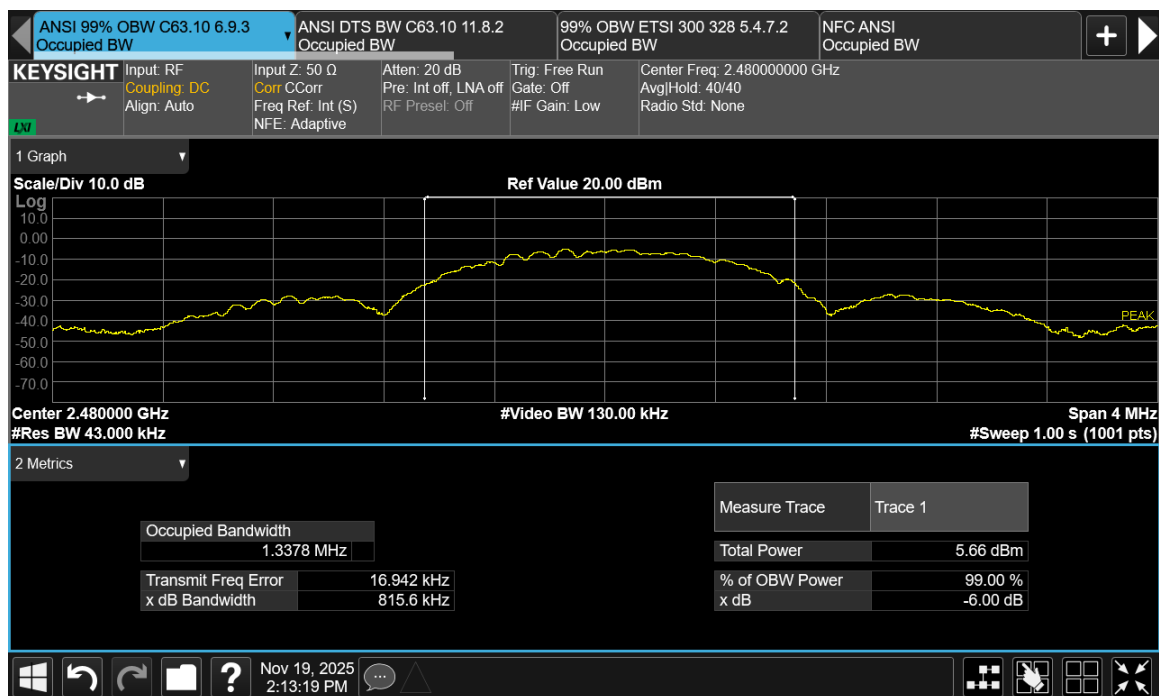
Figure TR15.2: Occupied bandwidth data for ANT at high channel (2480 MHz)
