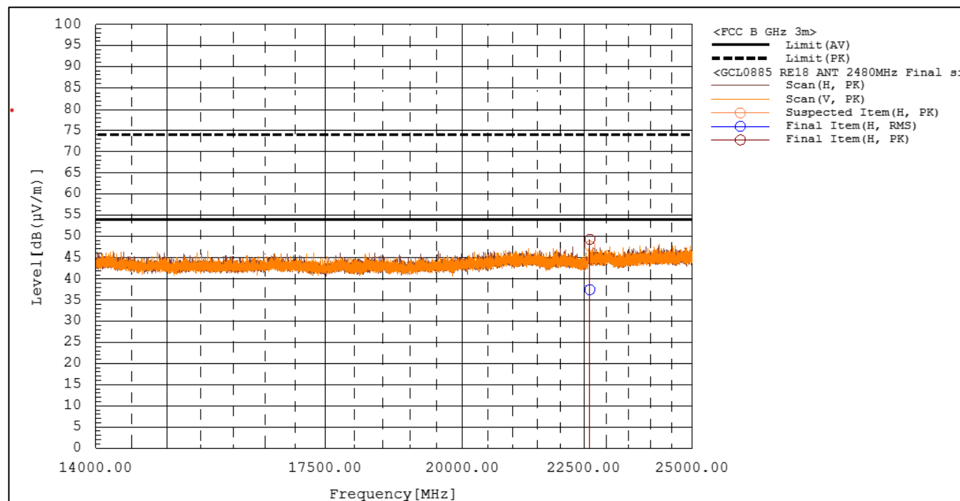
Figure RE18.1: Spectral data (ANT, 2480 MHz)
