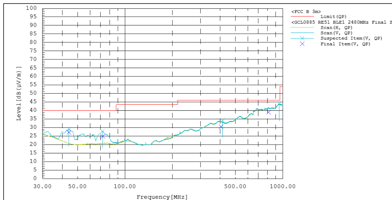
Figure RE51.1: Spectral data (BLE, 1 Mbps, 2480 MHz)
