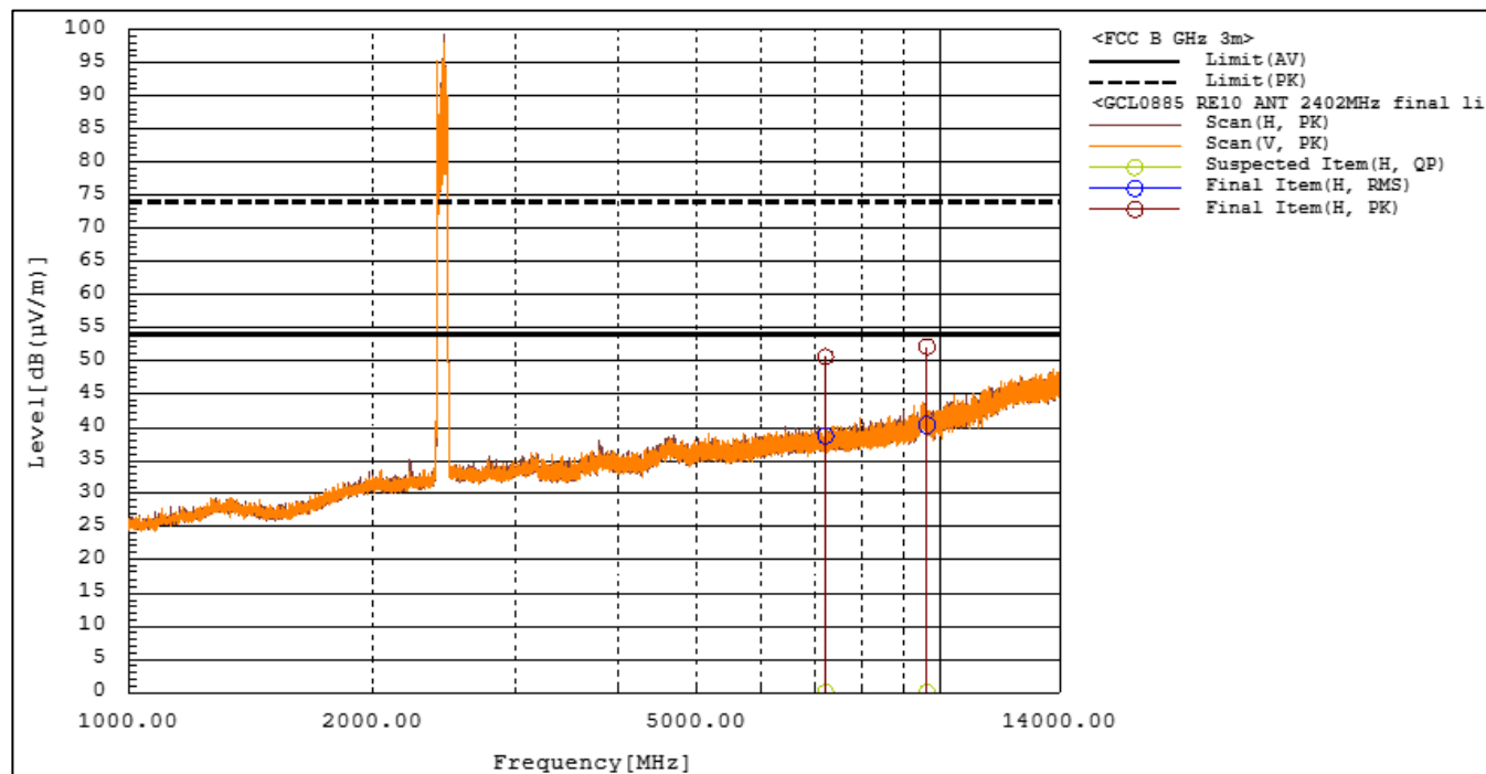
Figure RE10.1: Spectral data (ANT, 2402MHz)
