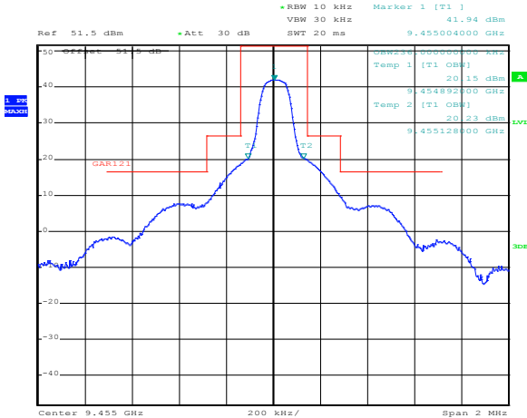
Figure 8.3-2: FCC mask 1/16 mile
