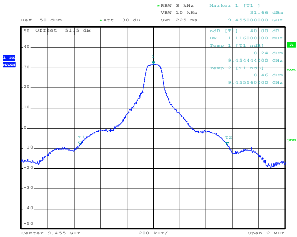
Figure 8.2-2: 40 dB bandwidth 1/16 mile
