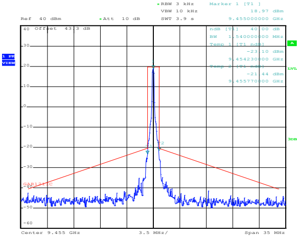
Figure 8.3-1: ISD Mask 1/16 mile
