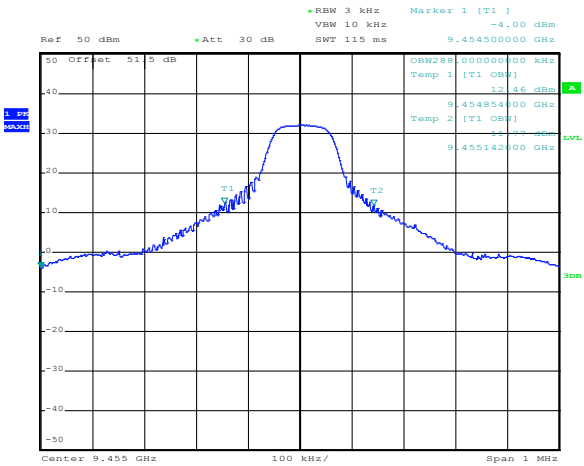
Figure 8.2-1: 99 % Occupied bandwidth 1/16 mile
