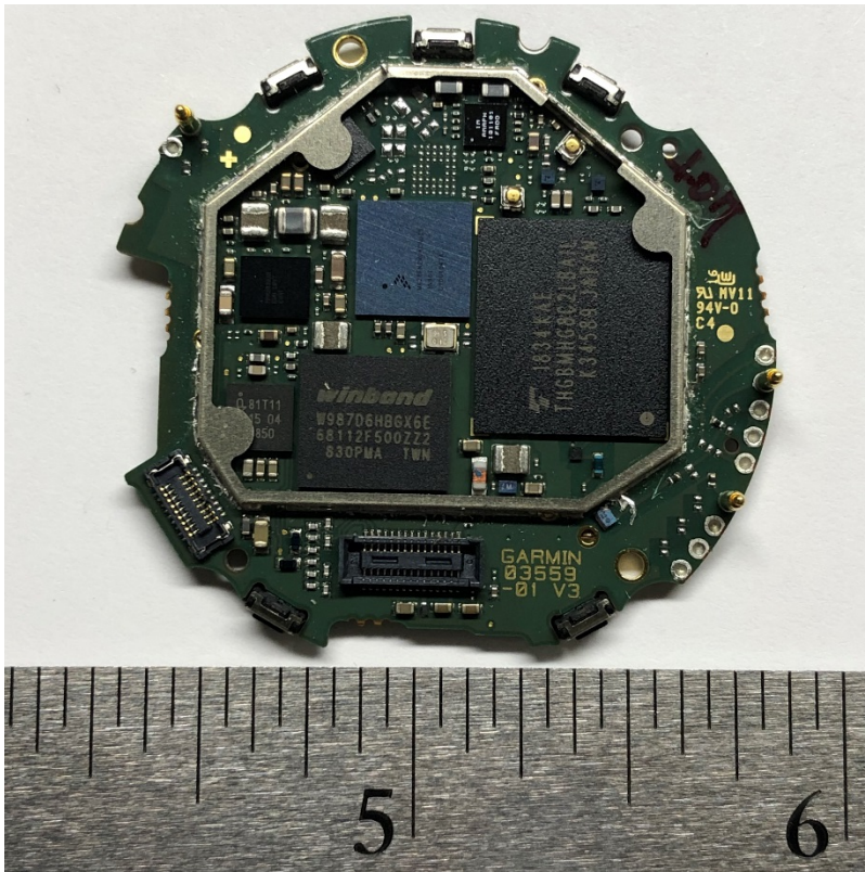
Figure 5 - PCB Rear (un-shielded)
