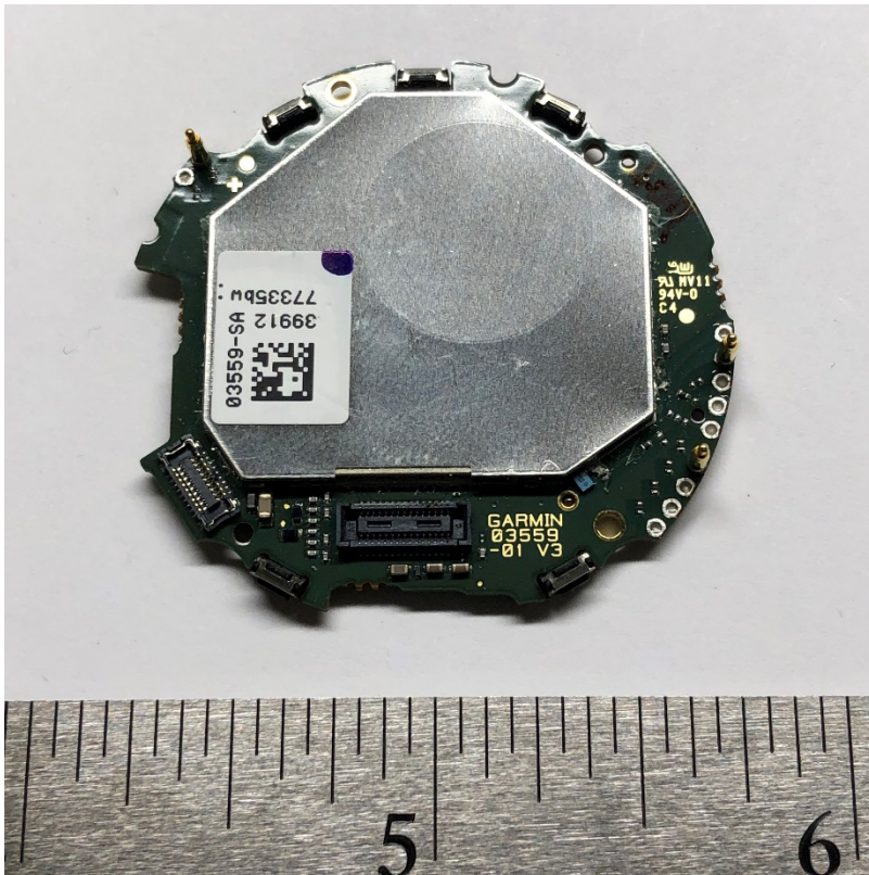
Figure 4 - PCB Rear (shielded)
