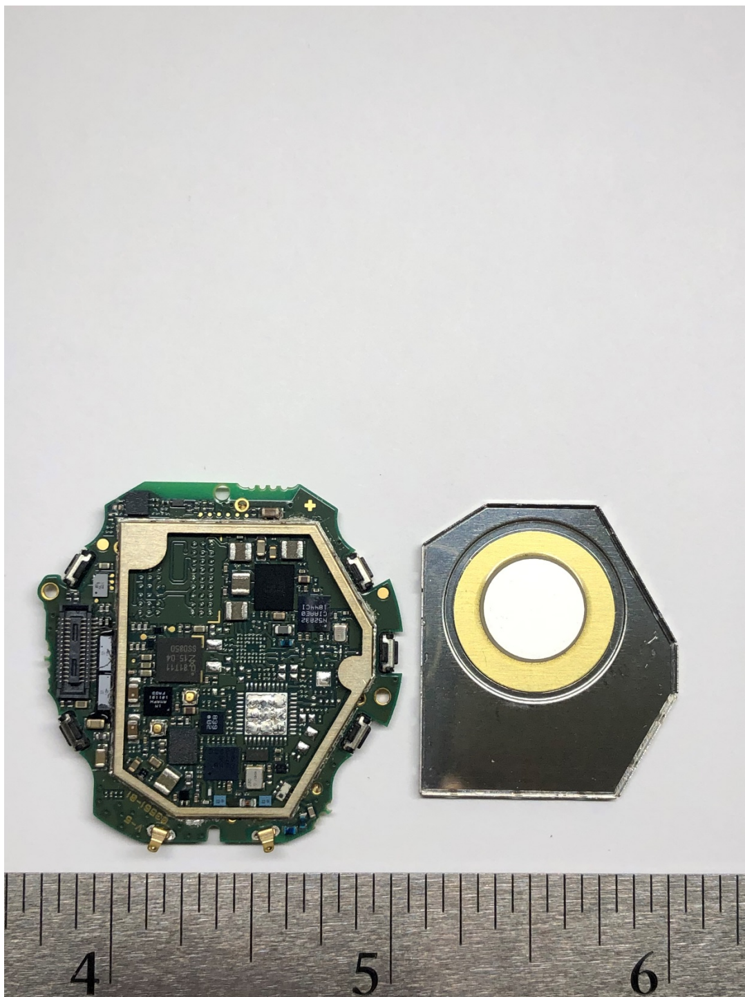
Figure 5 - PCB Rear (un-shielded)
