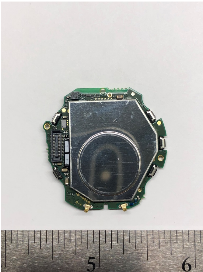
Figure 4 - PCB Rear (shielded)
