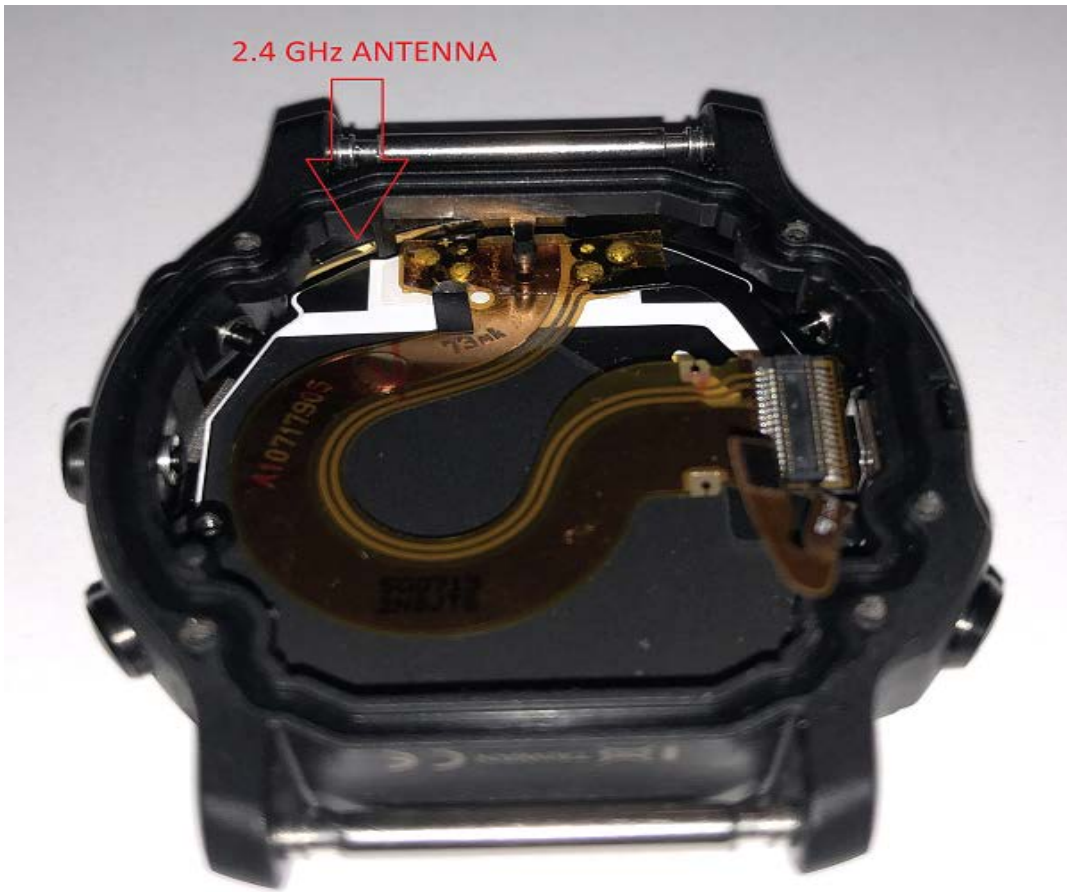
Figure 6 - Antenna
