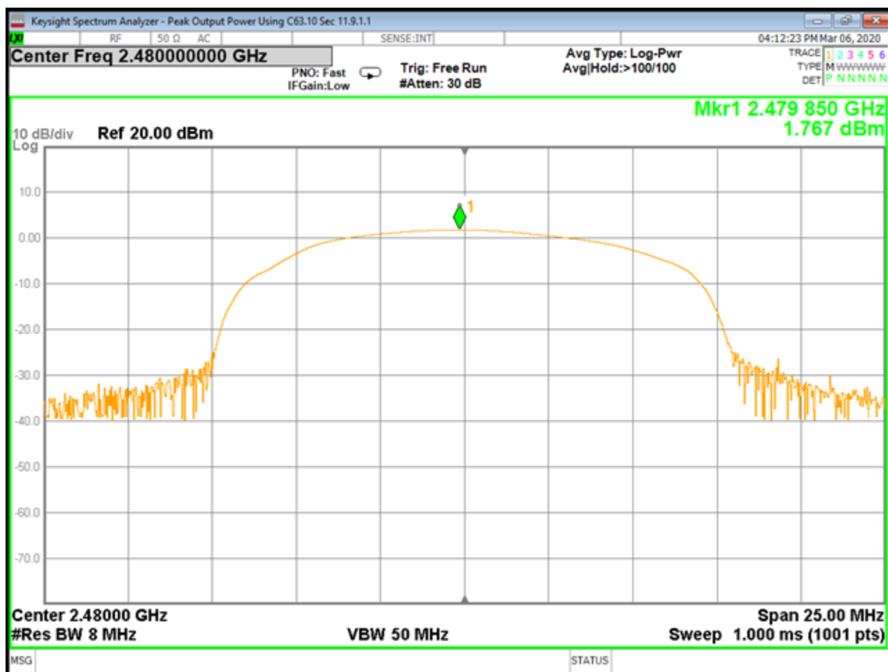
B03908 Peak Output Power High Ch GFSK
