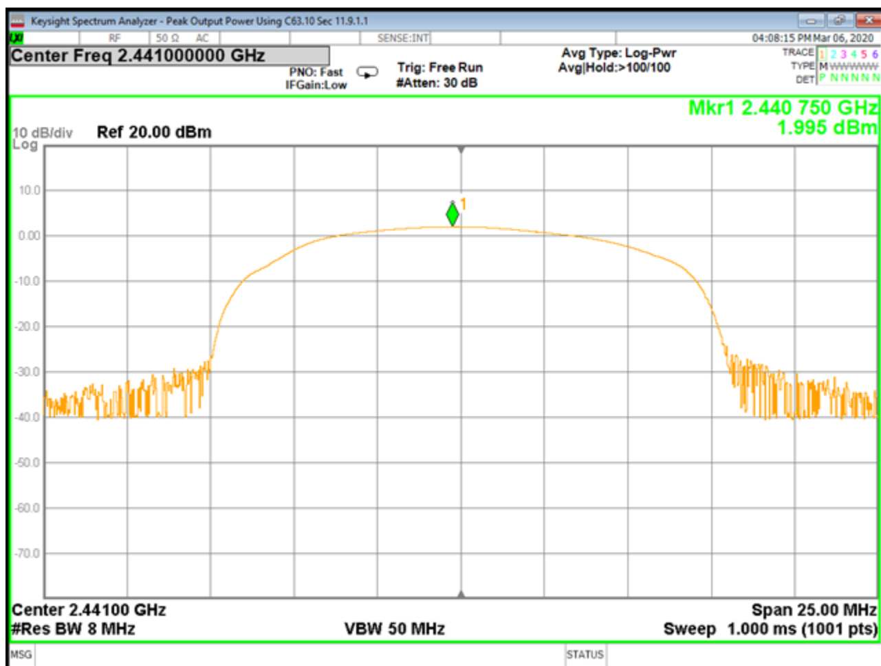
B03908 Peak Output Power Mid Ch GFSK
