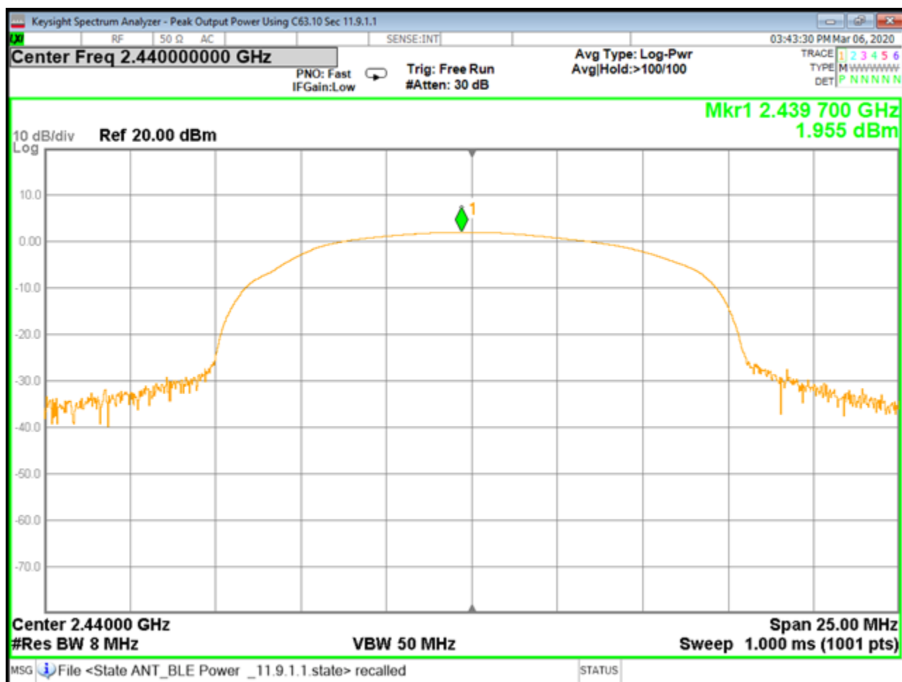
B03908 Peak Output Power Mid Ch GMSK
