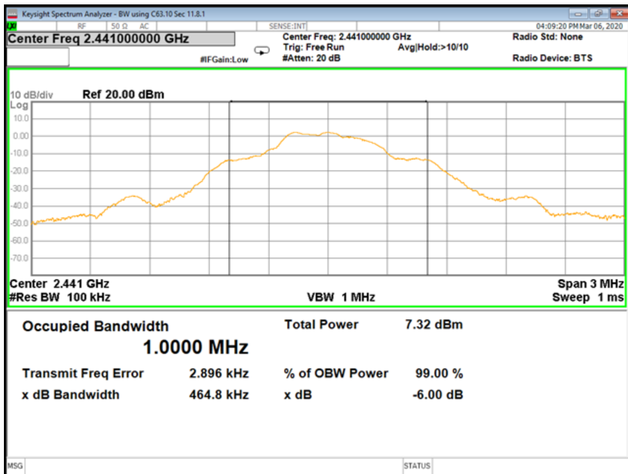
B03908 BW Mid Ch GFSK
