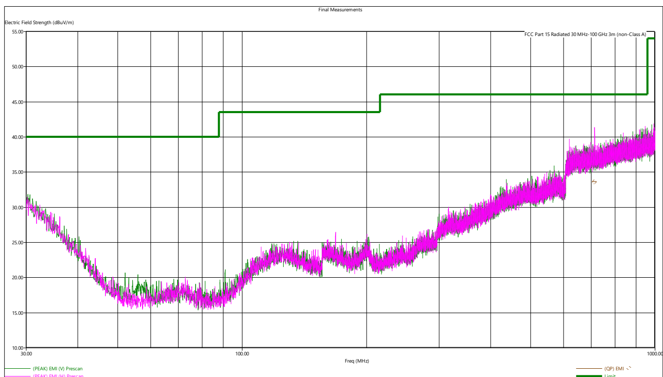
Figure 5 - Radiated Emissions Plot, GMSK
