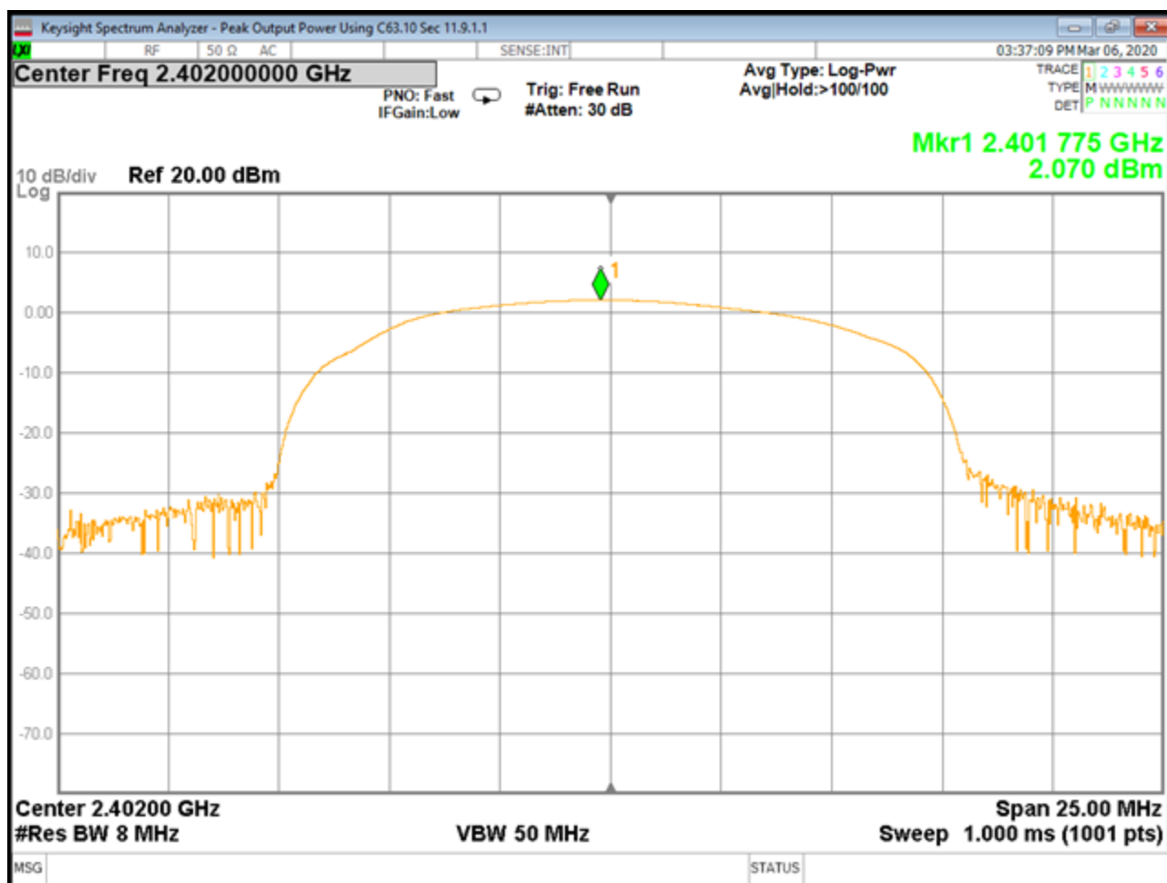
B03908 Peak Output Power Low Ch GMSK
