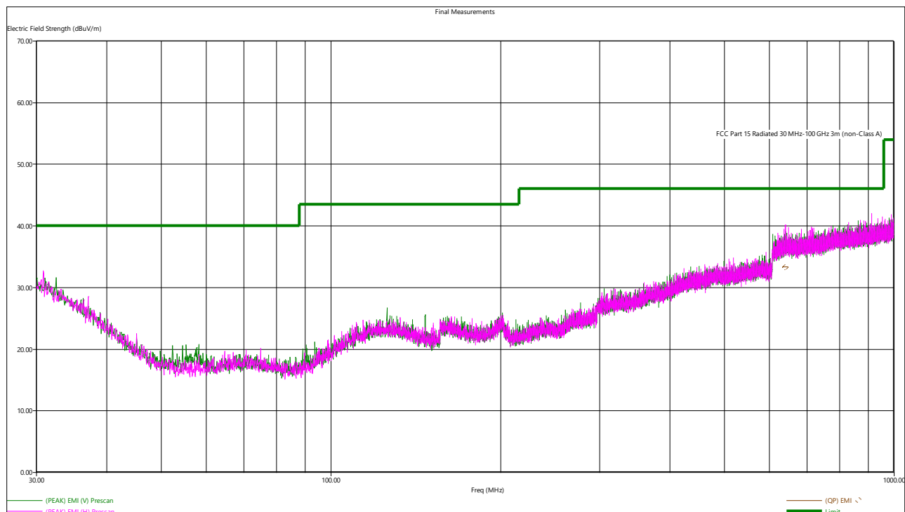
Figure 6 - Radiated Emissions Plot, GFSK
