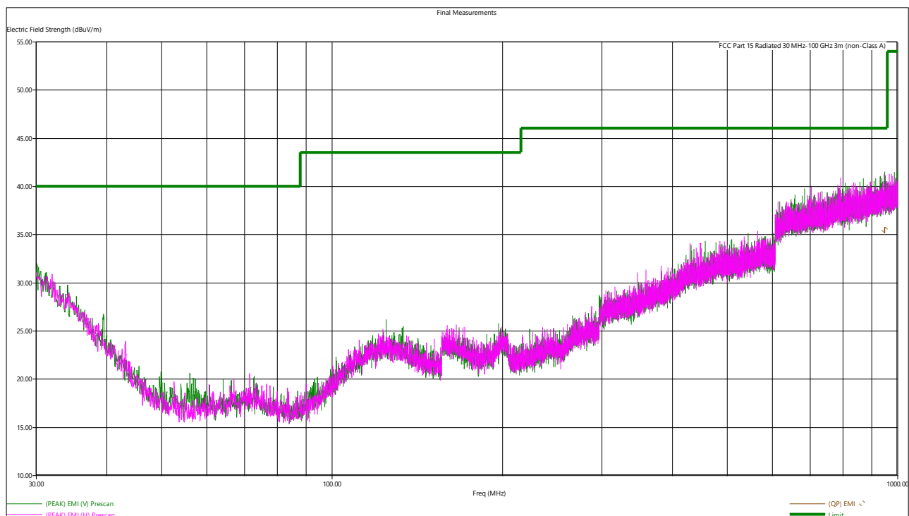
Figure 4 - Radiated Emissions Plot, Receive, GMSK
