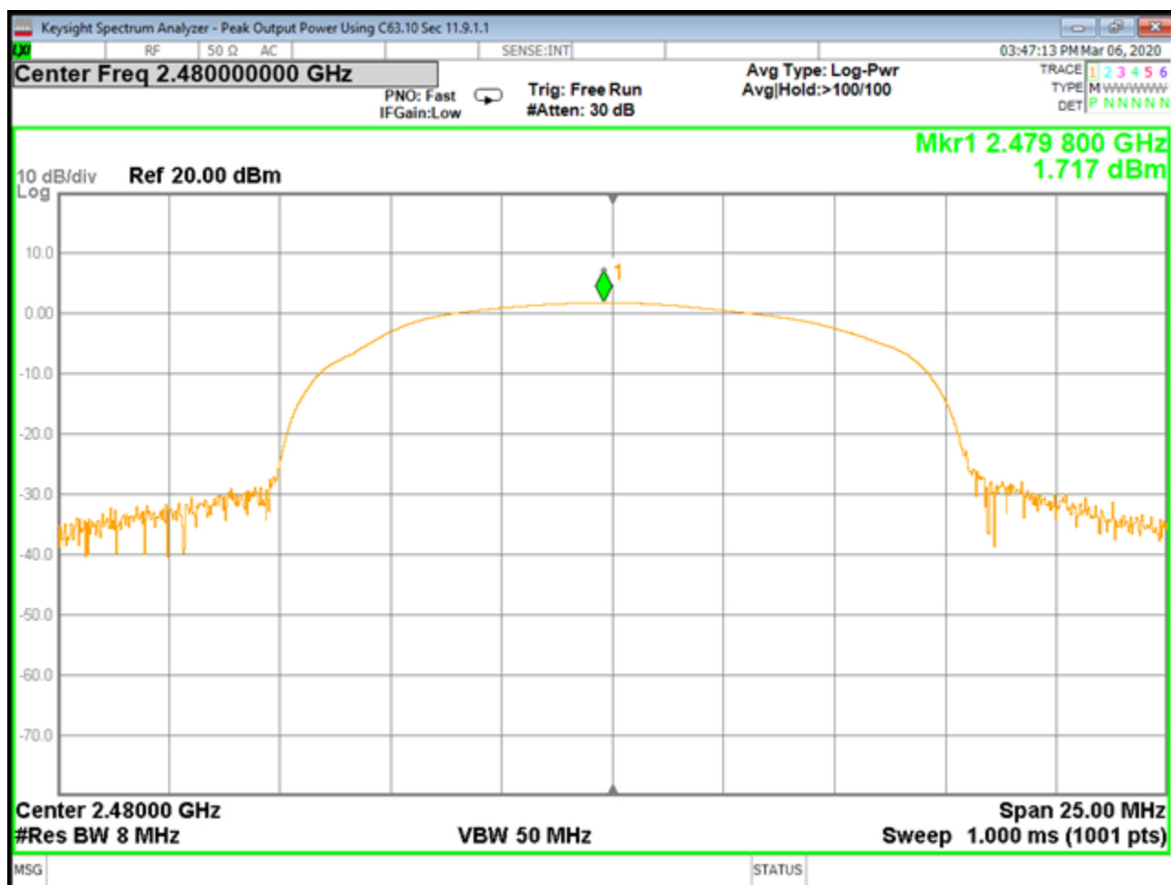
B03908 Peak Output Power High Ch GMSK
