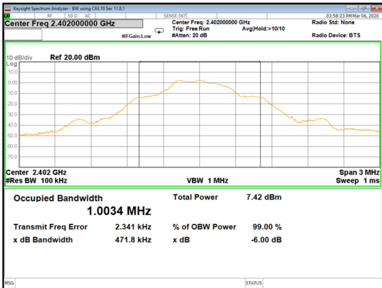
B03908 BW Low Ch GFSK
