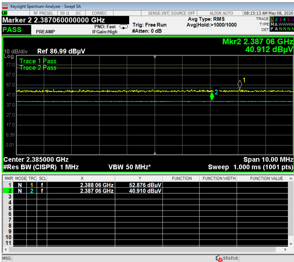
B03908 Peak Restricted Lower Band Edge GFSK
