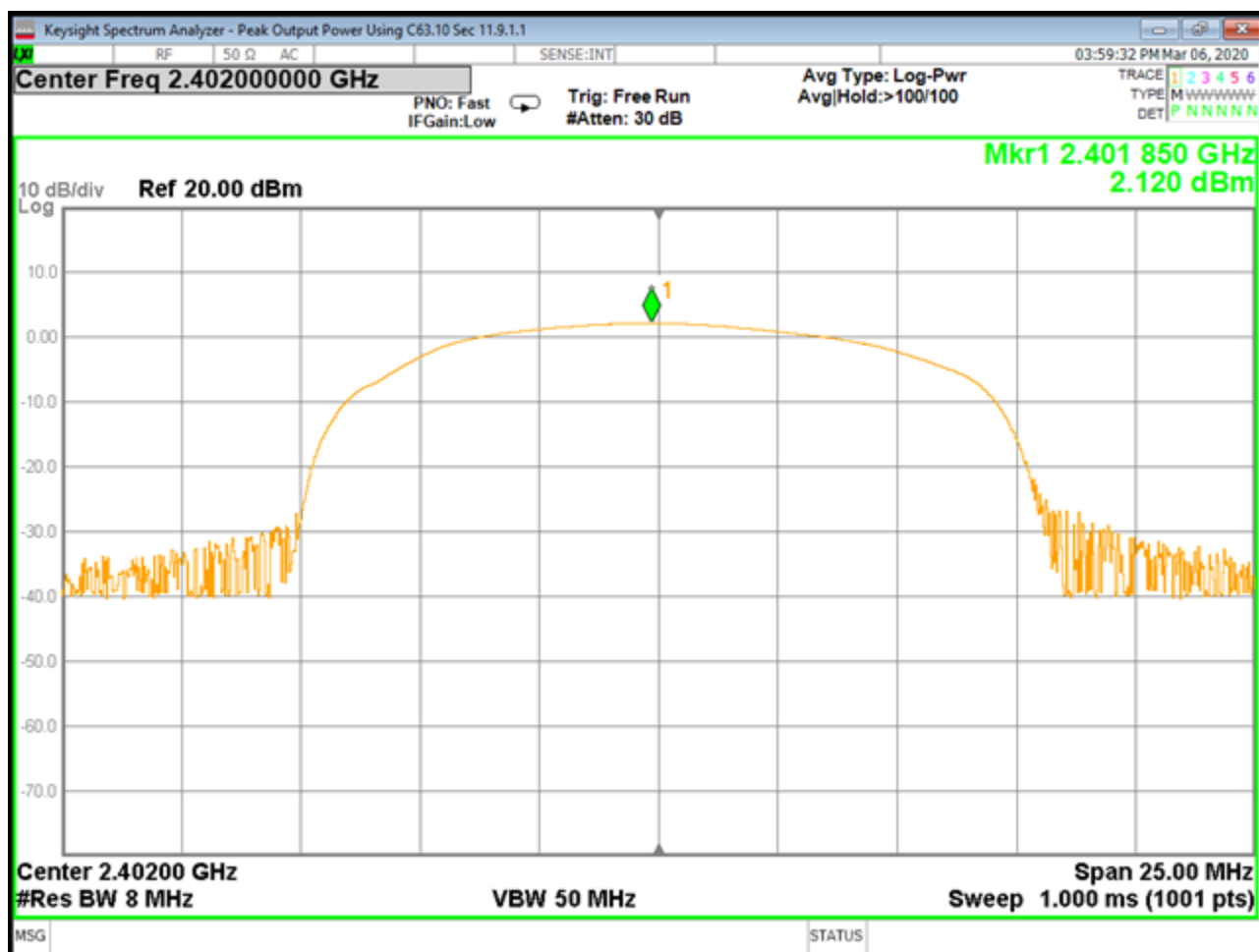
B03908 Peak Output Power Low Ch GFSK
