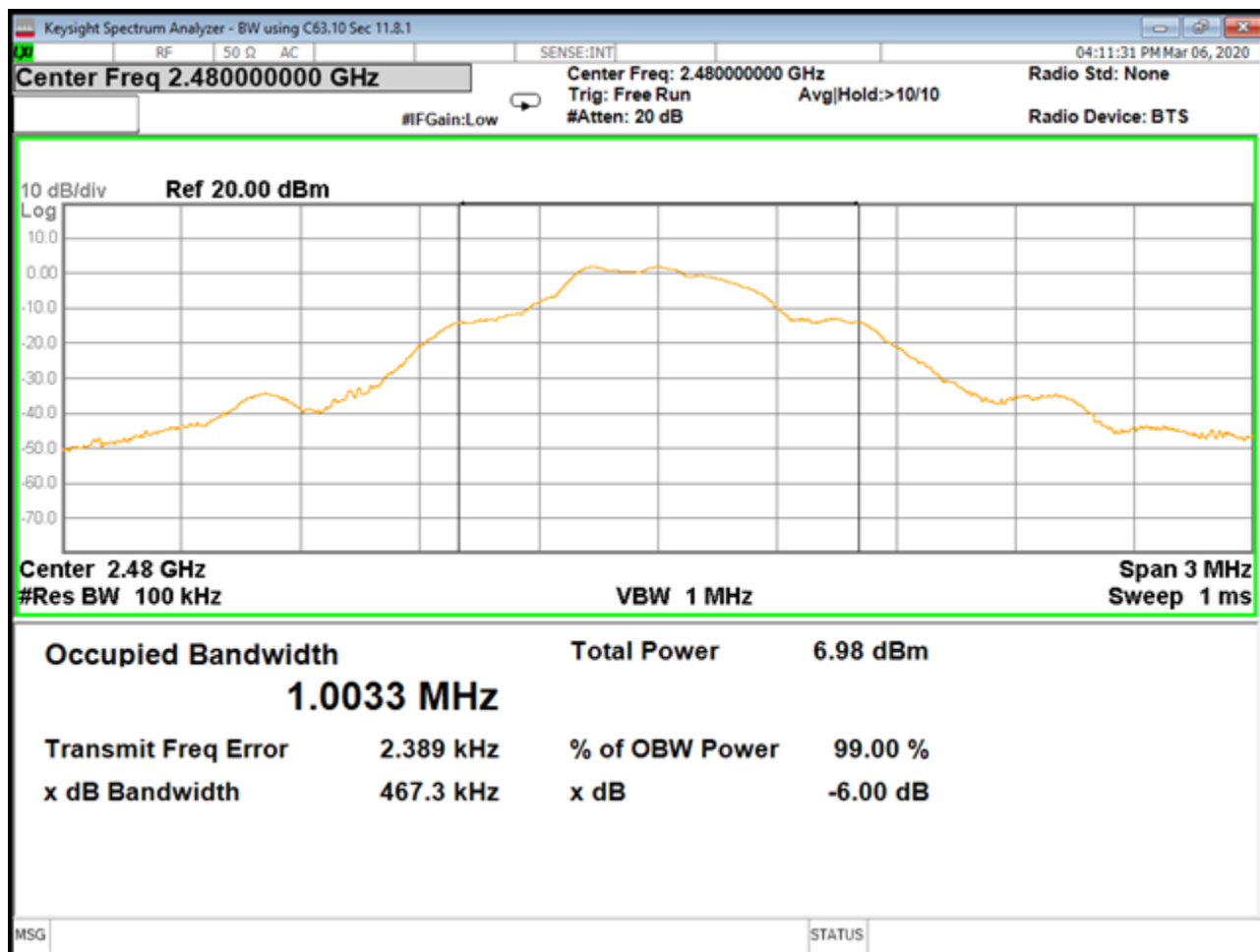
B03908 Bandwidth High Ch GFSK
