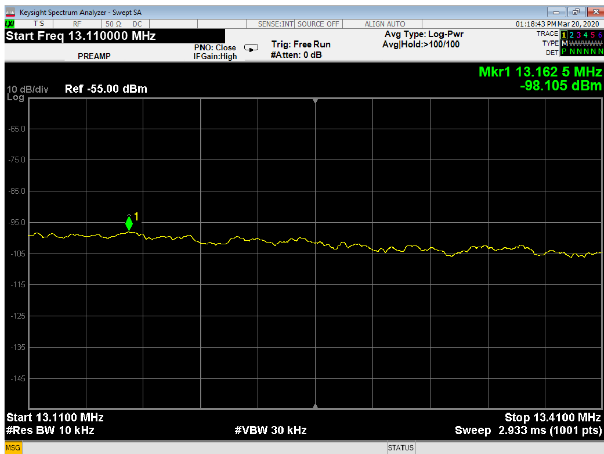
Figure 5 – Lower Band-edge
