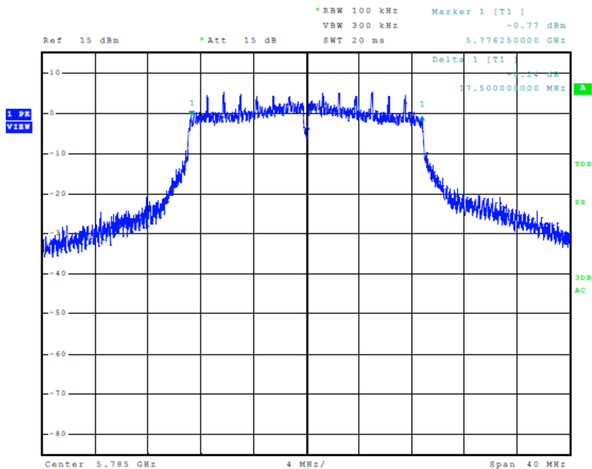
Figure 28 Plot of 6-dB Occupied Bandwidth 5725-5850 MHz Mode 12 U-NII-3 (802.11n)
