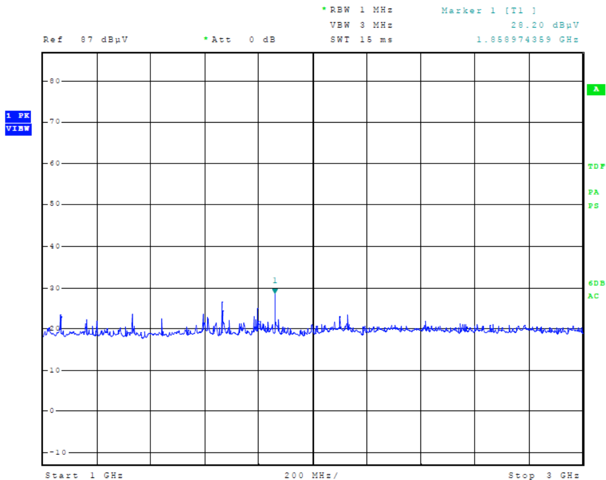
Figure 5 Radiated Emissions Plot taken in screen room (Config #4 / EUT – PC / 1 – 3 GHz)
