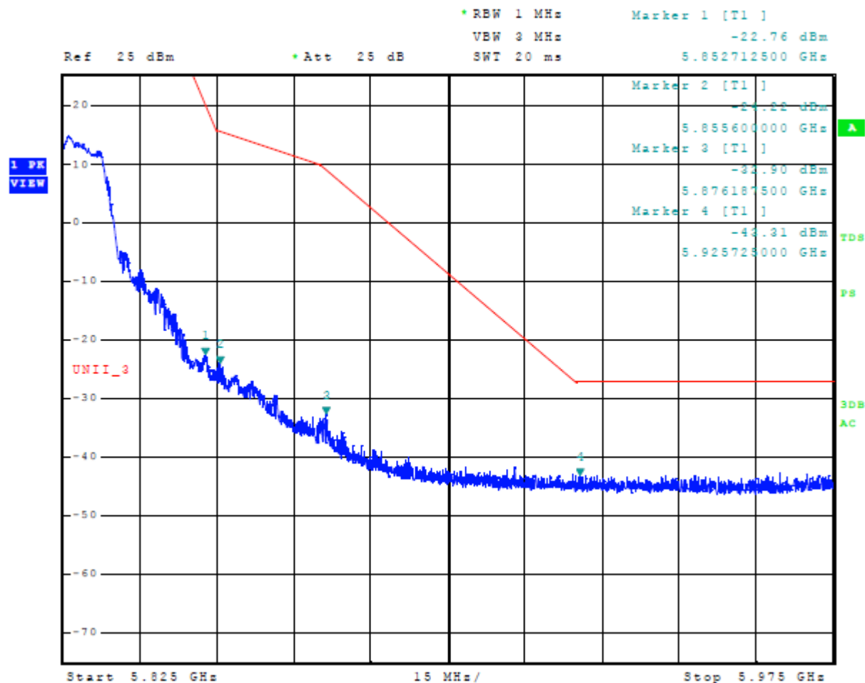
Figure 19 Plot of Upper Band Edge Across 5725-5850 MHz Mode 12 U-NII-3 (802.11a)
