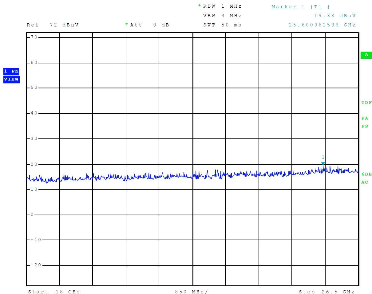
Figure 9 Radiated Emissions Plot taken in screen room (Config #4 / EUT – PC / 18 – 26.5 GHz)
