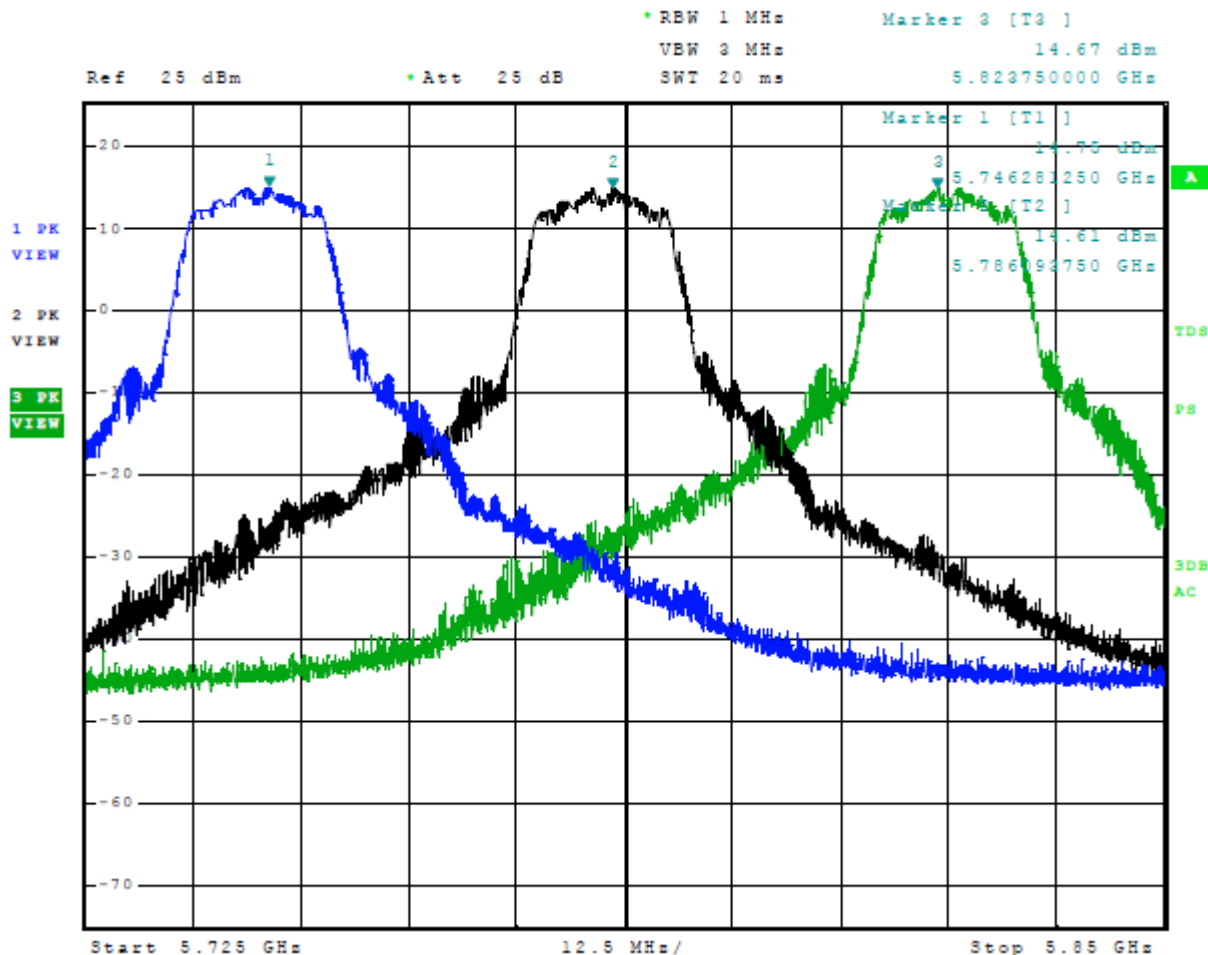
Figure 11 Plot of Transmitter Emissions Across 5725-5850 MHz Mode 12 U-NII-3 (802.11a)
