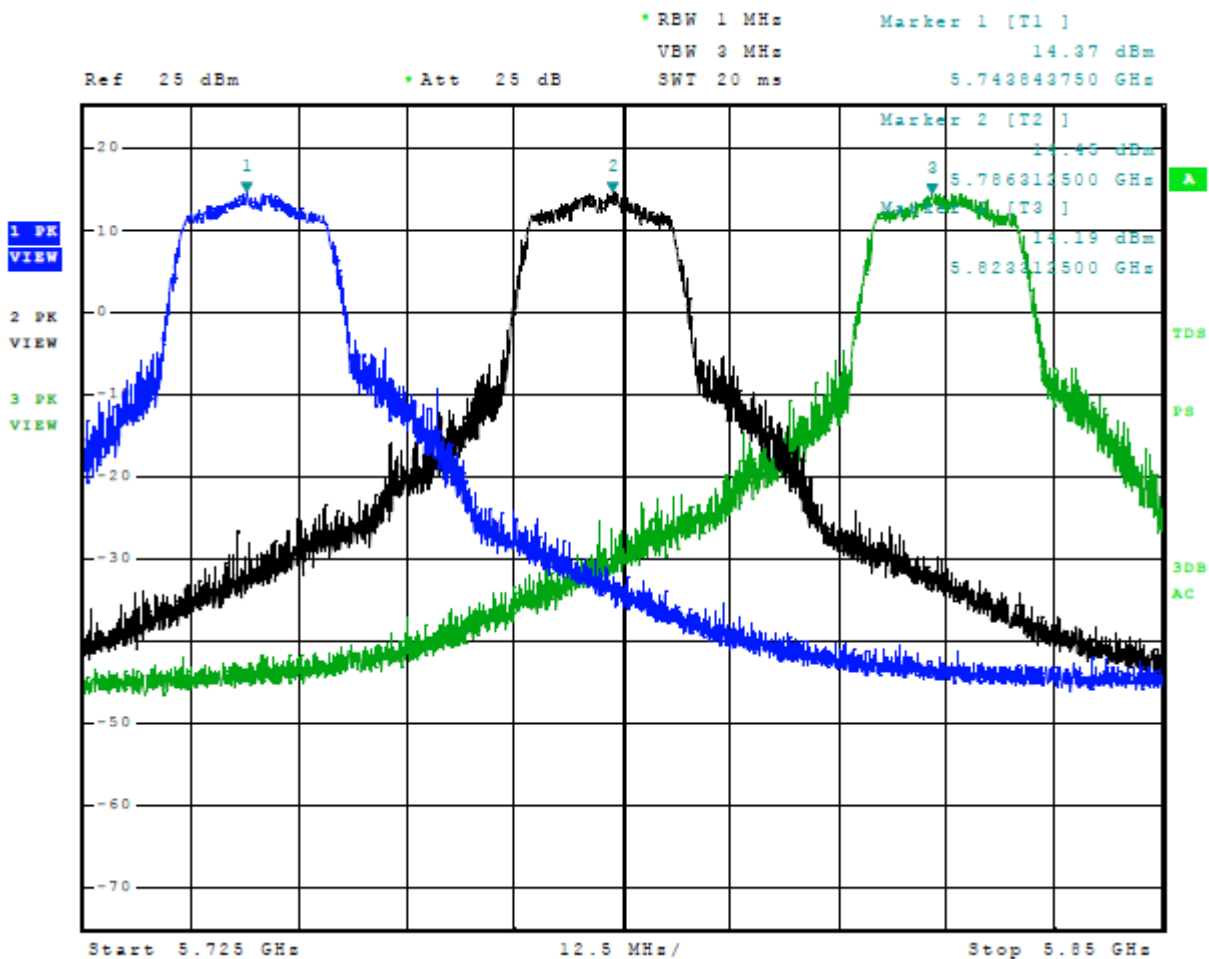
Figure 12 Plot of Transmitter Emissions Across 5725-5850 MHz Mode 13 U-NII-3 (802.11n)
