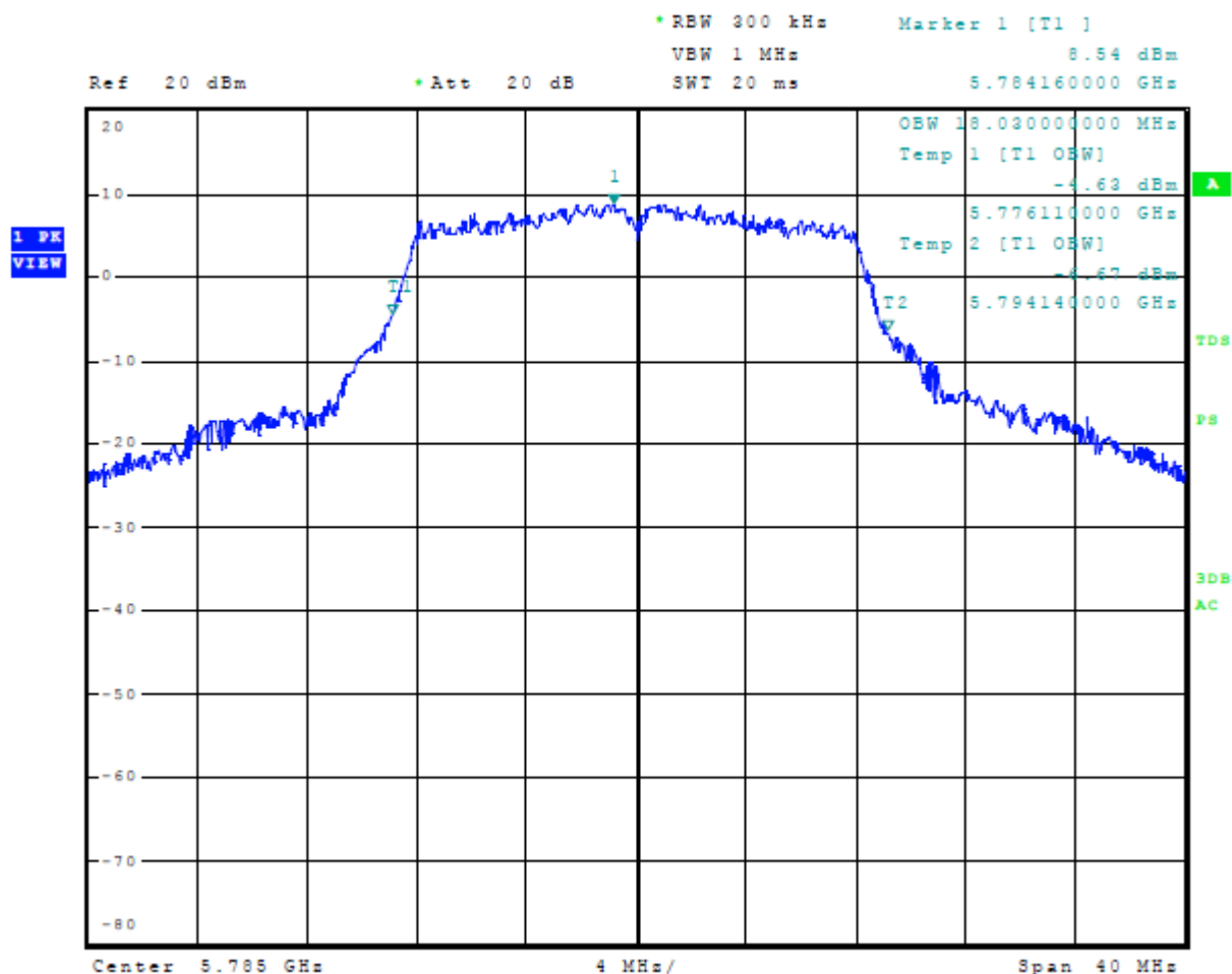
Figure 23 Plot of 99% Occupied Bandwidth 5725-5850 MHz Mode 12 U-NII-3 (802.11a)
