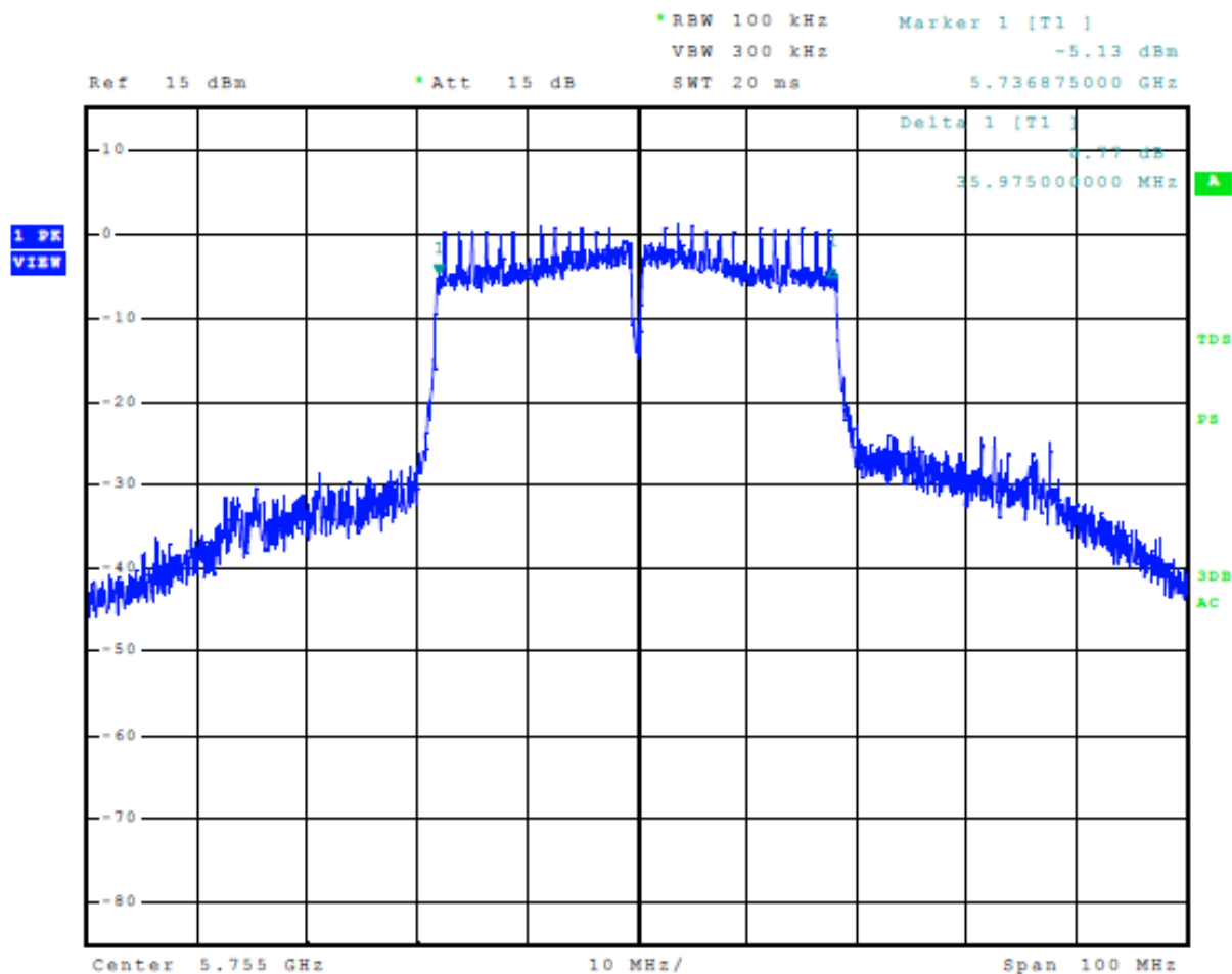
Figure 29 Plot of 6-dB Occupied Bandwidth 5725-5850 MHz Mode 13 U-NII-3 (802.11n40)
