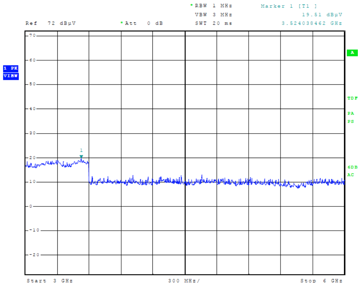
Figure 6 Radiated Emissions Plot taken in screen room (Config #4 / EUT – PC / 3 – 6 GHz)
