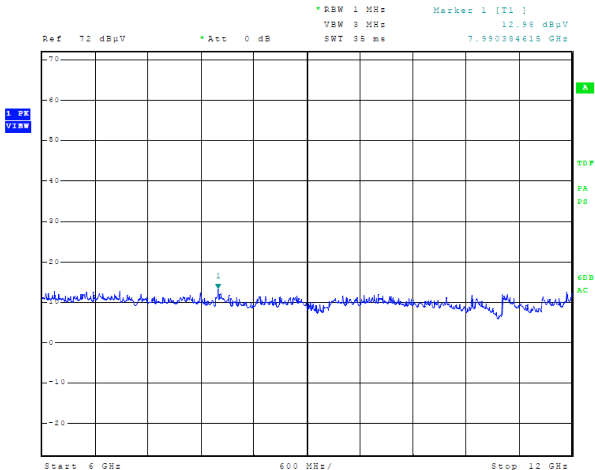
Figure 7 Radiated Emissions Plot taken in screen room (Config #4 / EUT – PC / 6 – 12 GHz)
