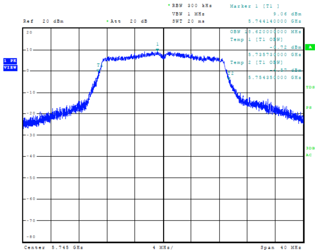
Figure 24 Plot of 99% Occupied Bandwidth 5725-5850 MHz Mode 13 U-NII-3 (802.11n)
