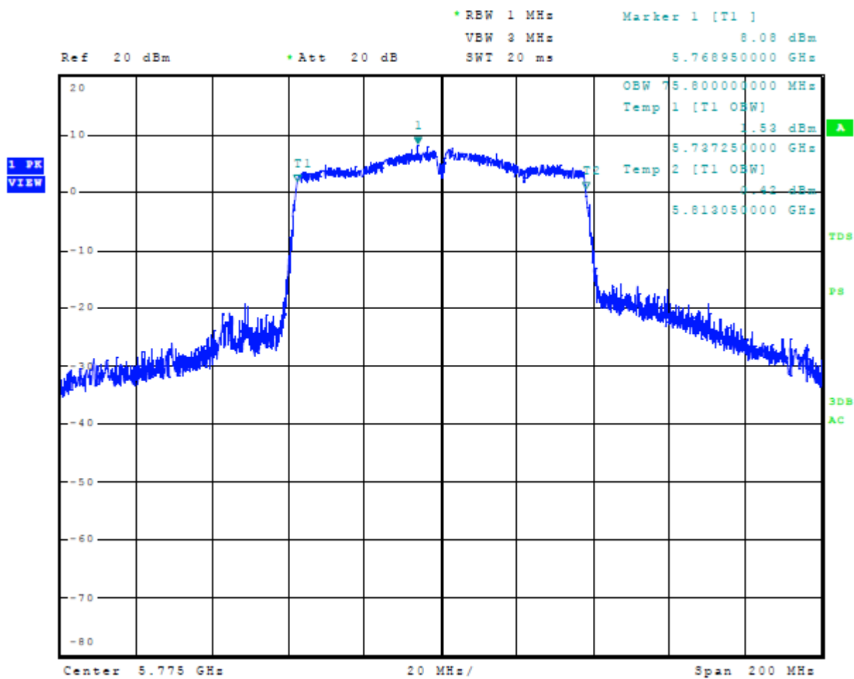
Figure 26 Plot of 99% Occupied Bandwidth 5725-5850 MHz Mode 15 U-NII-3 (802.11ac80)
