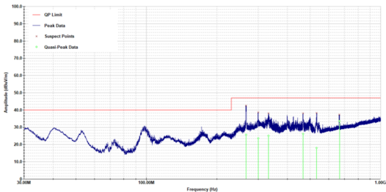
Figure 4 Plot of General Radiated Emissions – Vertical Polarization
