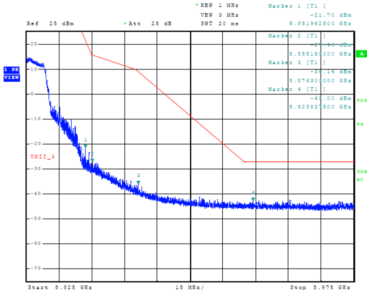
Figure 20 Plot of Upper Band Edge Across 5725-5850 MHz Mode 13 U-NII-3 (802.11n)
