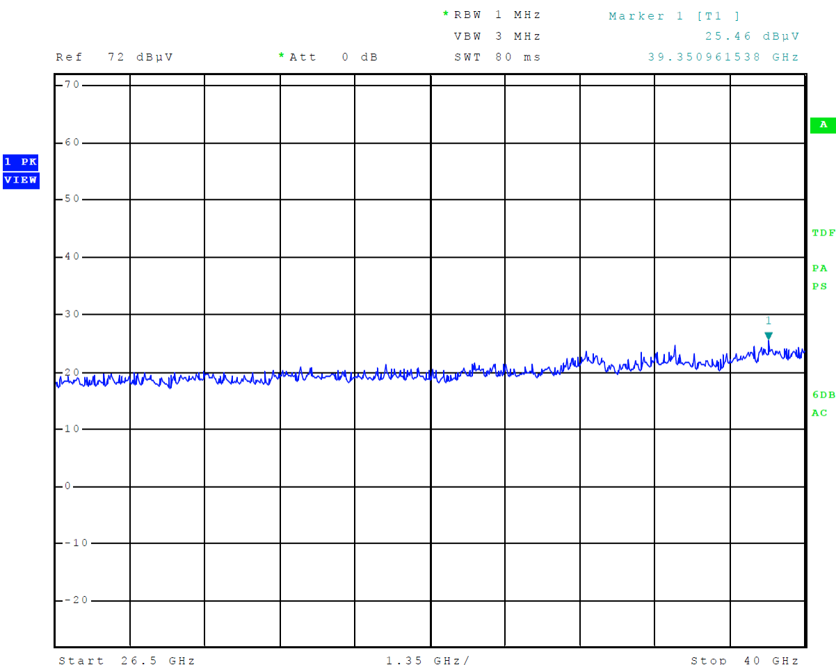
Figure 10 Radiated Emissions Plot taken in screen room (Config #4 / EUT – PC / 26.5 – 40 GHz)
