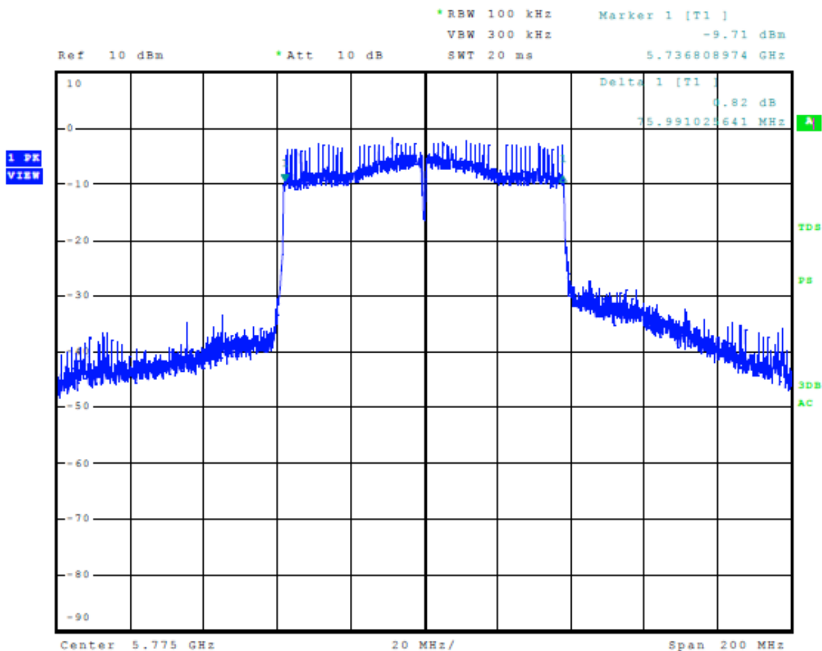
Figure 30 Plot of 6-dB Occupied Bandwidth 5725-5850 MHz Mode 15 U-NII-3 (802.11ac80)
