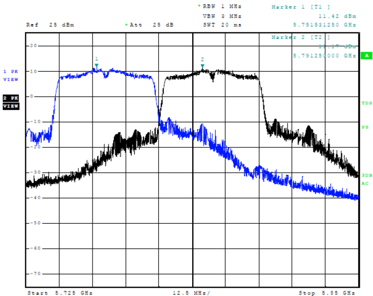
Figure 13 Plot of Transmitter Emissions Across 5725-5850 MHz Mode 14 U-NII-3 (802.11n40)
