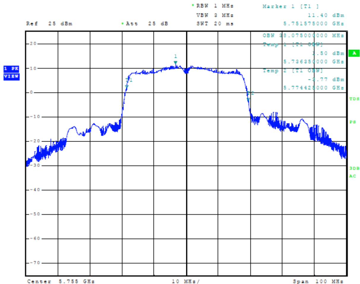
Figure 25 Plot of 99% Occupied Bandwidth 5725-5850 MHz Mode 14 U-NII-3 (802.11n40)
