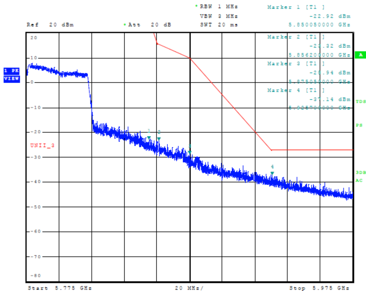
Figure 22 Plot of Upper Band Edge Across 5725-5850 MHz Mode 15 U-NII-3 (802.11ac80)
