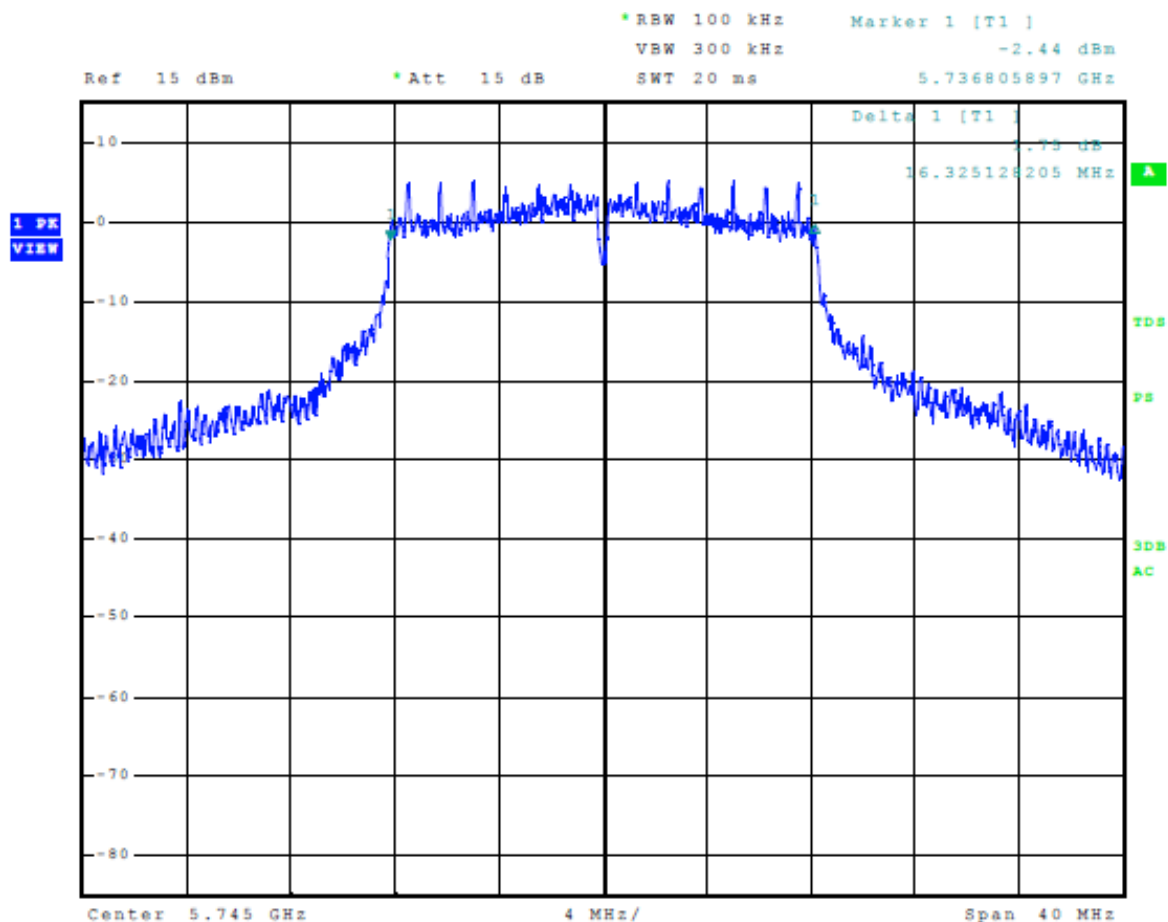
Figure 27 Plot of 6-dB Occupied Bandwidth 5725-5850 MHz Mode 11 U-NII-3 (802.11a)
