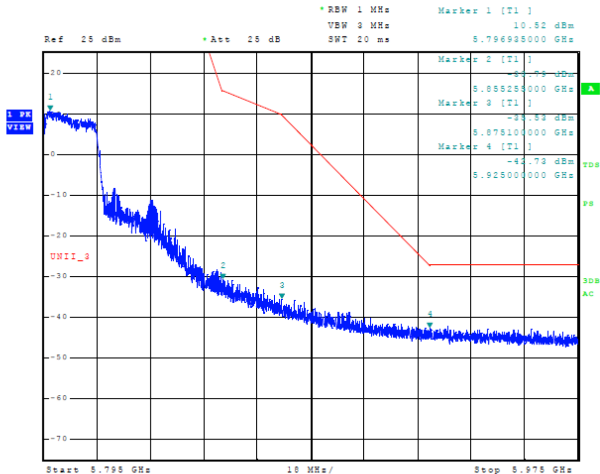
Figure 21 Plot of Upper Band Edge Across 5725-5850 MHz Mode 14 U-NII-3 (802.11n40)
