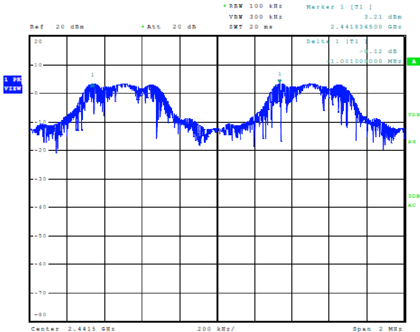
Figure 13 Plot of Channel Separation Mode 1 BT BR (GFSK)
