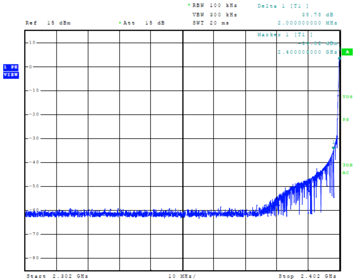
Figure 15 Plot of Transmitter Emissions Low Band Edge Mode 1, BT BR
