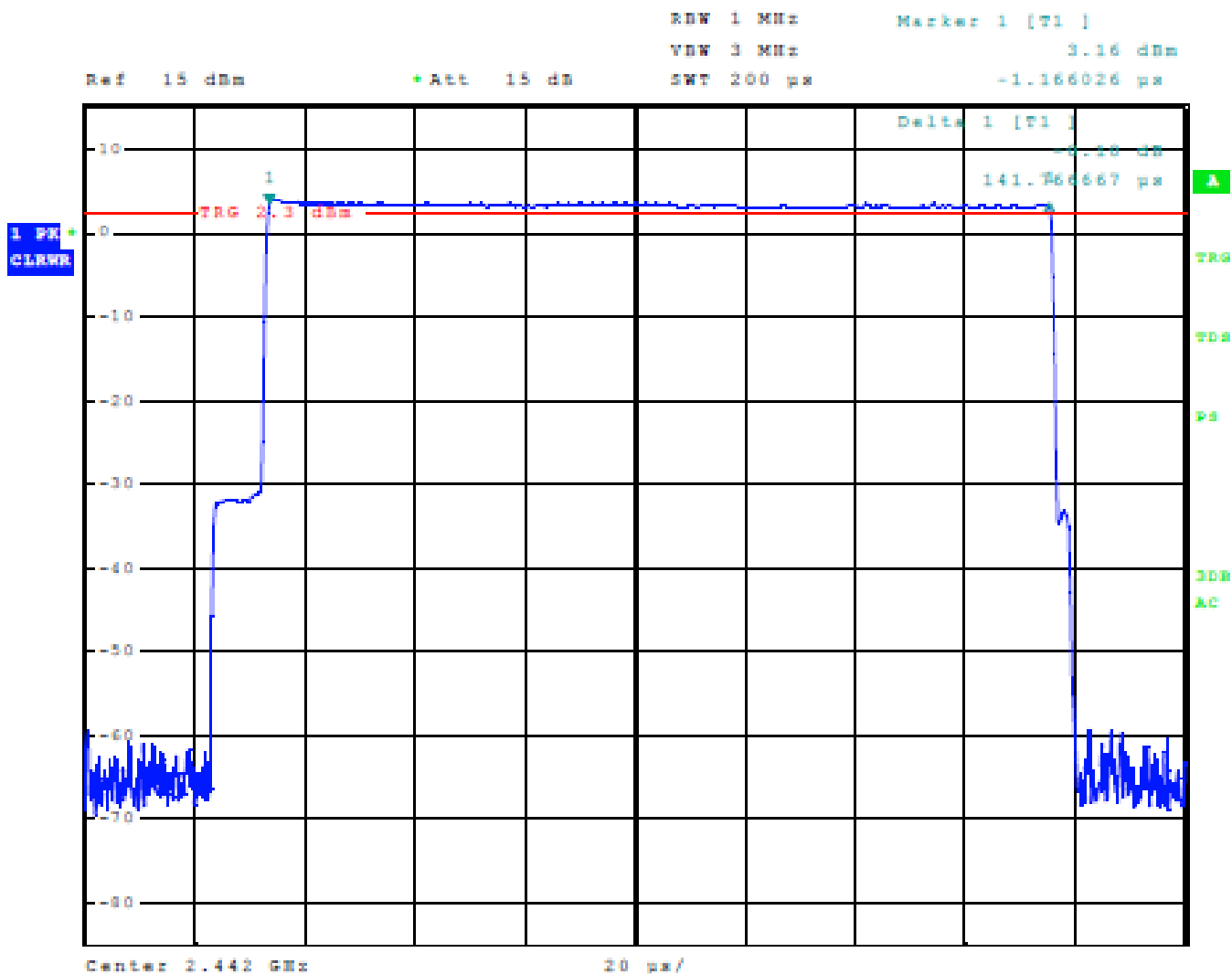
Figure 12 Plot of Dwell time On Channel Mode 1 BT BR (GFSK)
