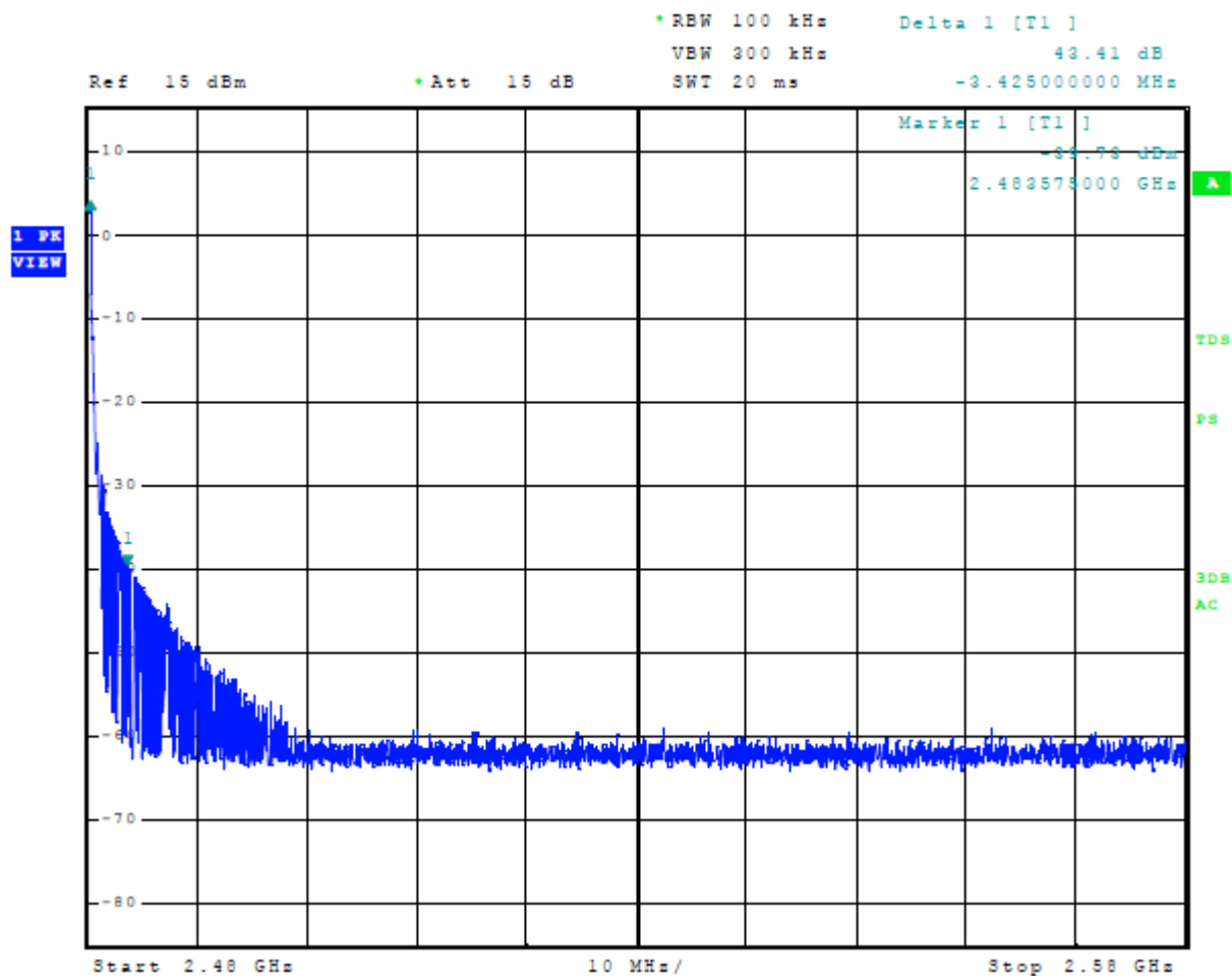
Figure 16 Plot of Transmitter Emissions High Band Edge Mode 1, BT BR
