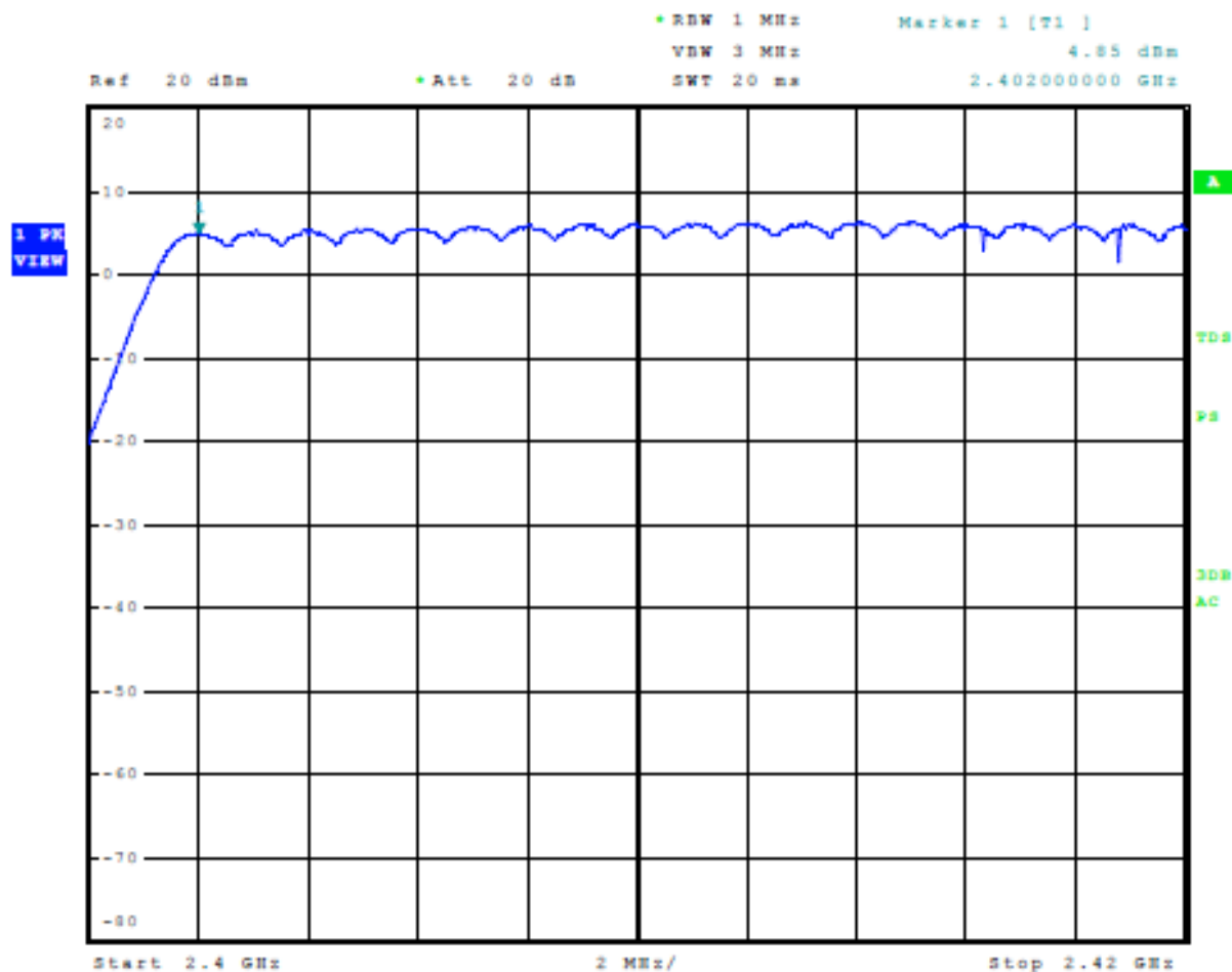
Figure 8 Plot of Number of Hopping Channels Mode 1 BT BR (GFSK)
