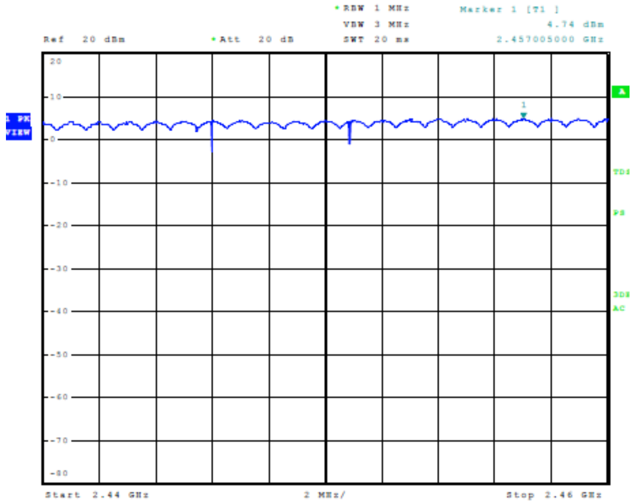
Figure 10 Plot of Number of Hopping Channels Mode 1 BT BR (GFSK)
