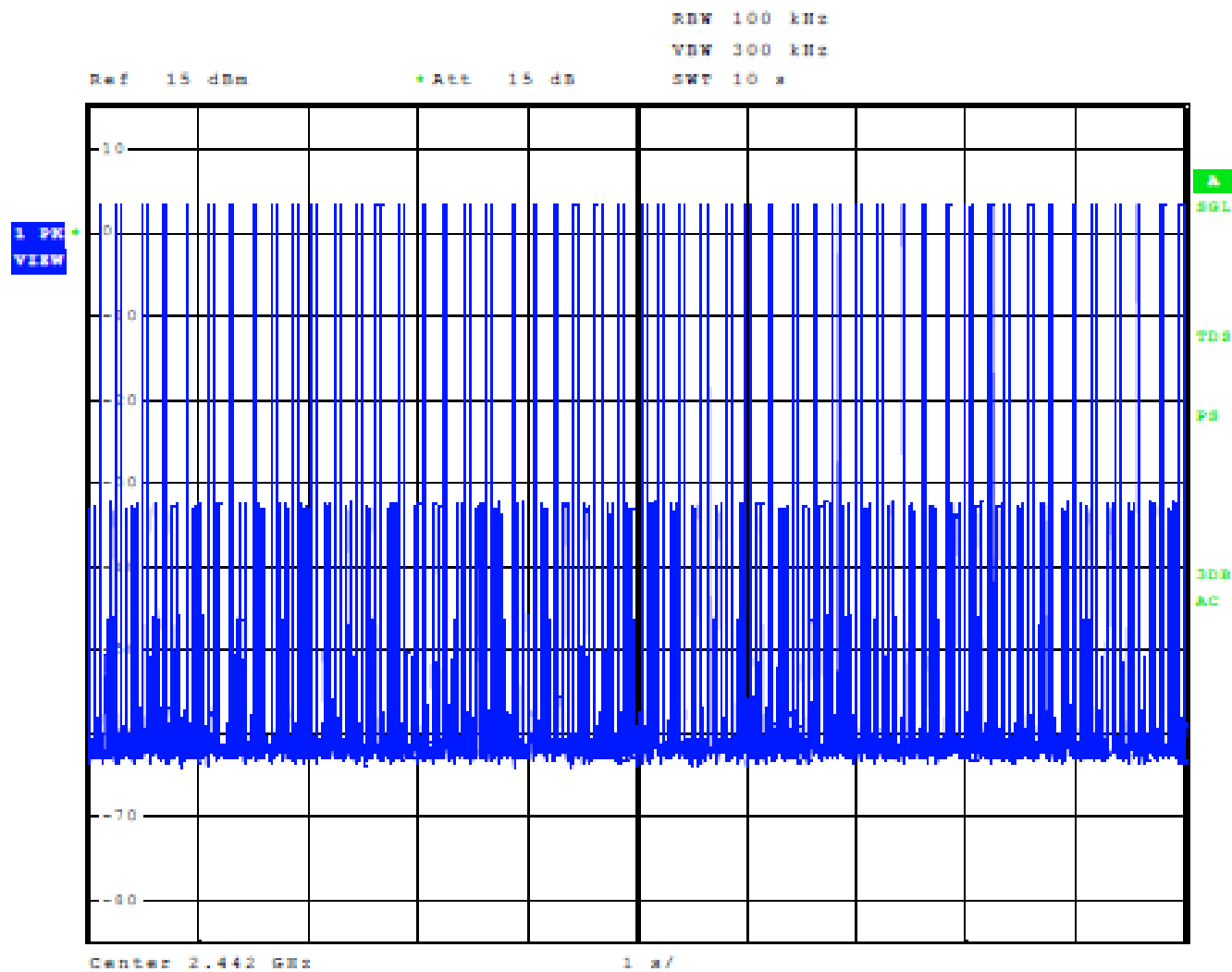
Figure 14 Plot of Number of Times on Channel over 10 Second Period Mode 1 BT BR (GFSK)
