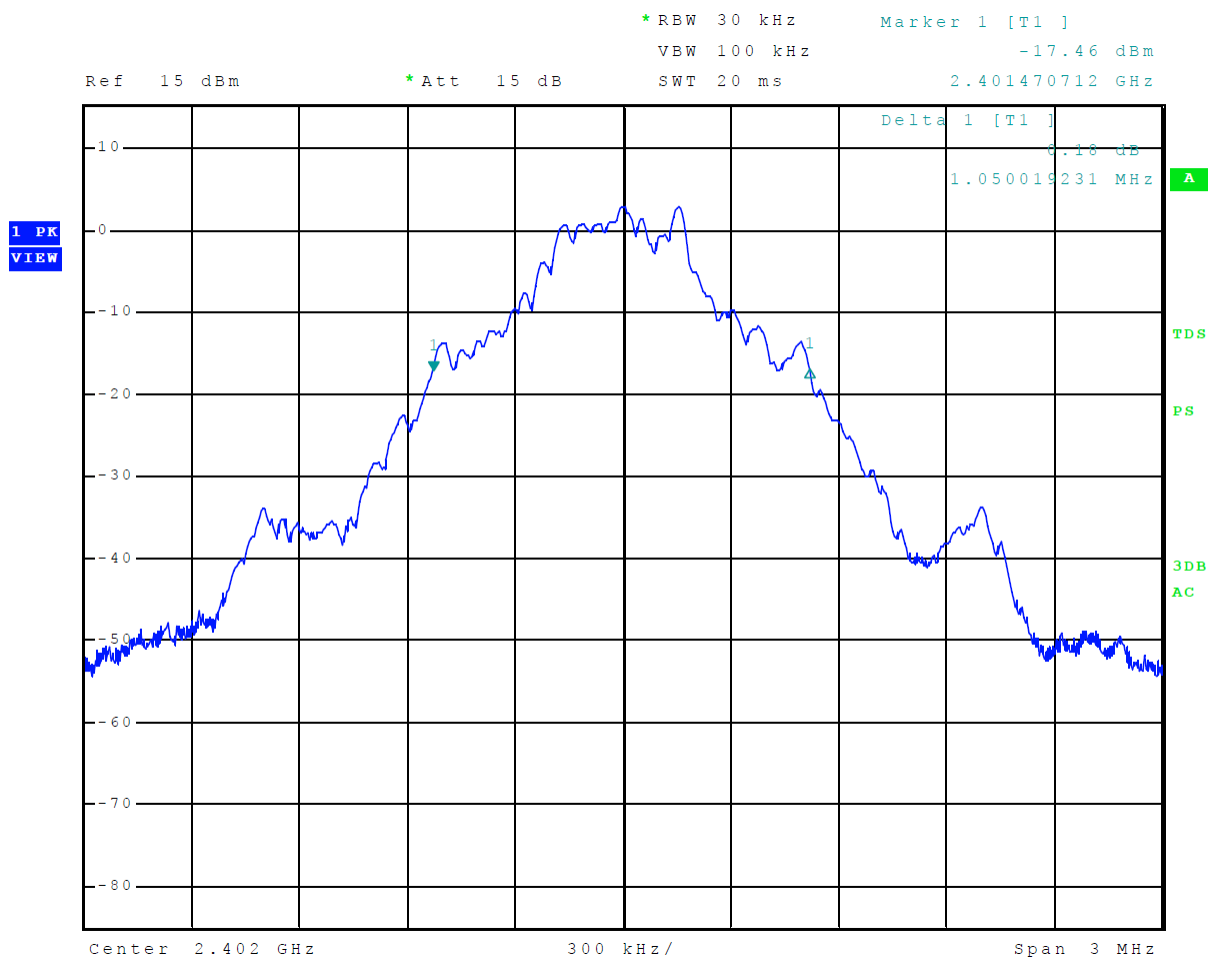
Figure 6 Plot of Transmitter Emissions 20-dB Occupied Bandwidth Mode 1, BT BR
