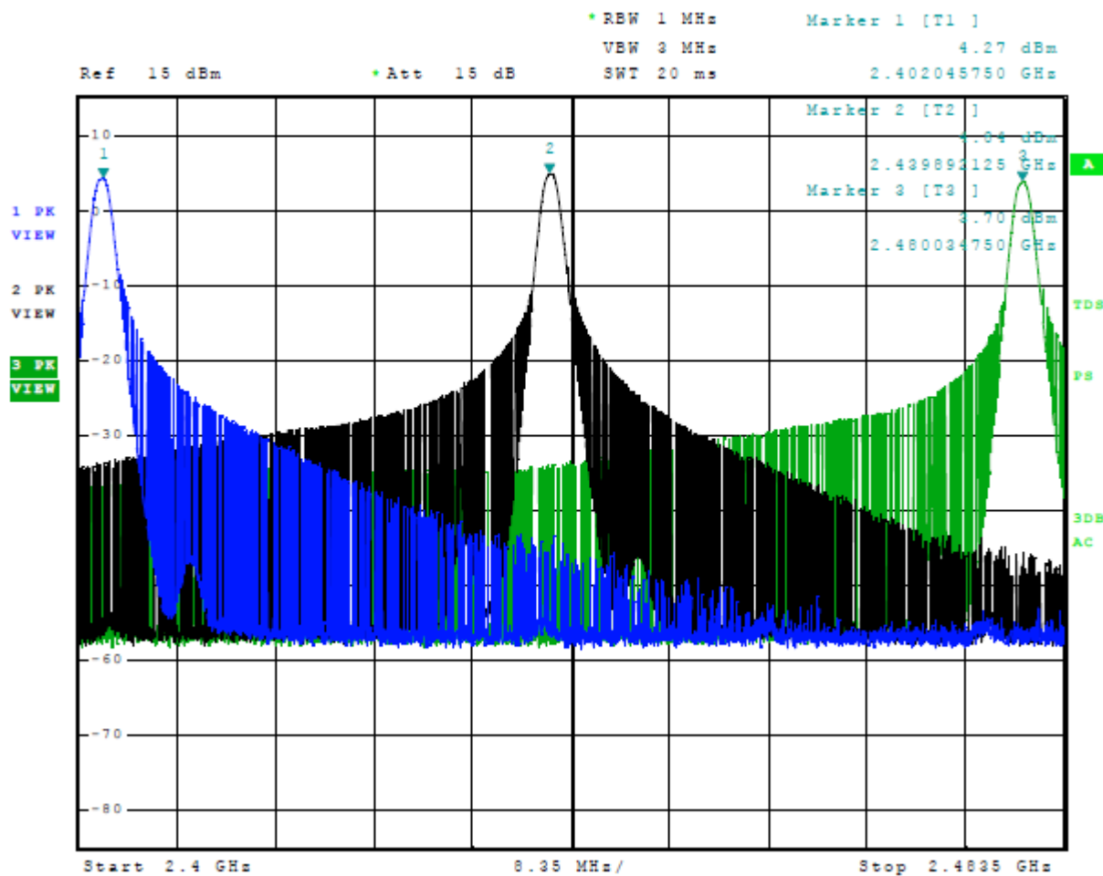
Figure 5 Plot of Transmitter Emissions Operation in 2402-2480 MHz Mode 1, BT BR
