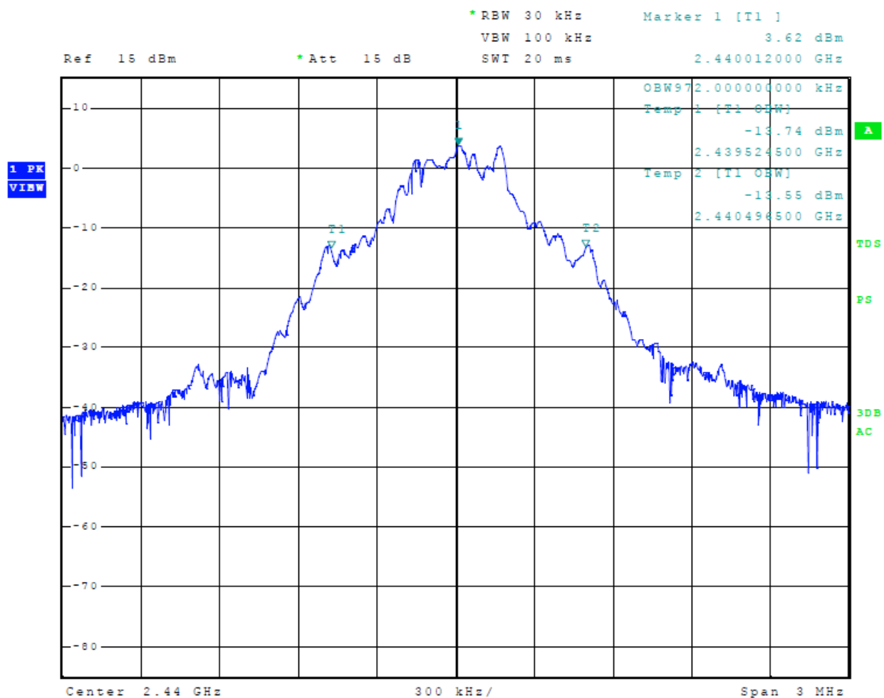
Figure 7 Plot of Transmitter Emissions 99% Occupied Bandwidth Mode 1, BT BR
