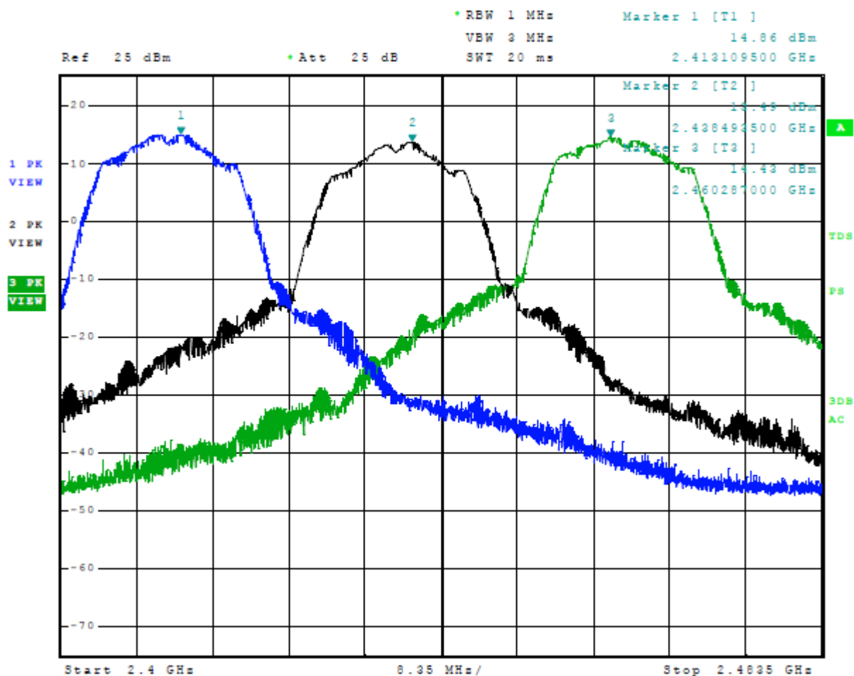
Figure 9 Plot of Transmitter Operation in 2402-2480 MHz Mode 6, 802.11g
