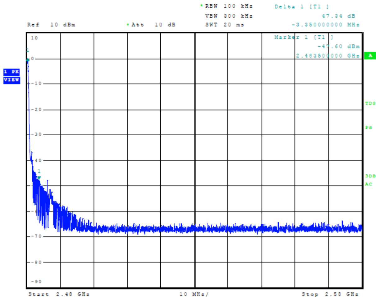
Figure 18 Plot of Transmitter Emissions High Band Edge Mode 3, BT (3EDR 8DPSK)
