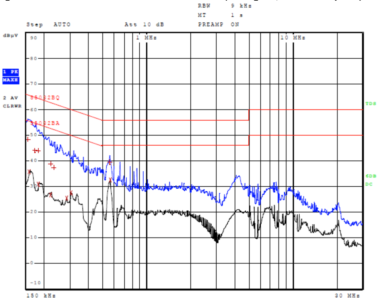
Figure 1 AC Line Conducted Emissions Data L1 (Config. #4, EUT – Computer)
