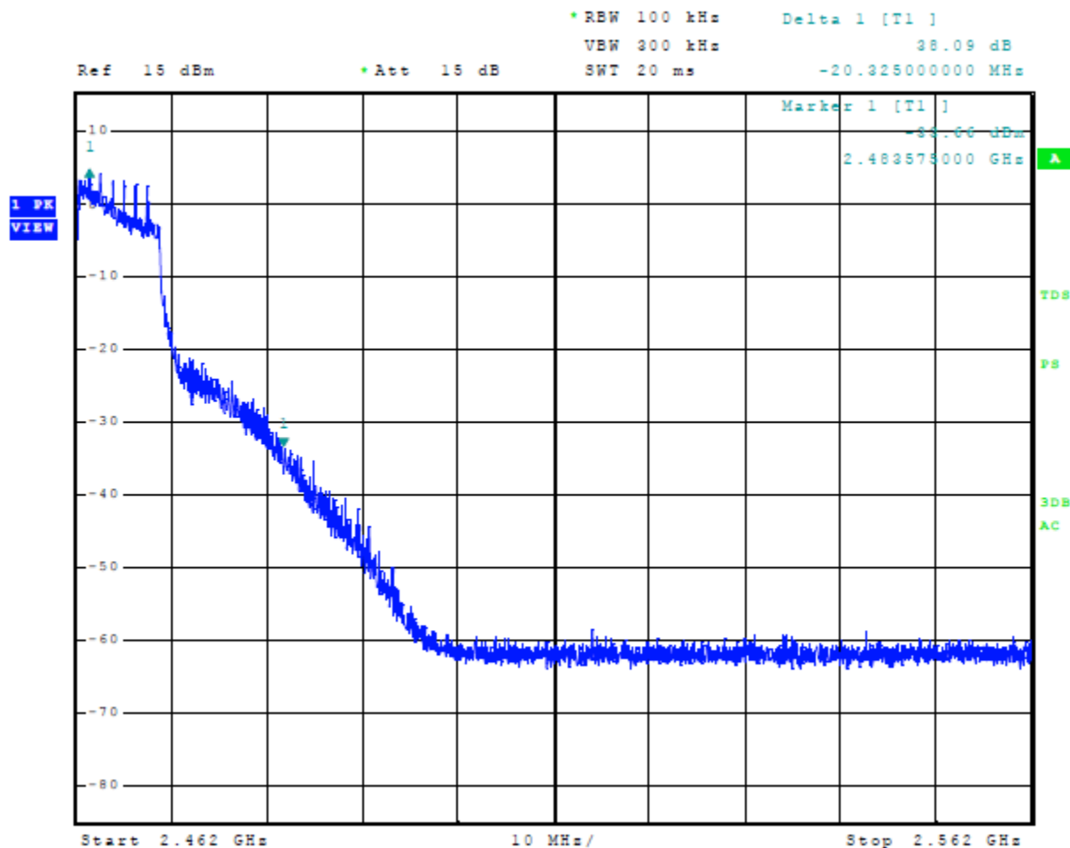
Figure 22 Plot of Transmitter Emissions High Band Edge Mode 7, 802.11n
