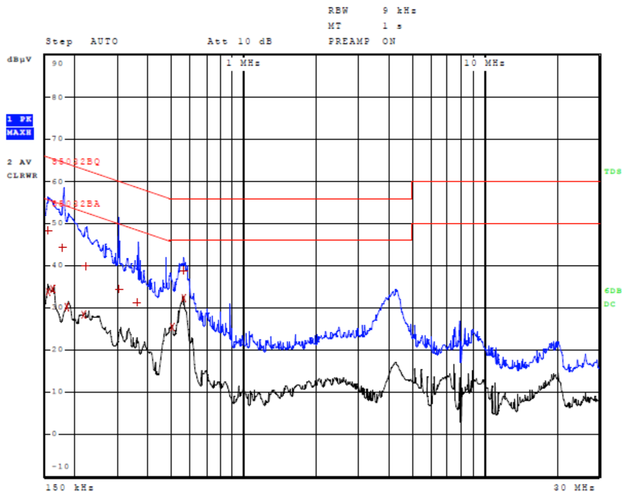
Figure 2 AC Line Conducted Emissions Data L2 (Config. #4, EUT – Computer)
