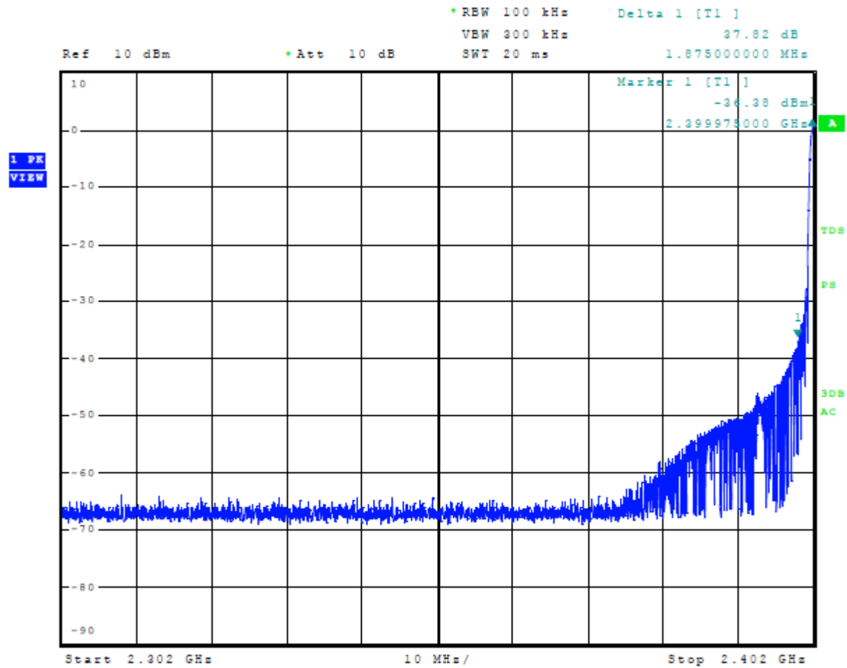
Figure 12 Plot of Emissions Low Band Edge Mode 3, BT (3EDR 8DPSK)
