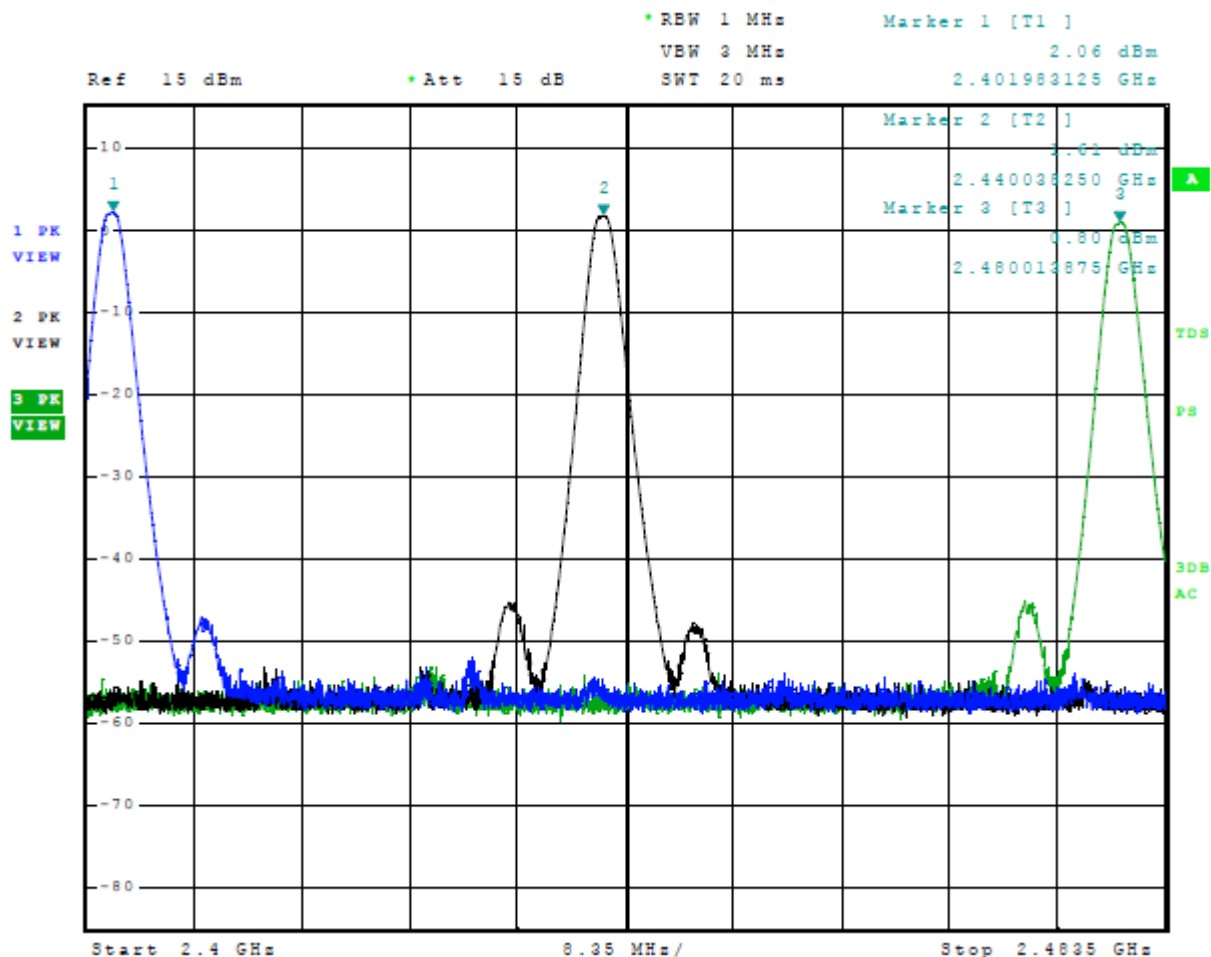
Figure 7 Plot of Transmitter Operation in 2402-2480 MHz Mode 4, BT BLE (GMSK)
