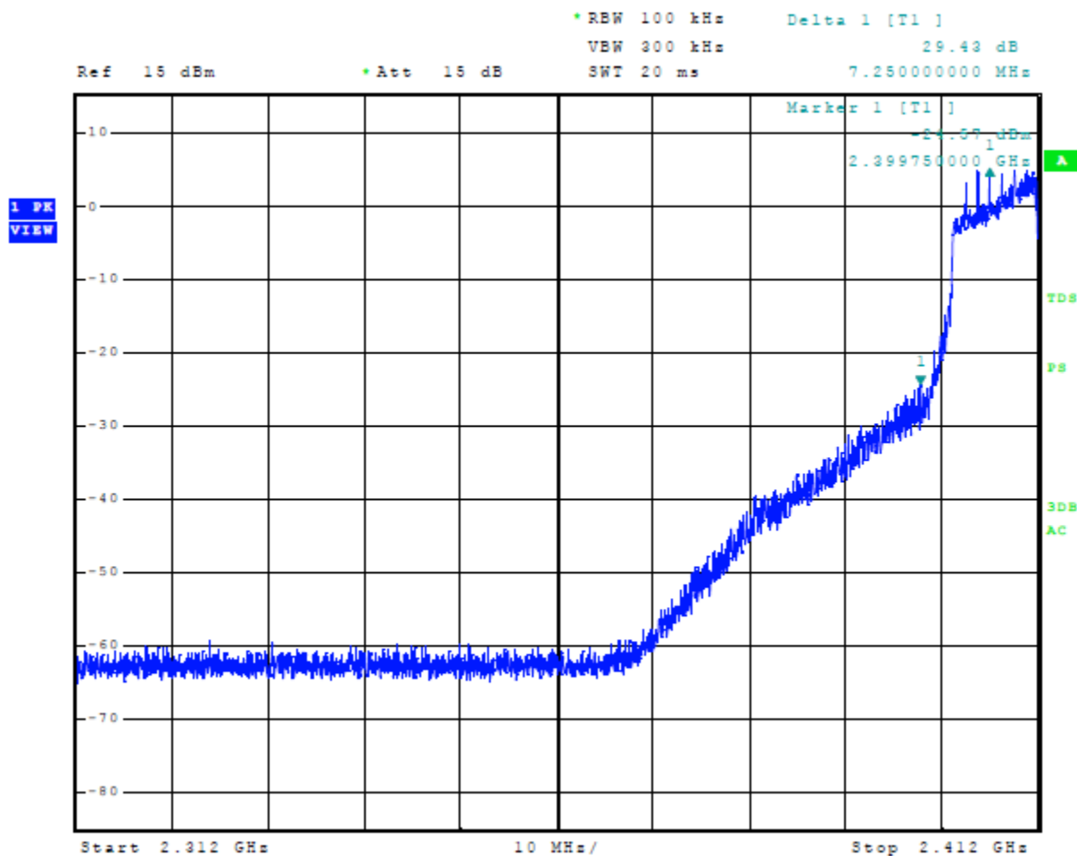
Figure 16 Plot of Emissions Low Band Edge Mode 7, 802.11n
