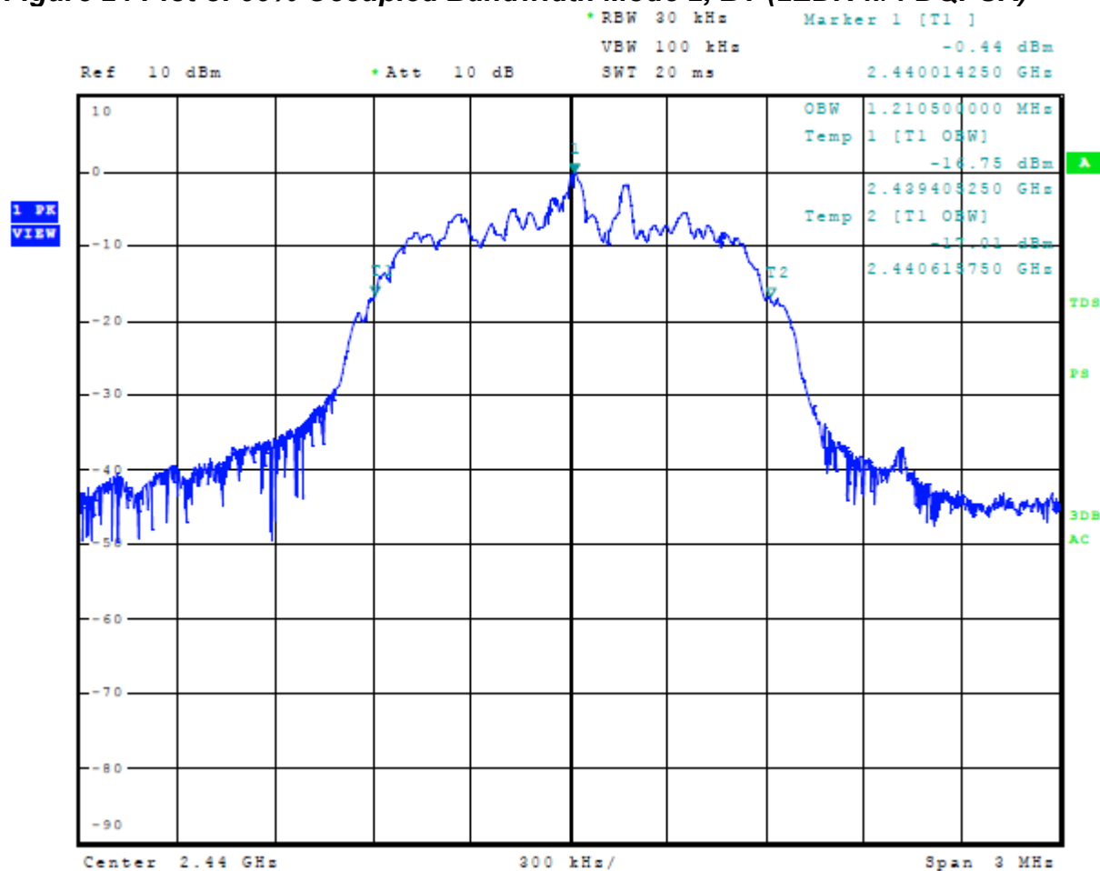
Figure 24 Plot of 99% Occupied Bandwidth Mode 2, BT (2EDR \pi/4 DQPSK)
