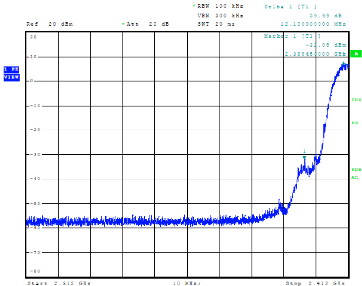
Figure 14 Plot of Emissions Low Band Edge Mode 5, 802.11b
