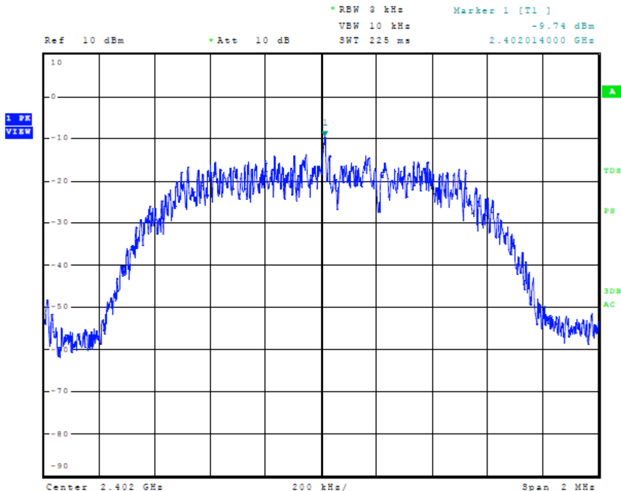
Figure 36 Plot of Transmitter Power Spectral Density Mode 3, BT (3EDR 8DPSK)
