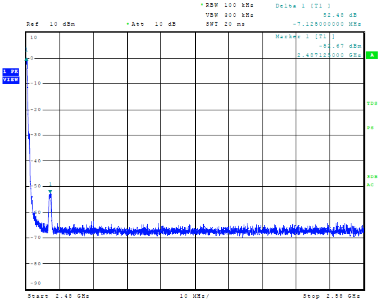
Figure 19 Plot of Transmitter Emissions High Band Edge Mode 4, BT BLE (GMSK)
