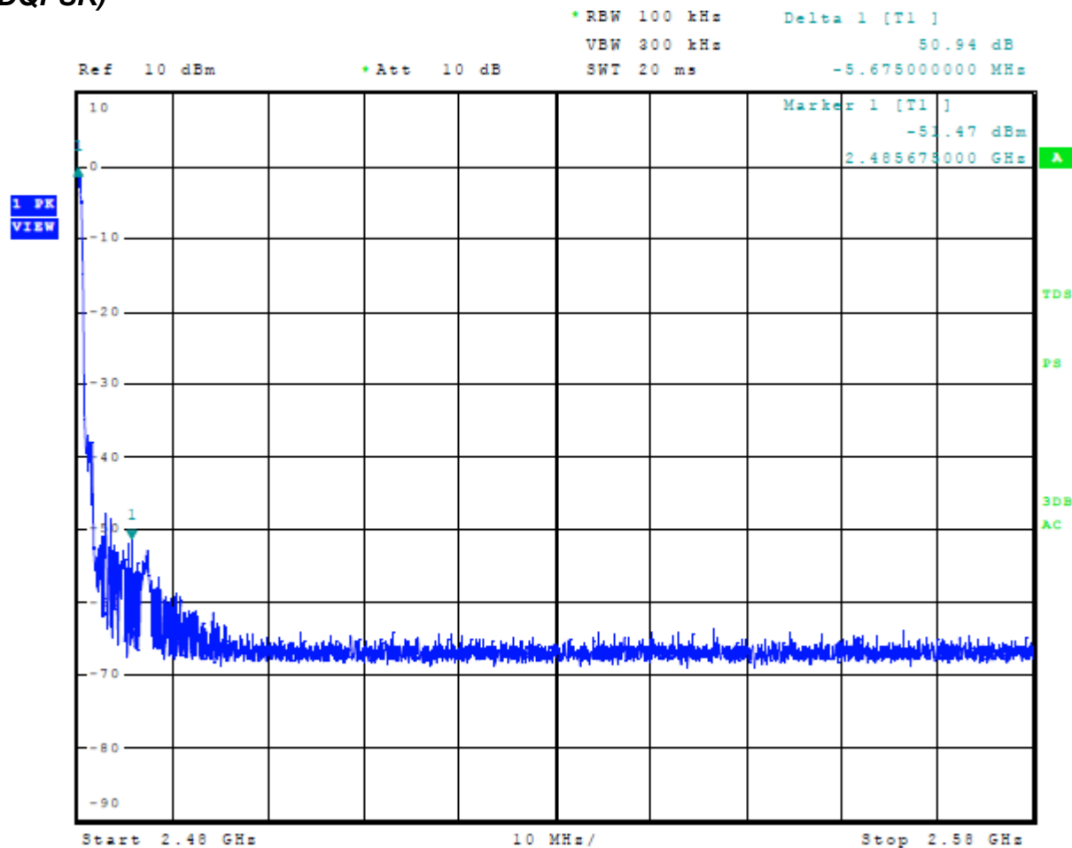
Figure 17 Plot of Transmitter Emissions High Band Edge Mode 2, BT (2EDR \pi/4 DQPSK)
