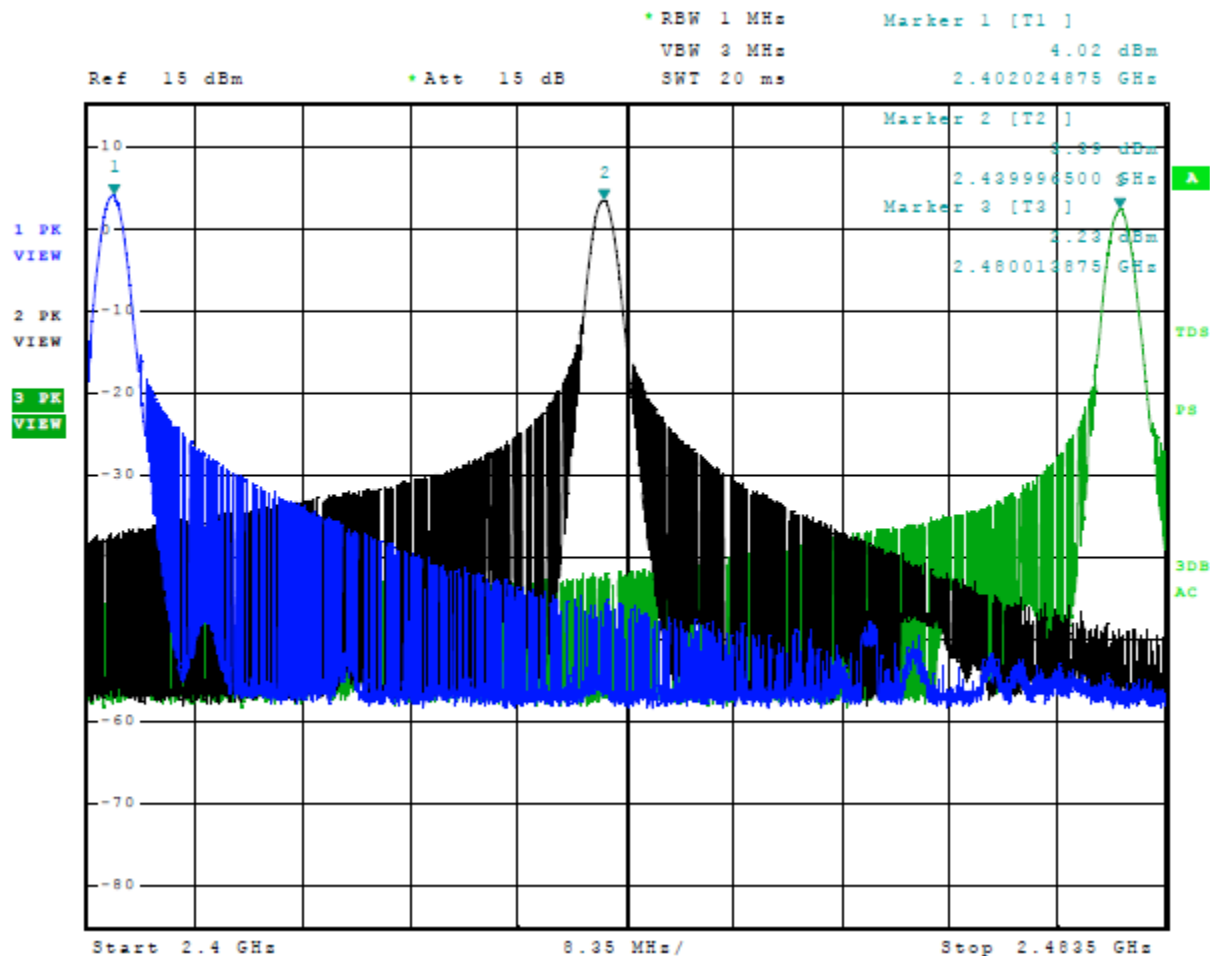
Figure 6 Plot of Transmitter Operation in 2402-2480 MHz Mode 3, BT (3EDR 8DPSK)
