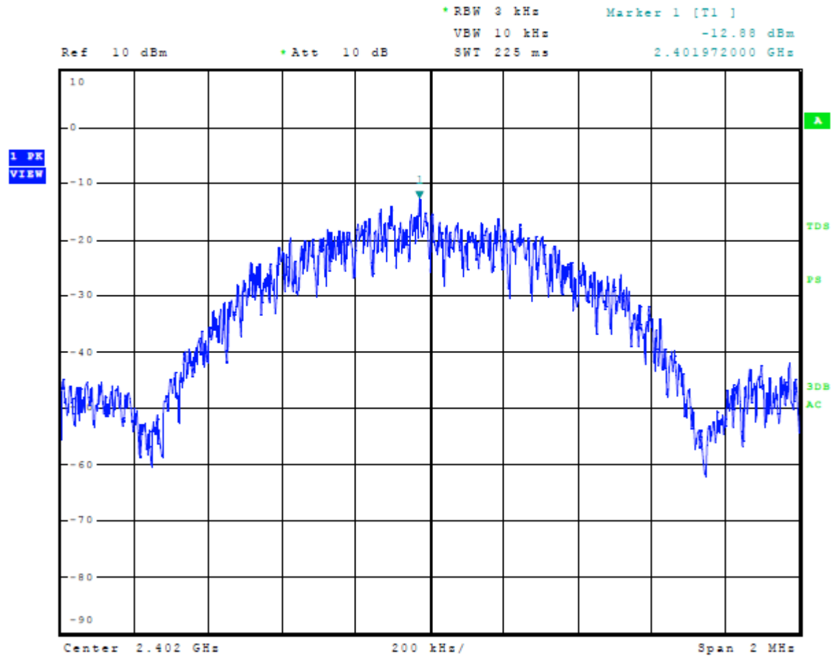
Figure 37 Plot of Transmitter Power Spectral Density Mode 4, BT BLE (GMSK)
