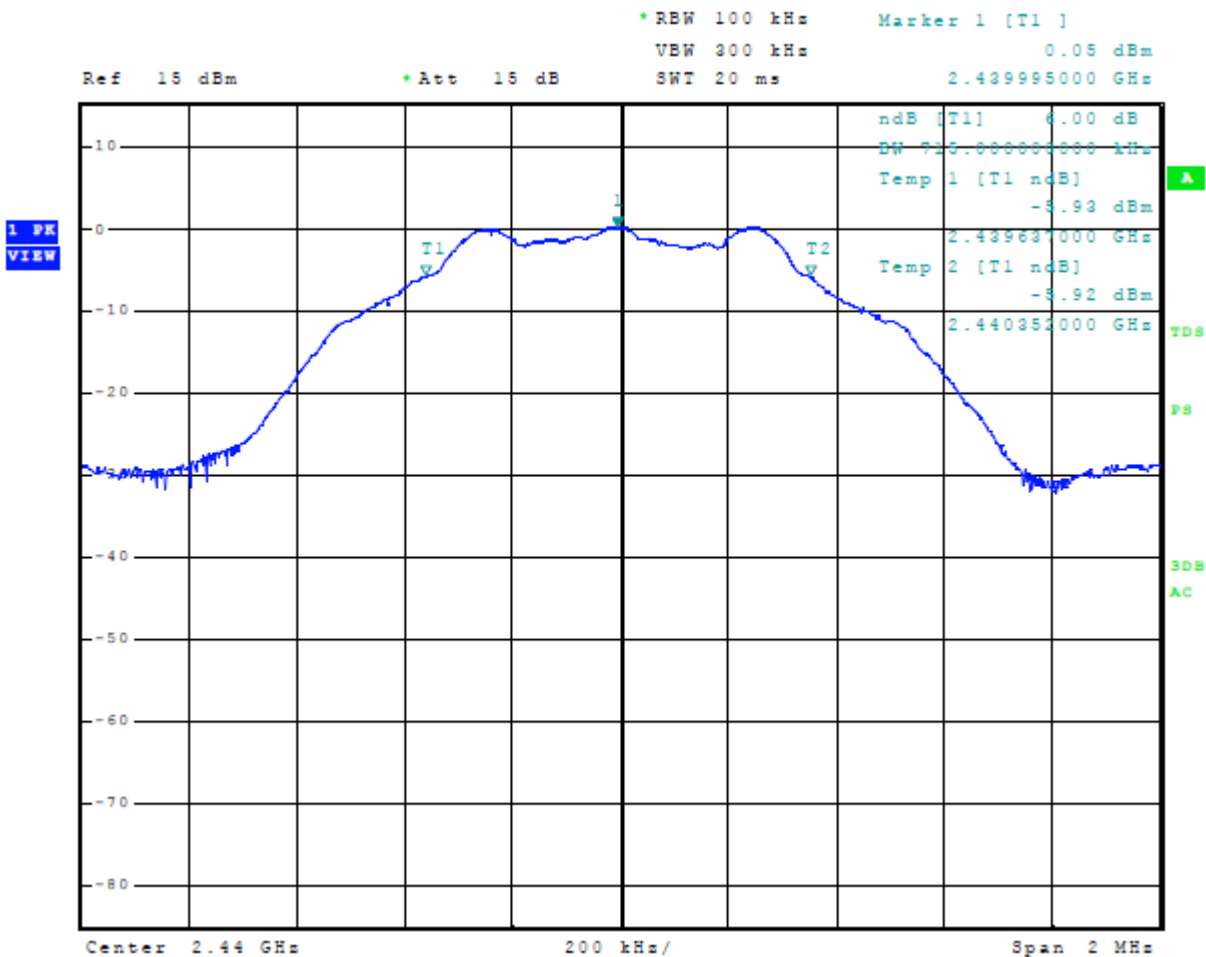
Figure 27 Plot of 6-dB Occupied Bandwidth Mode 4, BT BLE (GMSK)
