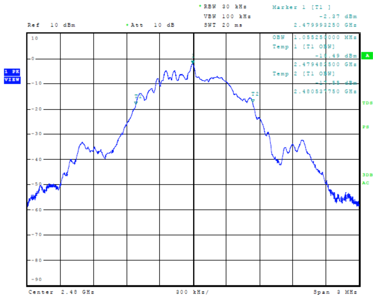
Figure 28 Plot of 99% Occupied Bandwidth Mode 4, BT BLE (GMSK)
