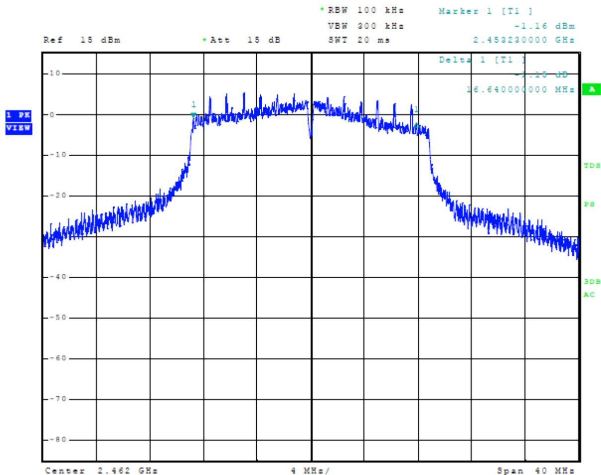
Figure 33 Plot of 6-dB Occupied Bandwidth Mode 7, 802.11n
