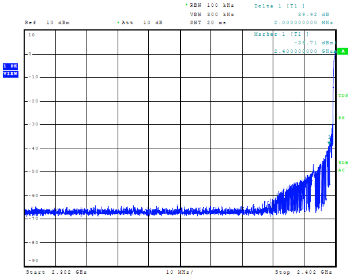
Figure 11 Plot of Emissions Low Band Edge Mode 2, BT (2EDR \pi/4 DQPSK)
