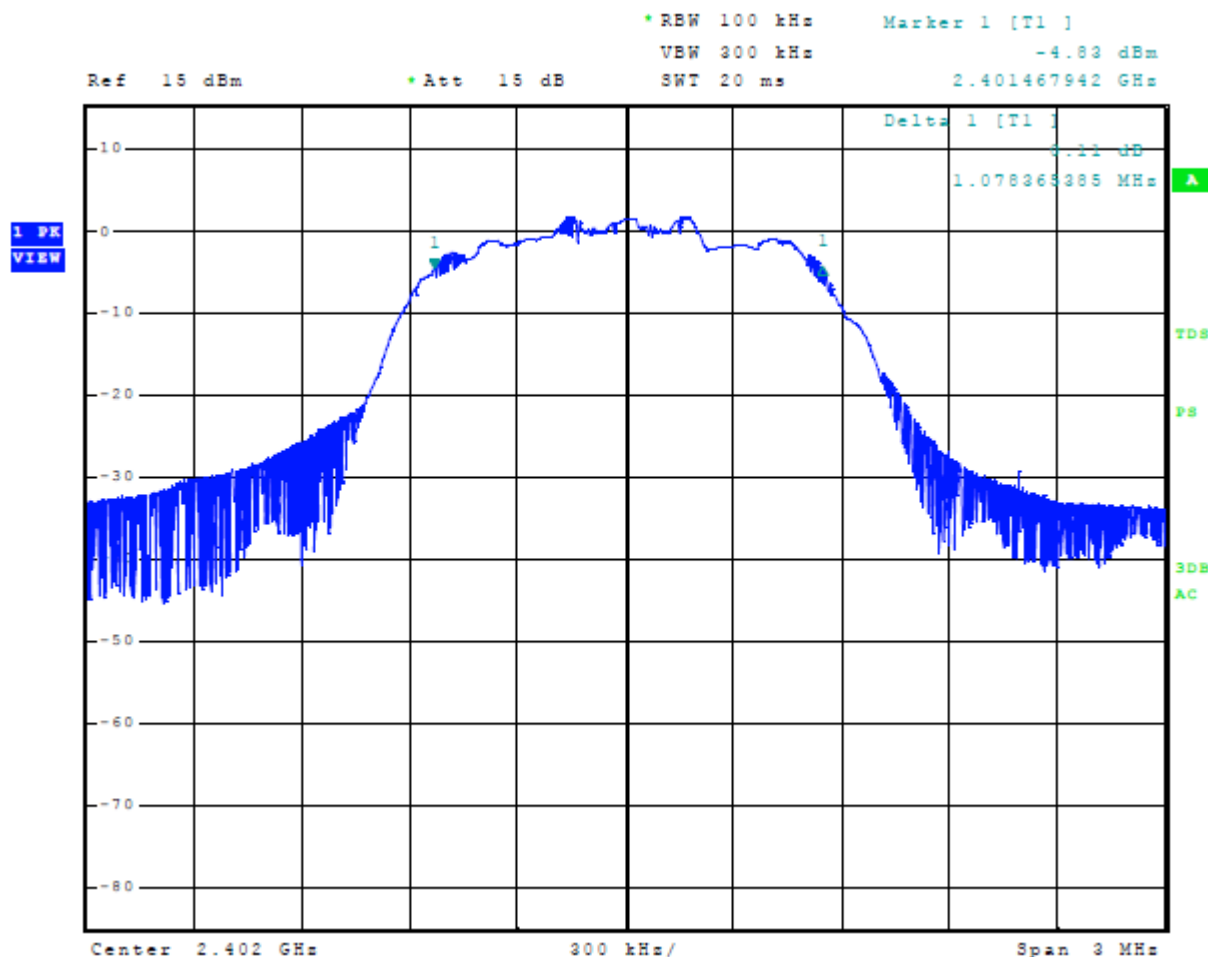
Figure 25 Plot of 6-dB Occupied Bandwidth Mode 3, BT (3EDR 8DPSK)
