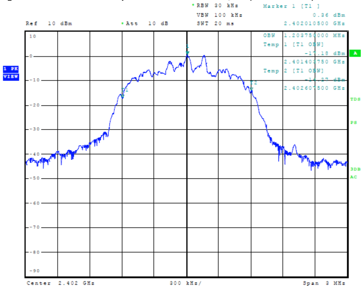
Figure 26 Plot of 99% Occupied Bandwidth Mode 3, BT (3EDR 8DPSK)
