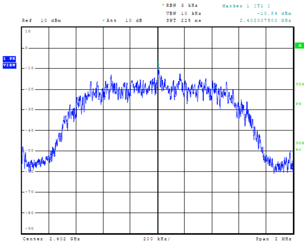
Figure 35 Plot of Transmitter Power Spectral Density Mode 2, BT (2EDR \pi/4 DQPSK)
