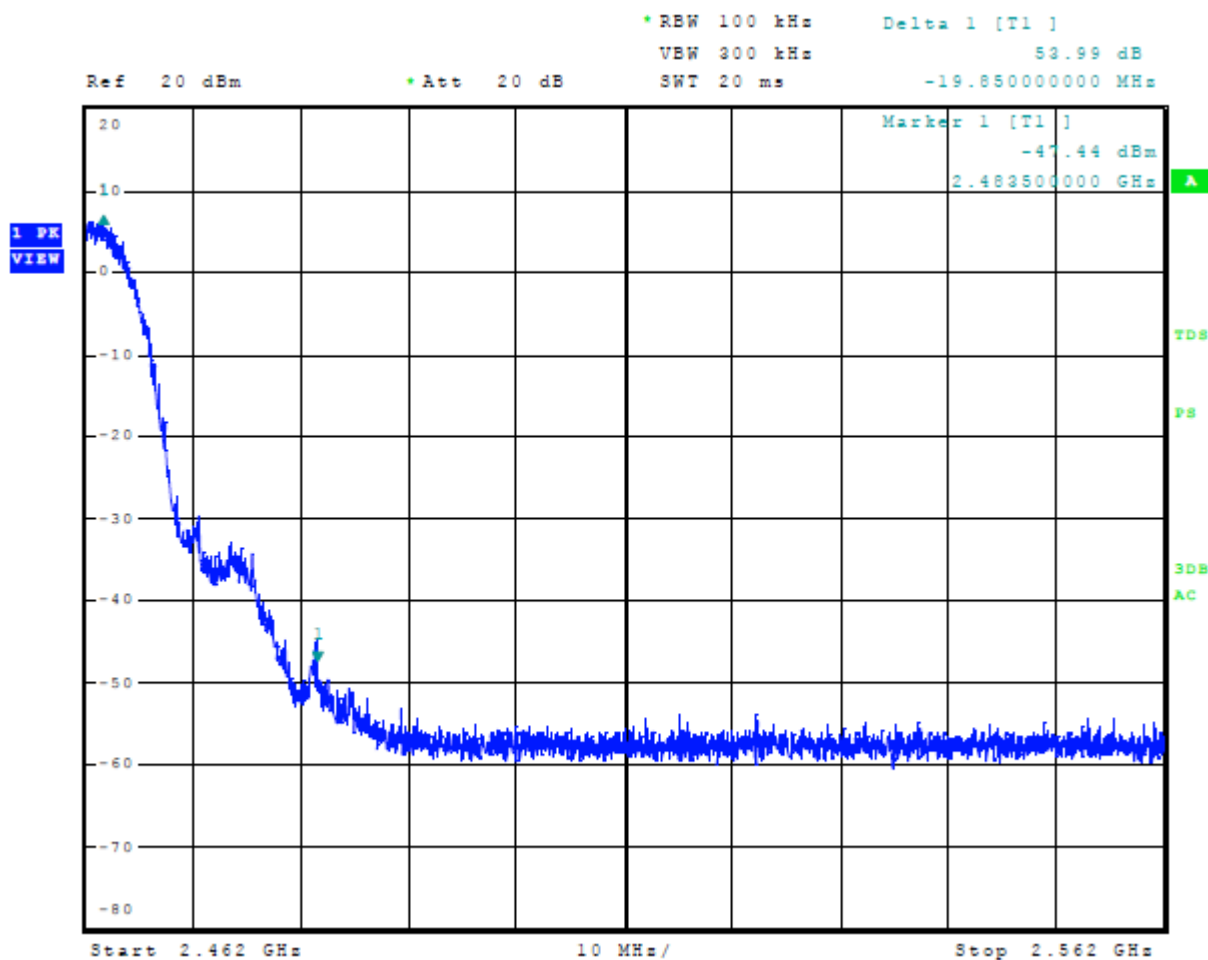
Figure 20 Plot of Transmitter Emissions High Band Edge Mode 5, 802.11b
