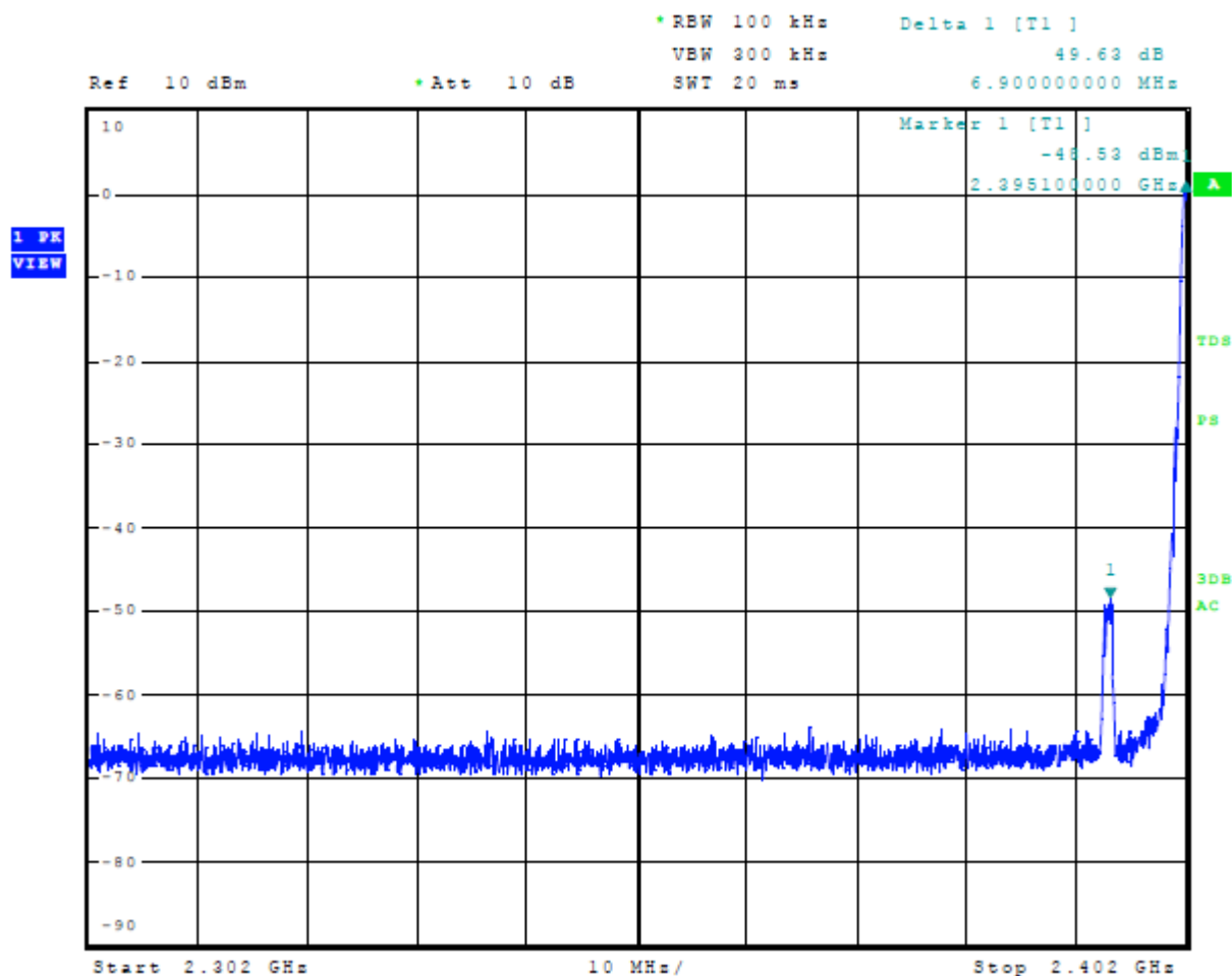
Figure 13 Plot of Emissions Low Band Edge Mode 4, BT BLE (GMSK)
