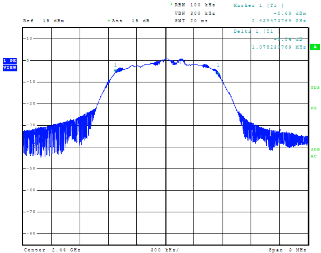
Figure 23 Plot of 6-dB Occupied Bandwidth Mode 2, BT (2EDR \pi/4 DQPSK)
