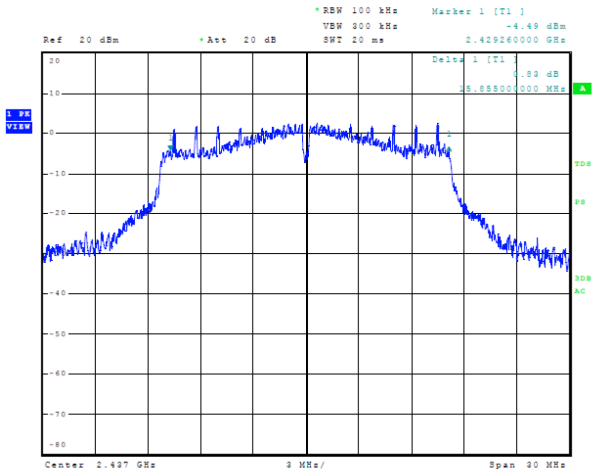
Figure 31 Plot of 6-dB Occupied Bandwidth Mode 6, 802.11g
