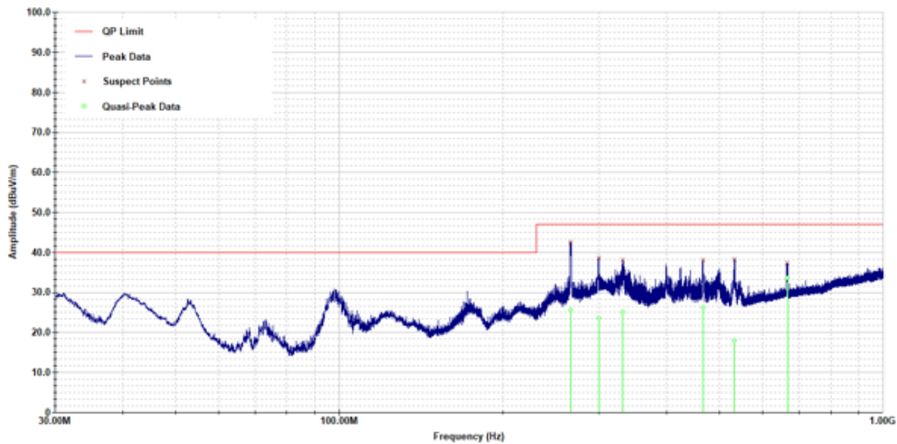
Figure 4 Plot of General Radiated Emissions – Vertical Polarization
