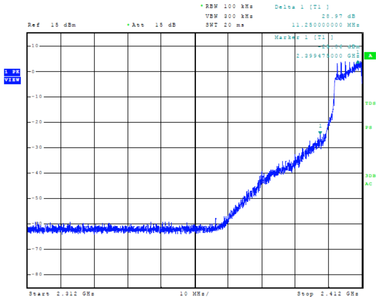
Figure 15 Plot of Emissions Low Band Edge Mode 6, 802.11g
