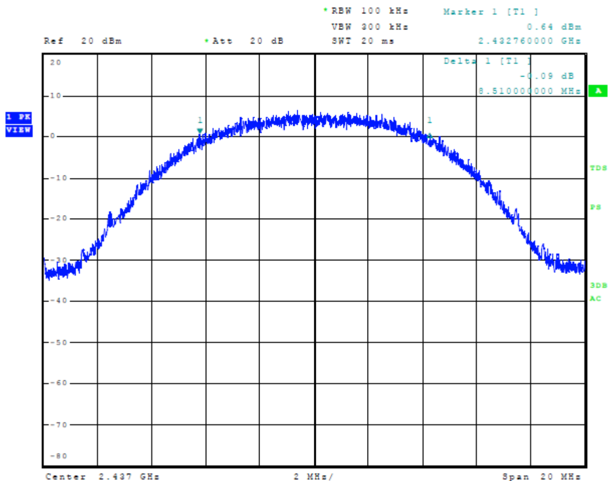
Figure 29 Plot of 6-dB Occupied Bandwidth Mode 5, 802.11b
