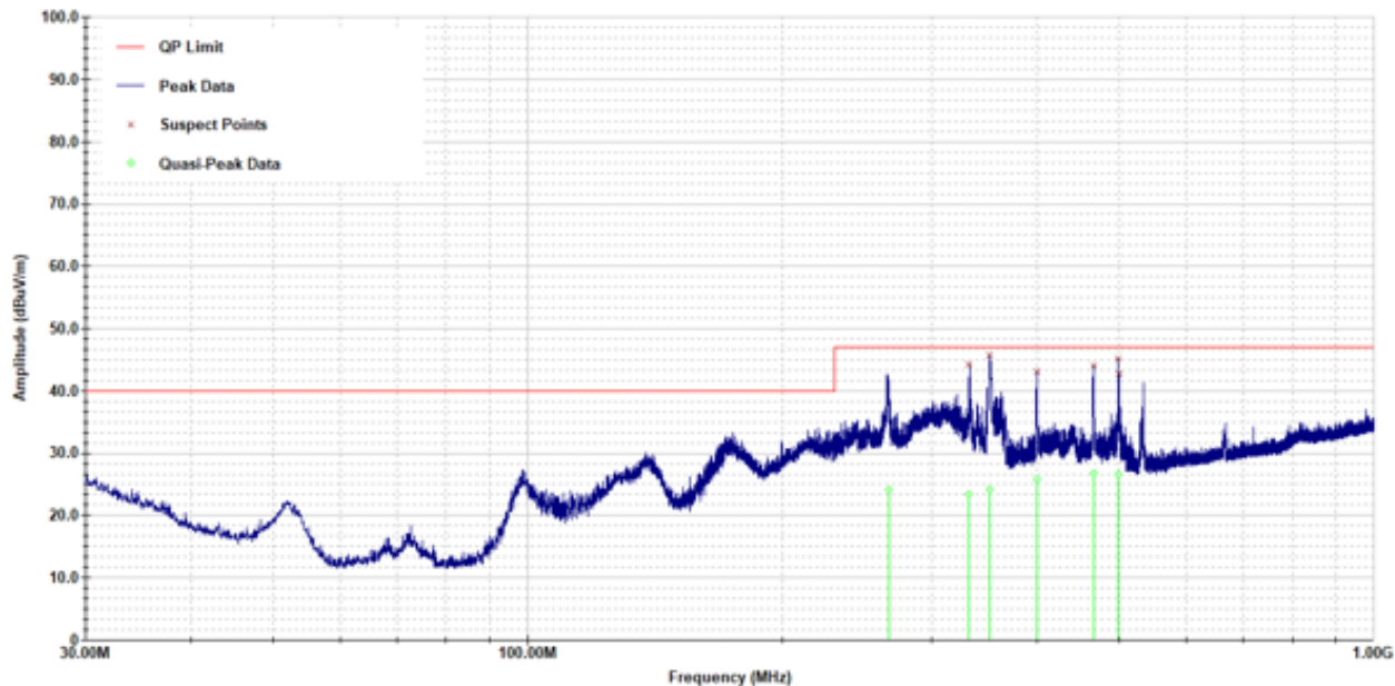
Figure 3 Plot of General Radiated Emissions – Horizontal Polarization
