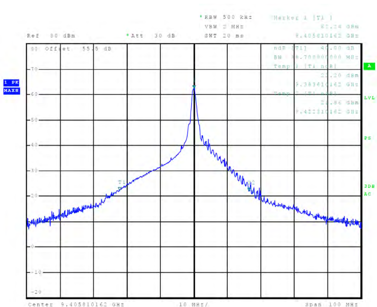
Figure 33 40-dB Occupied Bandwidth Plot, 12 nm
