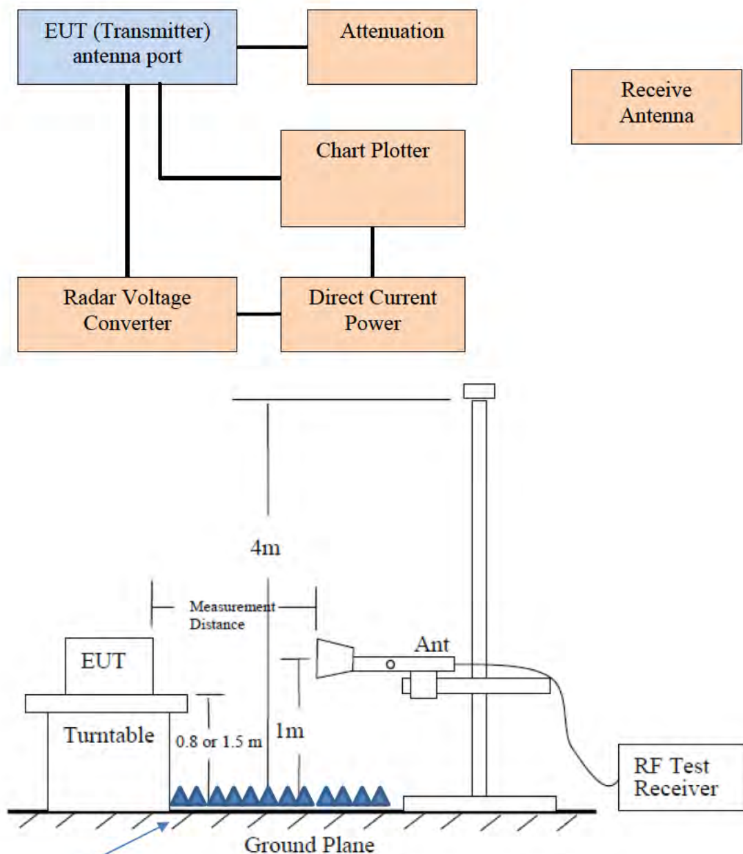
Figure 4—Test set-up for radiated spurious measurements
