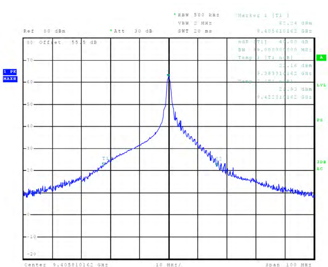
Figure 32 40-dB Occupied Bandwidth Plot, 8 nm
