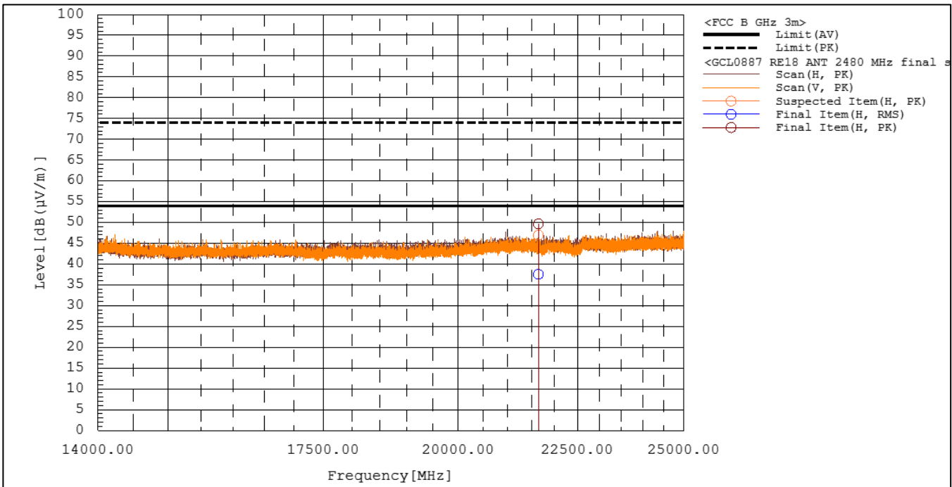
Figure RE18.1: Spectral data (ANT, 2480 MHz)
