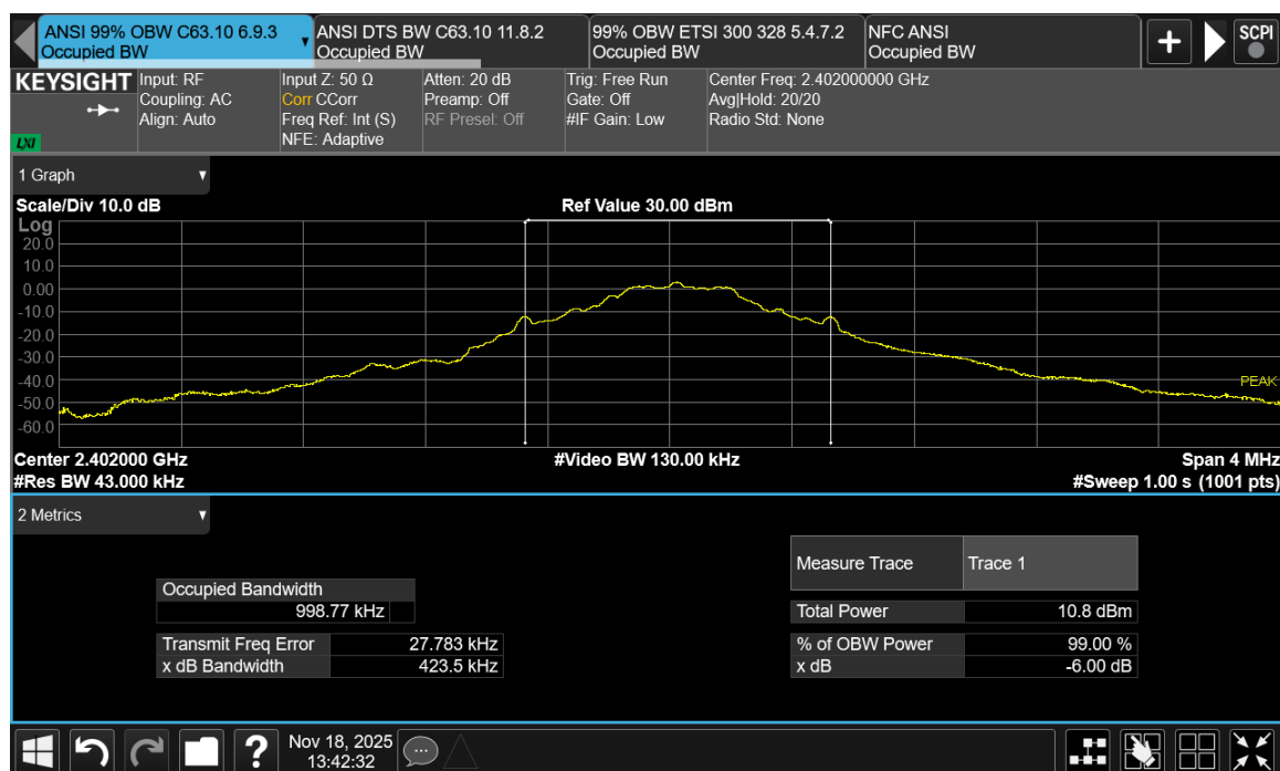
Figure TR16.2: Occupied bandwidth data for ANT at low channel (2402 MHz)
