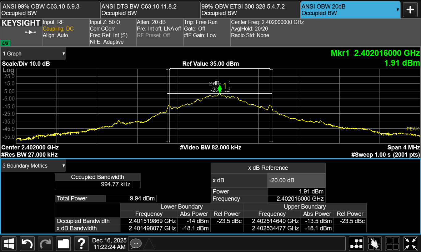
Figure TR89.2: 20dB occupied bandwidth data at 2402 MHz
