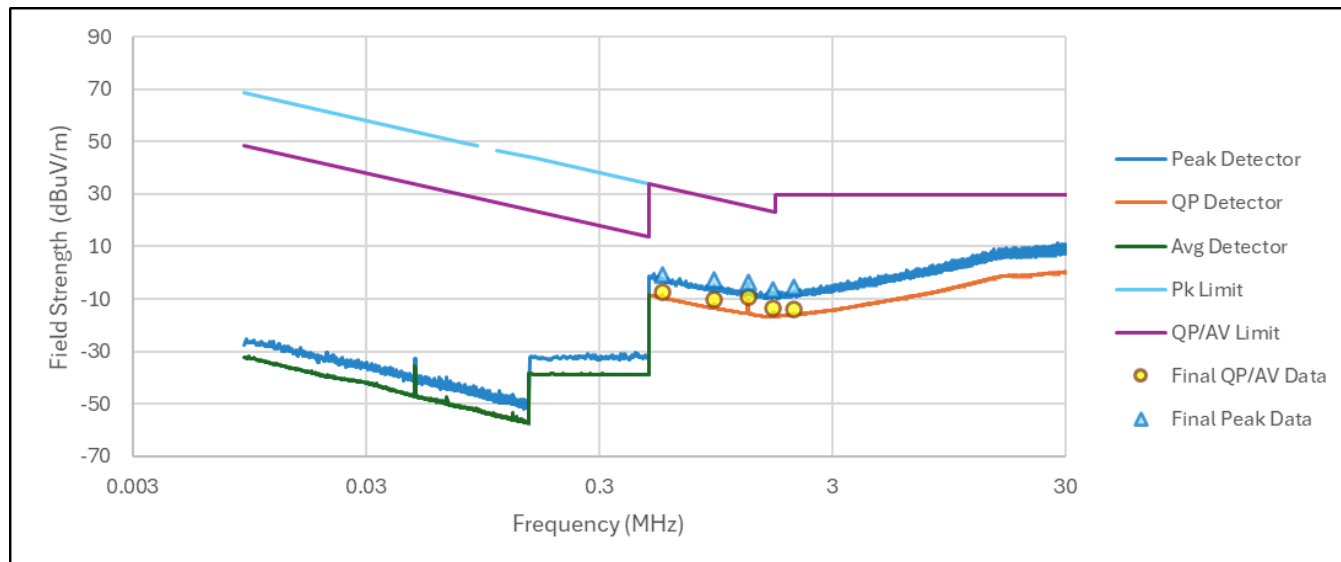
Figure RE21.1: Spectral data (ANT, 2480 MHz)
