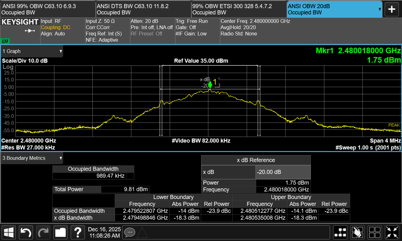
Figure TR89.2: 20dB occupied bandwidth data at 2480 MHz
