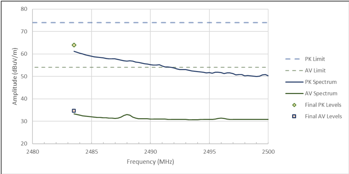
Figure RE04.2: FCC restricted band spectral data from 2483.5 to 2500 MHz (ANT, 2480 MHz)
