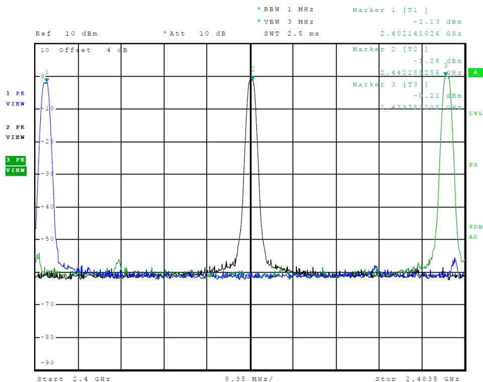
Figure 3 Plot of Transmitter Emissions Operation in 2402-2480 MHz
