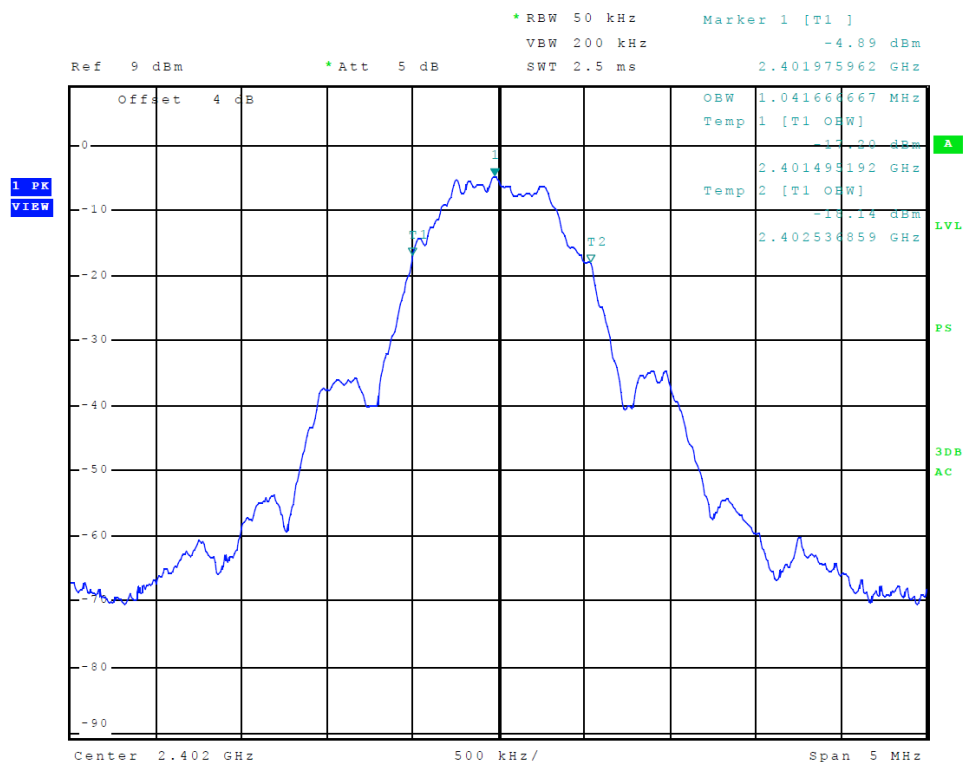
Figure 4 Plot of Transmitter Emissions 99% Occupied Bandwidth
