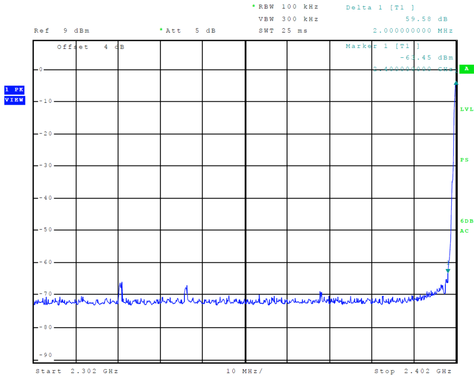
Figure 5 Plot of Transmitter Emissions Low Band Edge
