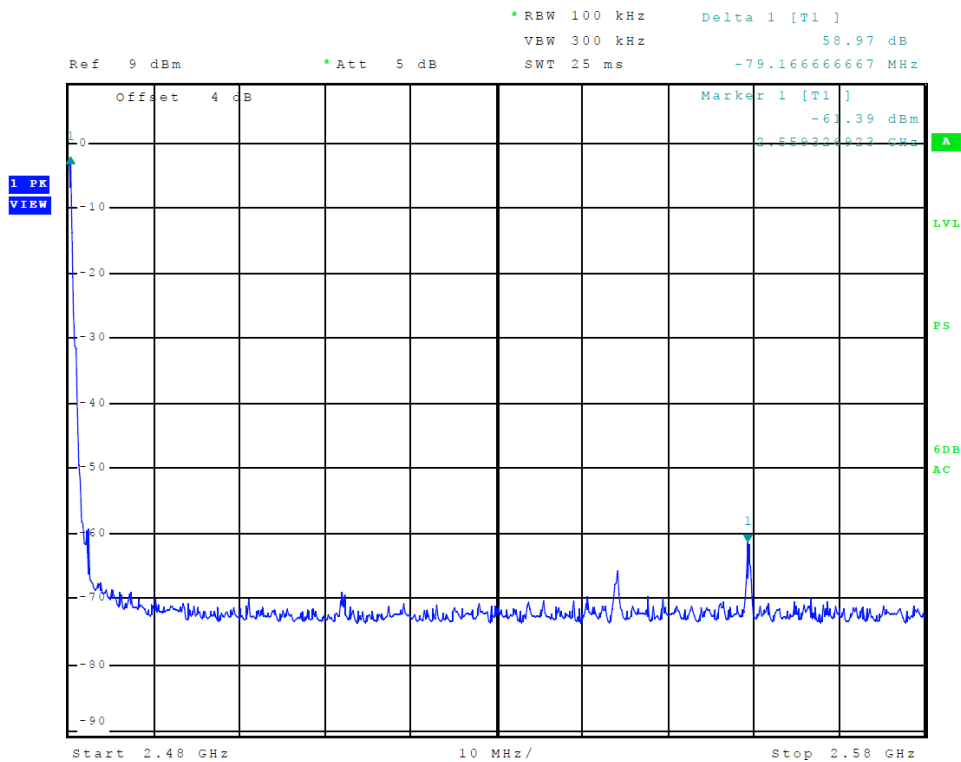
Figure 6 Plot of Transmitter Emissions High Band Edge
