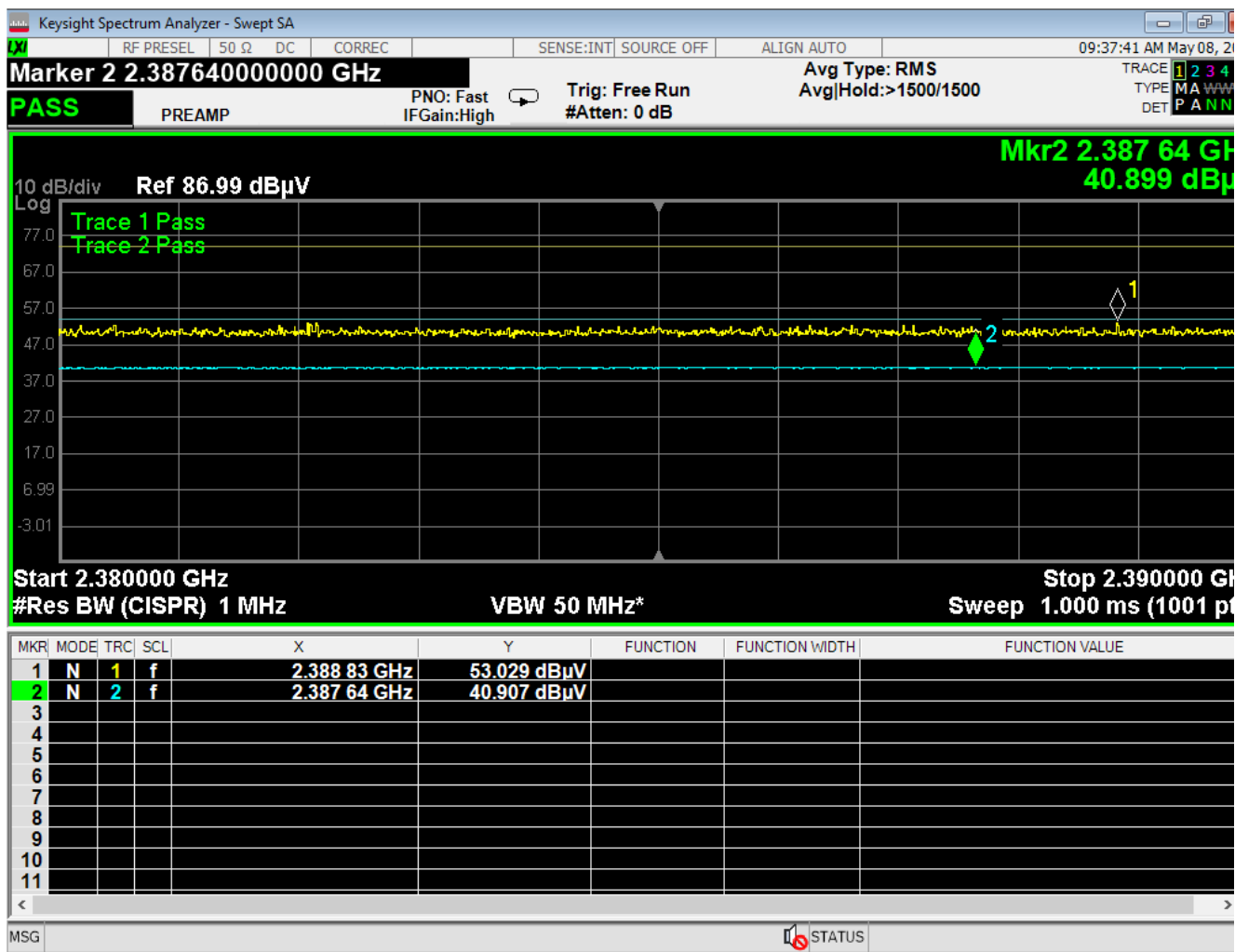
C03561 Peak Restricted Lower Band Edge BT BR
