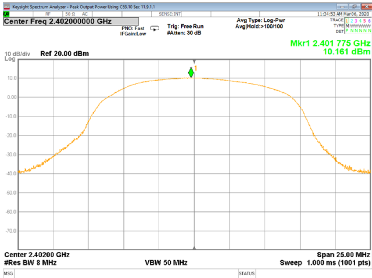
C03561 Peak Output Power Low Ch BT EDR 2MB
