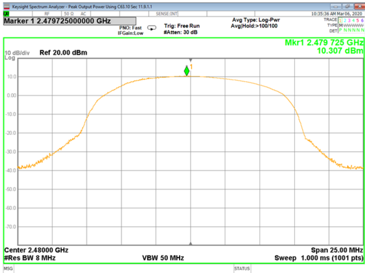
C03561 Peak Output Power High Ch BT EDR 2MB
