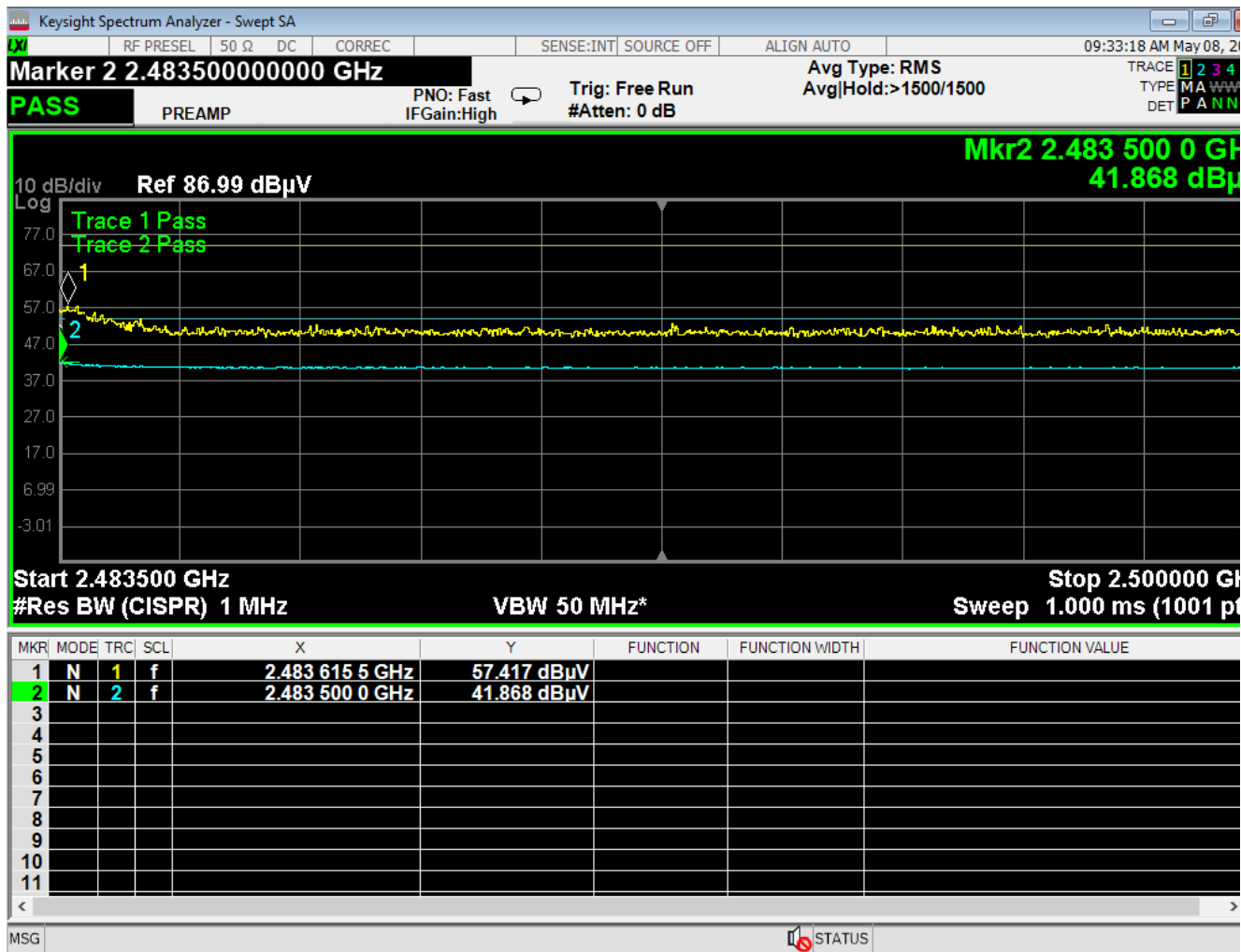
C03561 Peak Restricted Higher Band Edge BT EDR 2MB
