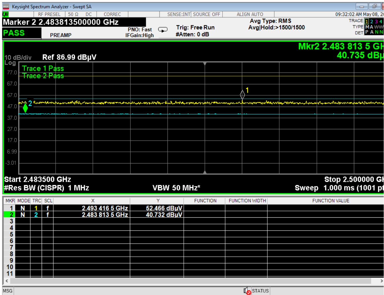
C03561 Peak Restricted Higher Band Edge BT BR
