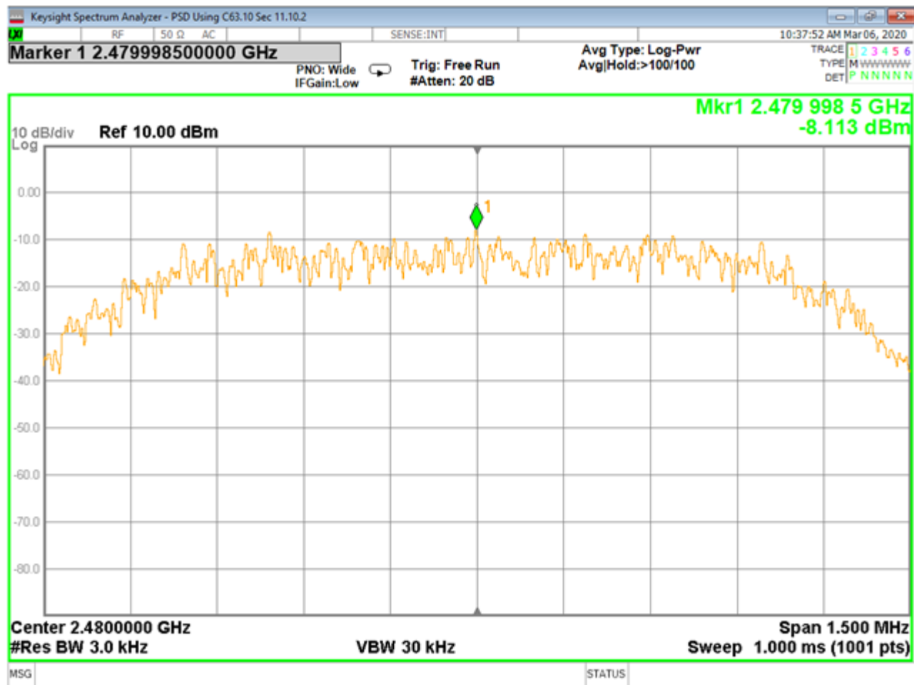
C03561 Peak PSD High Ch BT EDR 2MB
