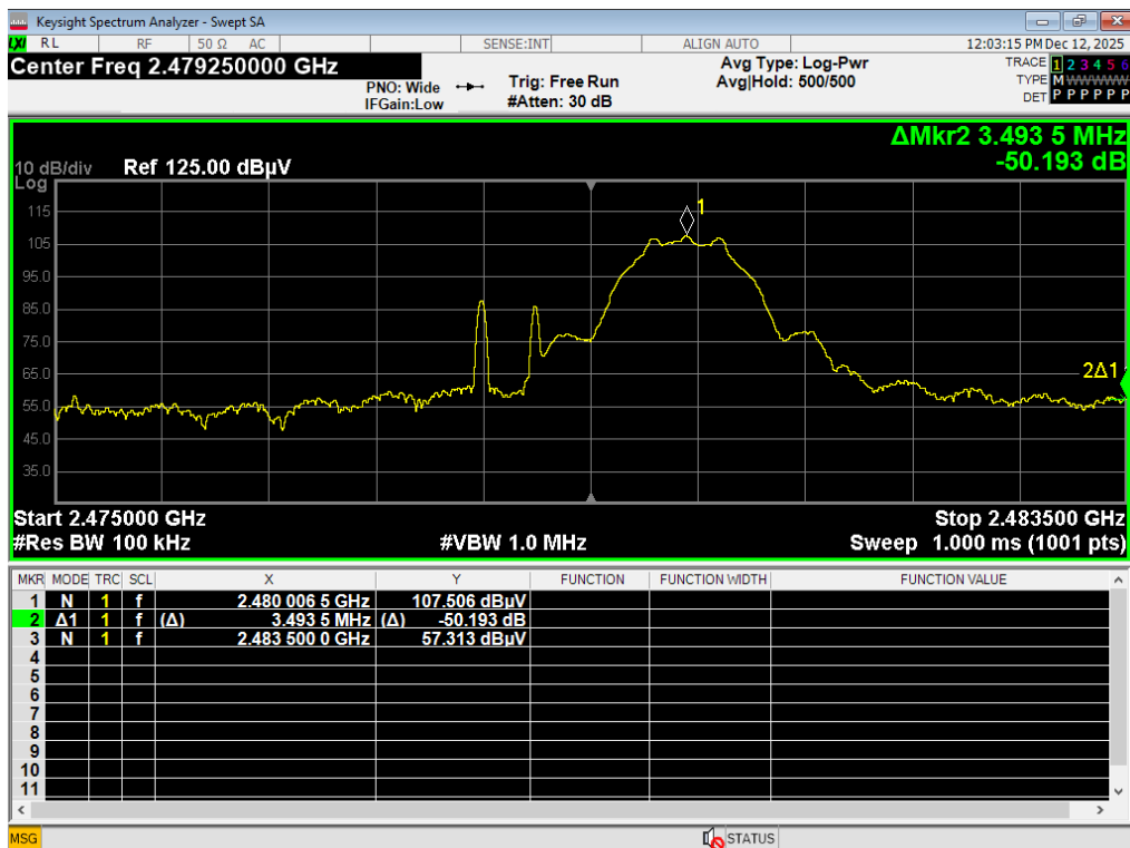
05 HBE Unrestricted, BLE 1MB, 2480MHz, 4dBm
