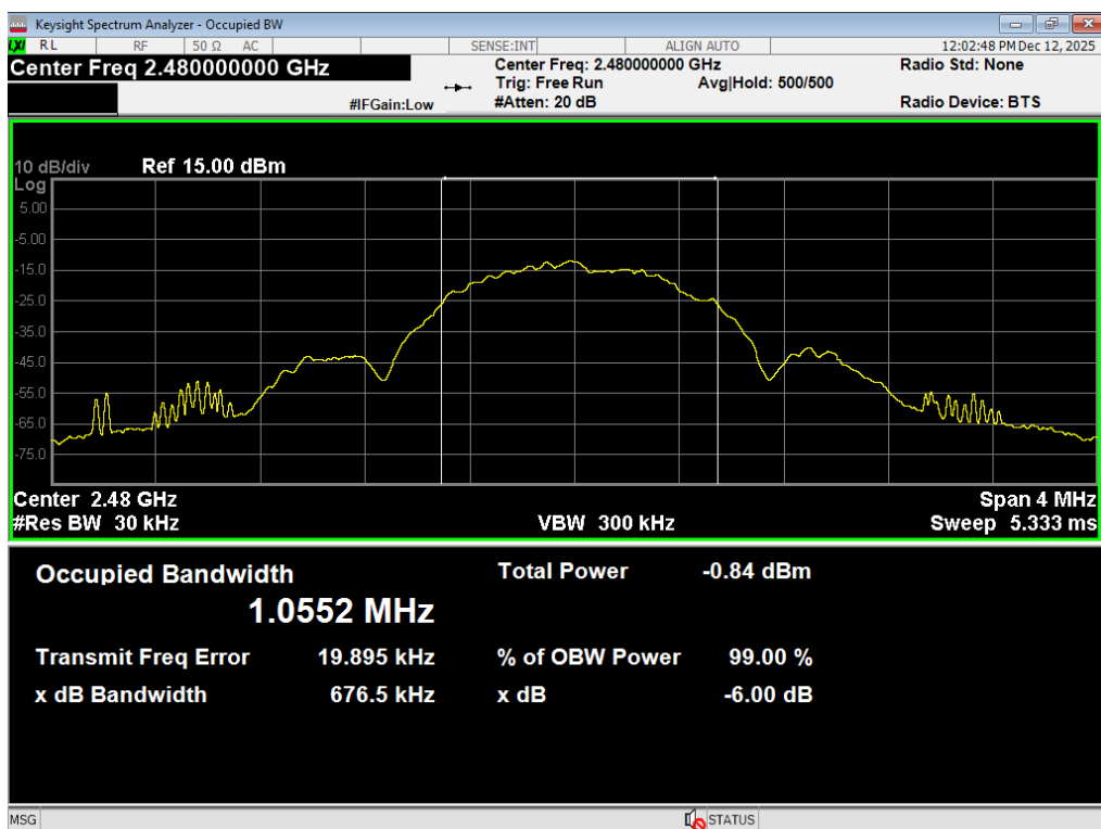
10 Occupied BW, BLE 1MB, 2480MHz, 4dBm
