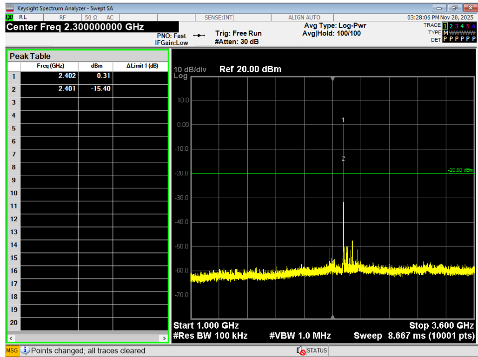
Figure 11 - Conducted Spurious Plot, 1GHz – 3.6GHz, GMSK Low
