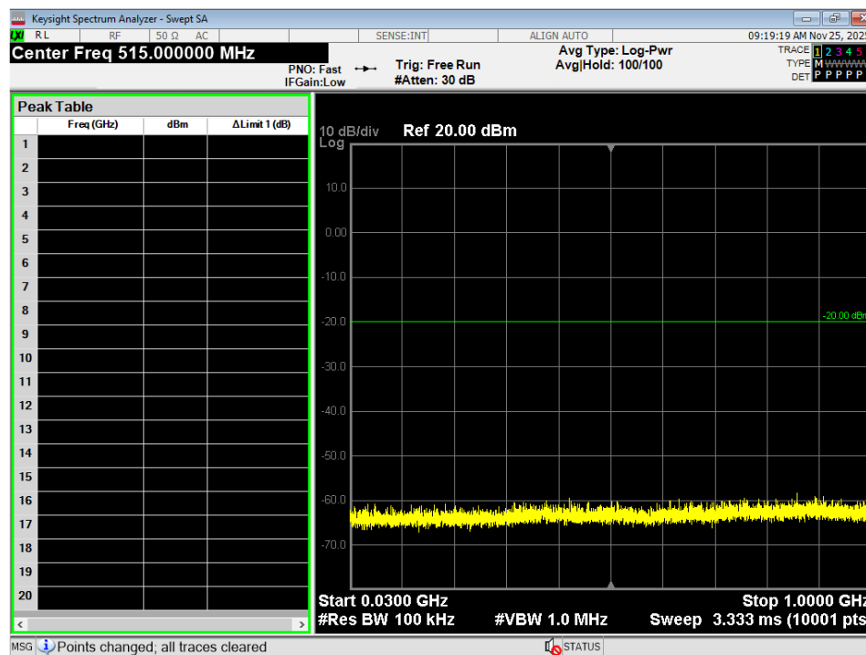
Figure 7 - Conducted Spurious Plot, 30MHz – 1GHz, RX
