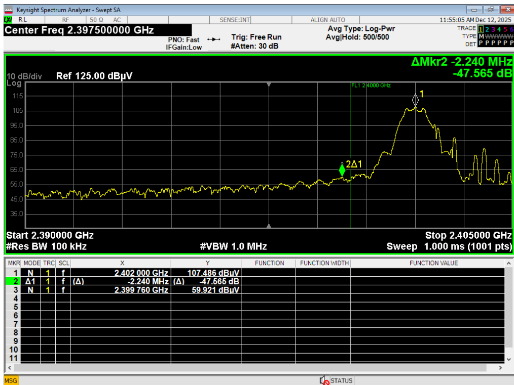
07 LBE Unrestricted, BLE 1MB, 2402MHz, 4dBm
