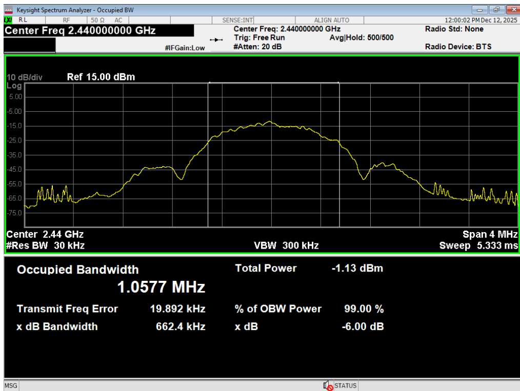
09 Occupied BW, BLE 1MB, 2440MHz, 4dBm
