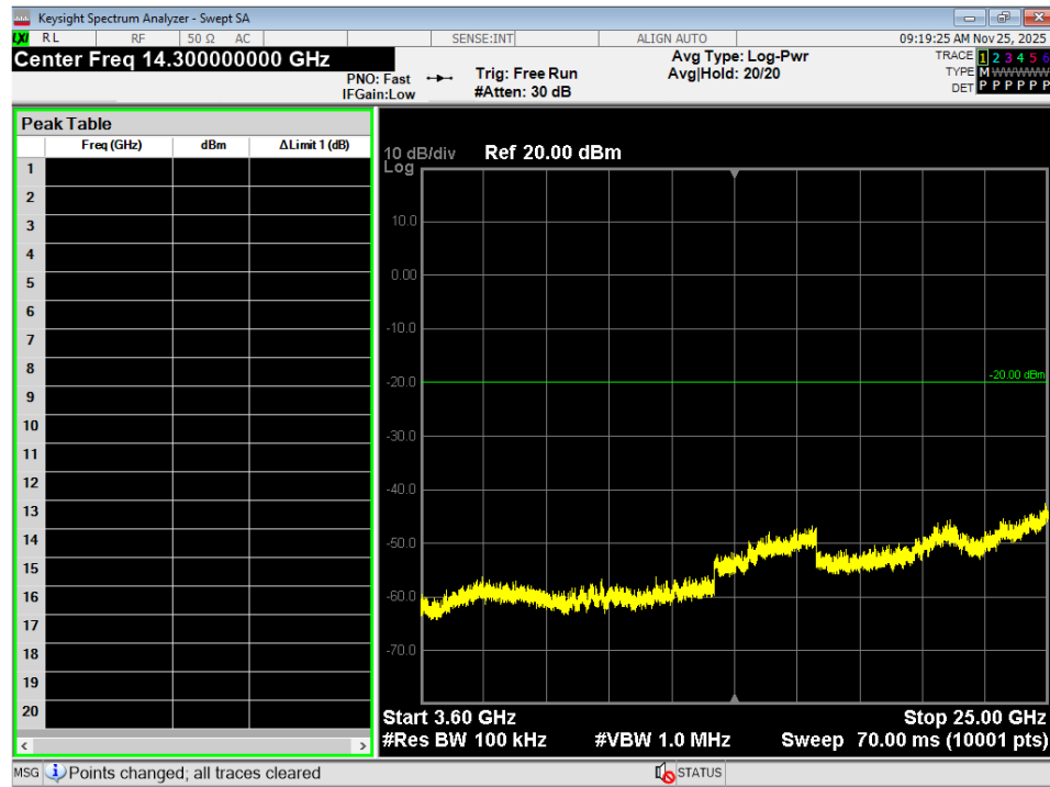
Figure 9 - Conducted Spurious Plot, 3.6 – 25GHz, RX
