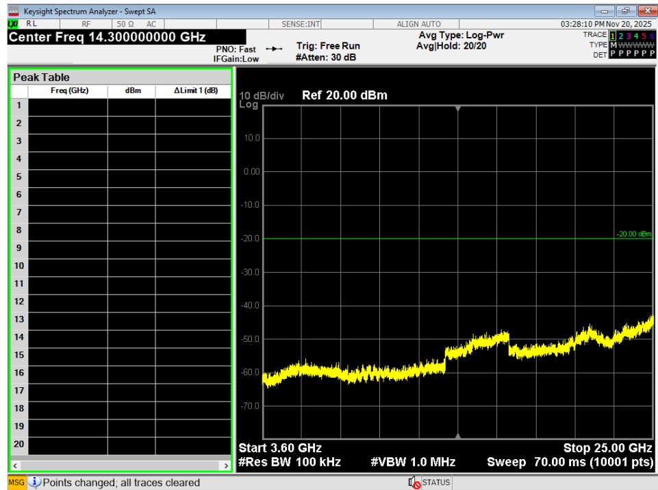
Figure 12 - Conducted Spurious Plot, 3.6GHz – 25GHz, GMSK Low
