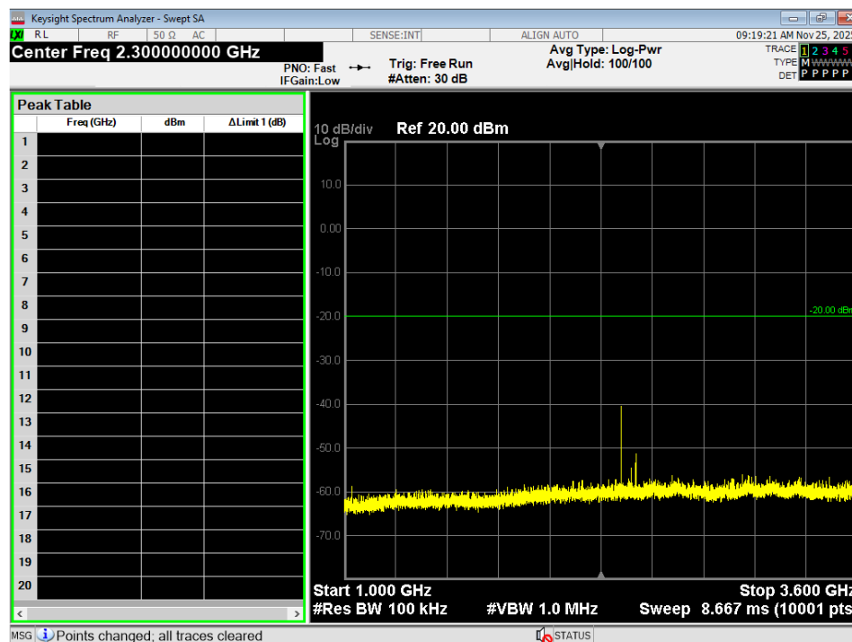
Figure 8 - Conducted Spurious Plot, 1 – 3.6GHz, RX
