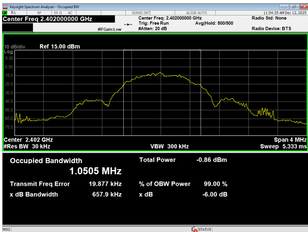
08 Occupied BW, BLE 1MB, 2402MHz, 4dBm
