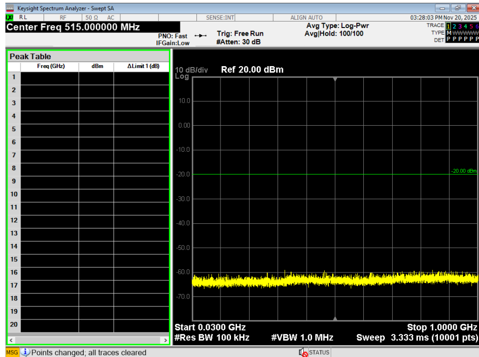
Figure 10 - Conducted Spurious Plot, 30MHz – 1GHz, GMSK Low
