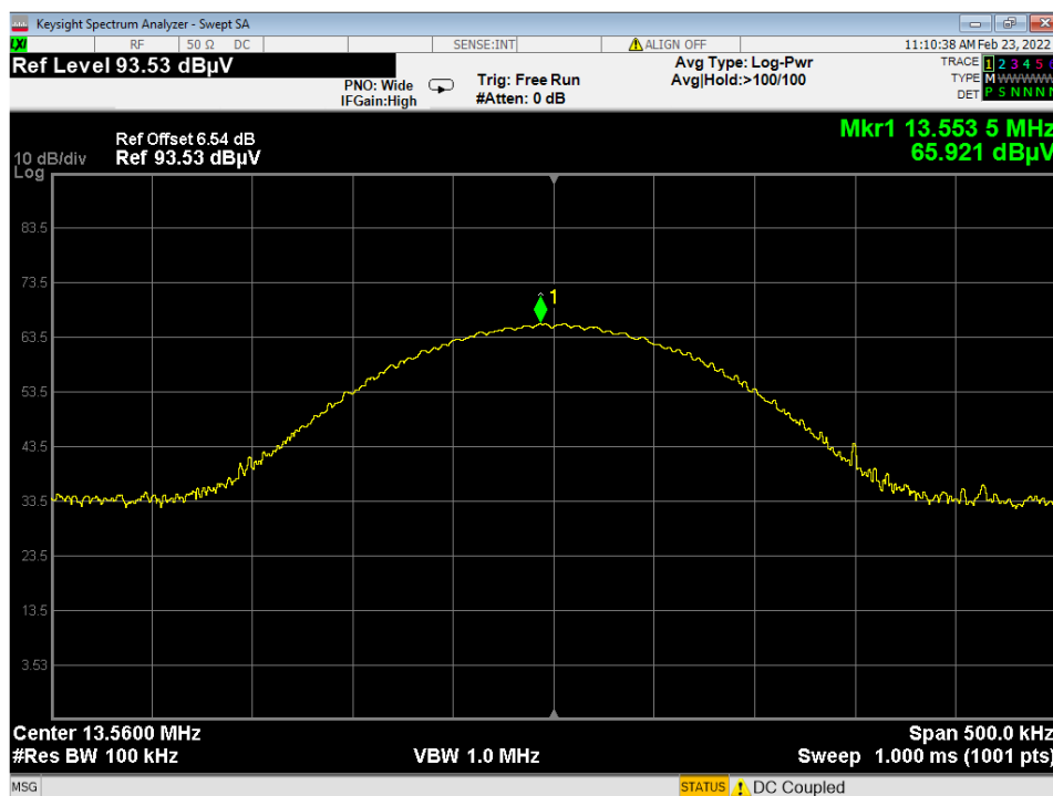
Figure 3 – NFC Field Strength Plot Corrections included
