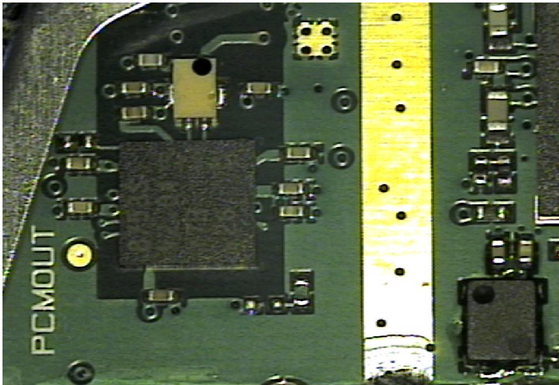
Transmitter section without shield front side.
