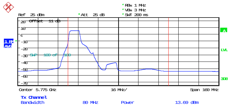
MAXIMUM CONDUCTED POWER ANT2_AX80_CH155_052RU16 Date: 5.FEB.2026 16:04:13
