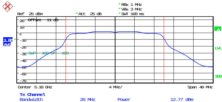
MAXIMUM CONDUCTED POWER ANT2_AX20_CH36_106RU2 Date: 5.FEB.2026 17:21:47
