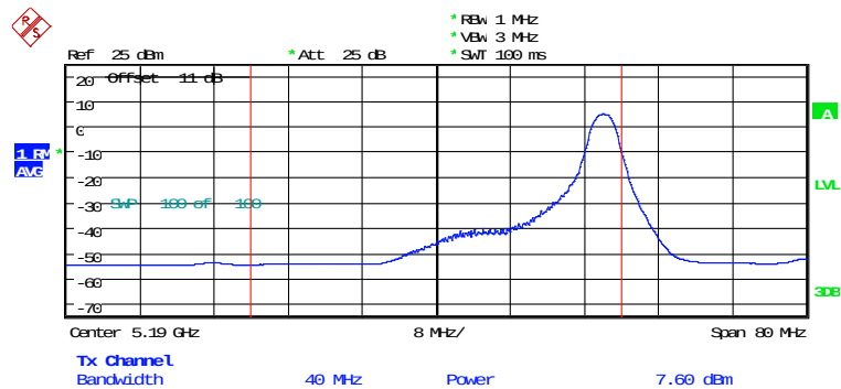
MAXIMUM CONDUCTED POWER ANT2_AX40_CH38_026RU1 Date: 5.FEB.2026 16:26:26
