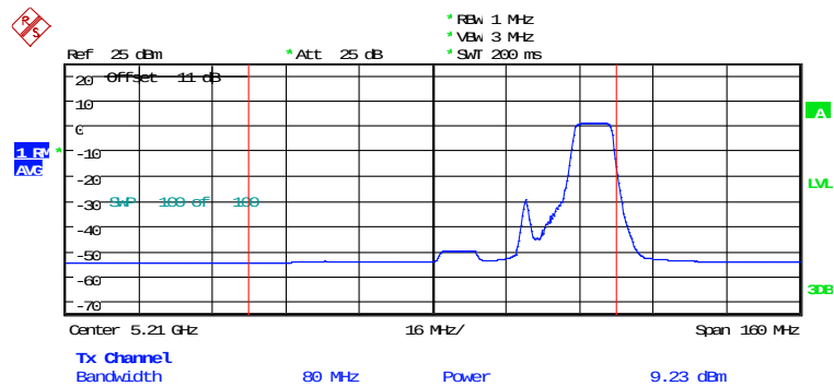
MAXIMUM CONDUCTED POWER ANT2_AX80_CH42_106RU1 Date: 5.FEB.2026 16:19:02
