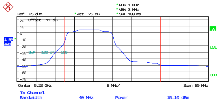
MAXIMUM CONDUCTED POWER ANT2_AX40_CH46_106RU4 Date: 5.FEB.2026 16:36:39
