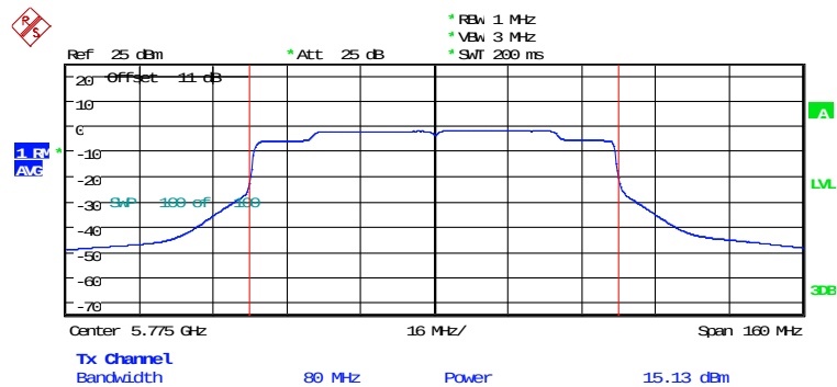
MAXIMUM CONDUCTED POWER ANT2_AX80_CH155_484RU2 Date: 5.FEB.2026 16:11:52
