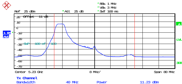
MAXIMUM CONDUCTED POWER ANT1_AX40_CH46_026RU18 Date: 5.FEB.2026 13:35:00
