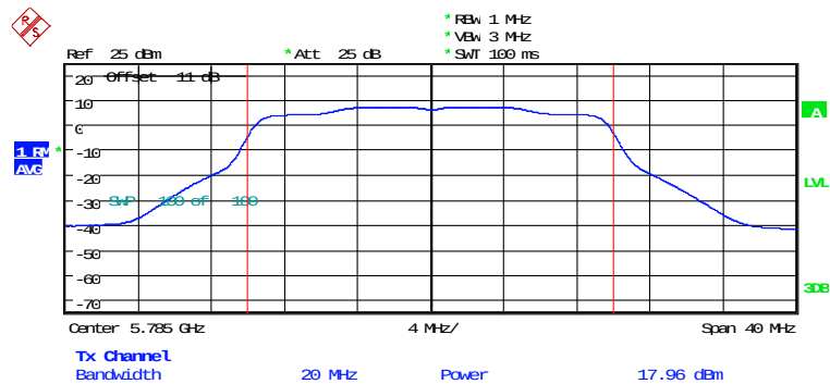
MAXIMUM CONDUCTED POWER ANT1_AX20_CH157_106RU2 Date: 5.FEB.2026 15:05:13
