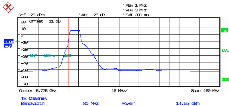
MAXIMUM CONDUCTED POWER ANT1_AX80_CH155_052RU16 Date: 5.FEB.2026 14:11:36
