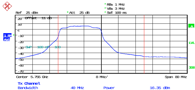
MAXIMUM CONDUCTED POWER ANT2_AX40_CH151_106RU4 Date: 5.FEB.2026 15:47:43
