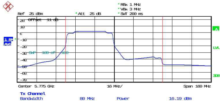
MAXIMUM CONDUCTED POWER ANT2_AX80_CH155_242RU4 Date: 5.FEB.2026 16:10:01
