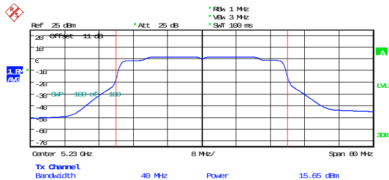
MAXIMUM CONDUCTED POWER ANT2_AX40_CH46_242RU2 Date: 5.FEB.2026 16:37:42
