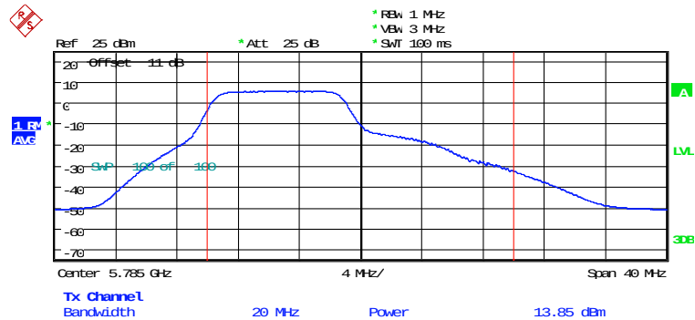
MAXIMUM CONDUCTED POWER ANT2_AX20_CH157_052RU4 Date: 5.FEB.2026 15:25:36
