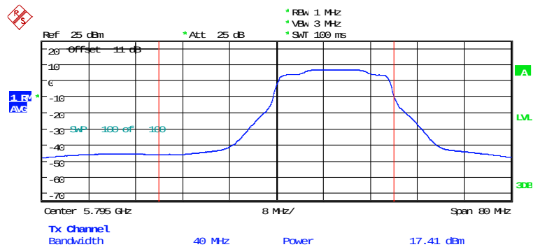
MAXIMUM CONDUCTED POWER ANT2_AX40_CH159_242RU1 Date: 5.FEB.2026 15:57:29
