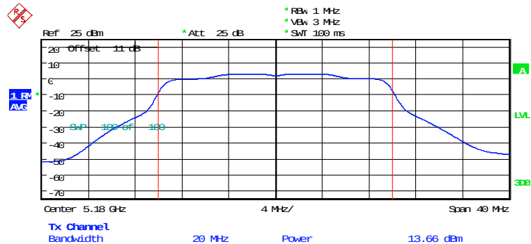
MAXIMUM CONDUCTED POWER ANT1_AX20_CH36_106RU2 Date: 5.FEB.2026 17:24:11
