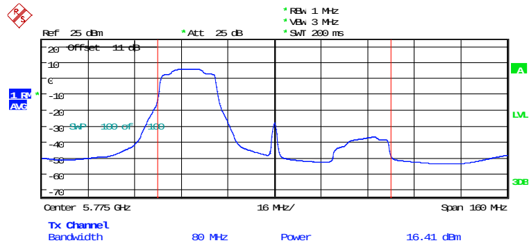
MAXIMUM CONDUCTED POWER ANT2_AX80_CH155_106RU8 Date: 5.FEB.2026 16:07:42
