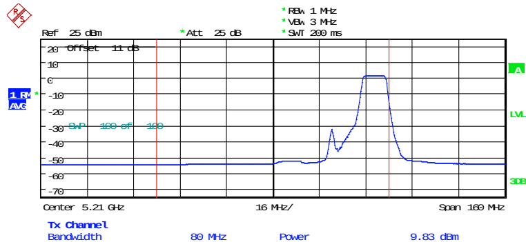
MAXIMUM CONDUCTED POWER ANT1_AX80_CH42_106RU1 Date: 5.FEB.2026 13:56:07
