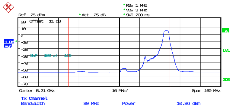
MAXIMUM CONDUCTED POWER ANT2_AX80_CH42_052RU1 Date: 5.FEB.2026 16:17:11
