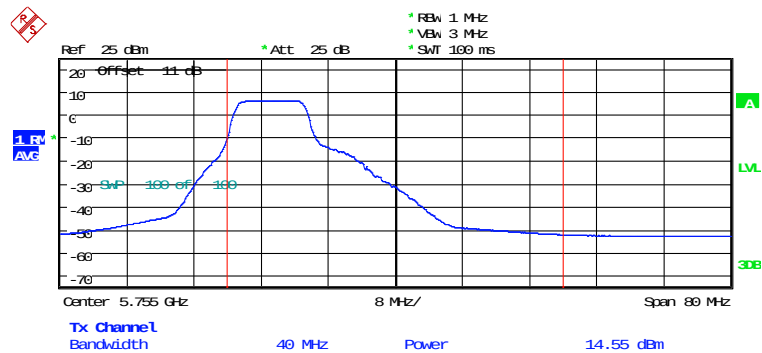
MAXIMUM CONDUCTED POWER ANT1_AX40_CH151_052RU8 Date: 5.FEB.2026 14:28:05
