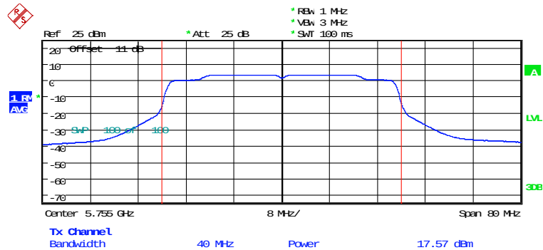
MAXIMUM CONDUCTED POWER ANT1_AX40_CH151_242RU2 Date: 5.FEB.2026 14:30:44
