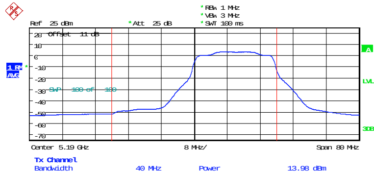
MAXIMUM CONDUCTED POWER ANT1_AX40_CH38_242RU1 Date: 5.FEB.2026 13:31:34
