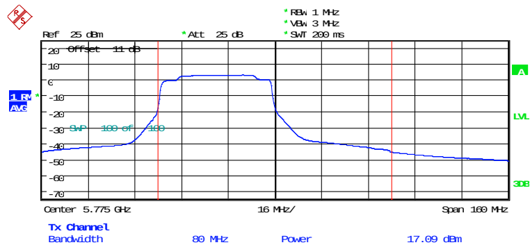
MAXIMUM CONDUCTED POWER ANT1_AX80_CH155_242RU4 Date: 5.FEB.2026 14:16:46
