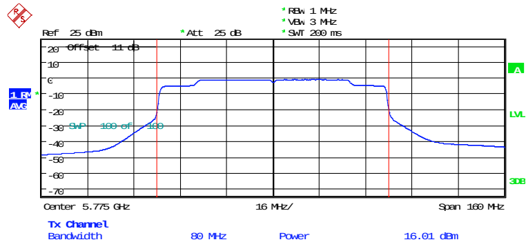
MAXIMUM CONDUCTED POWER ANT1_AX80_CH155_484RU2 Date: 5.FEB.2026 14:18:54
