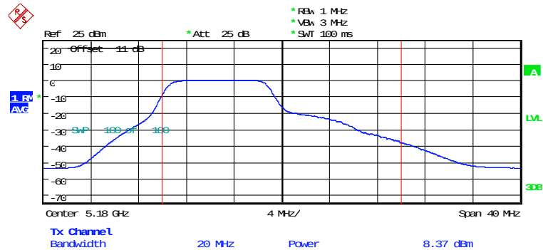
MAXIMUM CONDUCTED POWER ANT2_AX20_CH36_052RU4 Date: 5.FEB.2026 16:42:36
