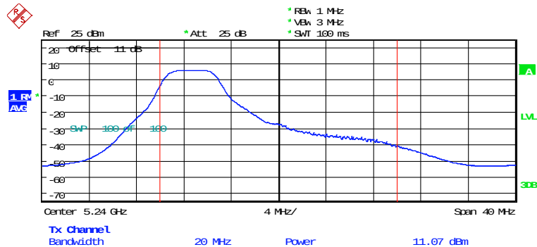
MAXIMUM CONDUCTED POWER ANT1_AX20_CH48_026RU9 Date: 5.FEB.2026 11:54:02
