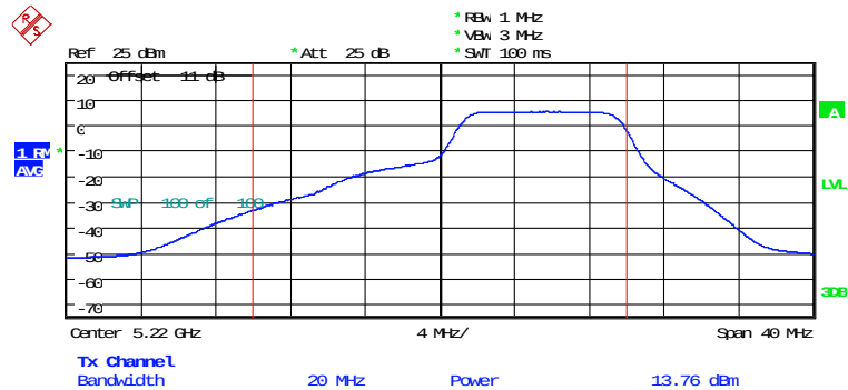
MAXIMUM CONDUCTED POWER ANT2_AX20_CH44_106RU1 Date: 5.FEB.2026 16:47:52
