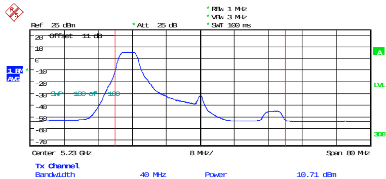
MAXIMUM CONDUCTED POWER ANT2_AX40_CH46_026RU18 Date: 5.FEB.2026 16:34:01
