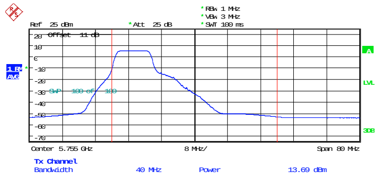
MAXIMUM CONDUCTED POWER ANT2_AX40_CH151_052RU8 Date: 5.FEB.2026 15:45:45
