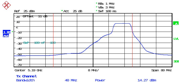
MAXIMUM CONDUCTED POWER ANT1_AX40_CH38_106RU1 Date: 5.FEB.2026 13:29:56
