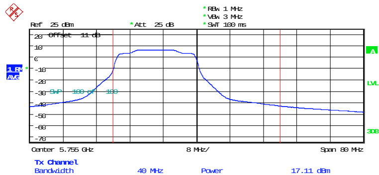
MAXIMUM CONDUCTED POWER ANT1_AX40_CH151_106RU4 Date: 5.FEB.2026 14:29:18
