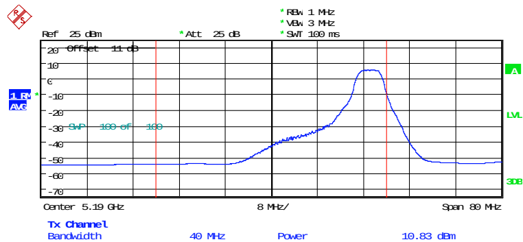
MAXIMUM CONDUCTED POWER ANT2_AX40_CH38_052RU1 Date: 5.FEB.2026 16:27:47
