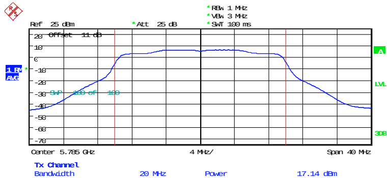
MAXIMUM CONDUCTED POWER ANT2_AX20_CH157_106RU2 Date: 5.FEB.2026 15:30:19
