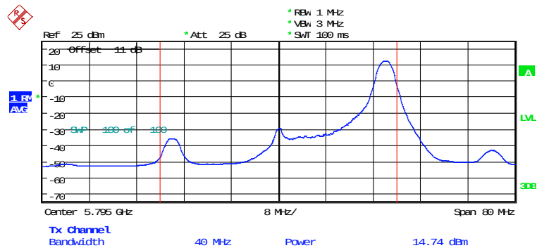
MAXIMUM CONDUCTED POWER ANT1_AX40_CH159_026RU1 Date: 5.FEB.2026 14:33:41
