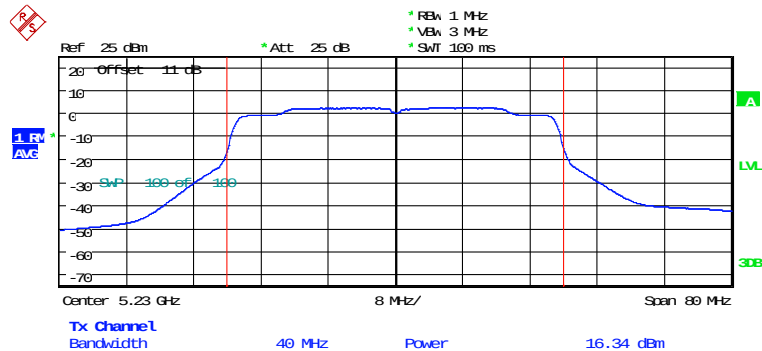
MAXIMUM CONDUCTED POWER ANT1_AX40_CH46_242RU2 Date: 5.FEB.2026 13:38:42
