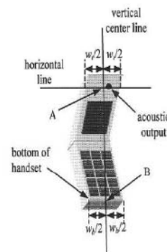
Fig 10.2.2 Handset vertical and horizontal reference lines—"clam-shell case"
