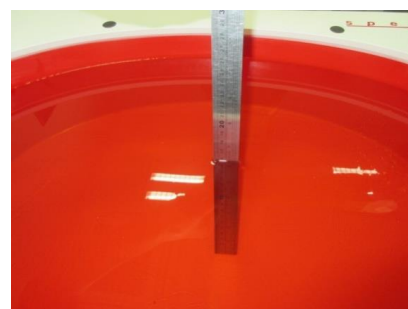
Liquid depth in the flat Phantom ( \geq 15\text{cm} depth) HSL(2450MHz) HSL(5GHz)
