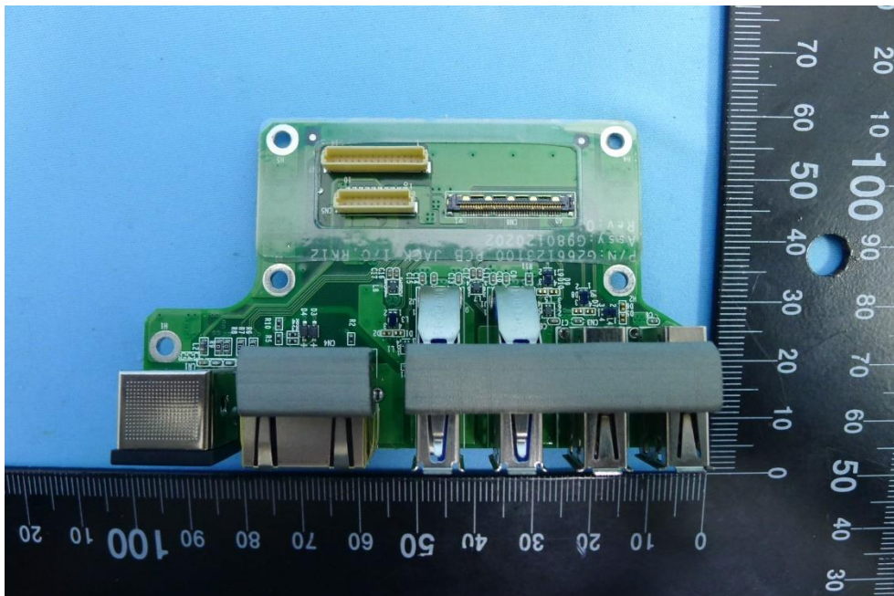
(43) EUT Photo
