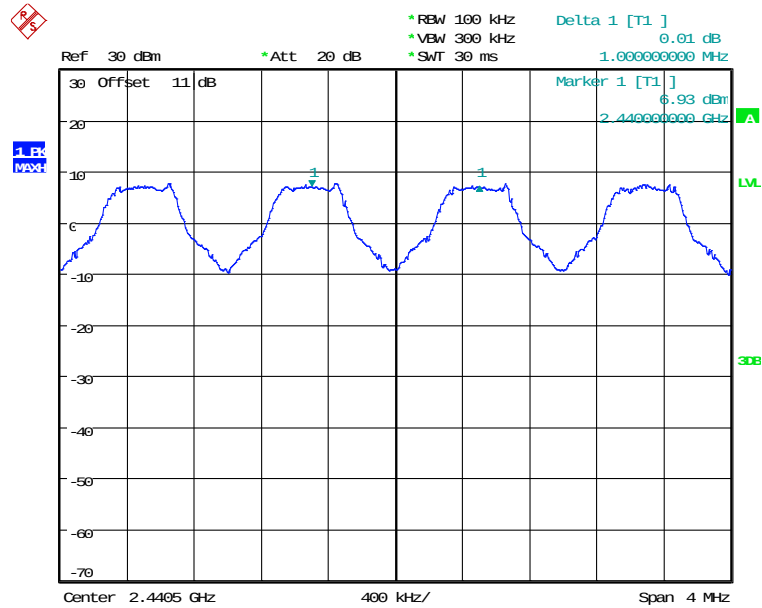
FREQUENCY SEPARATION CH39 Date: 5.AUG.2023 17:49:56
