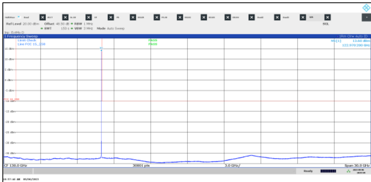
Plot 42: 115 GHz – 145 GHz, stop mode, high frequency, EUT 2
