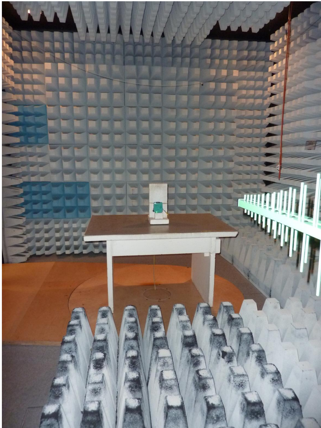
136258_a.JPG: IUH-F190-V1-FR2-02, test set-up fully anechoic chamber
