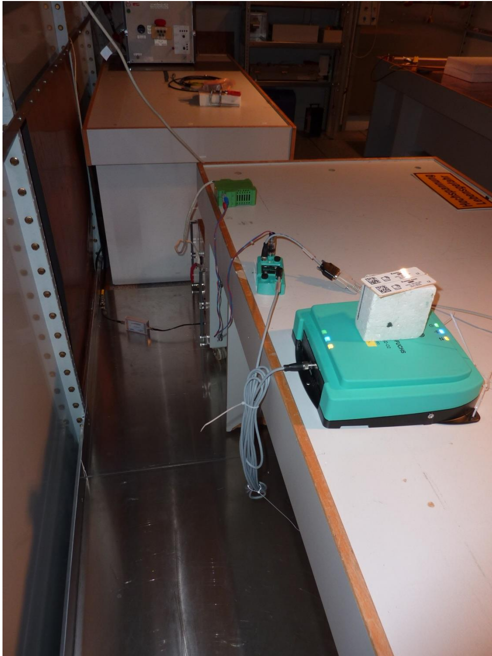
152117_a.JPG: IUH-F192-V1-FR2-02, test set-up shielded room
