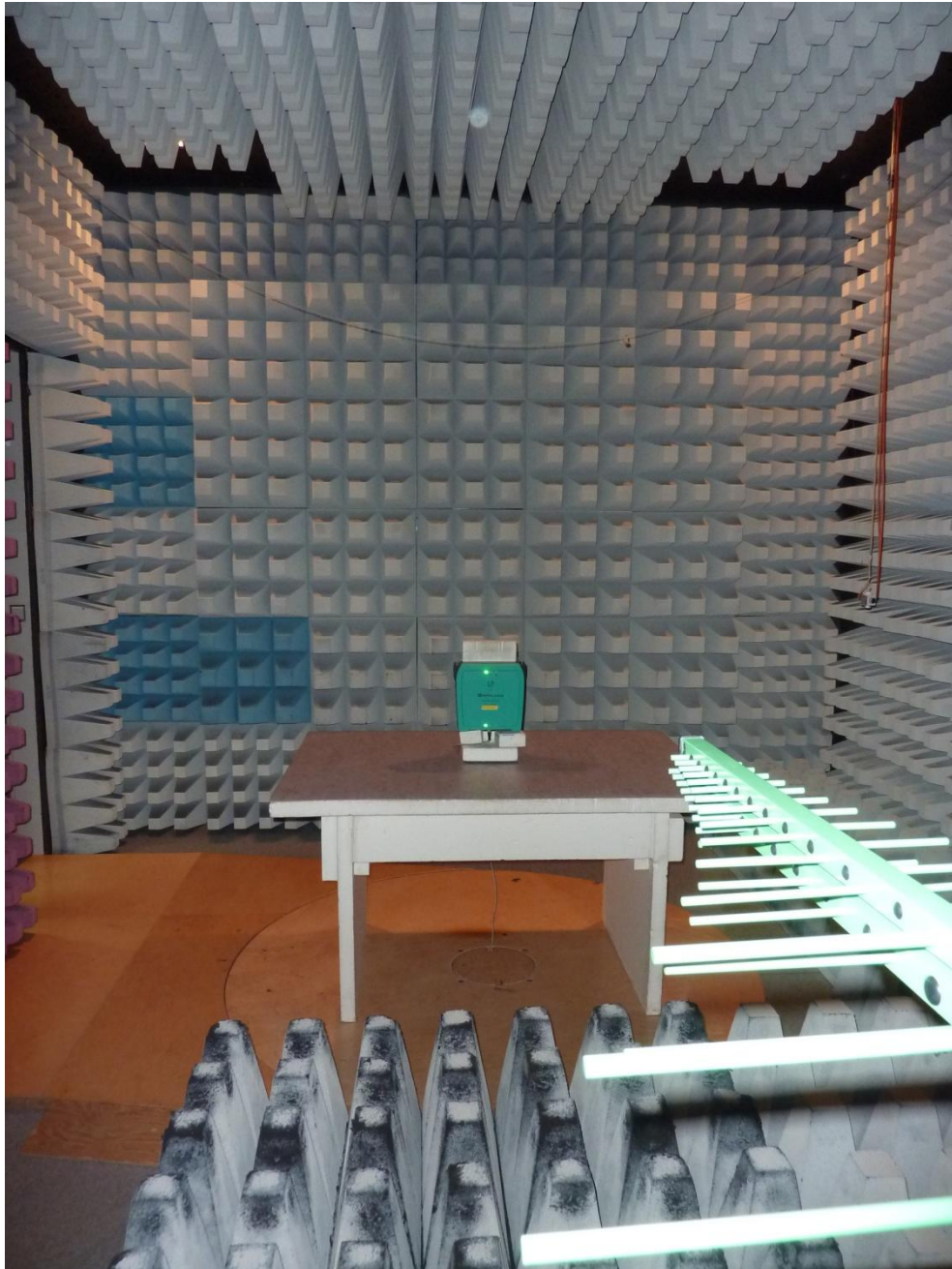
152117_d.JPG: IUH-F192-V1-FR2-02, test set-up fully anechoic chamber
