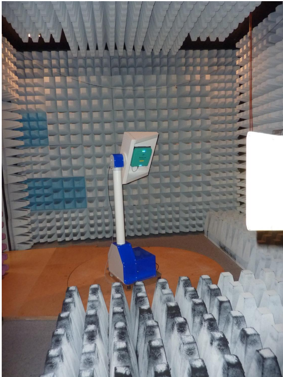
152117_b.JPG: IUH-F192-V1-FR2-02, test set-up fully anechoic chamber
