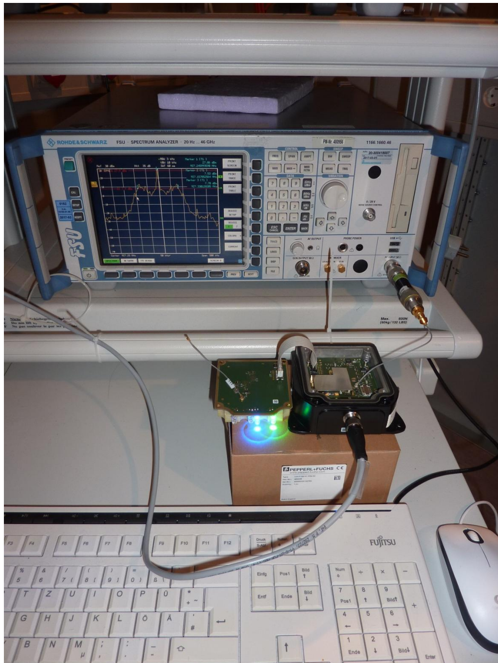
171663_k.JPG: IUHF190V1B, shielded chamber 1
