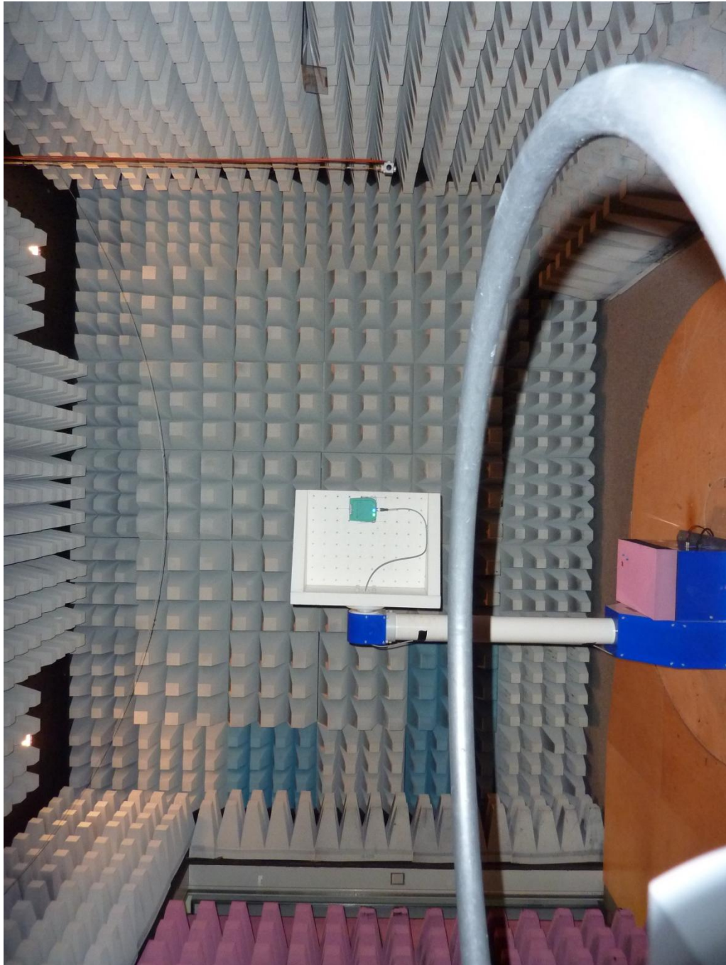
171663_f.JPG: IUHF190V1B, test setup fully anechoic chamber
