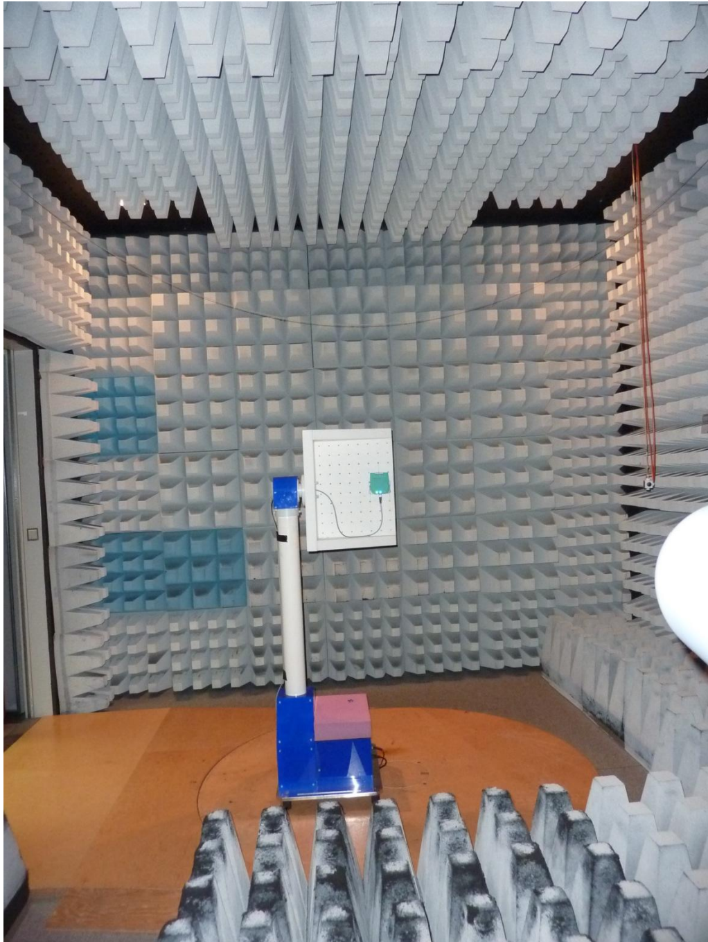
171663_d.JPG: IUHF190V1B, test setup fully anechoic chamber
