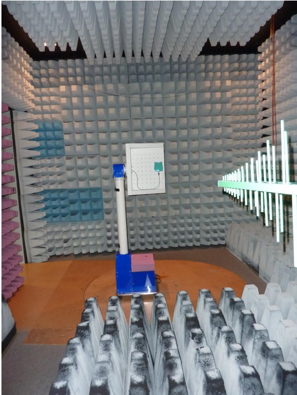
171663_c.JPG: IUHF190V1B, test setup fully anechoic chamber
