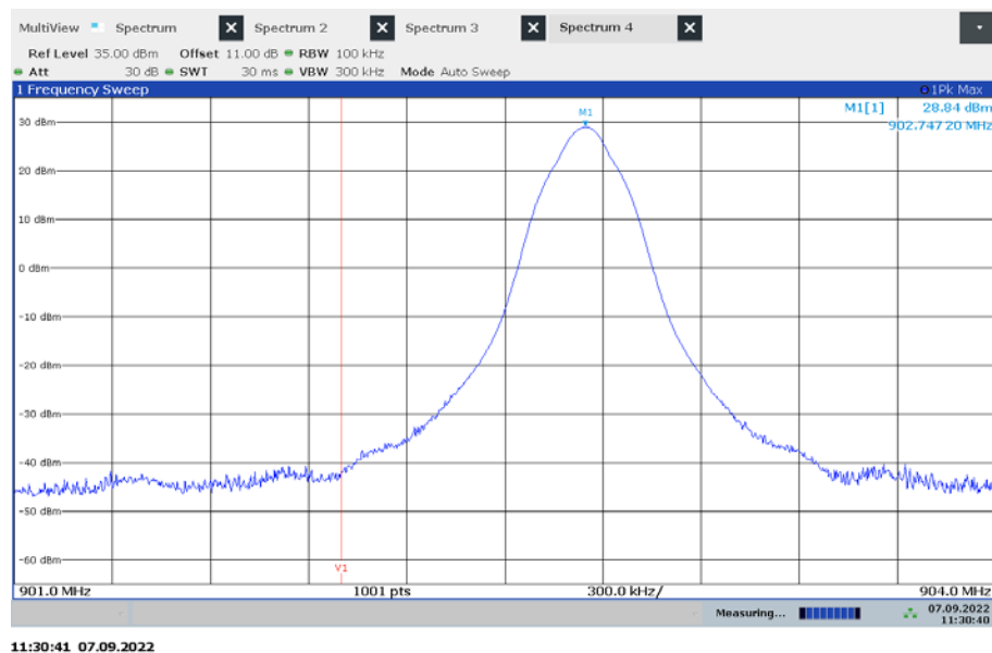
Plot 2: 20 dB – hopping off, lower band edge
