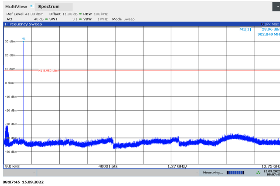
Plot 1: Low channel, 9 kHz – 12.75 GHz
