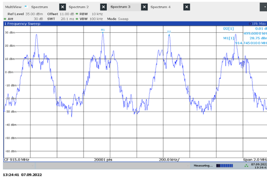
Plot 1: Frequency separation
