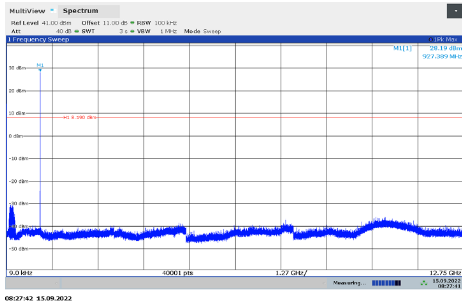
Plot 5: High channel, 9 kHz – 12.75 GHz
