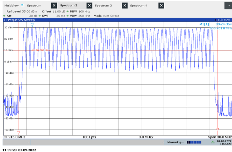
Plot 1: 20 dB – hopping on
