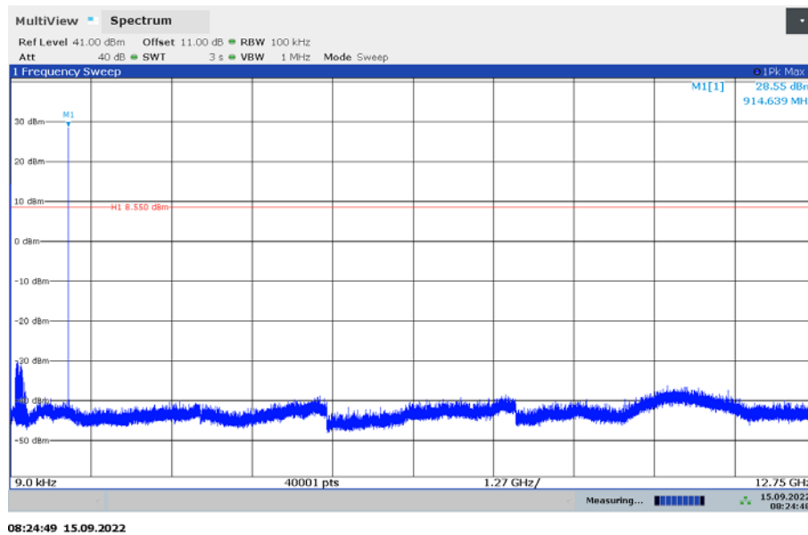
Plot 3: Middle channel, 9 kHz – 12.75 GHz
