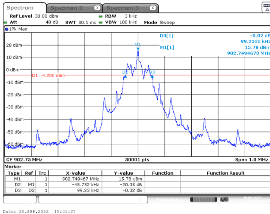
Plot 1: low Channel 20dB bandwidth
