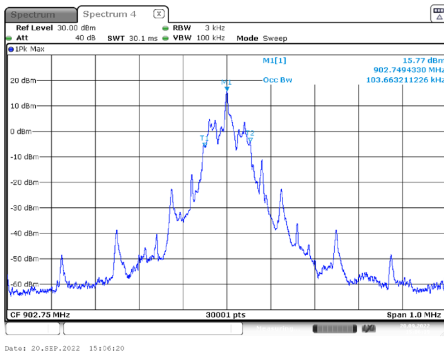
Plot 2: low Channel 99% bandwidth
