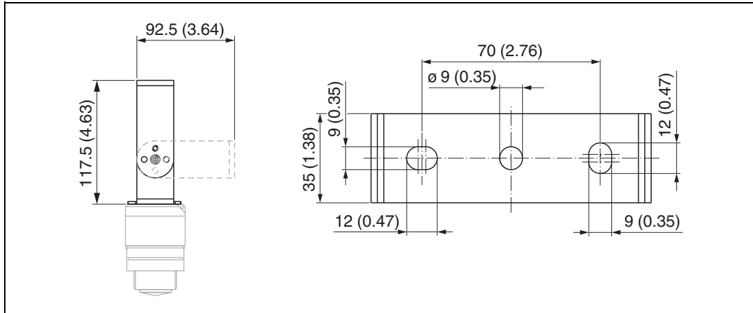
Figure 16.4 Dimensions of mounting bracket, engineering unit: mm (inch)
