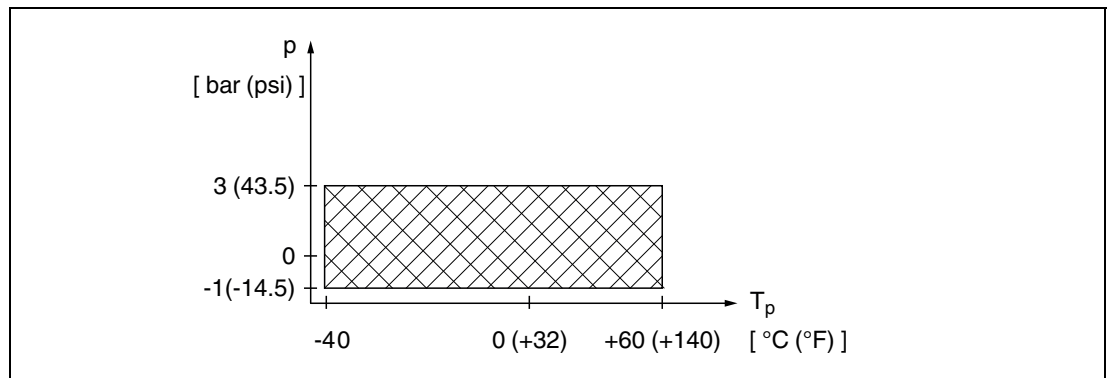
Figure 11.1 Permitted range for process temperature and process pressure
