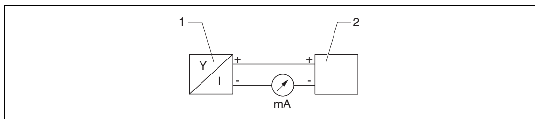
Figure 7.3 Block diagram of HART connection
