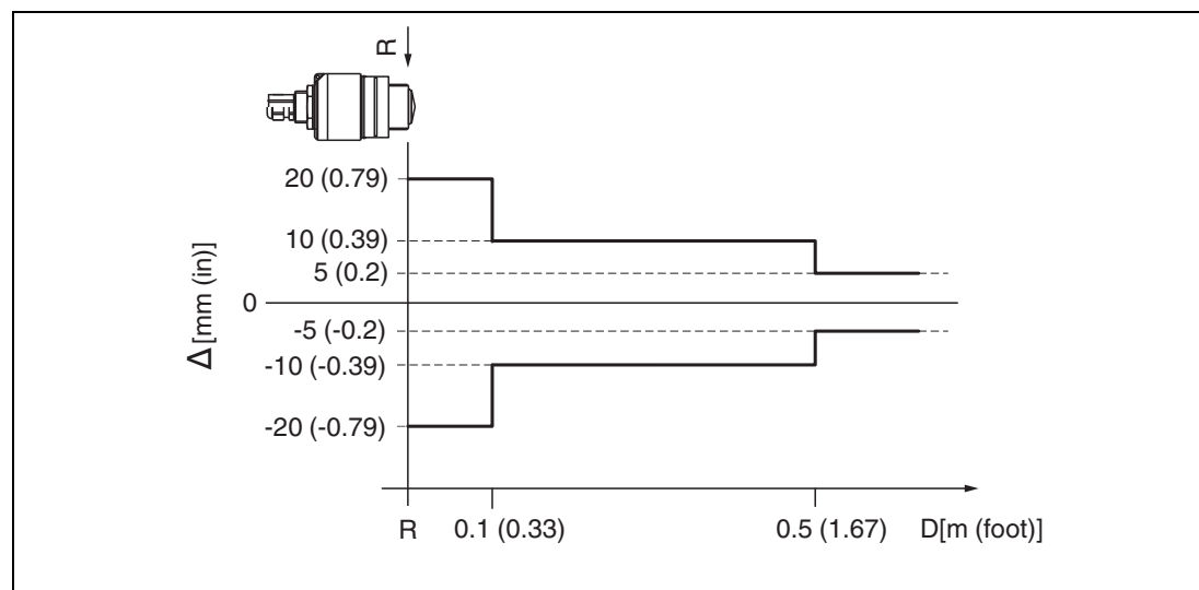
Figure 8.1 Maximum measured error in near-range applications; values for standard version
