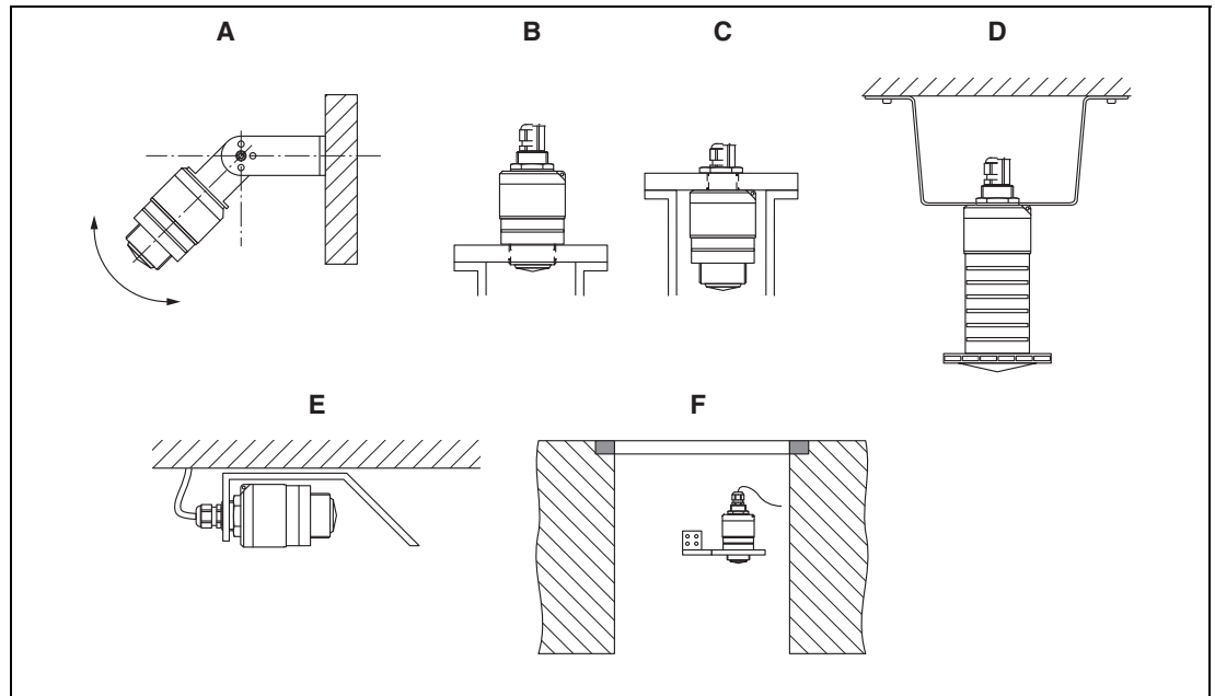
Figure 9.1 Wall, ceiling or nozzle installation
