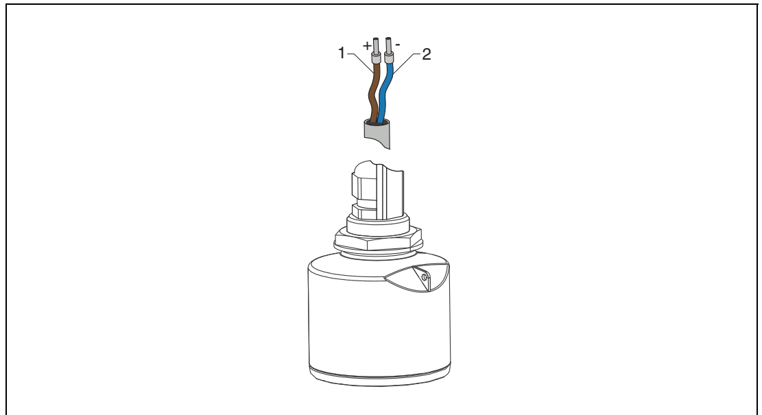
Figure 7.1 Cable assignment
