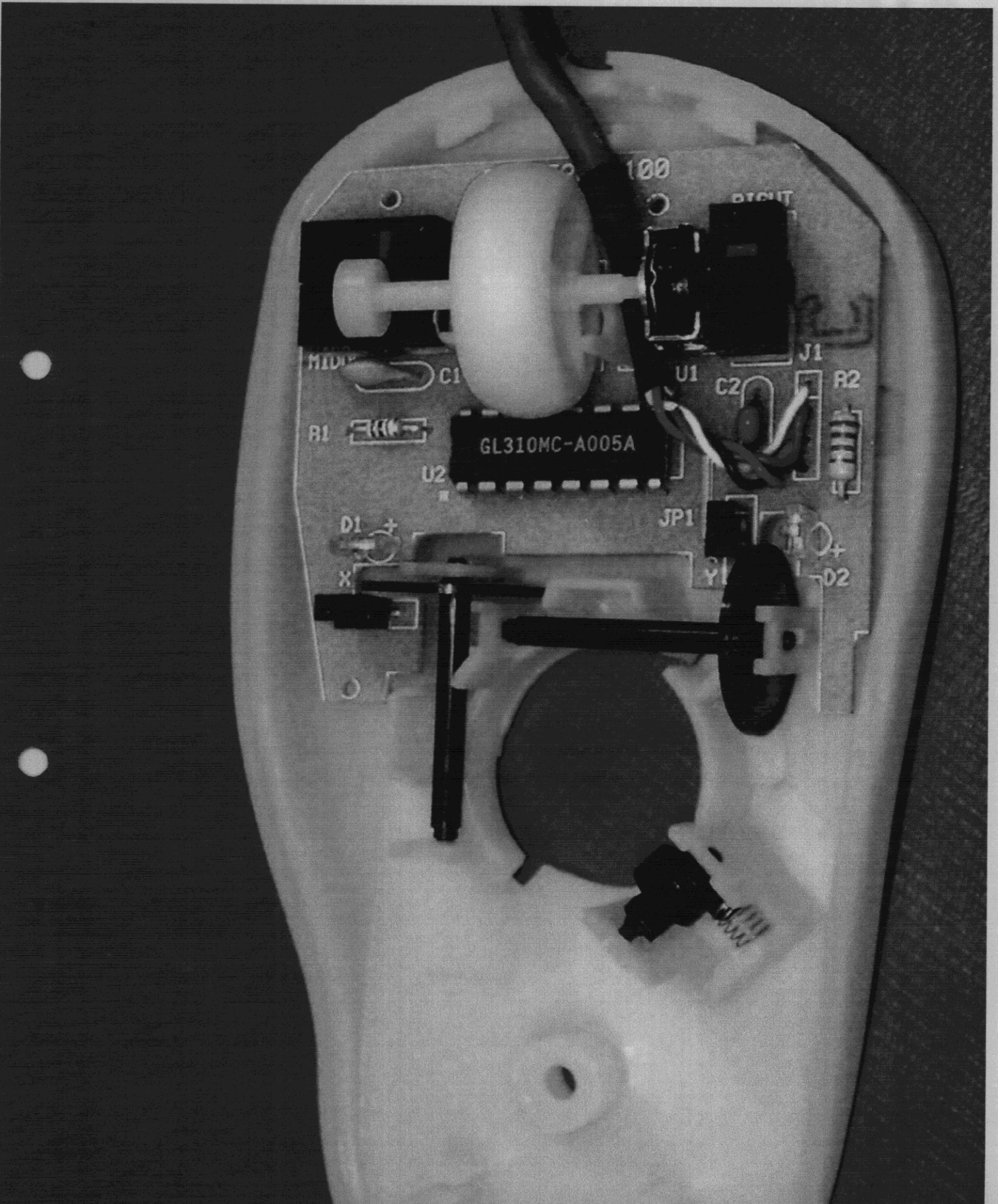
PHOTO 3. EUT COMPONENT SIDE VIEW
