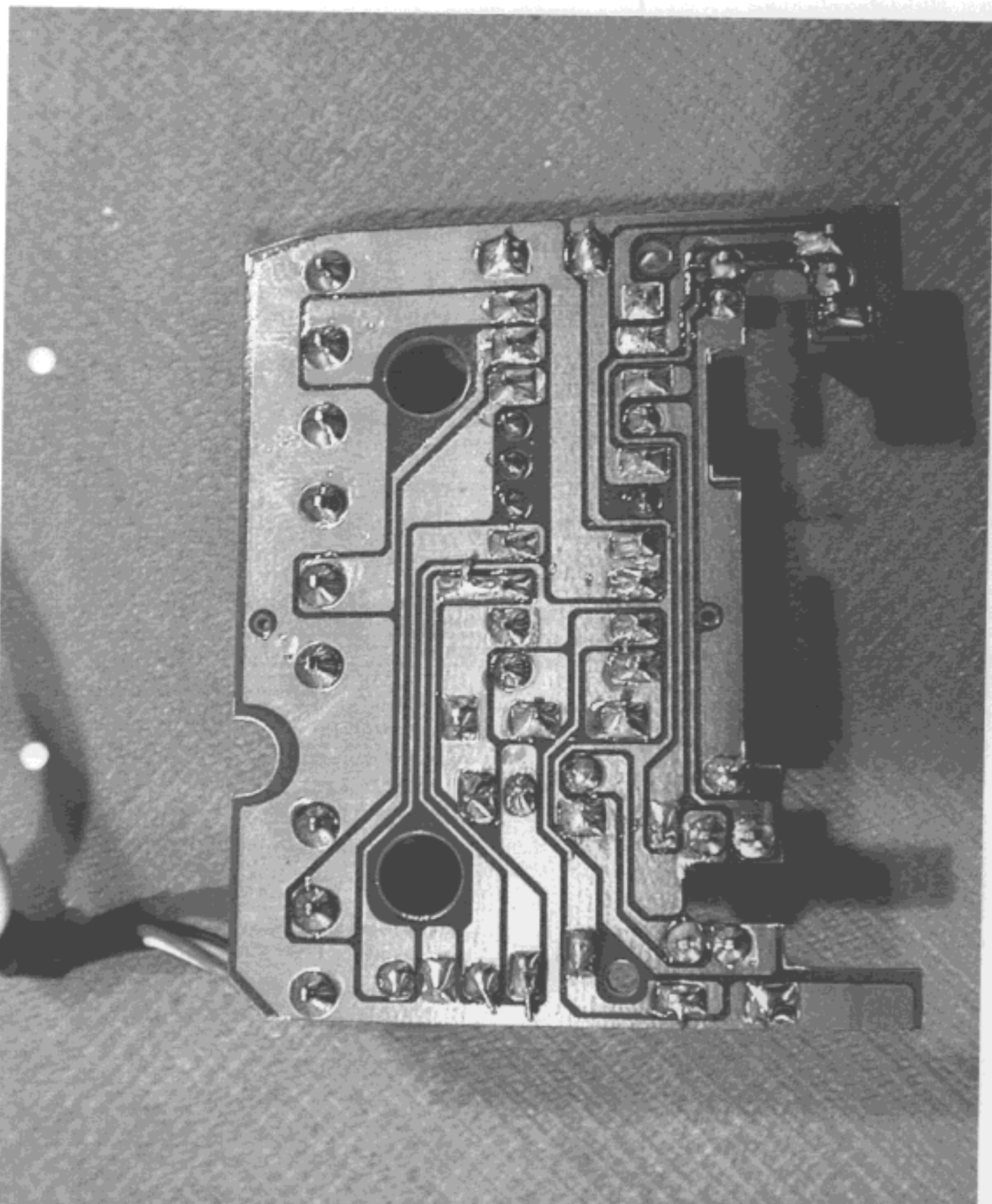
PHOTO 5. EUT SOLDERING SIDE VIEW
