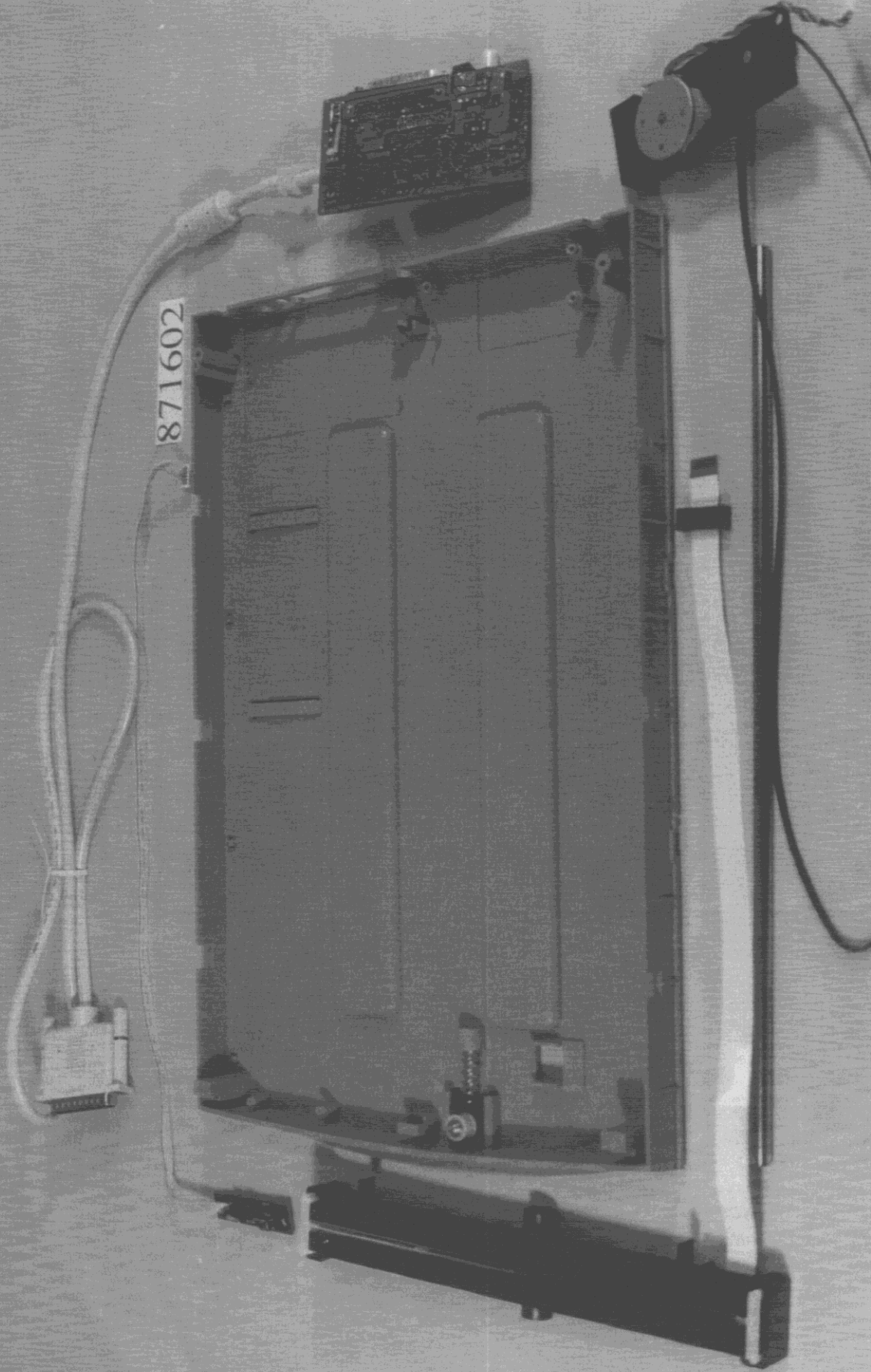
FCC ID: ITEUECVS12P Mechanical Construction
