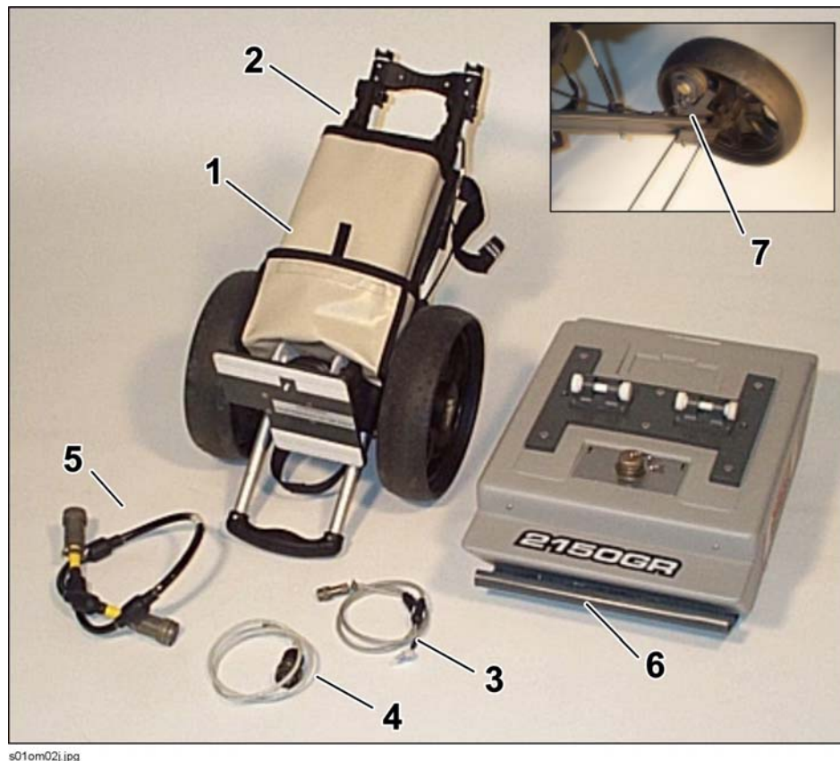
Fig. 3-1 – Overview of the 2150GR and its components
