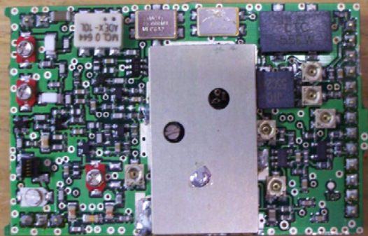
Radio Board top with shield
