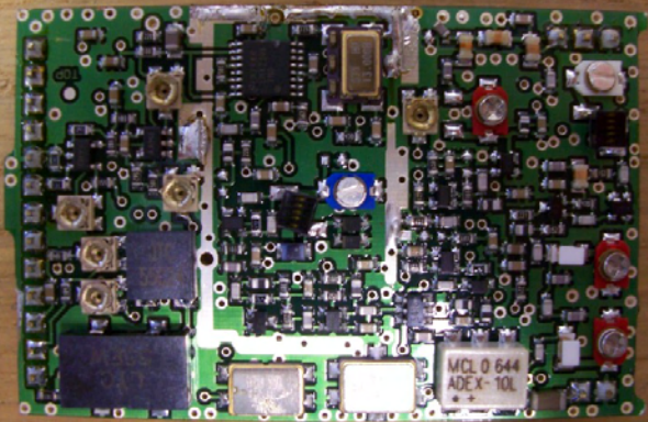
Radio Board top without shield
