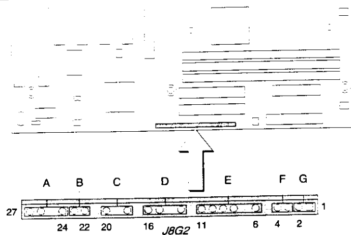
Figure 16. Front Panel Connectors
