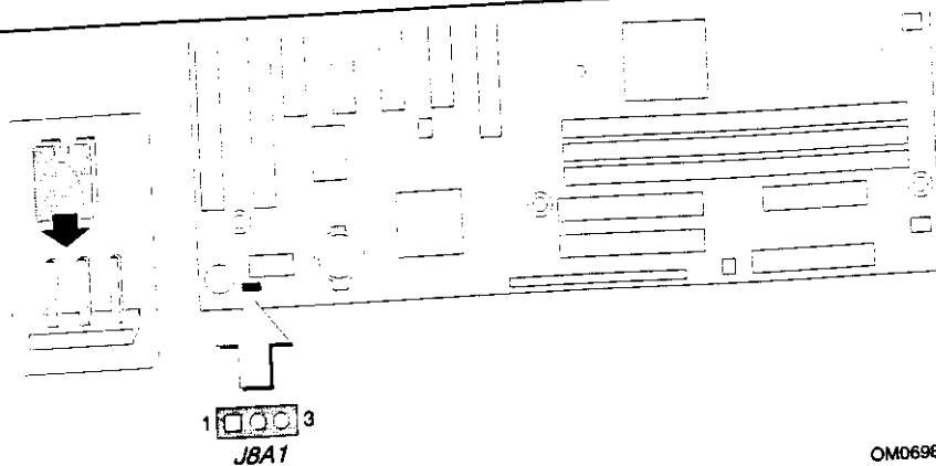
Figure 7. Location of the Configuration Jumper Block
