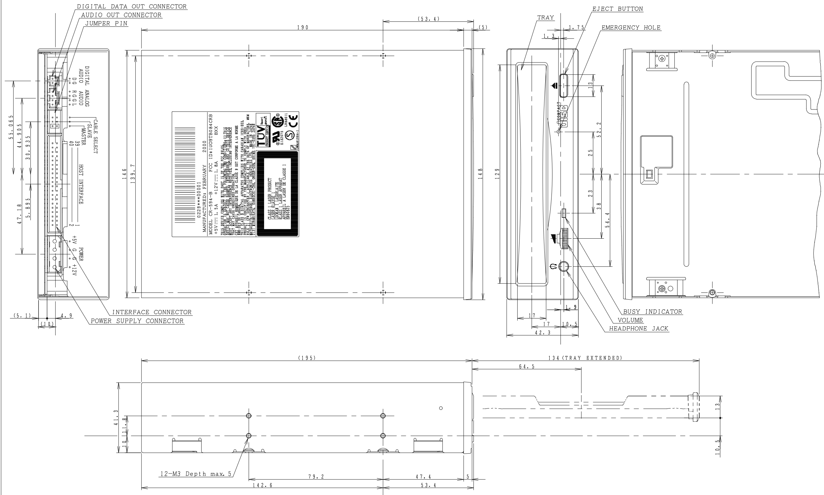
CR-594-B CD-ROM DRIVE APPEARANCE MATSUSHITA-KOTOBUKI ELECTRONICS INDUSTRIES 02.29.2000
