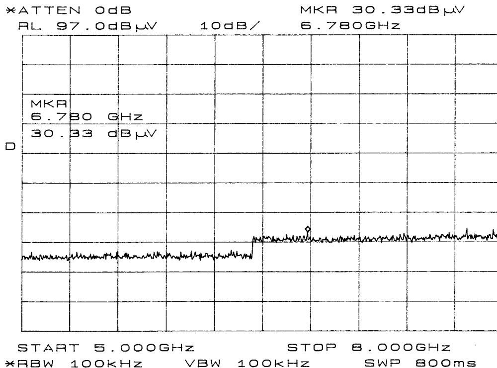
Figure 12 Emissions @ 1 Meter in Screen Room
