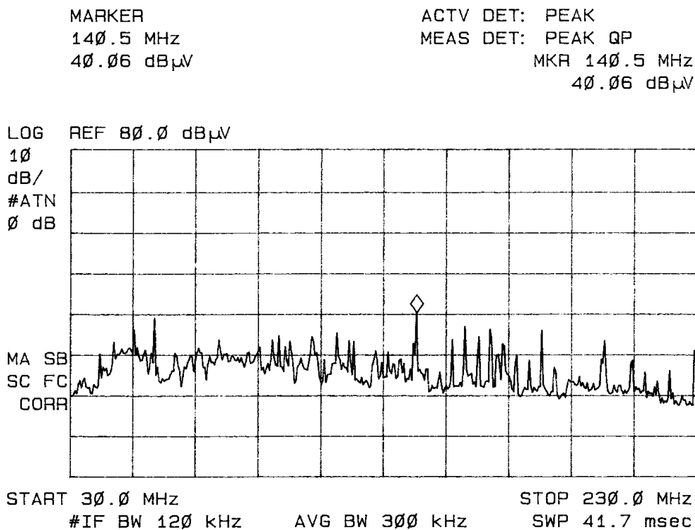
Figure 7 Radiated Emissions taken in screen room (Support Equipment only).
