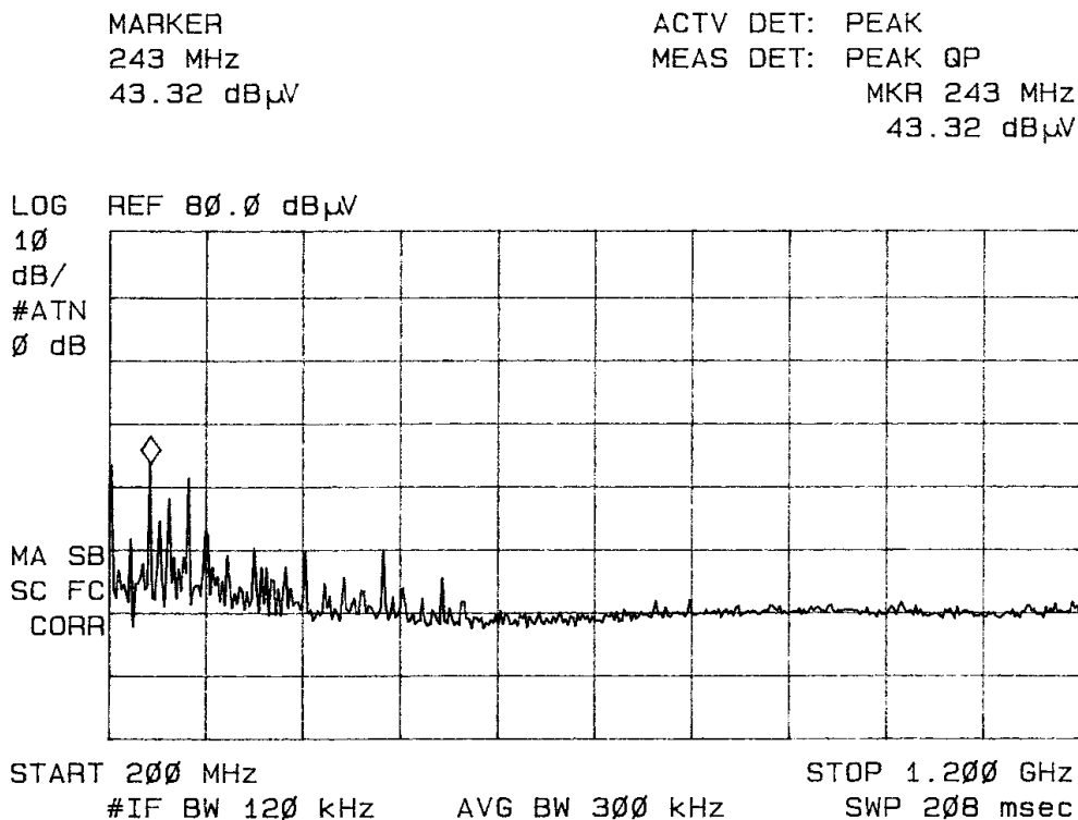
Figure 6 Radiated Emissions taken in screen room (EUT and support equipment).
