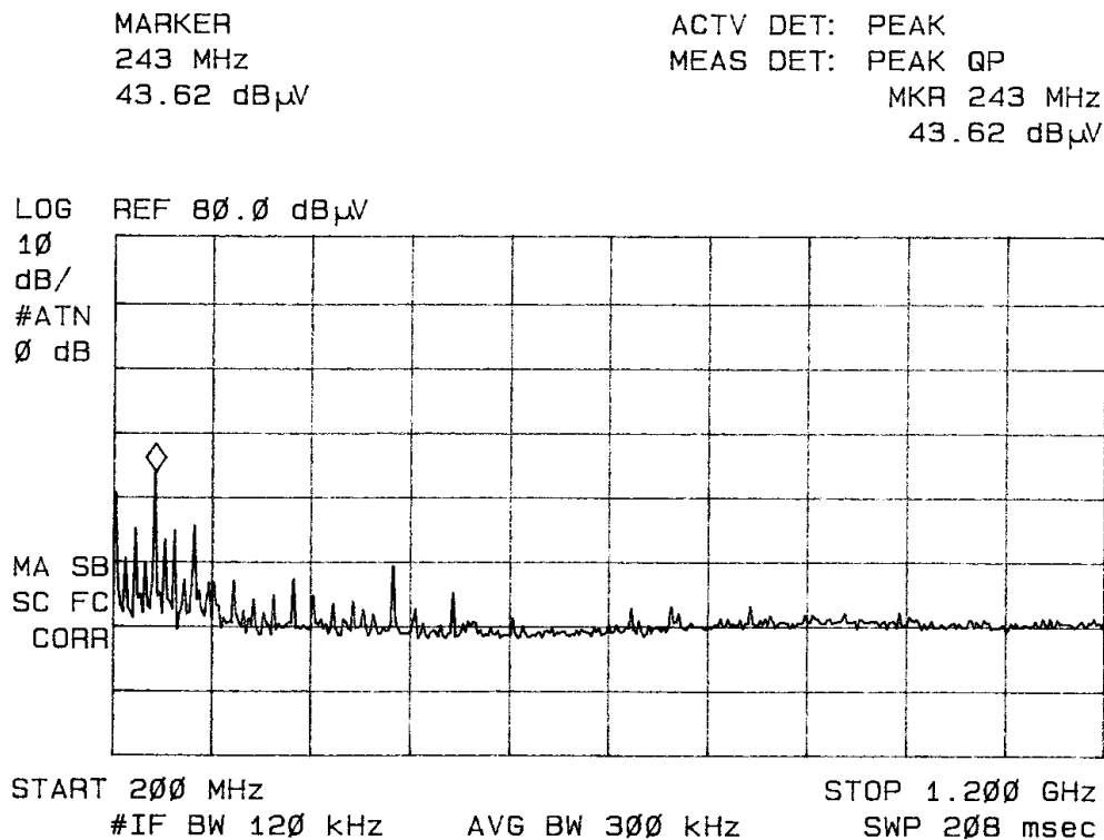
Figure 4 Radiated Emissions taken in screen room (EUT only).
