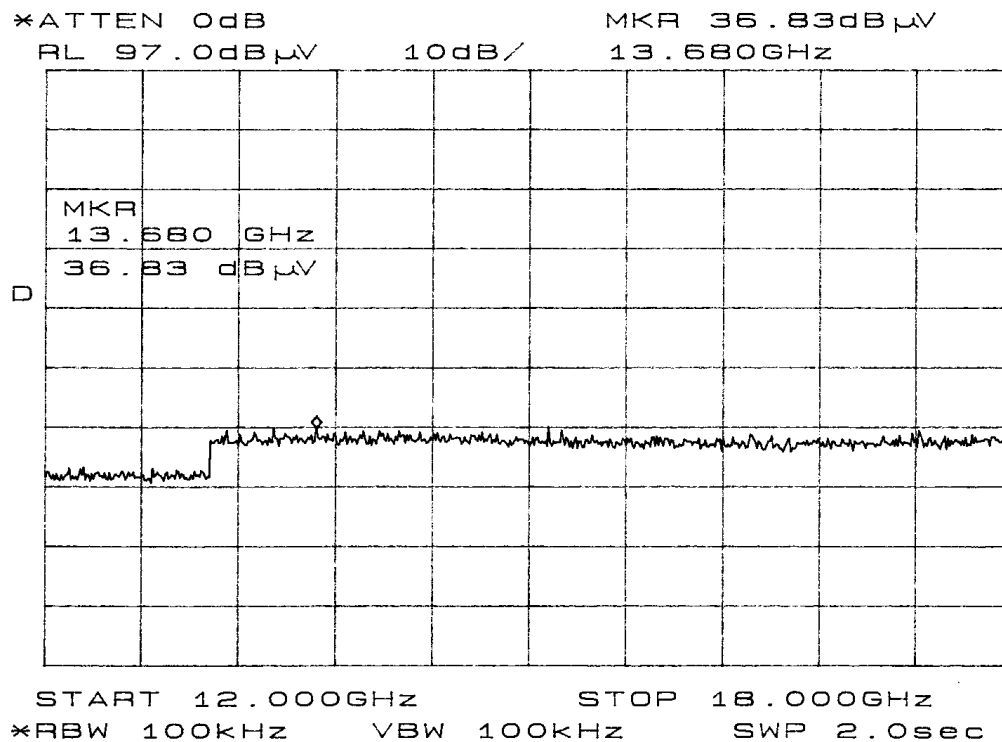
Figure 14 Emissions @ 1 Meter in Screen Room
