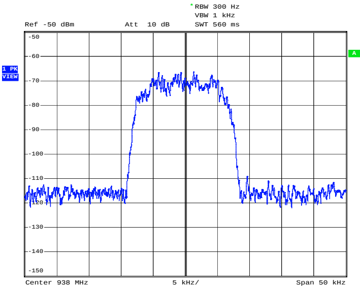
Downlink Input in 935-941MHz Band Date: 3.MAY.2005 13:46:15
