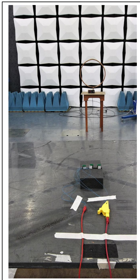
Loop Antenna
