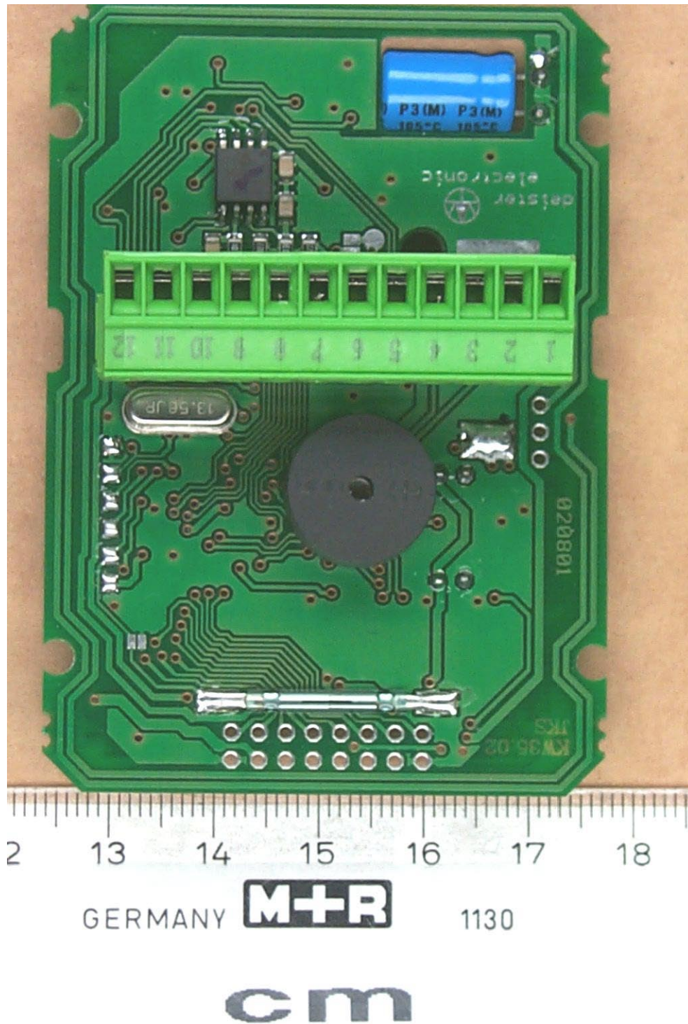
20646_1.jpg Model 240 (PRA5) PCB, top view
