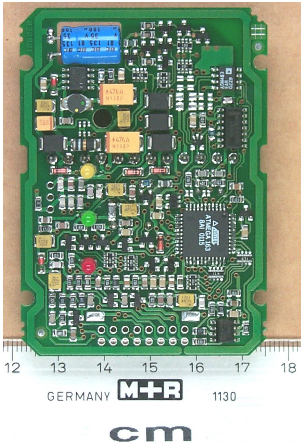
20646_4.jpg Model 240 (PRA5) PVB, bottom view
