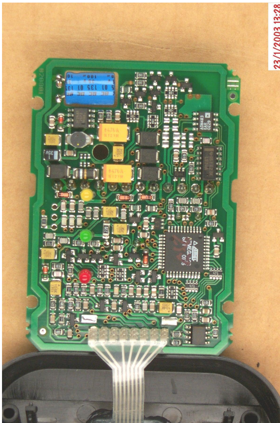
30013eut2.jpg PCB, front view
