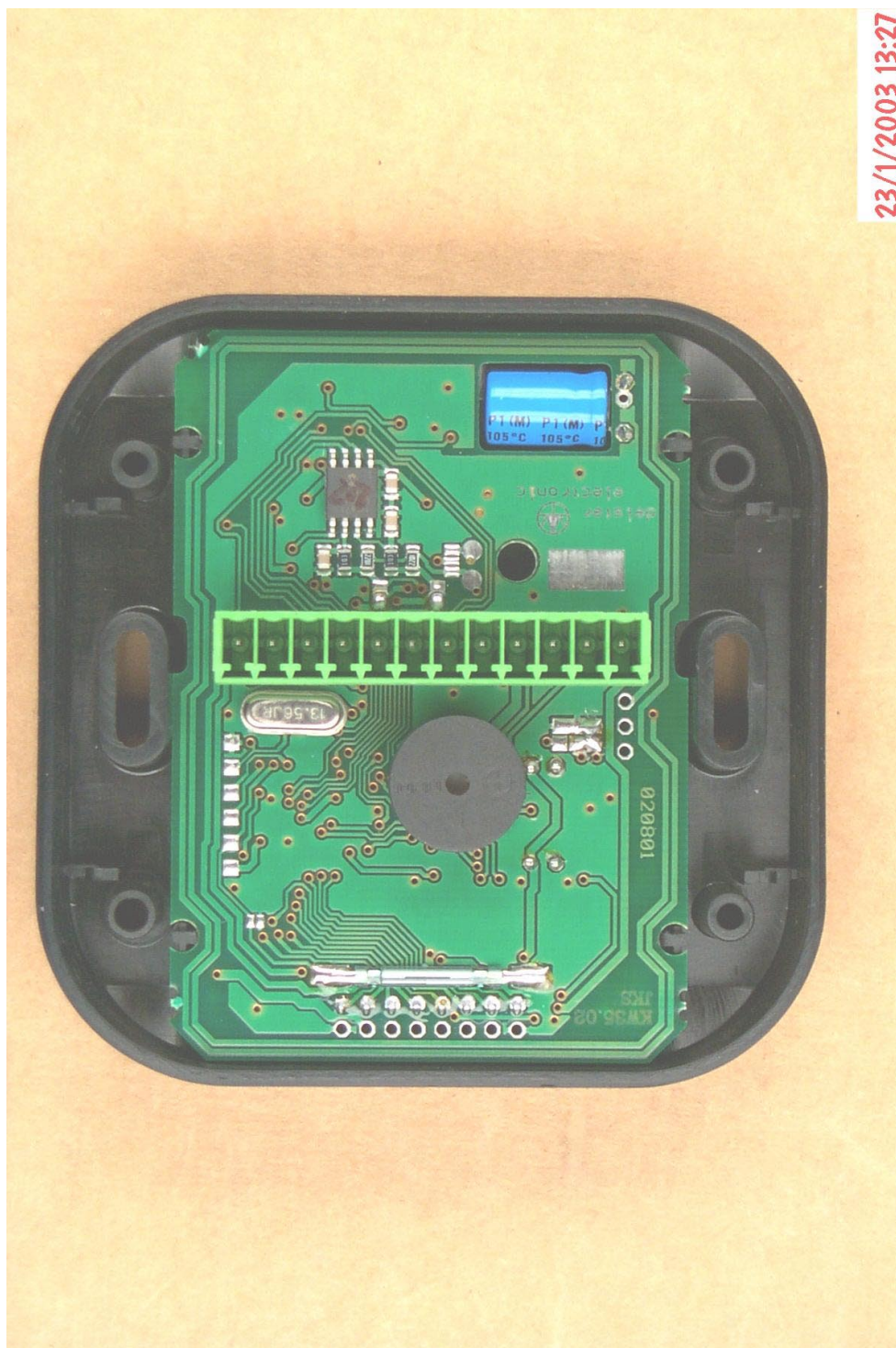
30013eut3.jpg EUT, inside view
