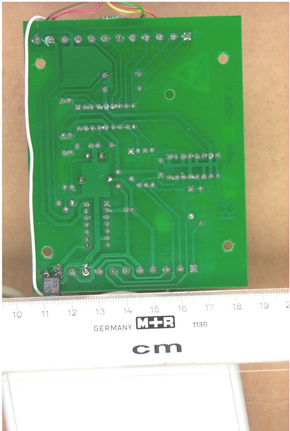
30422_6.jpg Model 24W PCB, bottom view
