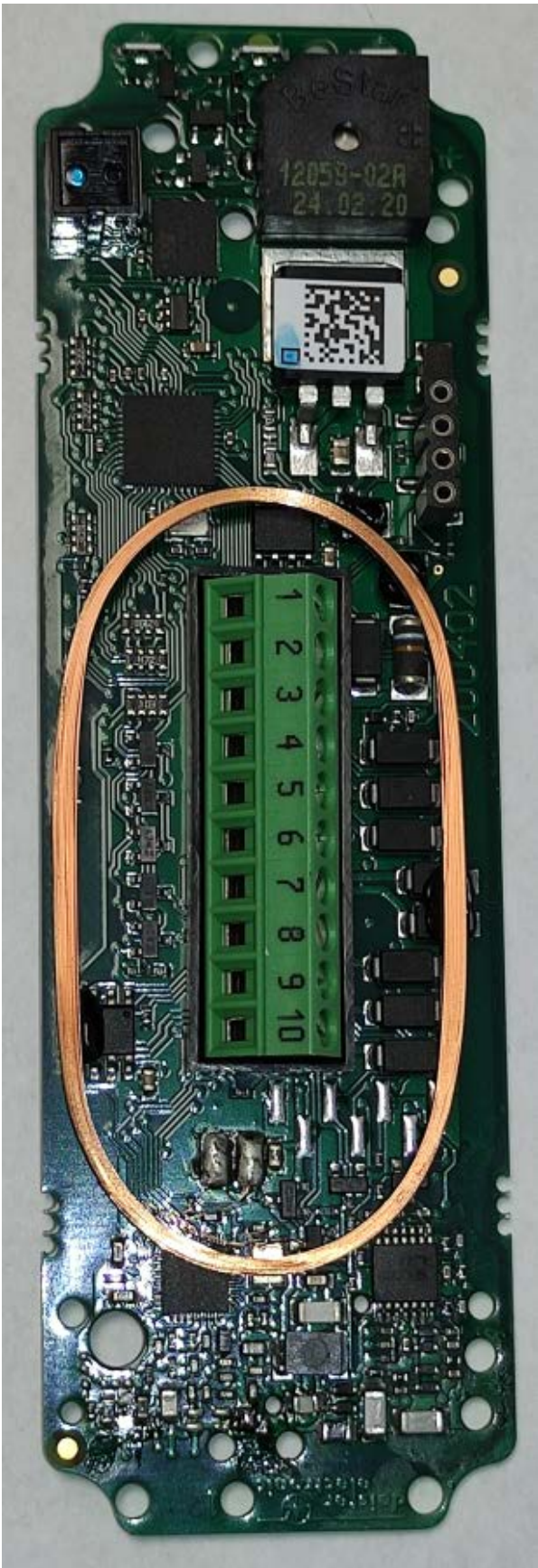
Circuit Board Rear
