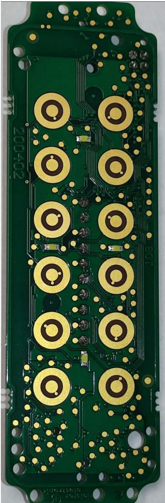
Circuit Board Front
