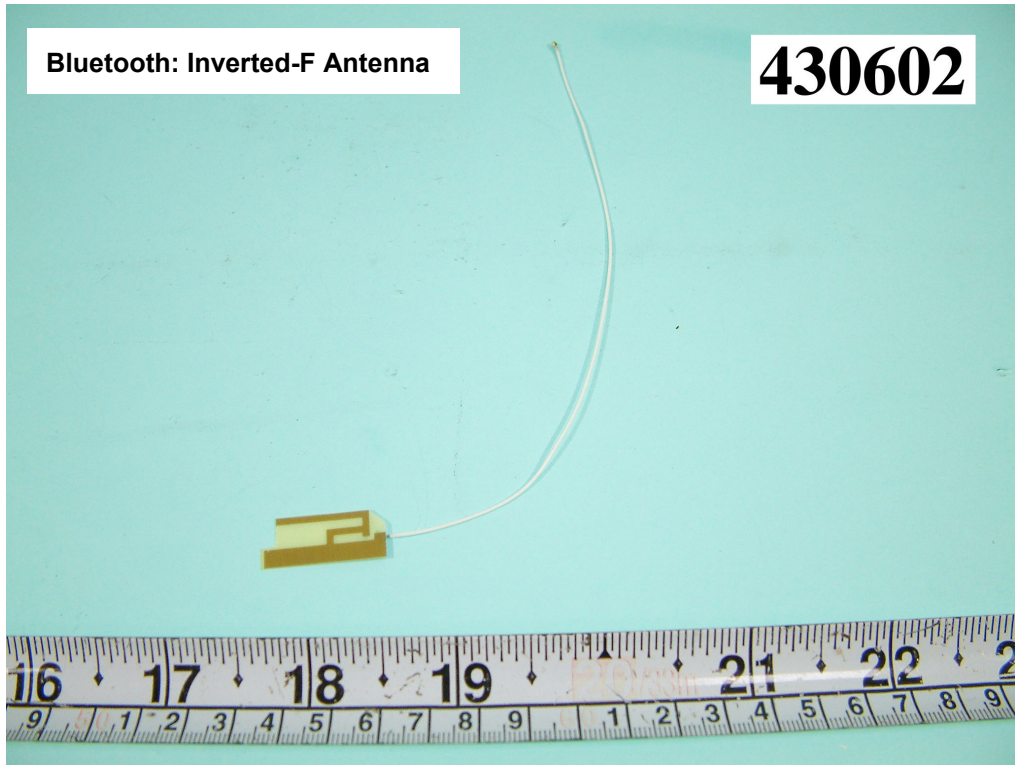
Bluetooth: Inverted-F Antenna
